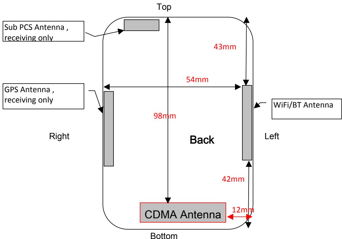
Figure 4.7 Antenna Distance to device edges
