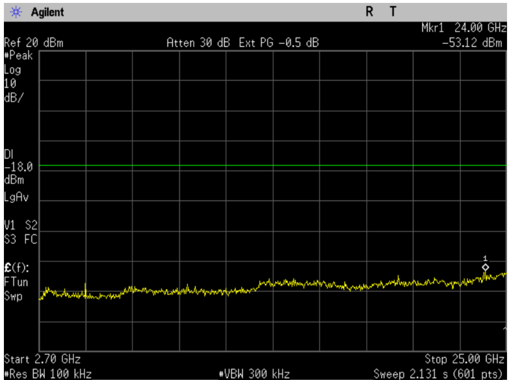
Figure 10-2c2: Conducted Spurious Emissions, 802.11g, Ch 11
