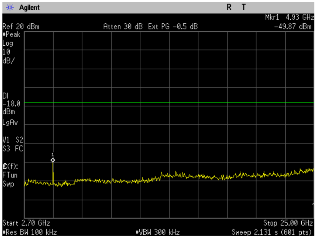
Figure 10-1c2: Conducted Spurious Emissions, 802.11b, Ch 11
