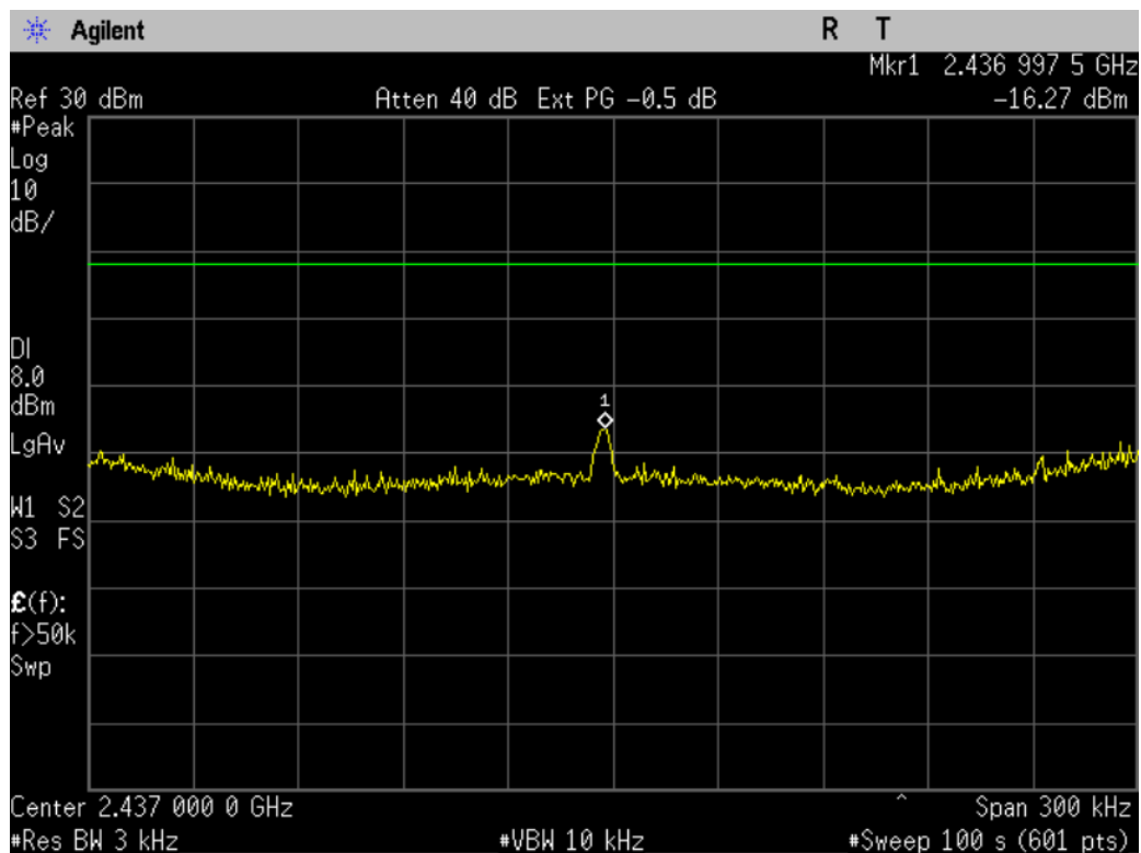
Figure 8-2b: Power Spectral Density, 802.11g, Ch 6.
