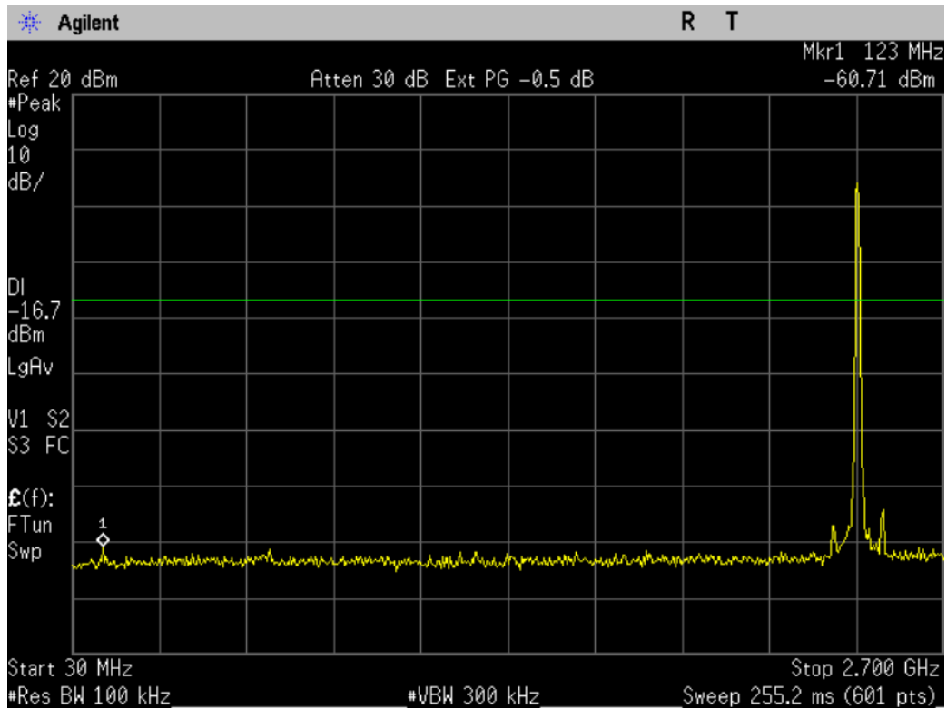
Figure 10-1b1: Conducted Spurious Emissions, 802.11b, Ch 6
