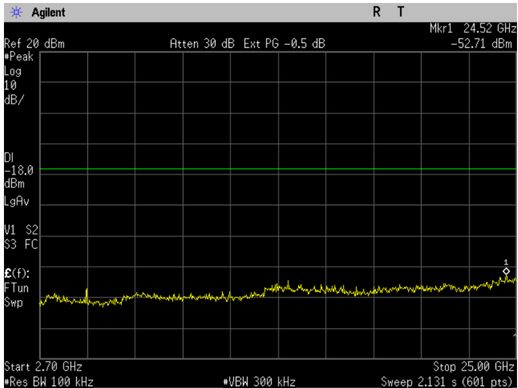
Figure 10-2b2: Conducted Spurious Emissions, 802.11g, Ch 6
