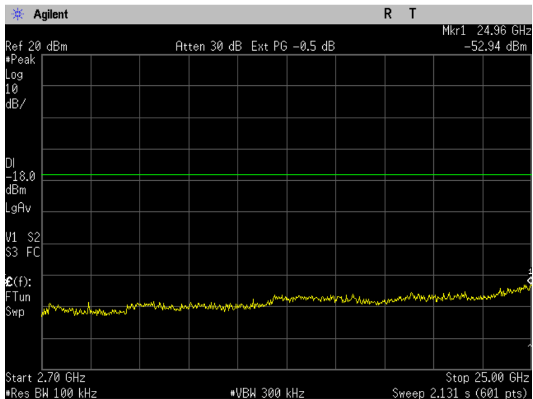
Figure 10-3a2: Conducted Spurious Emissions, 802.11n, Ch 1
