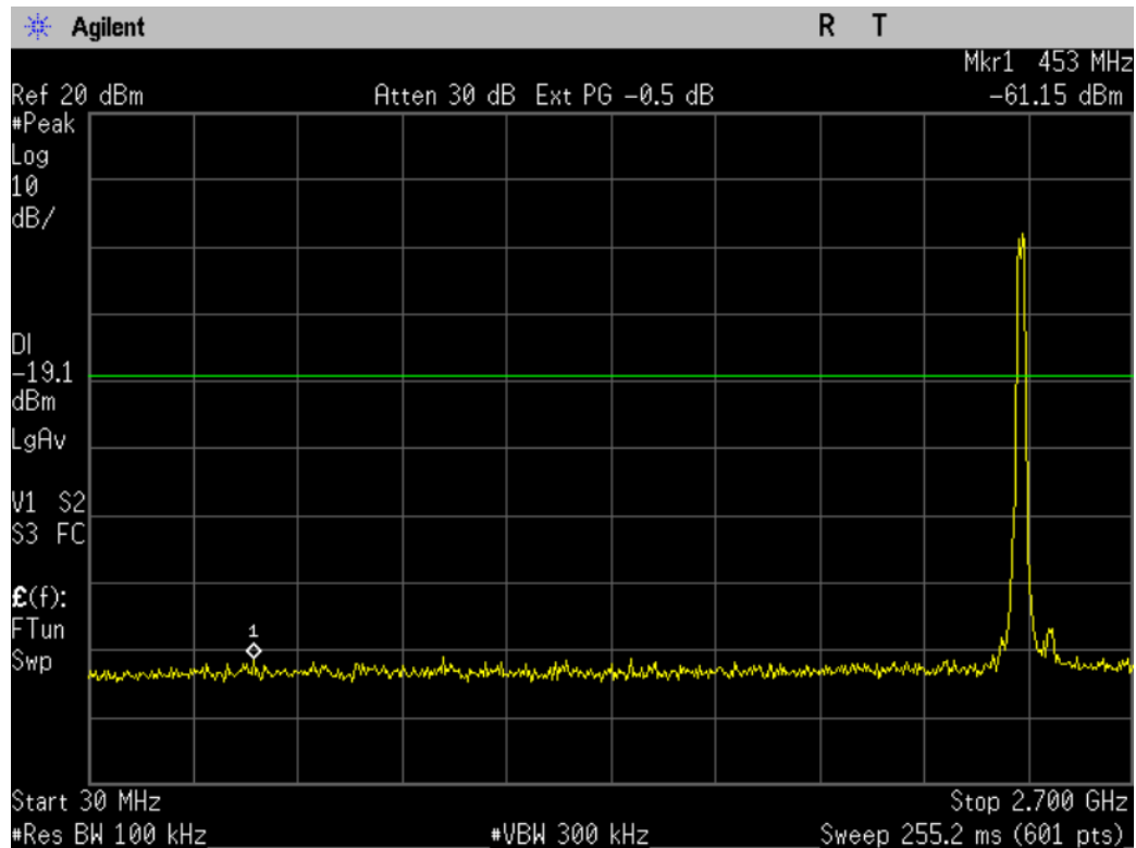
Figure 10-3a1: Conducted Spurious Emissions, 802.11n, Ch 1
