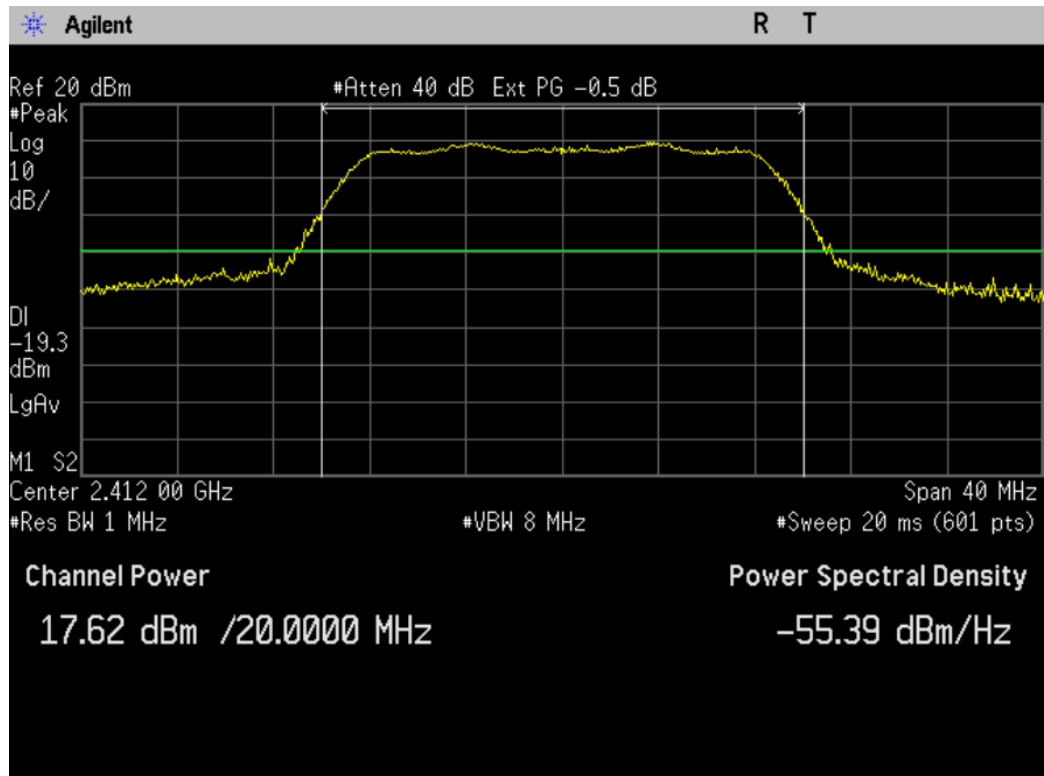
Figure 7-7: Output Power 802.11n, MSC0, Ch 1
