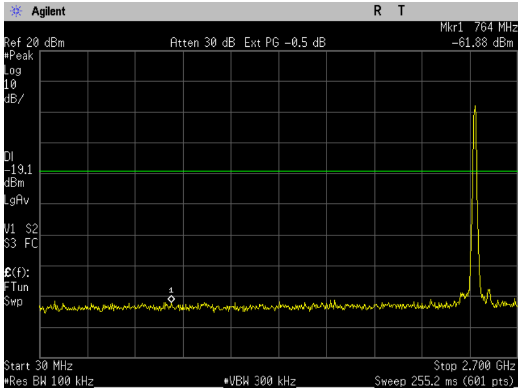
Figure 10-2c1: Conducted Spurious Emissions, 802.11g, Ch 11
