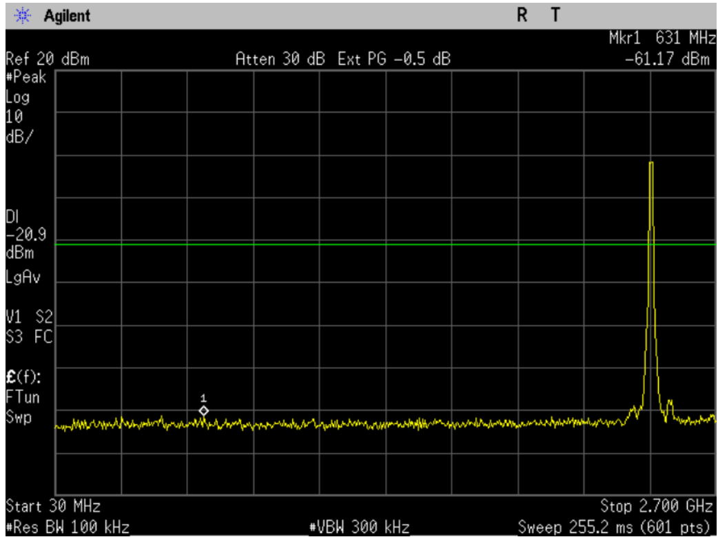
Figure 10-2b1: Conducted Spurious Emissions, 802.11g, Ch 6
