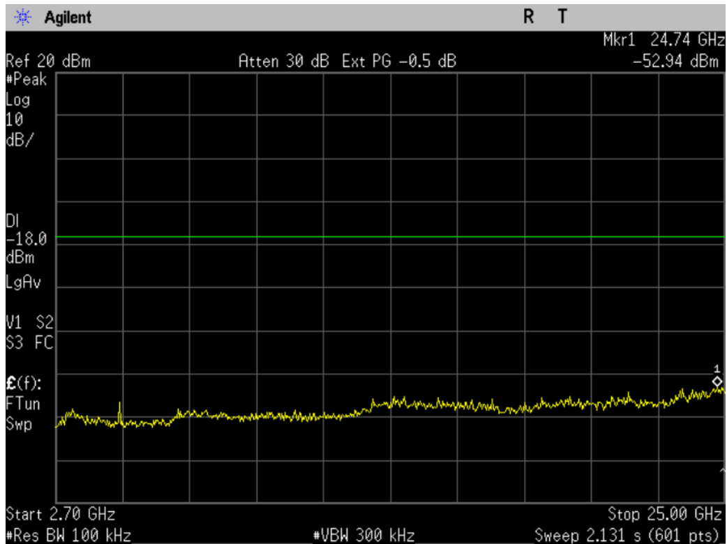
Figure 10-2a2: Conducted Spurious Emissions, 802.11g, Ch 1
