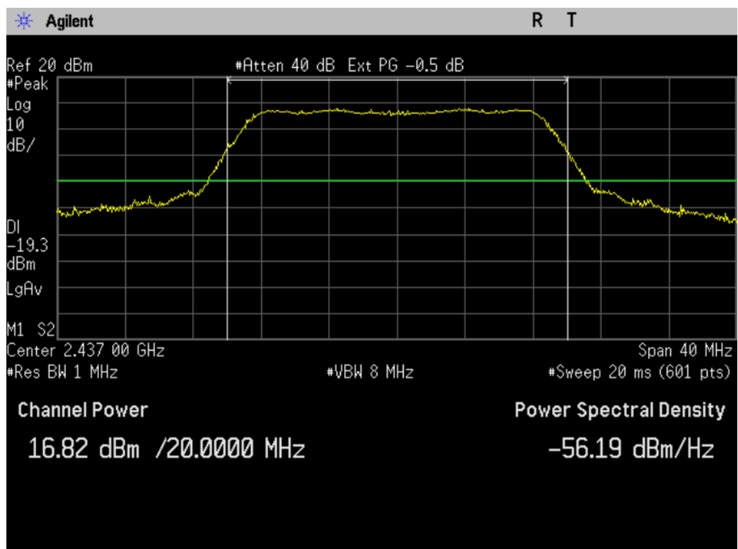
Figure 7-8: Output Power 802.11n, MSC0, Ch 6
