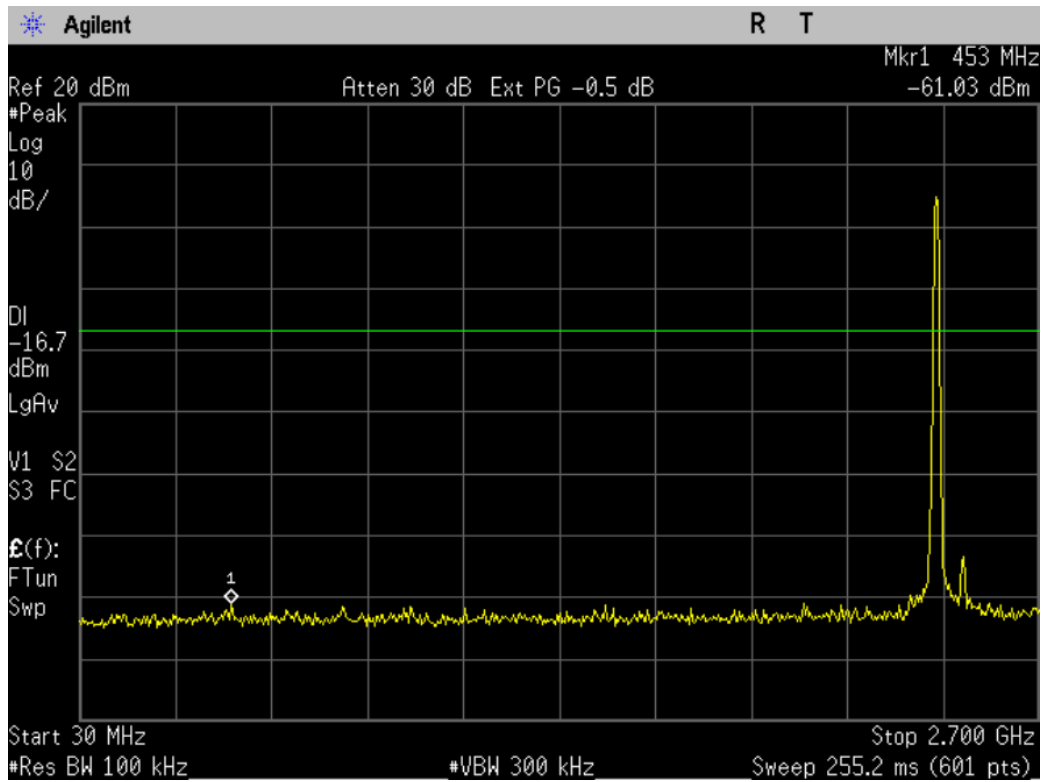
Figure 10-1a1: Conducted Spurious Emissions, 802.11b, Ch 1
