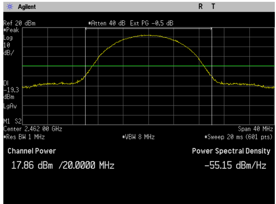
Figure 7-3: Output Power 802.11b, 11Mbps, Ch 11
