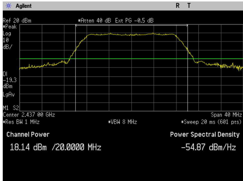
Figure 7-5: Output Power 802.11g, 6Mbps, Ch 6
