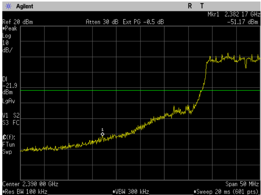
Figure 9-2a: Low band edge, 802.11g, ch1.
