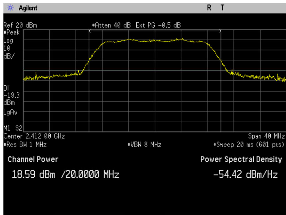
Figure 7-4: Output Power 802.11g, 6Mbps, Ch 1
