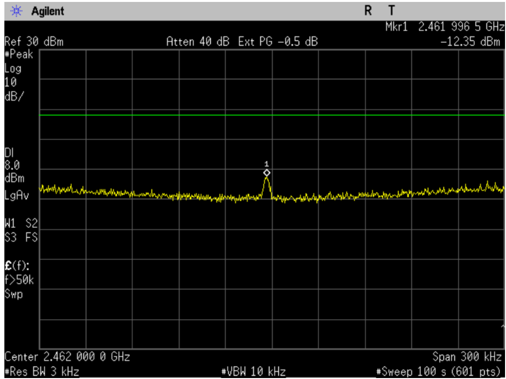
Figure 8-1c: Power Spectral Density, 802.11b, Ch 11.
