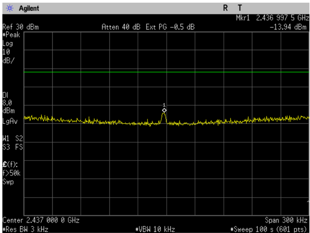
Figure 8-1b: Power Spectral Density, 802.11b, Ch 6.
