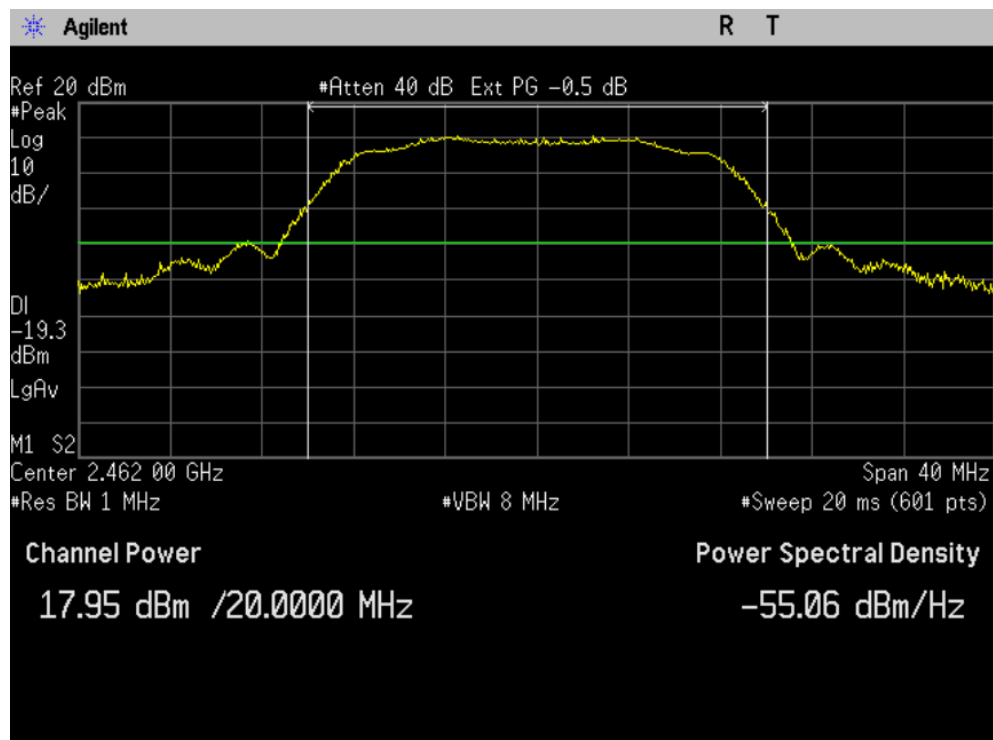
Figure 7-6: Output Power 802.11g, 6 Mbps, Ch 11
