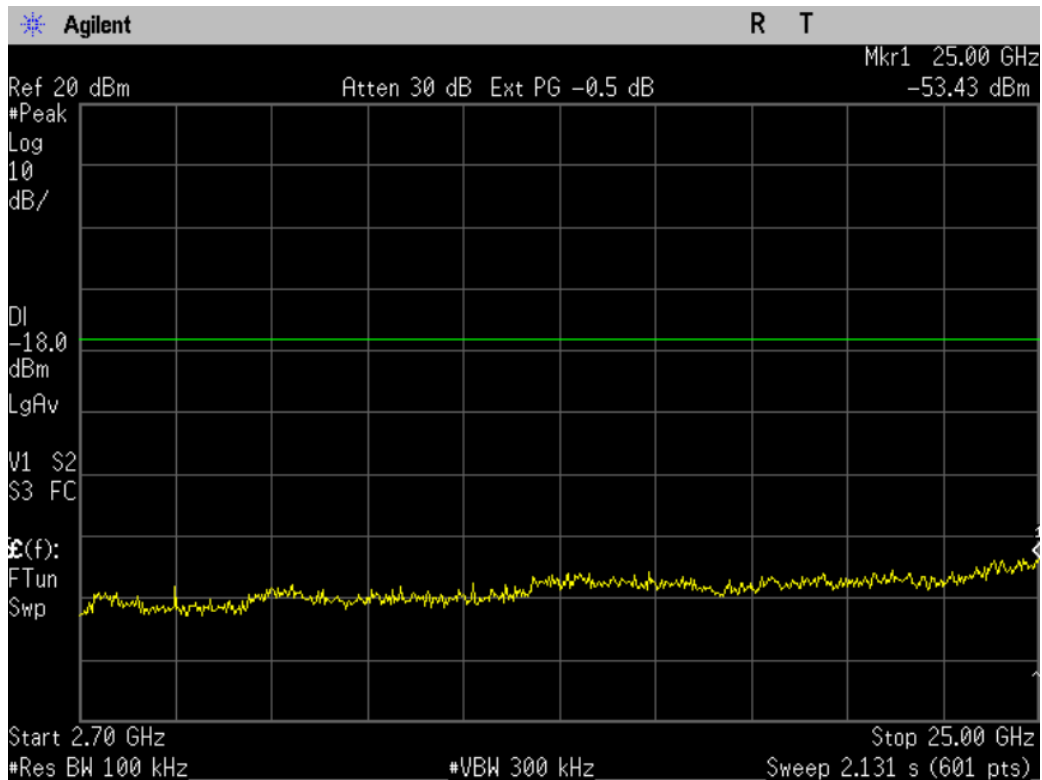
Figure 10-3c2: Conducted Spurious Emissions, 802.11n, Ch 11
