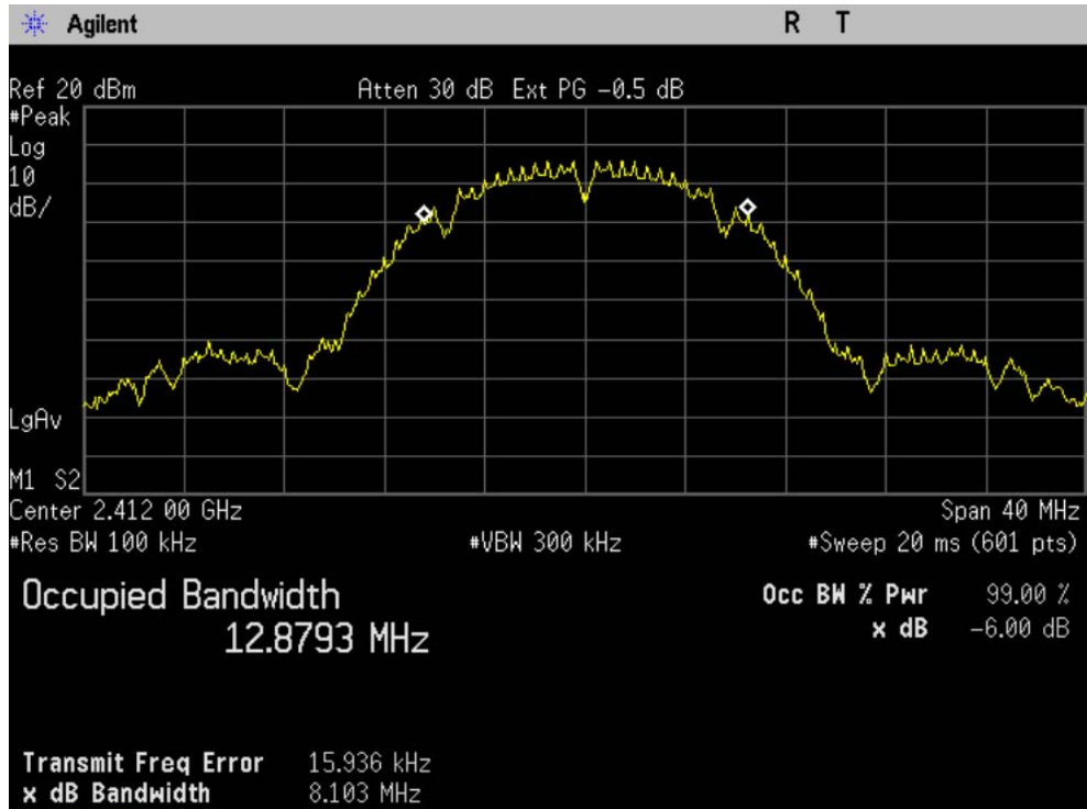
Figure 6-1a: 6 dB Bandwidth, 802.11b 1Mbps, Ch 1.
