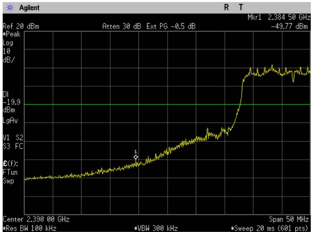
Figure 9-3a: Low band edge, 802.11n, ch1.
