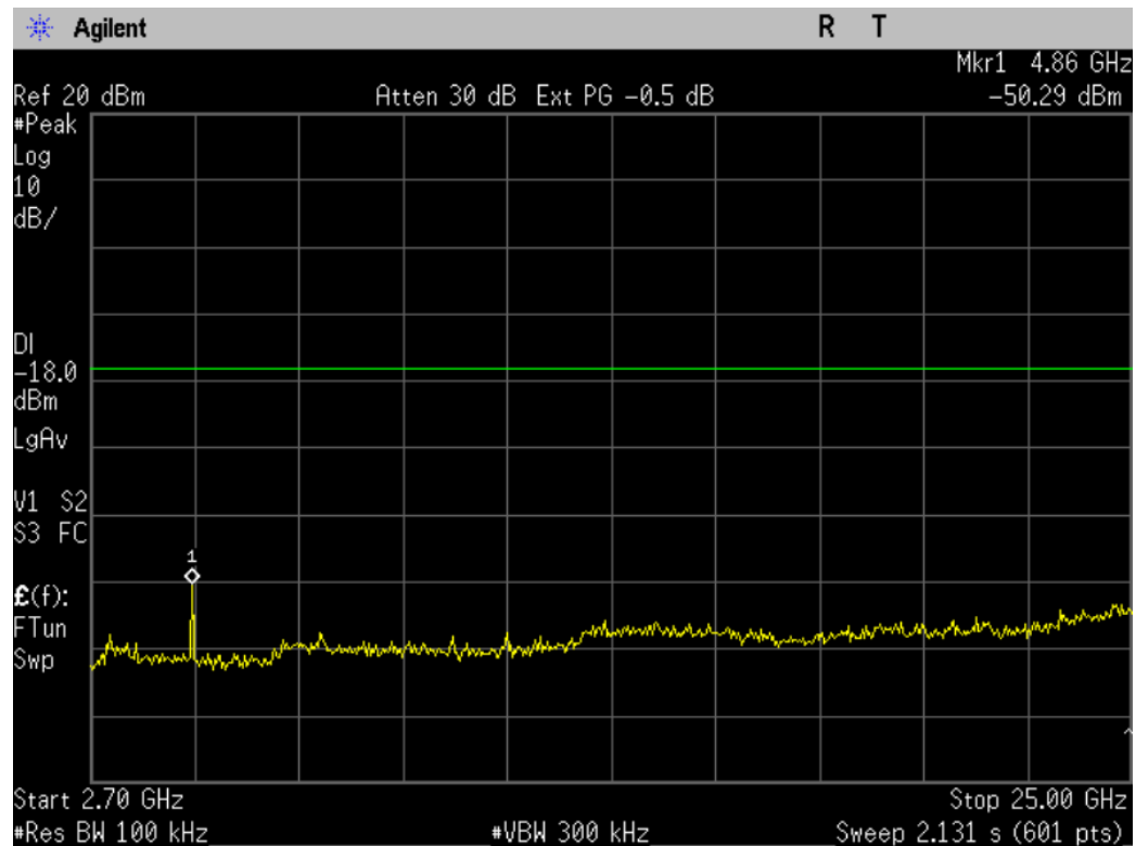
Figure 10-1b2: Conducted Spurious Emissions, 802.11b, Ch 6
