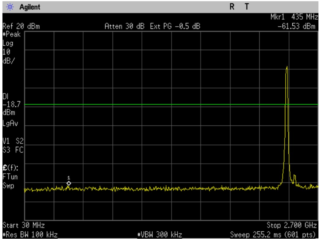
Figure 10-2a1: Conducted Spurious Emissions, 802.11g, Ch 1
