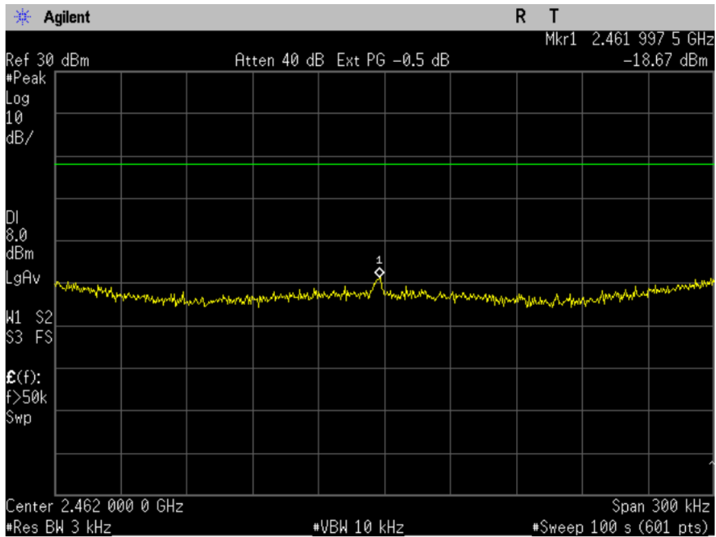
Figure 8-2c: Power Spectral Density, 802.11g, Ch 11.
