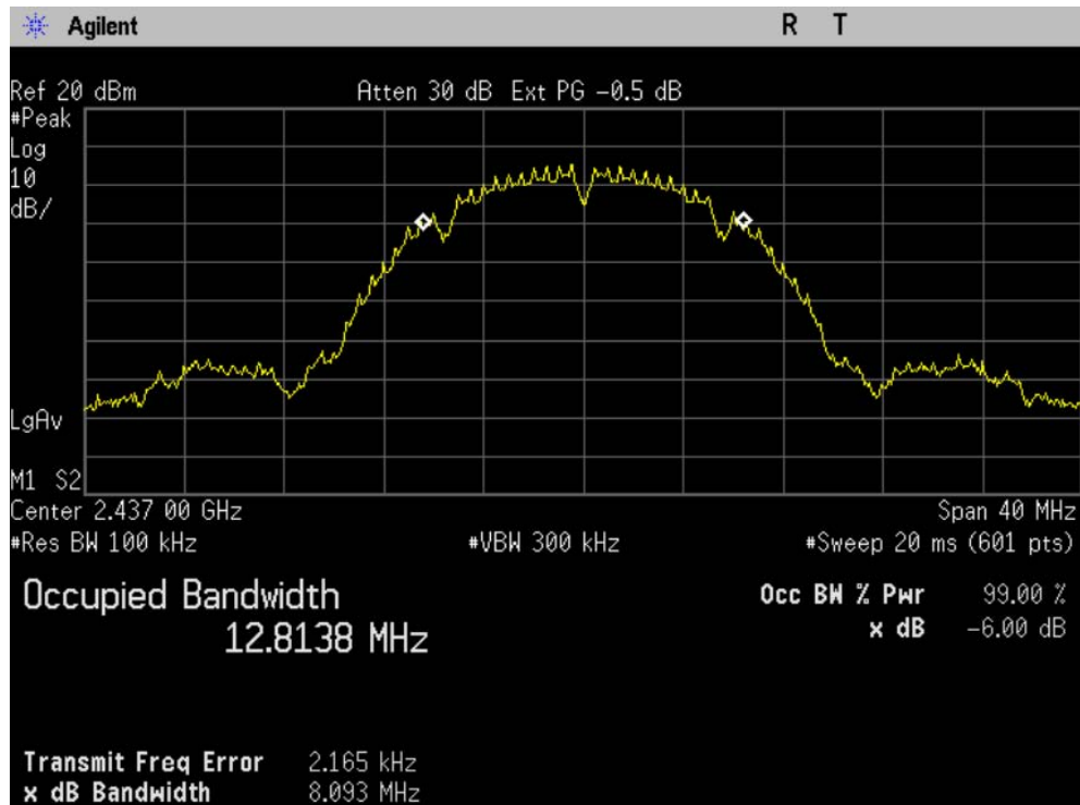
Figure 6-1b: 6 dB Bandwidth, 802.11b 1Mbps, Ch 6.
