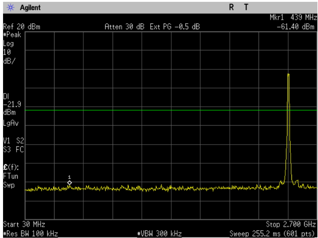
Figure 10-3b1: Conducted Spurious Emissions, 802.11n, Ch 6
