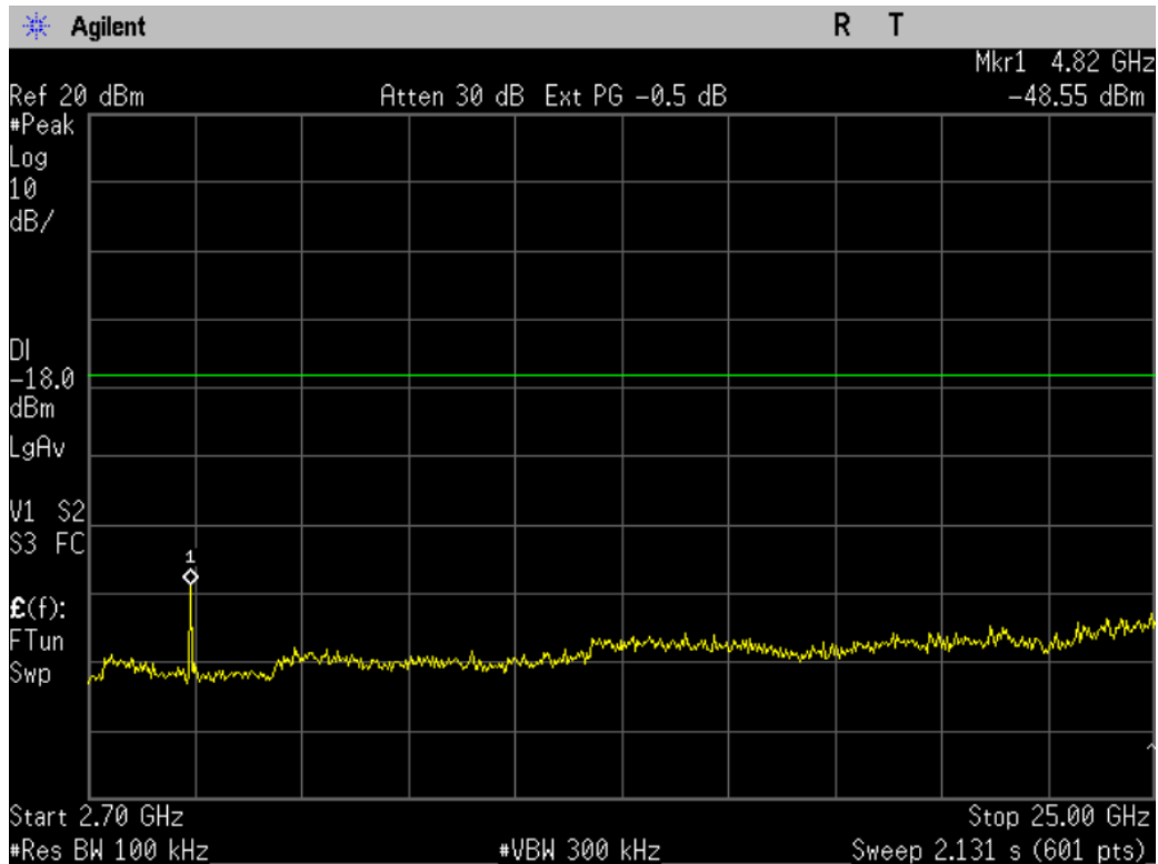
Figure 10-1a2: Conducted Spurious Emissions, 802.11b, Ch 1
