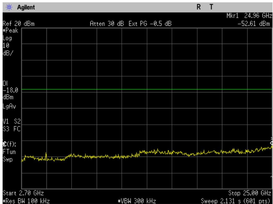
Figure 10-3b2: Conducted Spurious Emissions, 802.11n, Ch 6
