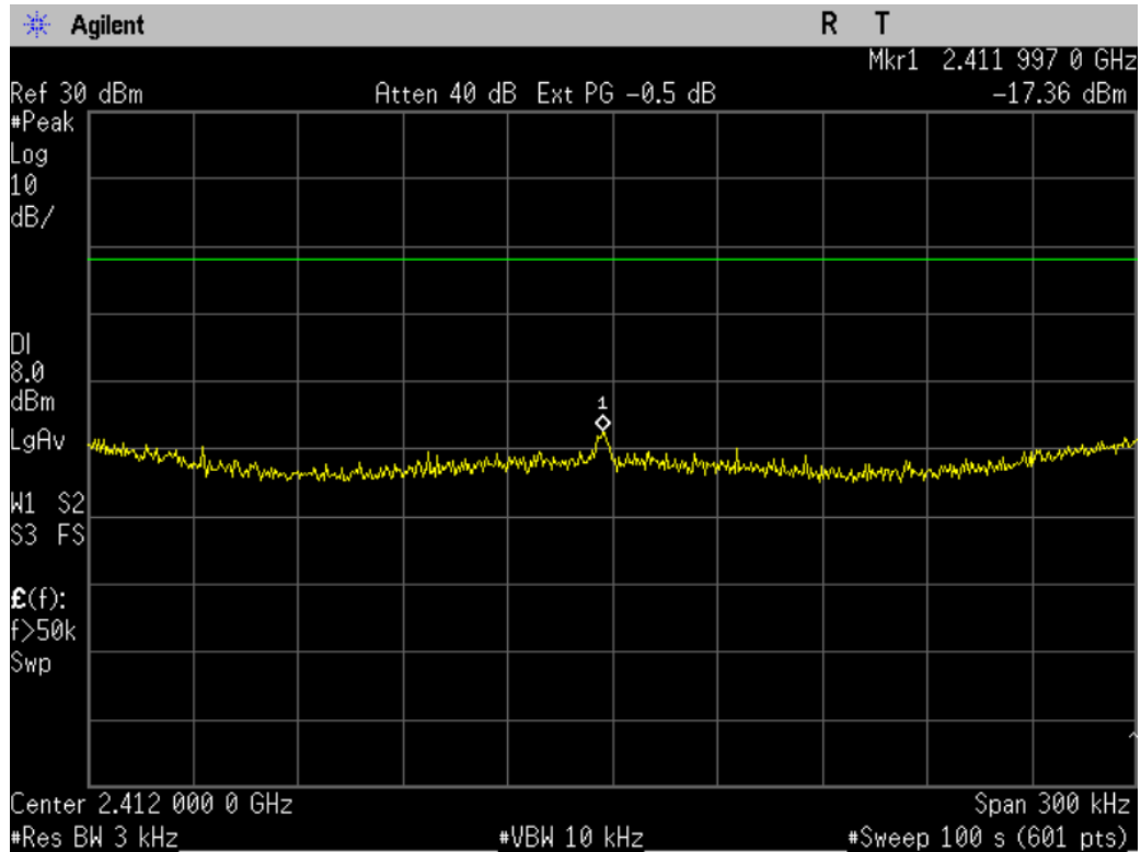
Figure 8-2a: Power Spectral Density, 802.11g, Ch 1.
