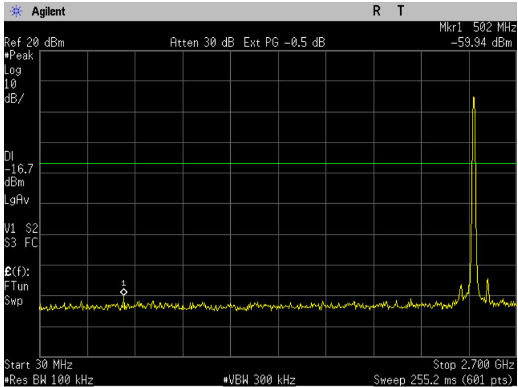
Figure 10-1c1: Conducted Spurious Emissions, 802.11b, Ch 11
