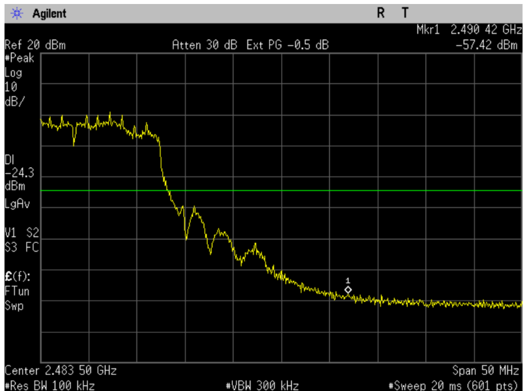
Figure 9-3b: High band edge, 802.11n, ch11.
