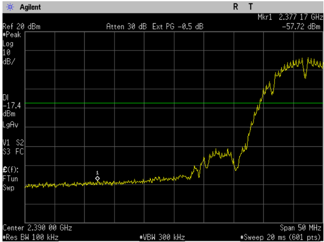
Figure 9-1a: Low band edge, 802.11b, ch1
