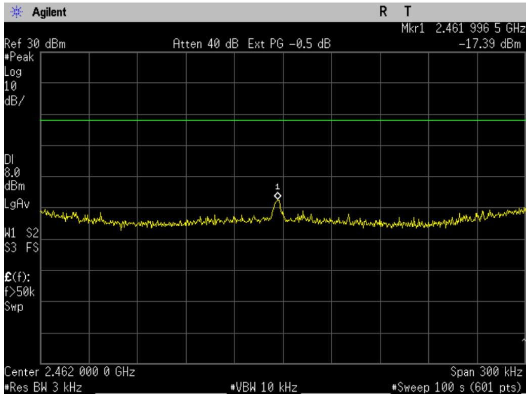
Figure 8-3c: Power Spectral Density, 802.11n, Ch 11.
