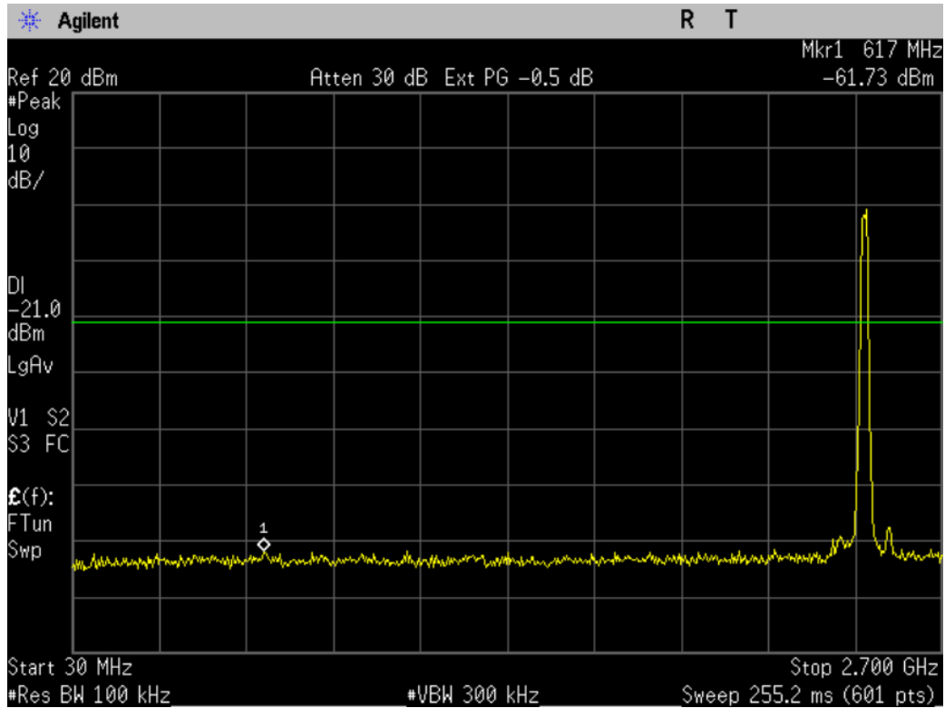
Figure 10-3c1: Conducted Spurious Emissions, 802.11n, Ch 11
