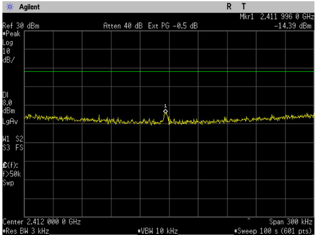
Figure 8-1a: Power Spectral Density, 802.11b, Ch 1.
