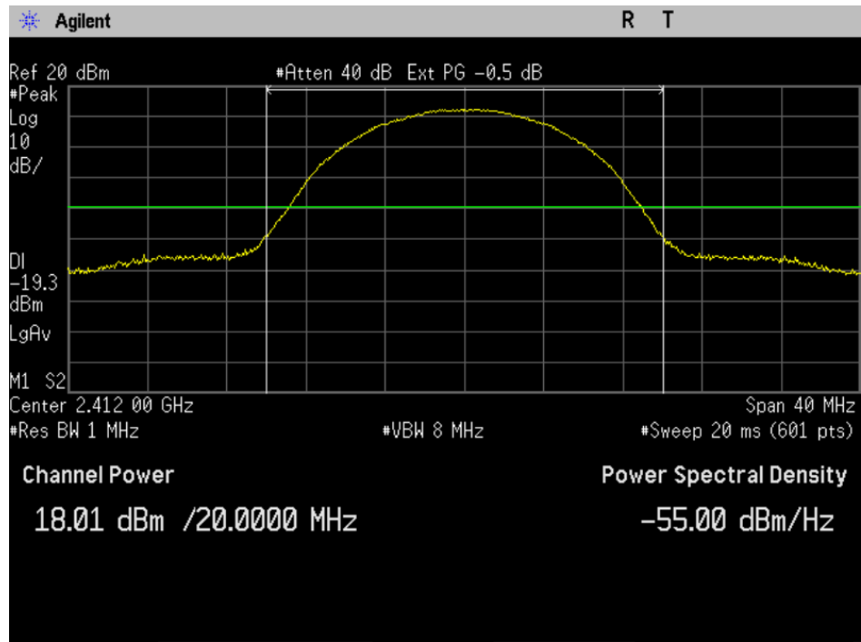
Figure 7-1: Output Power 802.11b, 11Mbps, Ch 1
