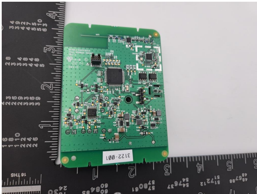
Multi-Function with Relay PCB Primary (EAPRO-WMFT-R)
