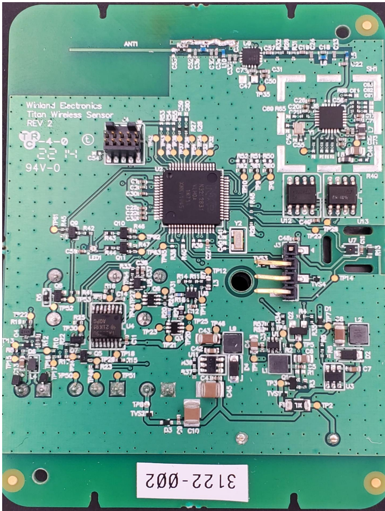
Multi-Function with Relay PCB Primary (EAPRO-WMFT-R)
