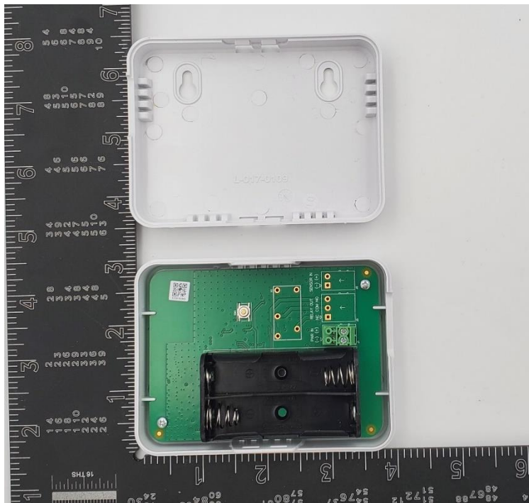
Humidity Sensor PCB Primary (EAPRO-WHS)
