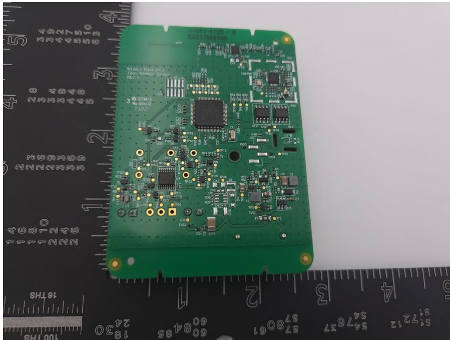
Multi-Function PCB Primary (EAPRO-WMFT)
