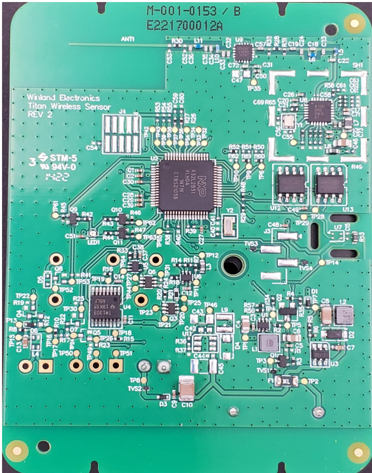
Temp Sensor PCB Primary (EAPRO-WTS)
