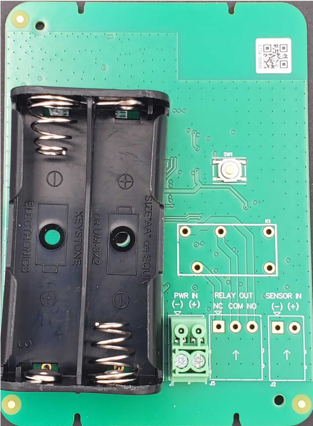
Temp Sensor PCB Secondary (EAPRO-WTS)
