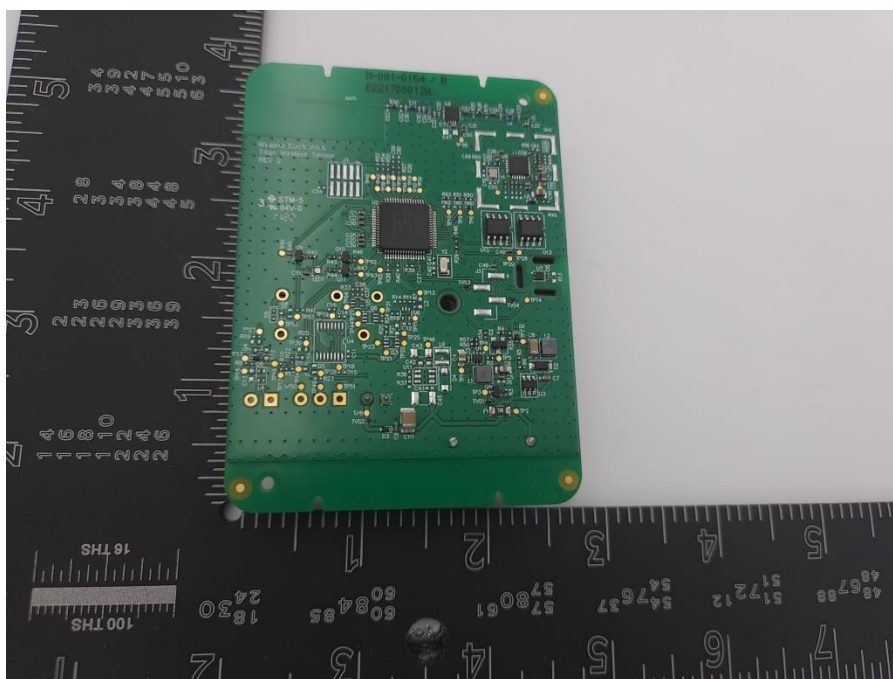
Humidity Sensor PCB Primary (EAPRO-WHS)
