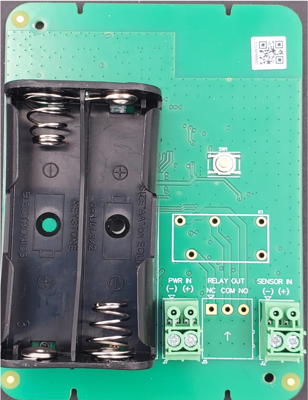
Multi-Function Sensor PCB Secondary (EAPRO-WMFT)
