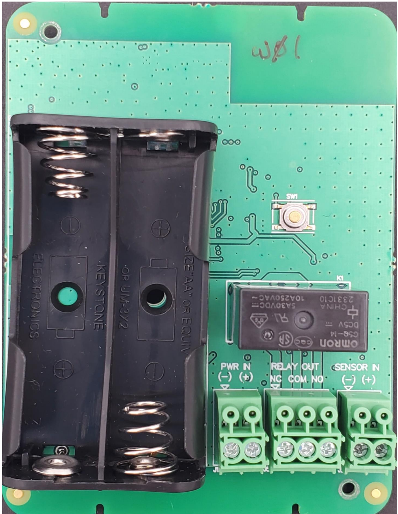
Multi-Function with Relay PCB Secondary (EAPRO-WMFT-R)
