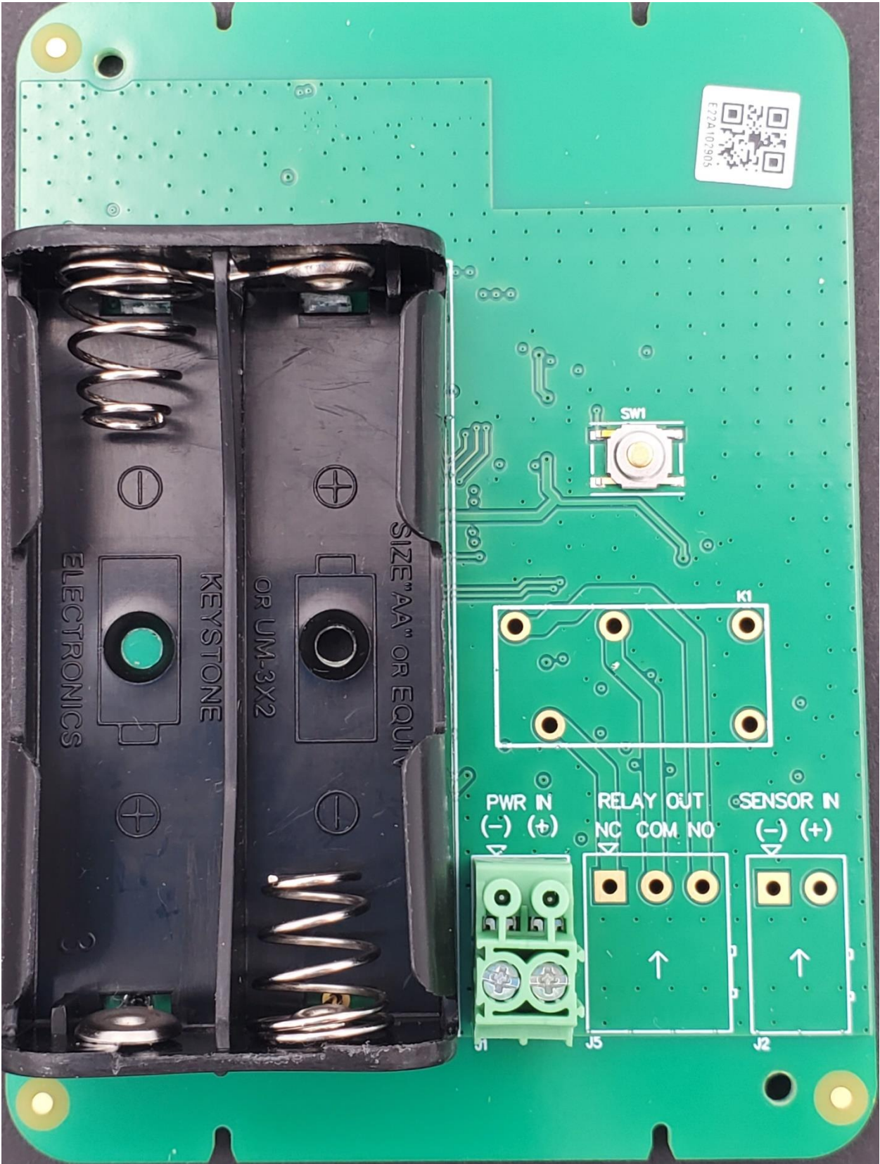
Humidity Sensor PCB Secondary (EAPRO-WHS)
