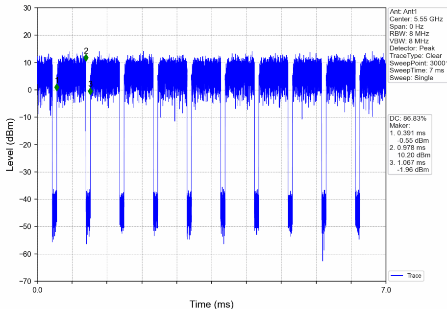
802.11n(HT40)_MCH_5550MHz_Ant1_NTNV
