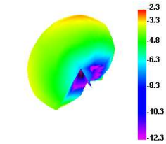
Low frequency antenna pattern
