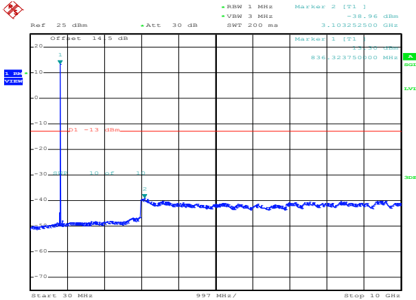
QPSK Middle channel-30MHz~10GHz
