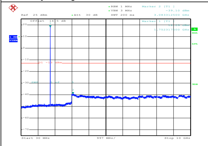
QPSK High channel-30MHz~10GHz
