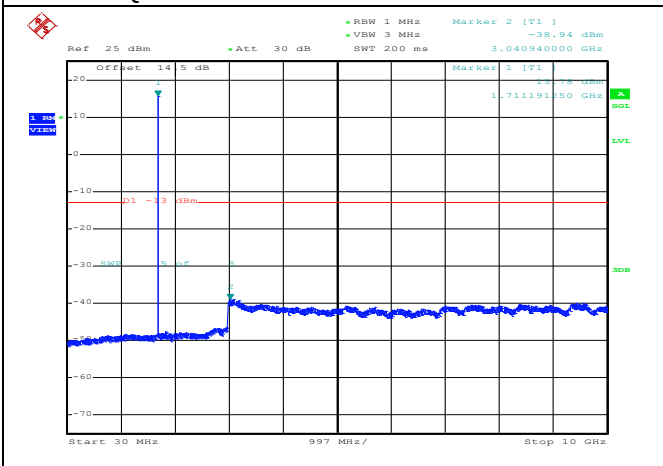
QPSK Middle channel-30MHz~10GHz
