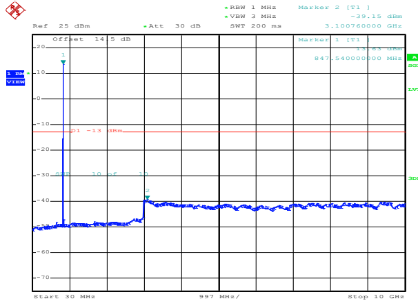
QPSK High channel-30MHz~10GHz
