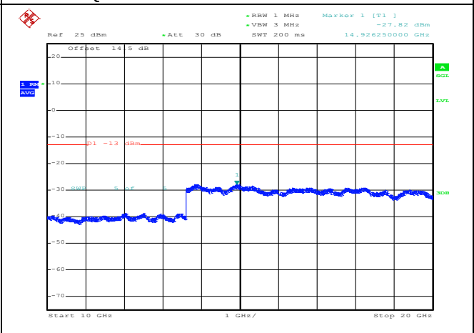
QPSK Middle channel-10GHz~20GHz
