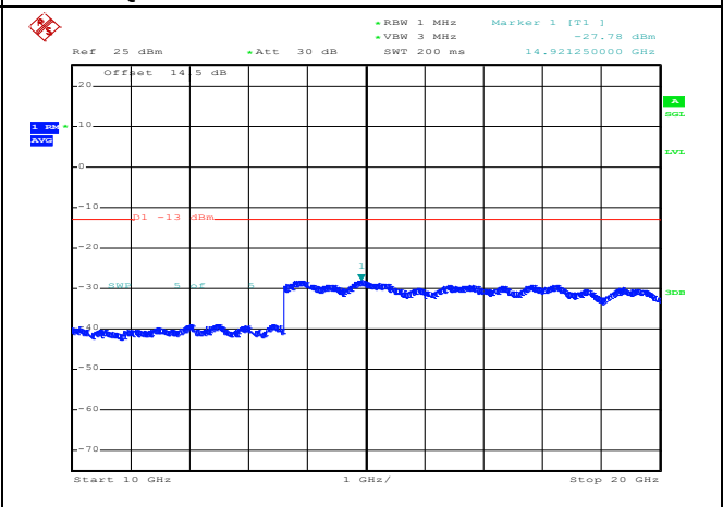
QPSK High channel-10GHz~20GHz
