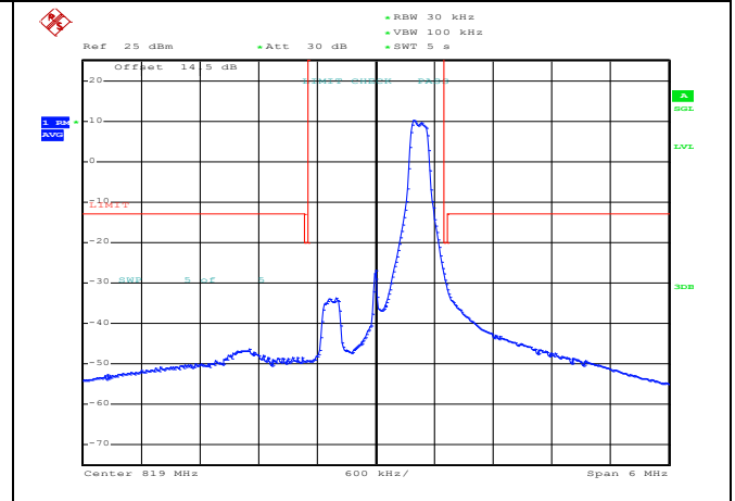
16QAM Mid channel-6 RB offset 0
