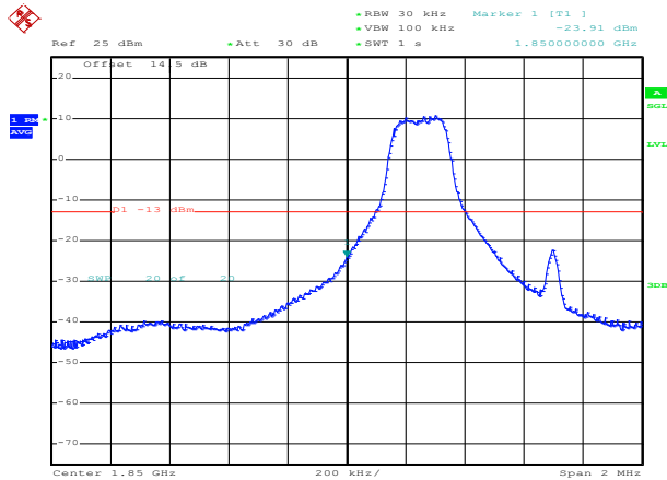
QPSK Low channel-6 RB offset 0
