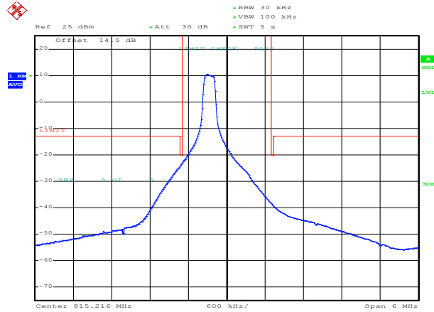
QPSK Mid channel-1 RB offset max
