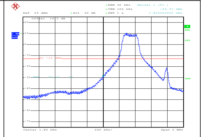
16QAM Low channel-6 RB offset 0
