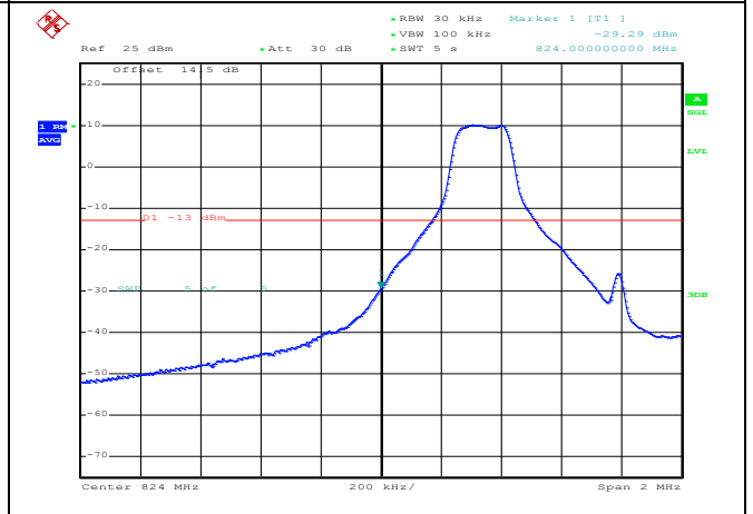
16QAM Low channel-6 RB offset 0
