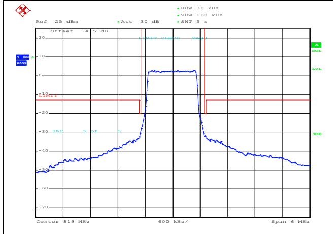
QPSK Mid channel-6 RB offset 0
