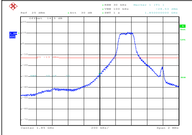
QPSK Low channel-6 RB offset 0
