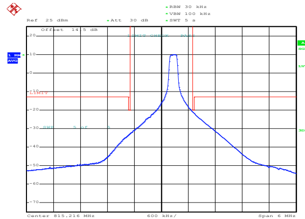
16QAM Mid channel-6 RB offset 0
