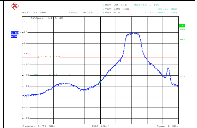
16QAM Low channel-6 RB offset 0
