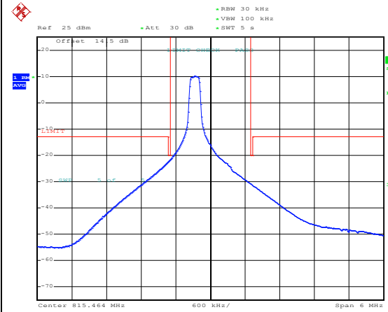
16QAM Middle channel-1 RB offset 0
