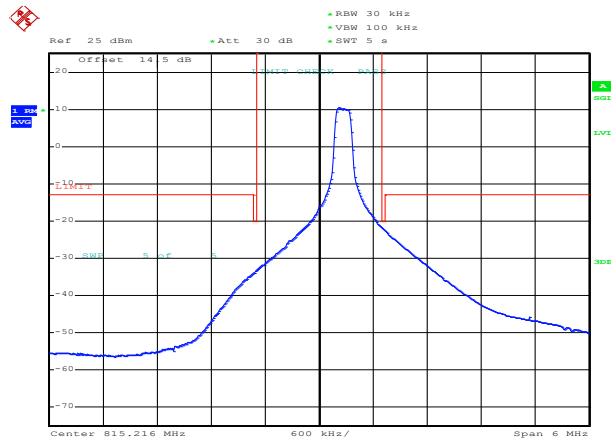
QPSK Mid channel-6 RB offset 0
