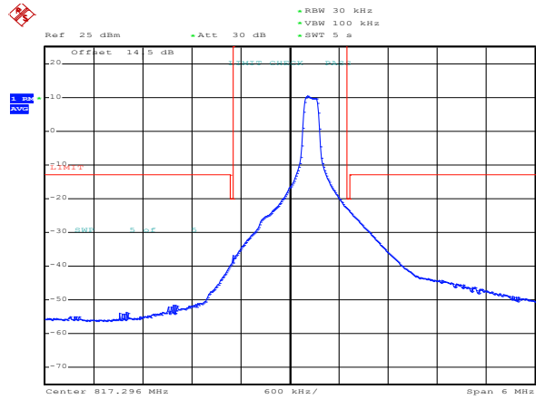
QPSK Mid channel-6 RB offset 0
