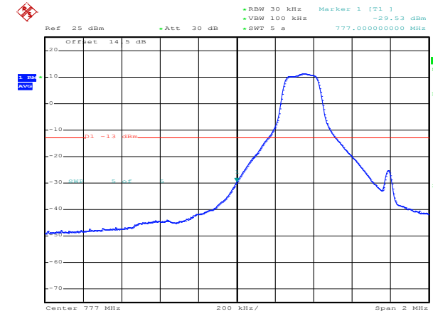
16QAM Low channel-6 RB offset 0
