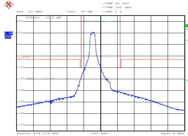
16QAM Mid channel-1 RB offset max
