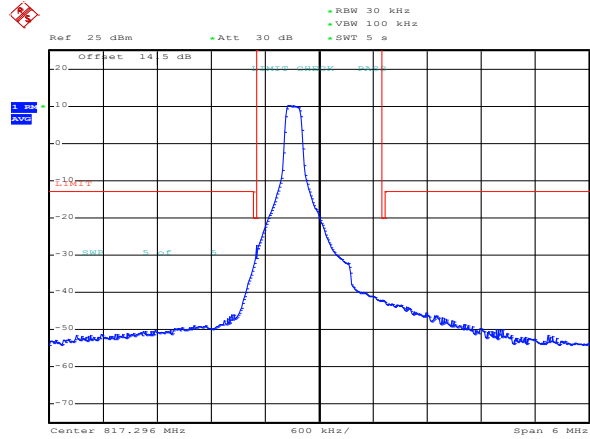
QPSK Mid channel-1 RB offset max
