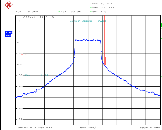
16QAM Middle channel-1 RB offset max
