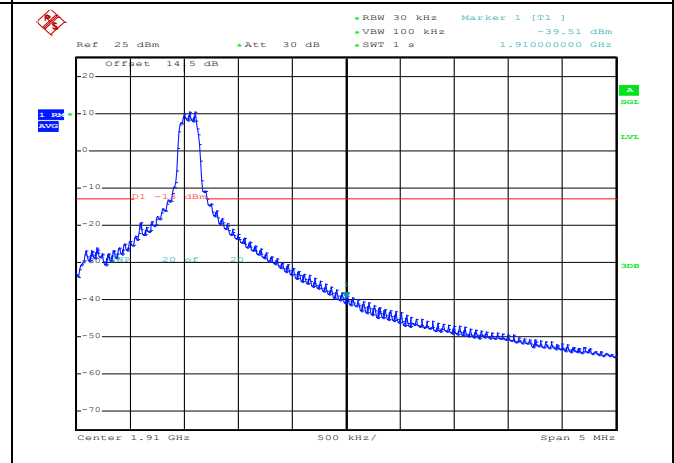
16QAM High channel-6 RB offset 0
