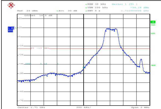
QPSK Low channel-6 RB offset 0
