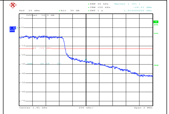
16QAM High channel-6 RB offset 0
