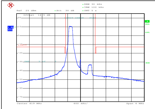
QPSK Mid channel-1 RB offset max
