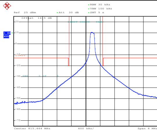
QPSK Middle channel-1 RB offset max
