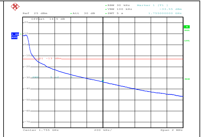
16QAM High channel-6 RB offset 0
