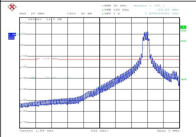
16QAM Low channel-6 RB offset 0
