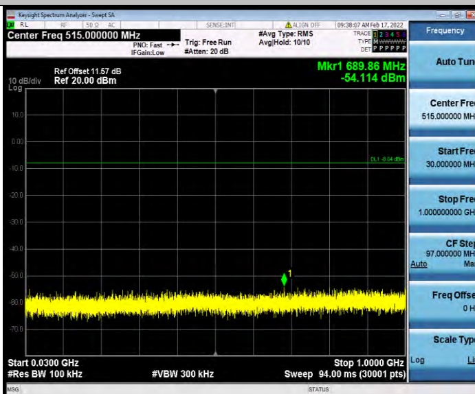
DH5_Ant1_2402_30~1000
