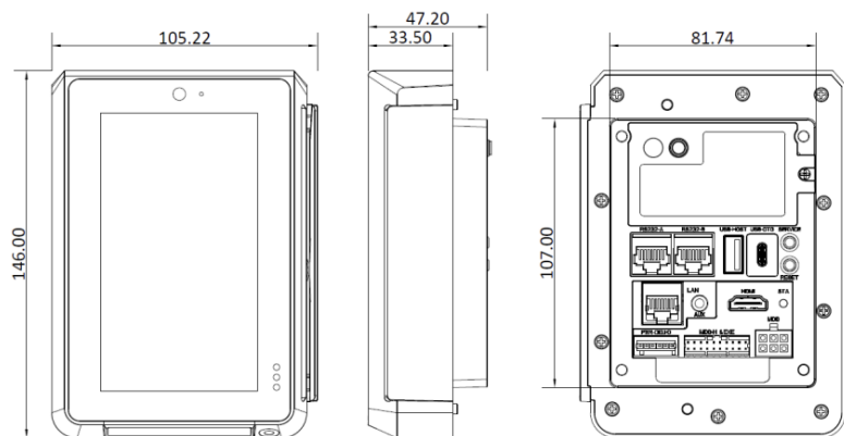
Figure 8: device dimensions (mm)
