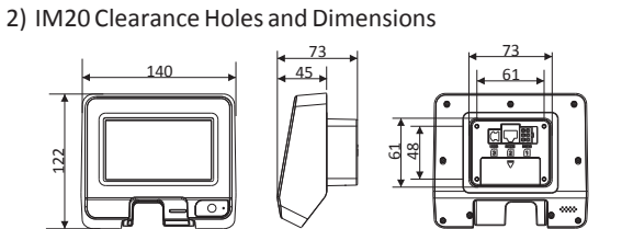
Figure 5: device dimensions (mm)
