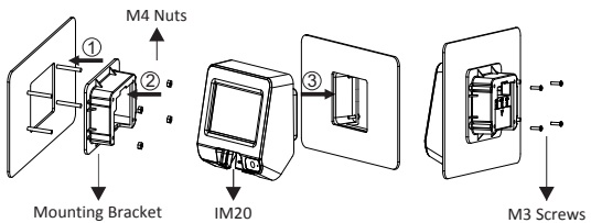
Figure 6: installation and mounting
