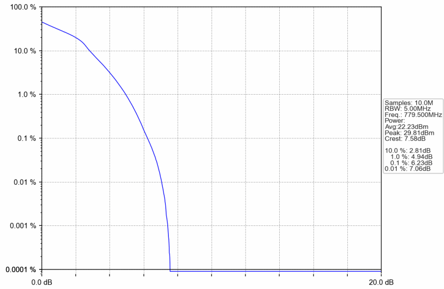
Band13_5MHz_16QAM_LCH_779.5MHz_RB_25_0_NTNV
