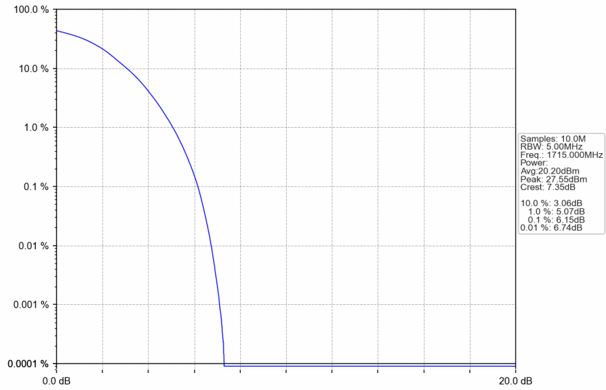
Band4 10MHz 16QAM LCH 1715MHz RB 50 0 NTNV
