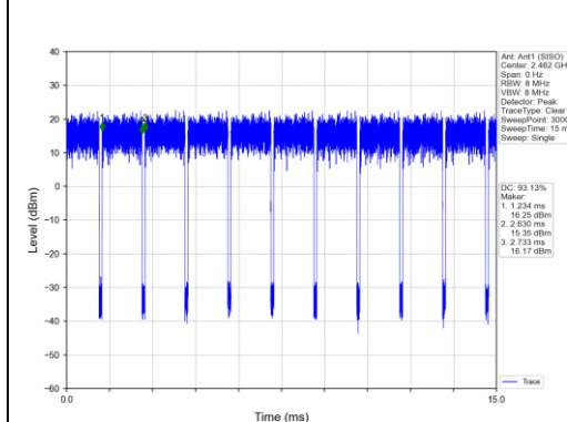
802.11g
