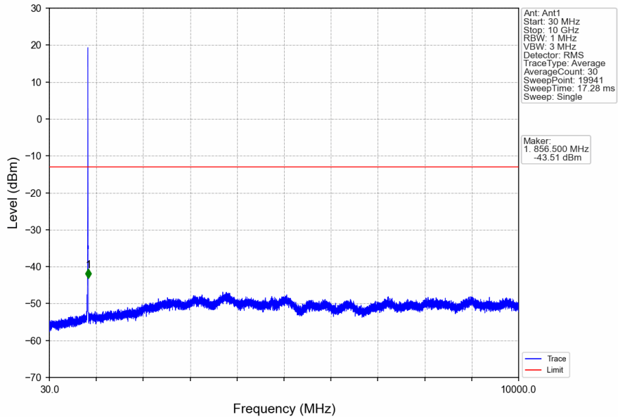
Band5_HSDPA_LCH_826.4MHz_Subtest 1_NTNV
