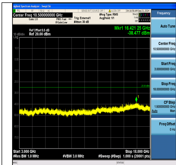
Band41_10MHz_16QAM_40690_50RB#0_3000~18000_3000~18000
