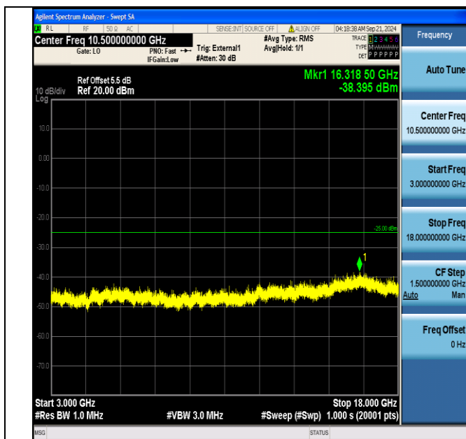
Band41_10MHz_QPSK_41190_1RB#0_3000~18000_3000~18000
