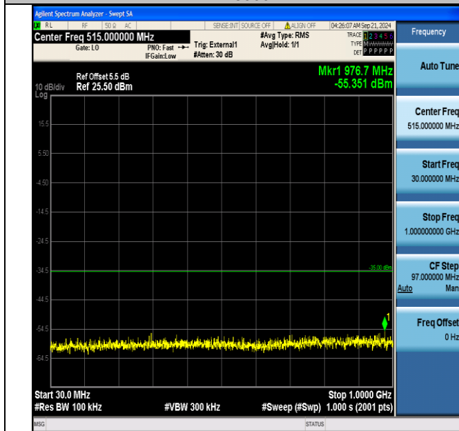
Band41_10MHz_16QAM_41190_50RB#0_30~1000_30~1000
