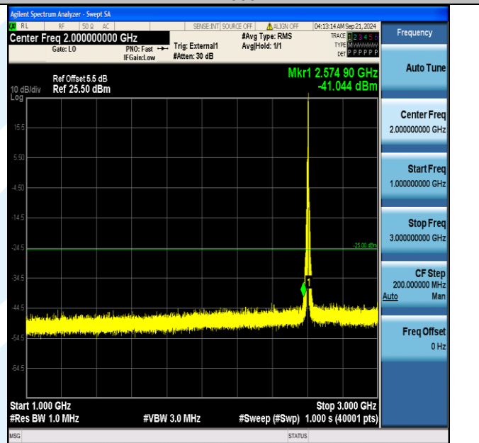
Band41_10MHz_16QAM_40690_1RB#49_1000~3000_1000~3000
