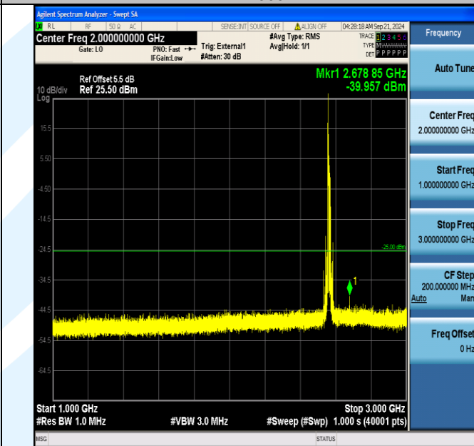
Band41_15MHz_QPSK_40315_1RB#0_1000~3000_1000~3000
