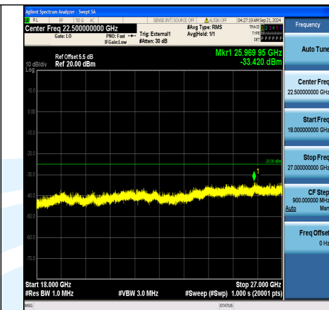
Band41_10MHz_16QAM_41190_50RB#0_18000~27000_18000~27000
