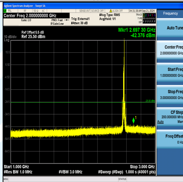
Band41_15MHz_QPSK_40315_1RB#74_1000~3000_1000~3000
