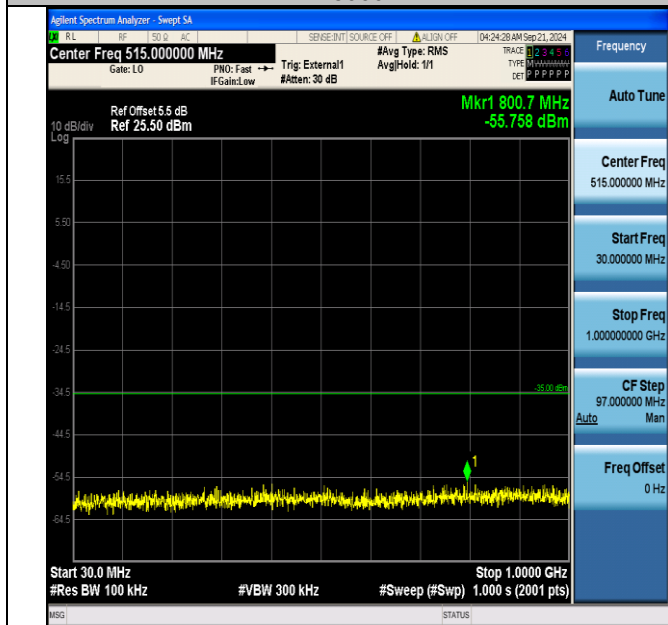
Band41_10MHz_QPSK_41190_50RB#0_30~1000_30~1000
