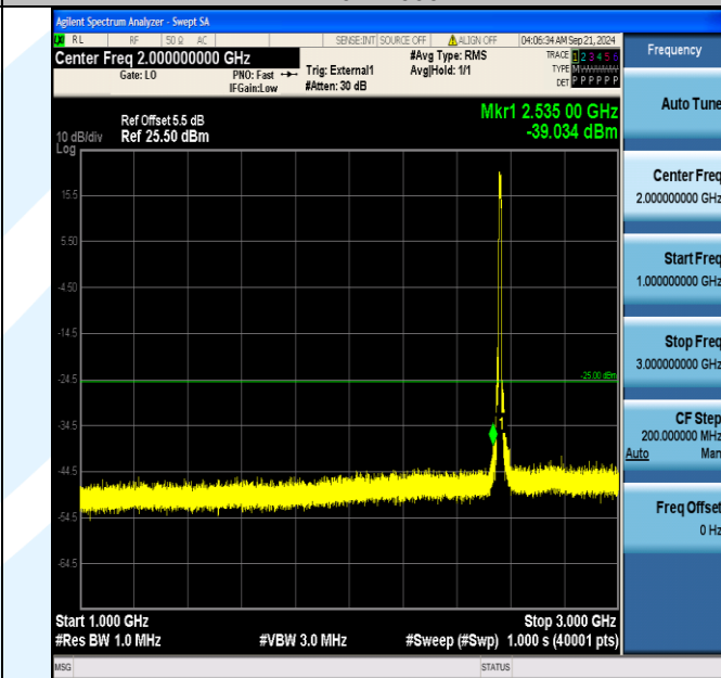
Band41_10MHz_16QAM_40290_50RB#0_1000~3000_1000~3000
