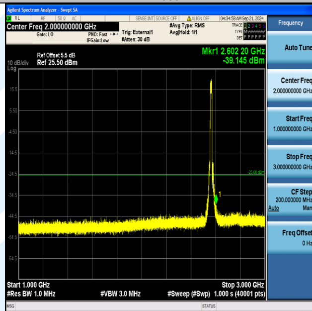
Band41_15MHz_QPSK_40315_75RB#0_1000~3000_1000~3000
