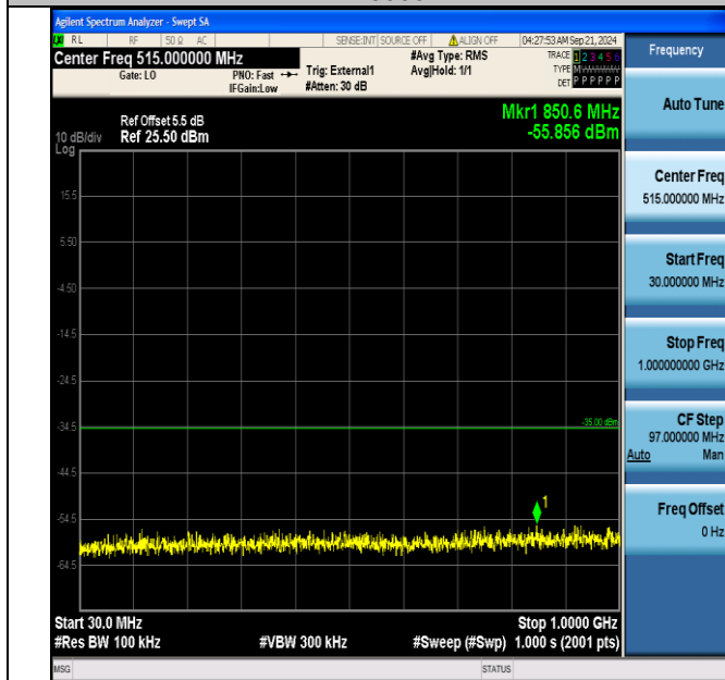
Band41_15MHz_QPSK_40315_1RB#0_30~1000_30~1000
