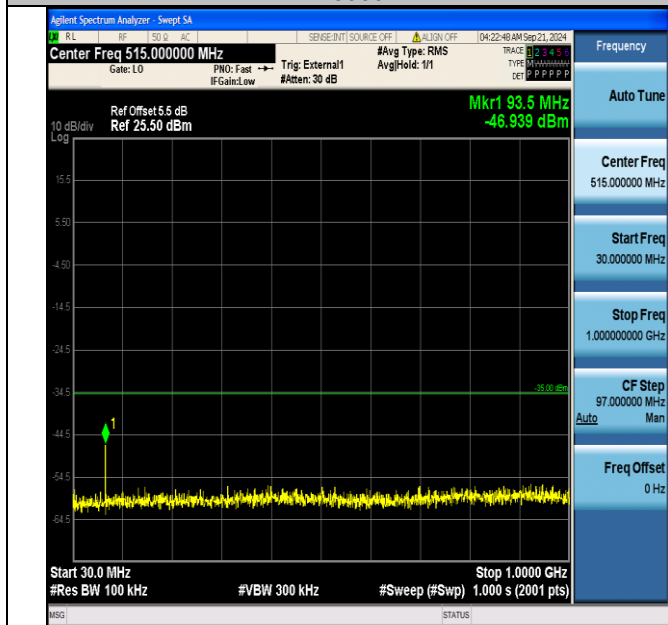
Band41_10MHz_16QAM_41190_1RB#49_30~1000_30~1000
