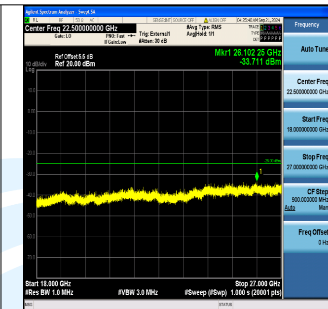
Band41_10MHz_QPSK_41190_50RB#0_18000~27000_18000~27000
