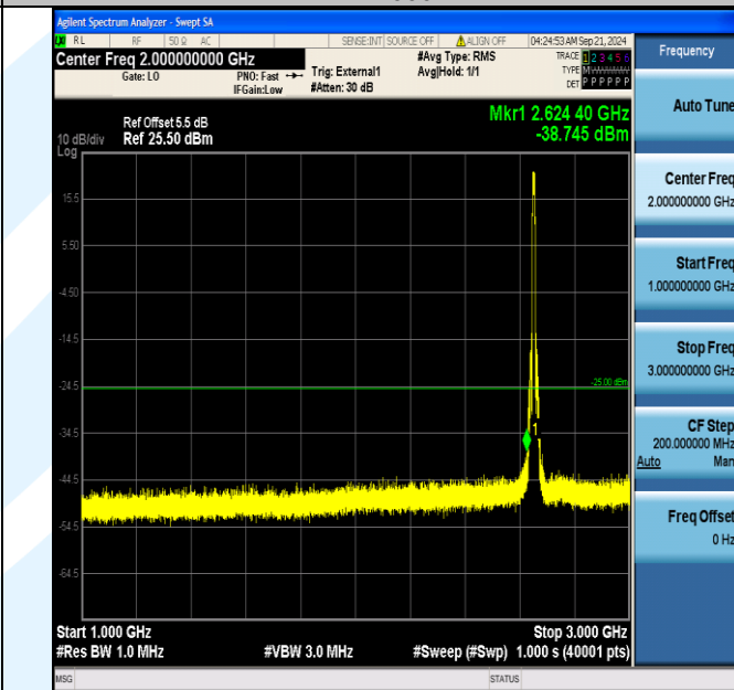
Band41_10MHz_QPSK_41190_50RB#0_1000~3000_1000~3000
