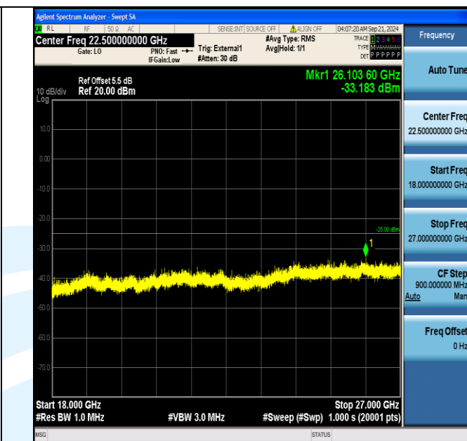
Band41_10MHz_16QAM_40290_50RB#0_18000~27000_18000~27000
