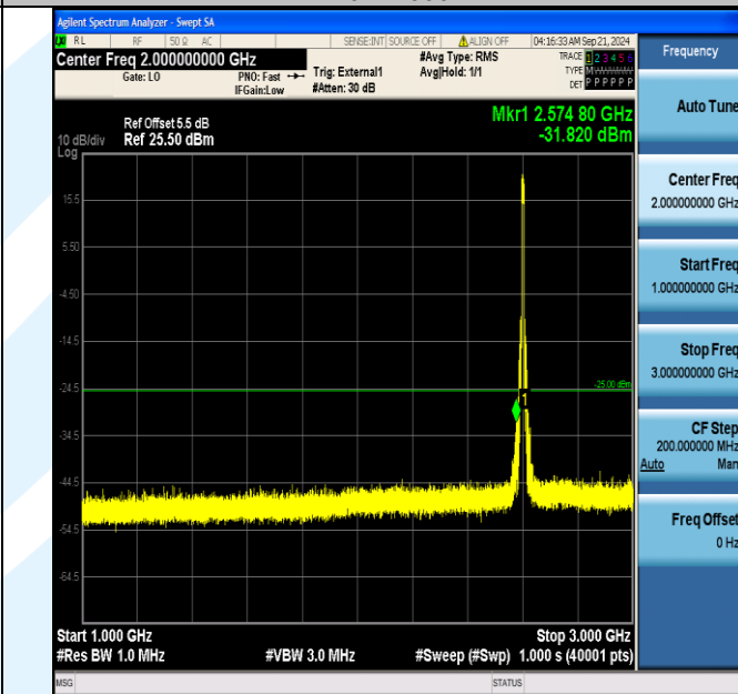
Band41_10MHz_16QAM_40690_50RB#0_1000~3000_1000~3000
