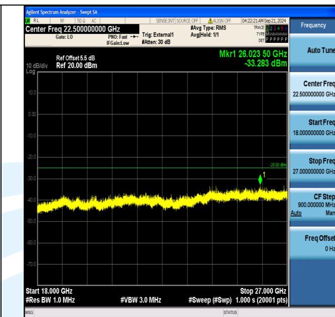
Band41_10MHz_QPSK_41190_1RB#49_18000~27000_18000~27000
