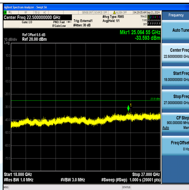
Band41_15MHz_QPSK_40315_1RB#0_18000~27000_18000~27000
