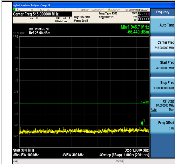
Band41_10MHz_16QAM_40690_50RB#0_30~1000_30~1000
