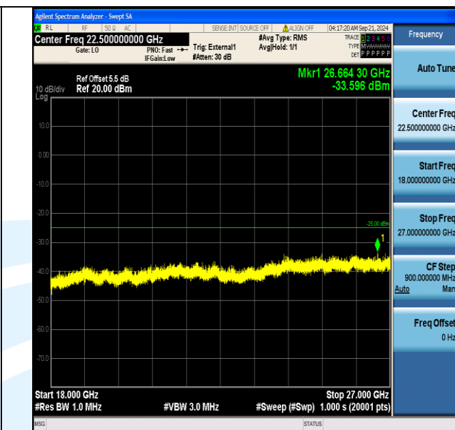
Band41_10MHz_16QAM_40690_50RB#0_18000~27000_18000~27000
