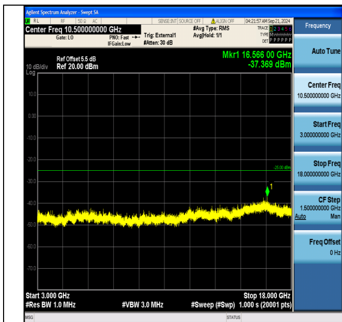
Band41_10MHz_QPSK_41190_1RB#49_3000~18000_3000~18000
