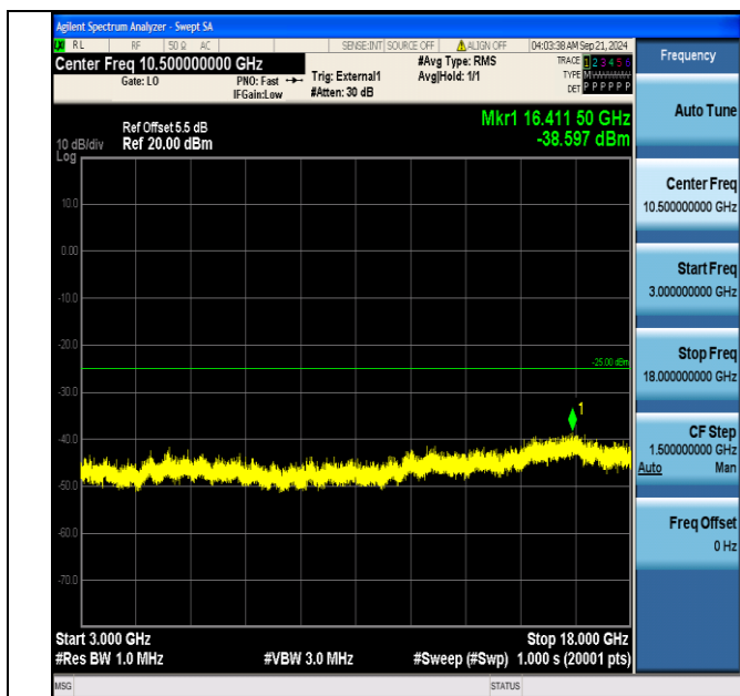
Band41_10MHz_16QAM_40290_1RB#49_3000~18000_3000~18000
