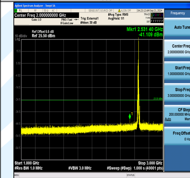
Band41_10MHz_16QAM_41190_1RB#49_1000~3000_1000~3000
