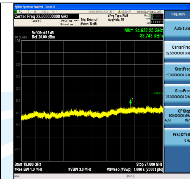
Band41_10MHz_16QAM_40290_1RB#49_18000~27000_18000~27000
