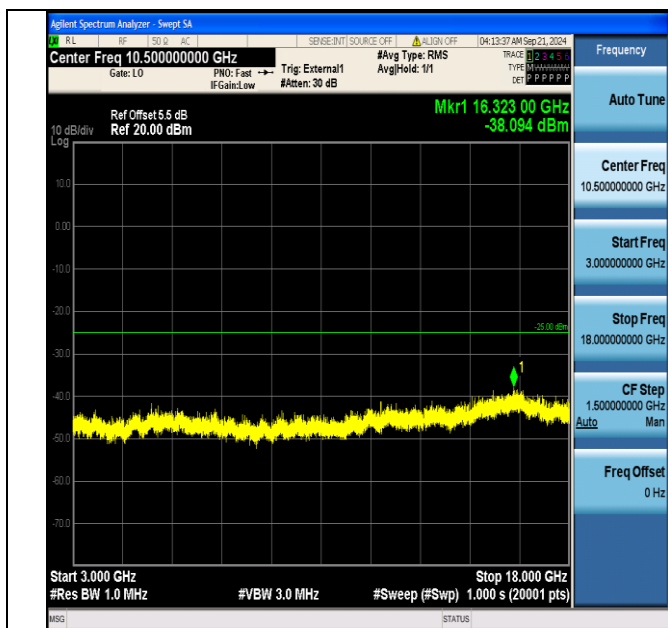
Band41_10MHz_16QAM_40690_1RB#49_3000~18000_3000~18000
