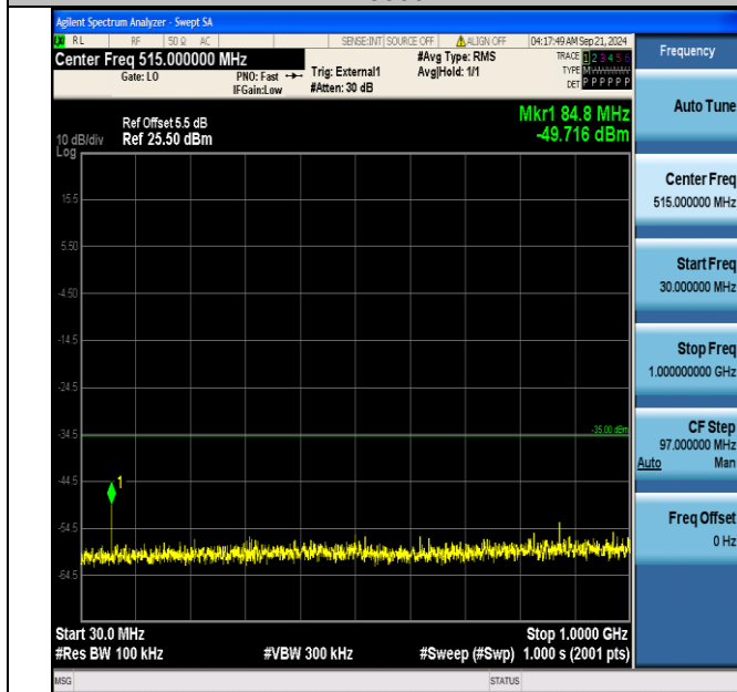
Band41_10MHz_QPSK_41190_1RB#0_30~1000_30~1000
