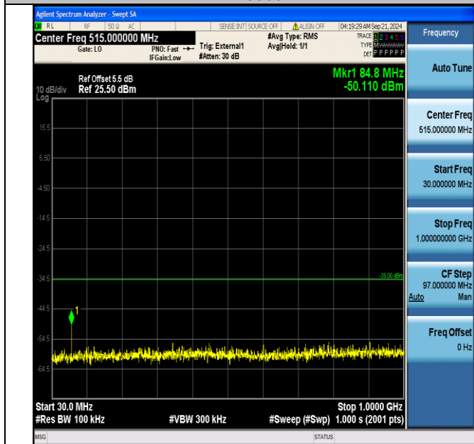
Band41_10MHz_16QAM_41190_1RB#0_30~1000_30~1000
