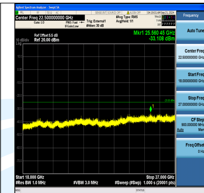
Band41_10MHz_QPSK_41190_1RB#0_18000~27000_18000~27000
