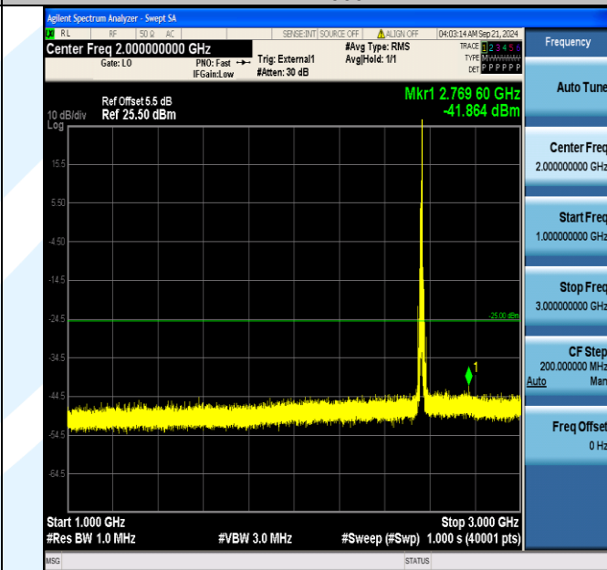
Band41_10MHz_16QAM_40290_1RB#49_1000~3000_1000~3000
