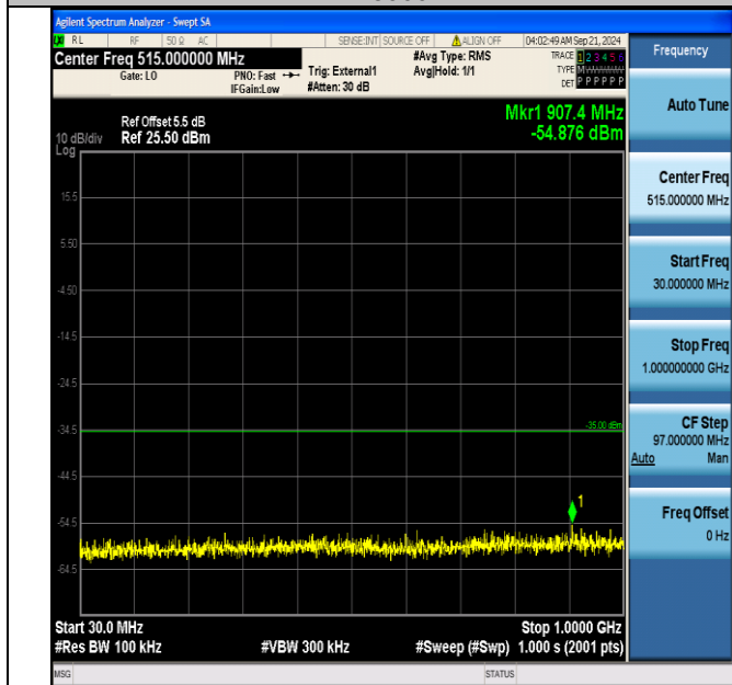
Band41_10MHz_16QAM_40290_1RB#49_30~1000_30~1000
