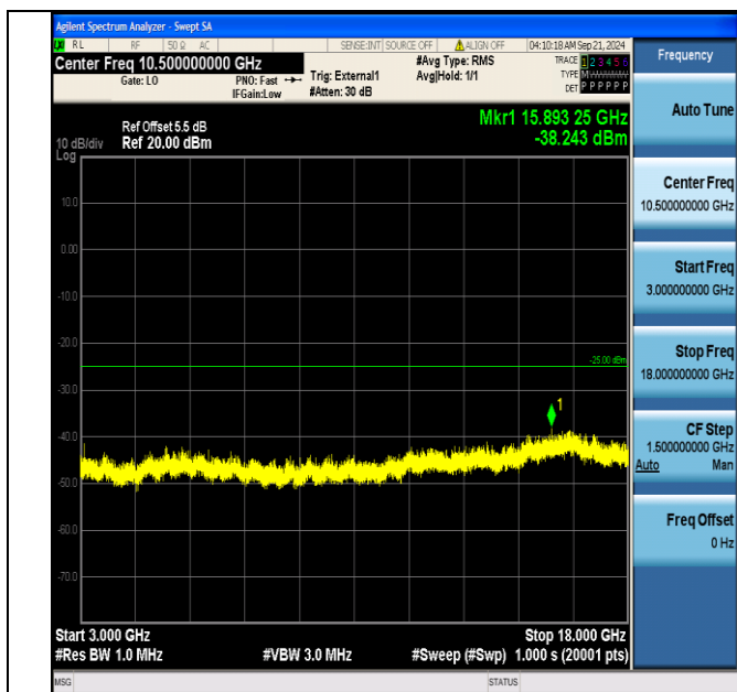
Band41_10MHz_16QAM_40690_1RB#0_3000~18000_3000~18000
