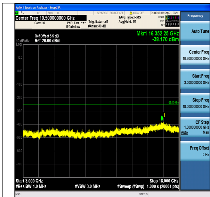
Band41_10MHz_16QAM_40290_1RB#0_3000~18000_3000~18000
