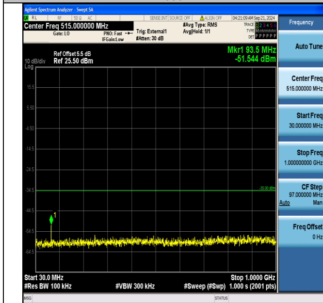
Band41_10MHz_QPSK_41190_1RB#49_30~1000_30~1000
