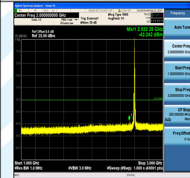
Band41_10MHz_16QAM_40690_1RB#0_1000~3000_1000~3000
