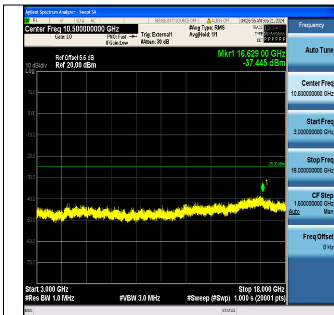
Band41_10MHz_16QAM_41190_50RB#0_3000~18000_3000~18000
