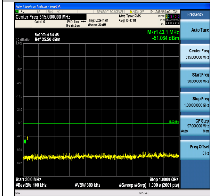
Band41_10MHz_16QAM_40690_1RB#49_30~1000_30~1000
