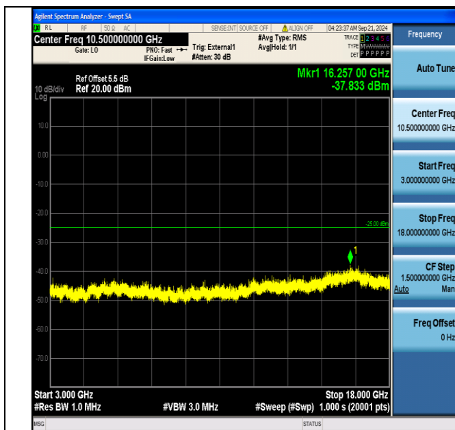
Band41_10MHz_16QAM_41190_1RB#49_3000~18000_3000~18000
