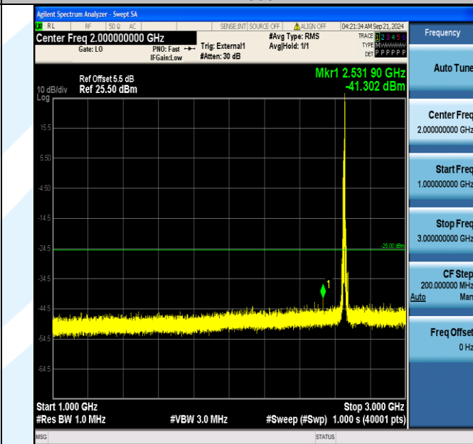
Band41_10MHz_QPSK_41190_1RB#49_1000~3000_1000~3000
