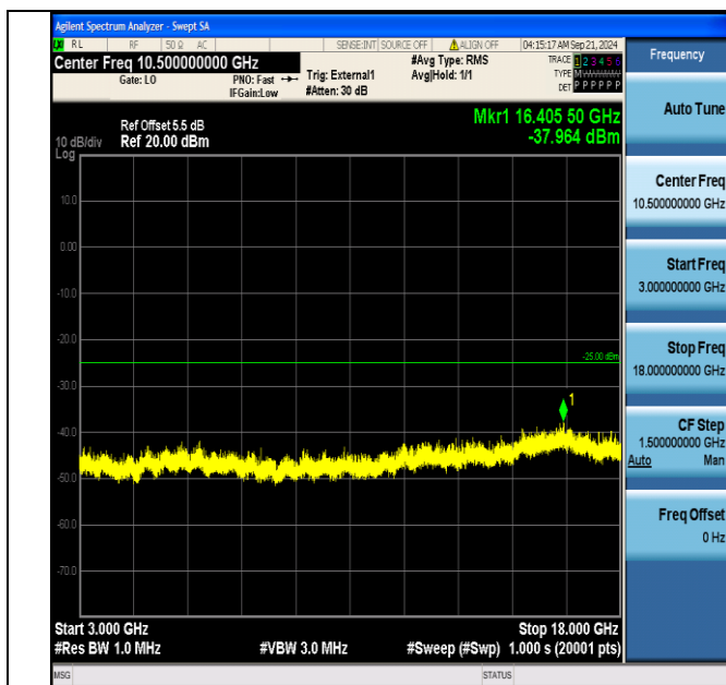
Band41_10MHz_QPSK_40690_50RB#0_3000~18000_3000~18000
