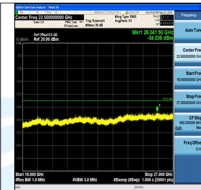
Band41_10MHz_16QAM_41190_1RB#49_18000~27000_18000~27000
