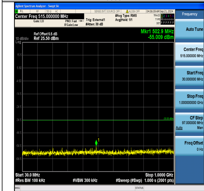
Band41_10MHz_16QAM_40290_50RB#0_30~1000_30~1000
