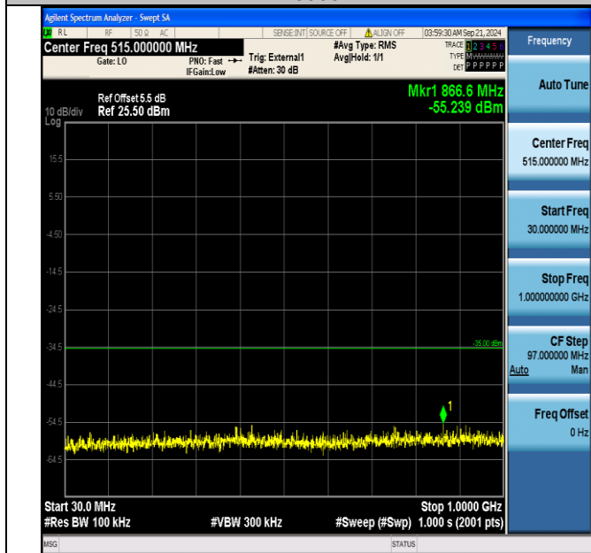
Band41_10MHz_16QAM_40290_1RB#0_30~1000_30~1000
