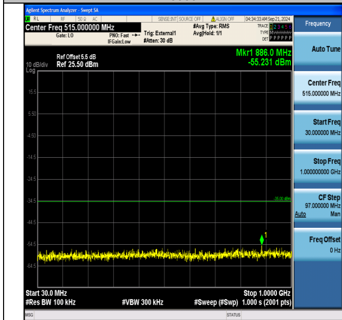
Band41_15MHz_QPSK_40315_75RB#0_30~1000_30~1000
