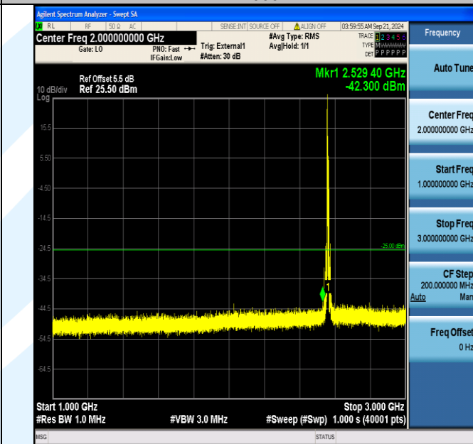
Band41_10MHz_16QAM_40290_1RB#0_1000~3000_1000~3000
