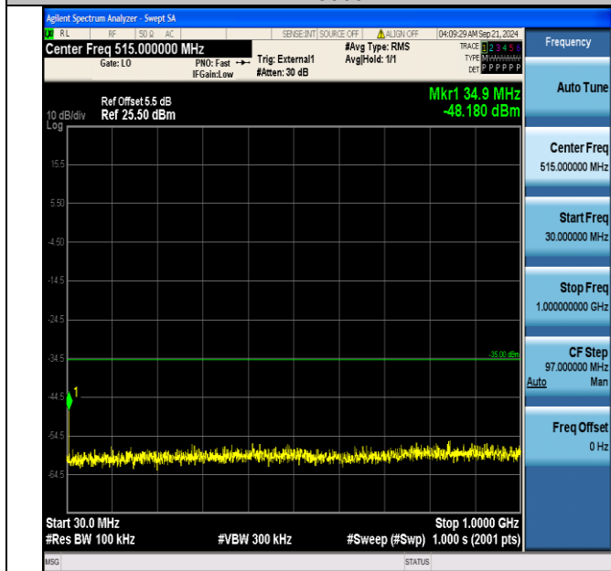
Band41_10MHz_16QAM_40690_1RB#0_30~1000_30~1000
