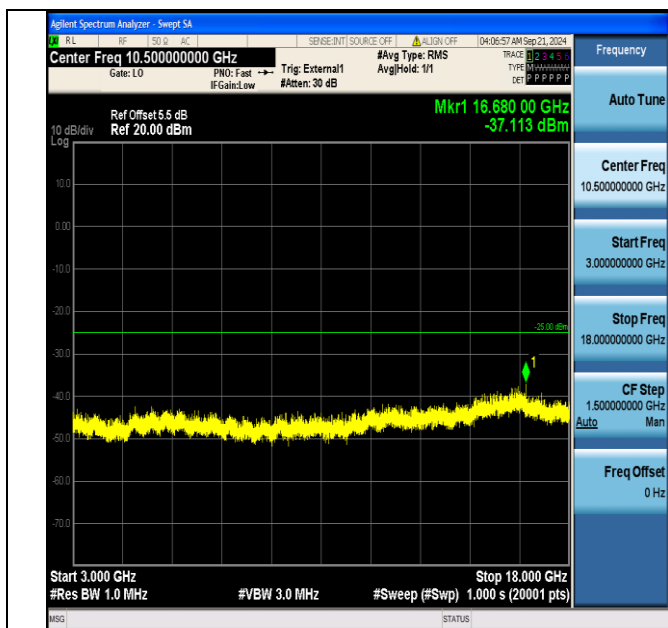
Band41_10MHz_16QAM_40290_50RB#0_3000~18000_3000~18000
