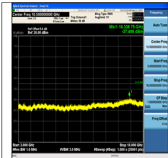
Band41_15MHz_QPSK_40315_1RB#74_3000~18000_3000~18000
