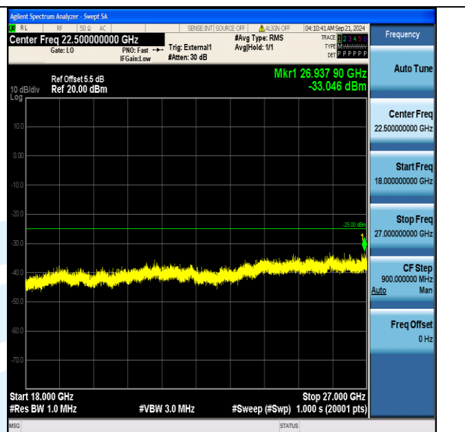
Band41_10MHz_16QAM_40690_1RB#0_18000~27000_18000~27000
