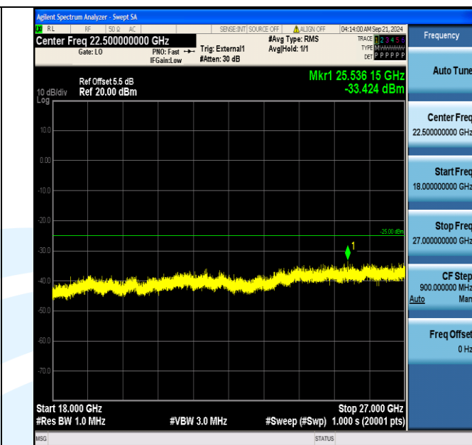
Band41_10MHz_16QAM_40690_1RB#49_18000~27000_18000~27000
