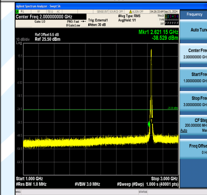
Band41_10MHz_16QAM_41190_50RB#0_1000~3000_1000~3000
