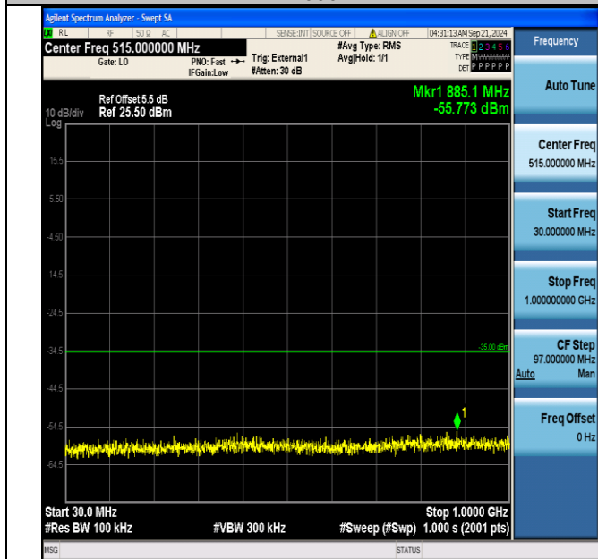
Band41_15MHz_QPSK_40315_1RB#74_30~1000_30~1000
