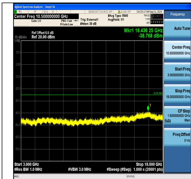
Band41_10MHz_QPSK_41190_50RB#0_3000~18000_3000~18000
