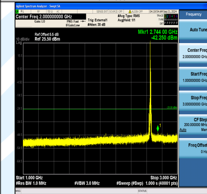
Band41_10MHz_16QAM_41190_1RB#0_1000~3000_1000~3000
