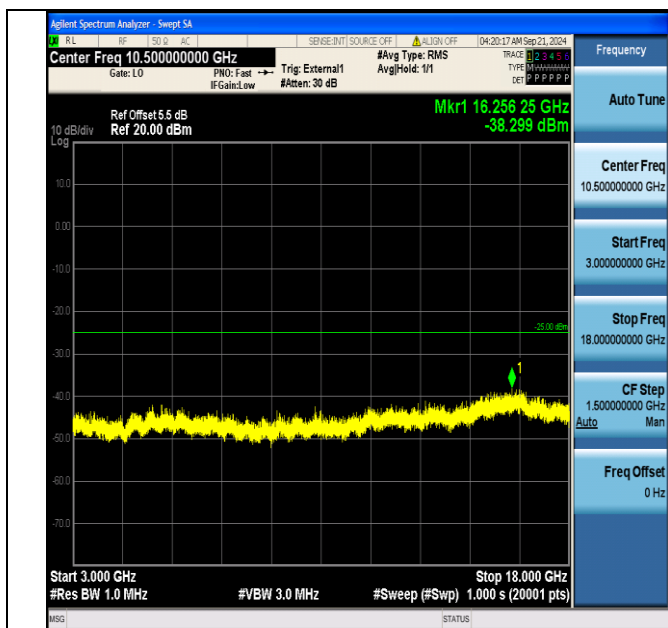
Band41_10MHz_16QAM_41190_1RB#0_3000~18000_3000~18000
