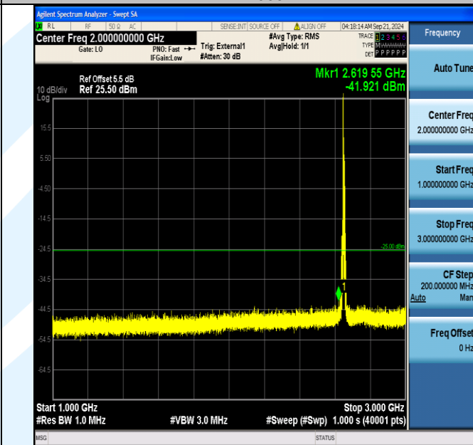
Band41_10MHz_QPSK_41190_1RB#0_1000~3000_1000~3000
