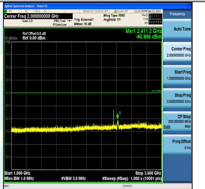
Band40_5MHz_16QAM_39225_1RB#24_1000~3000_1000~3000
