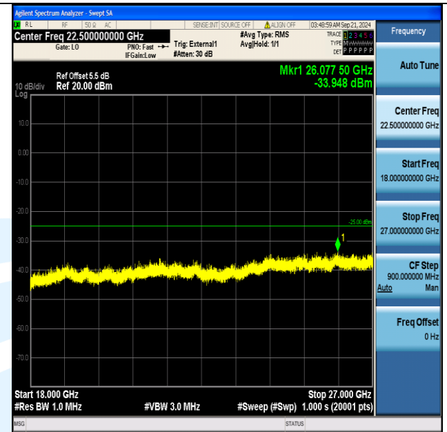
Band41_5MHz_QPSK_41215_1RB#0_18000~27000_18000~27000
