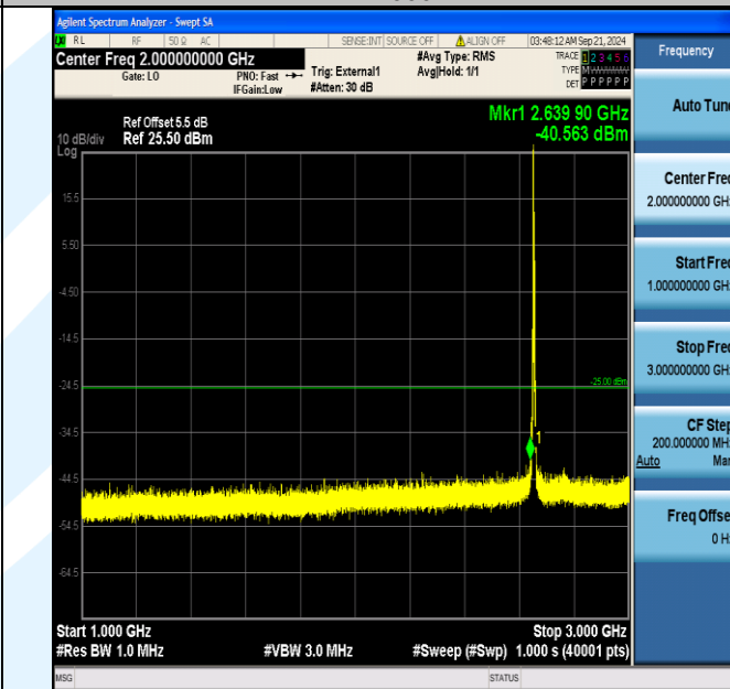
Band41_5MHz_QPSK_41215_1RB#0_1000~3000_1000~3000
