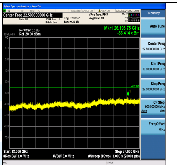
Band41_5MHz_QPSK_40265_1RB#24_18000~27000_18000~27000
