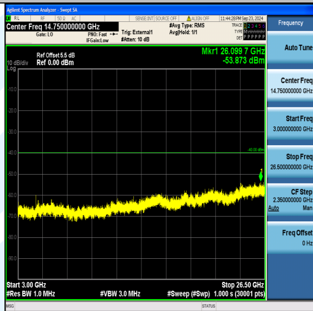
Band40_5MHz_16QAM_39225_25RB#0_3000~26500_3000~26500
