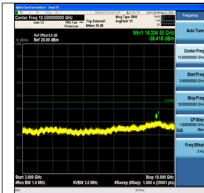
Band41_5MHz_QPSK_40690_1RB#24_3000~18000_3000~18000
