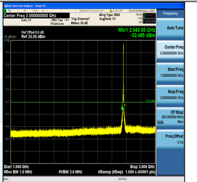
Band41_5MHz_QPSK_40265_25RB#0_1000~3000_1000~3000
