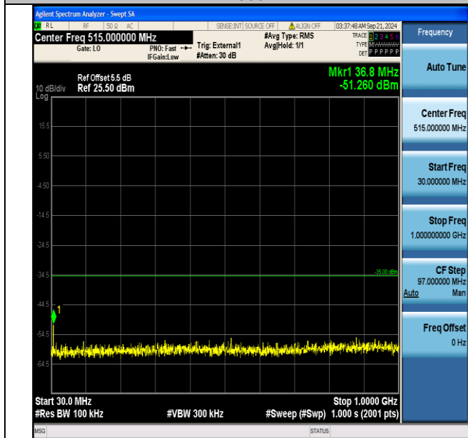
Band41_5MHz_QPSK_40690_1RB#0_30~1000_30~1000
