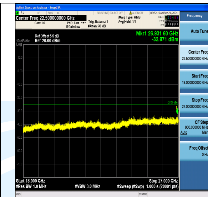
Band41_5MHz_QPSK_41215_1RB#24_18000~27000_18000~27000
