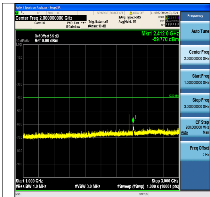
Band40_10MHz_QPSK_39200_1RB#49_1000~3000_1000~3000
