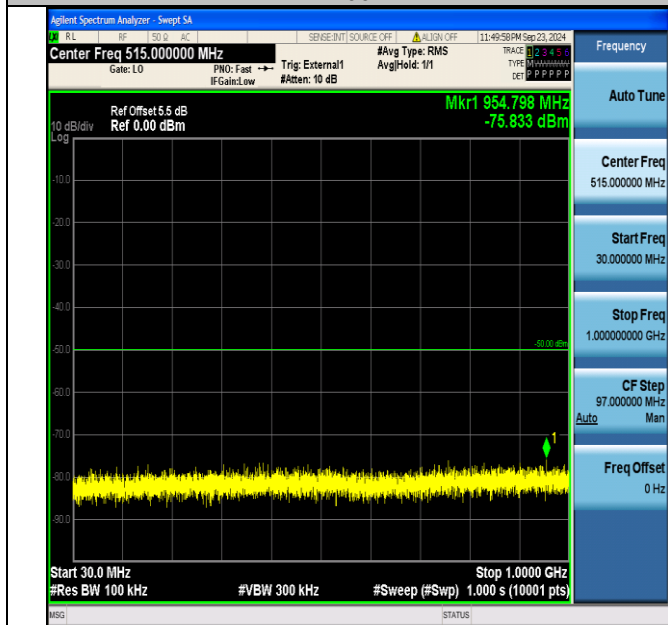
Band40_10MHz_QPSK_39200_50RB#0_30~1000_30~1000
