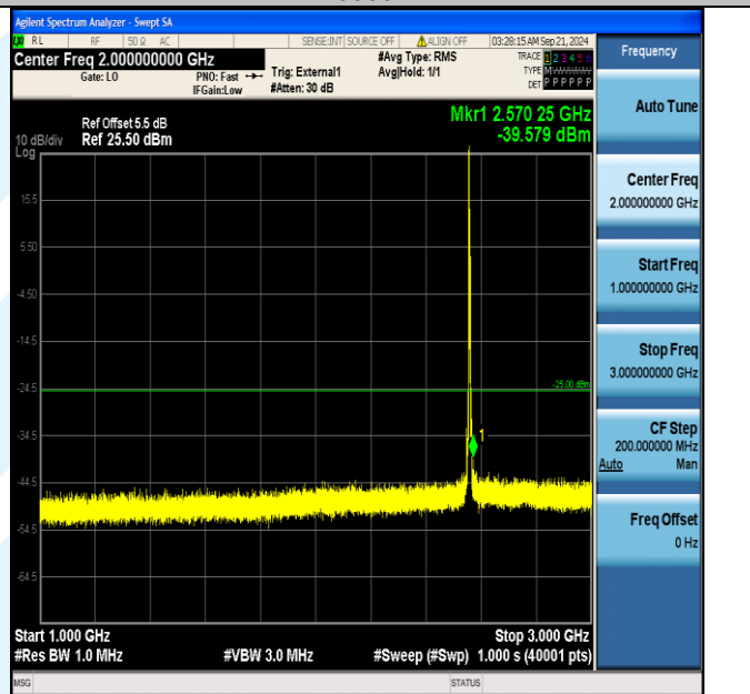
Band41_5MHz_QPSK_40265_1RB#0_1000~3000_1000~3000
