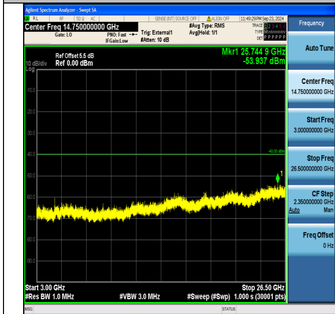
Band40_10MHz_16QAM_39200_1RB#49_3000~26500_3000~26500
