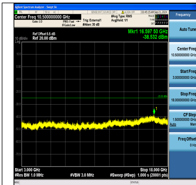
Band41_5MHz_QPSK_40690_25RB#0_3000~18000_3000~18000
