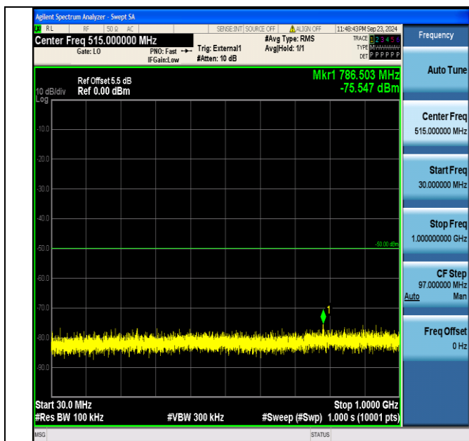
Band40_10MHz_16QAM_39200_1RB#49_30~1000_30~1000
