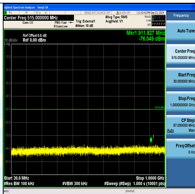
Band40_5MHz_16QAM_39225_25RB#0_30~1000_30~1000
