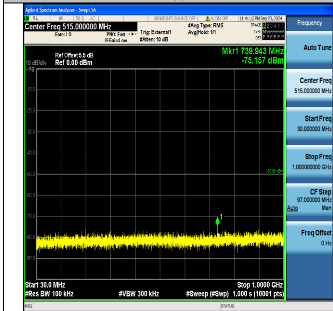
Band40_5MHz_16QAM_39225_1RB#24_30~1000_30~1000
