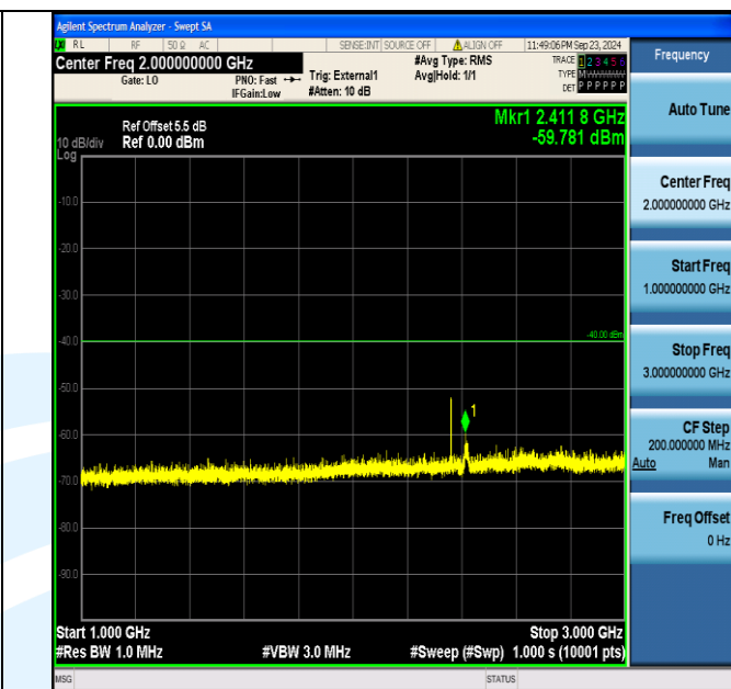
Band40_10MHz_16QAM_39200_1RB#49_1000~3000_1000~3000
