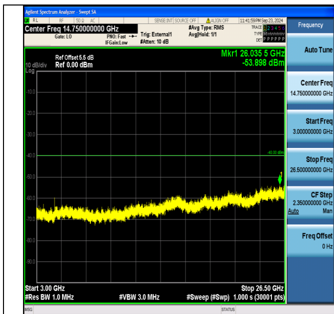
Band40_5MHz_16QAM_39225_1RB#24_3000~26500_3000~26500
