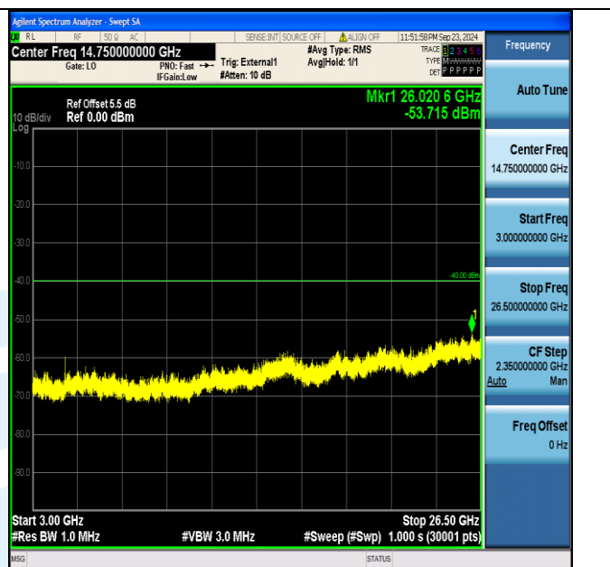
Band40_10MHz_16QAM_39200_50RB#0_3000~26500_3000~26500
