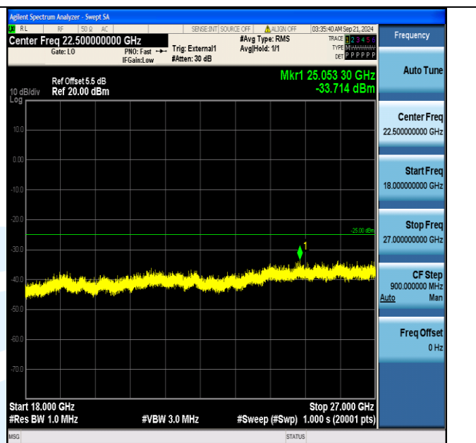
Band41_5MHz_QPSK_40265_25RB#0_18000~27000_18000~27000
