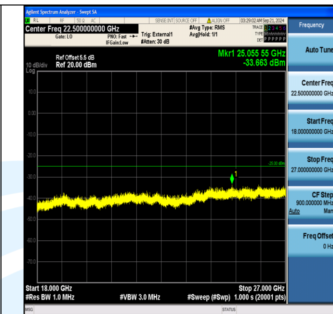
Band41_5MHz_QPSK_40265_1RB#0_18000~27000_18000~27000
