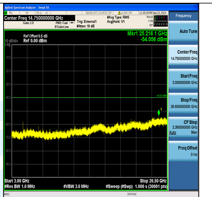
Band40_5MHz_16QAM_39225_1RB#0_3000~26500_3000~26500
