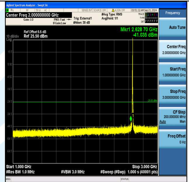
Band41_5MHz_QPSK_41215_1RB#24_1000~3000_1000~3000
