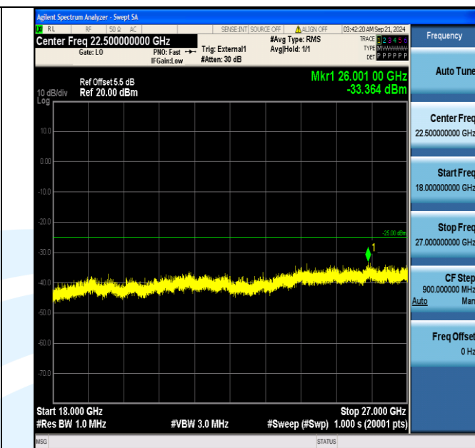
Band41_5MHz_QPSK_40690_1RB#24_18000~27000_18000~27000
