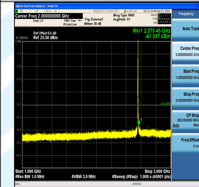
Band41_5MHz_QPSK_40265_1RB#24_1000~3000_1000~3000
