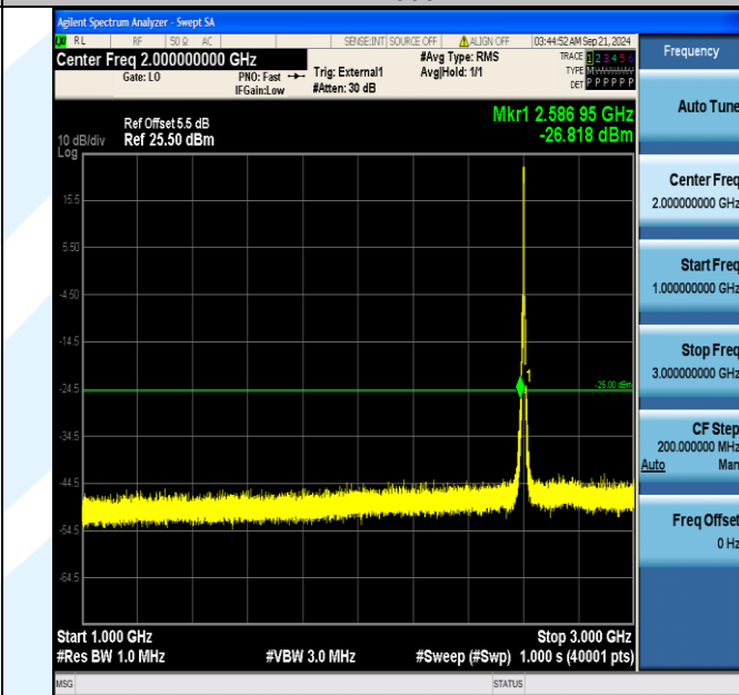
Band41_5MHz_QPSK_40690_25RB#0_1000~3000_1000~3000
