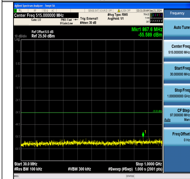
Band41_5MHz_QPSK_40265_1RB#24_30~1000_30~1000
