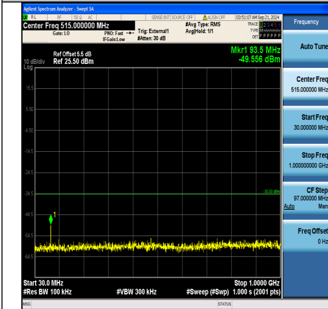
Band41_5MHz_QPSK_41215_1RB#24_30~1000_30~1000
