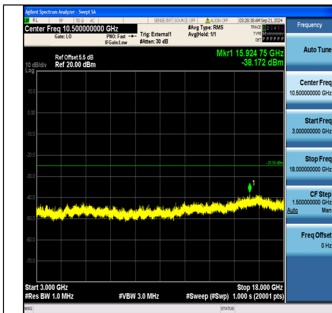
Band41_5MHz_QPSK_40265_1RB#0_3000~18000_3000~18000
