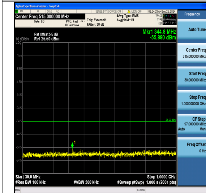
Band41_5MHz_QPSK_41215_25RB#0_30~1000_30~1000
