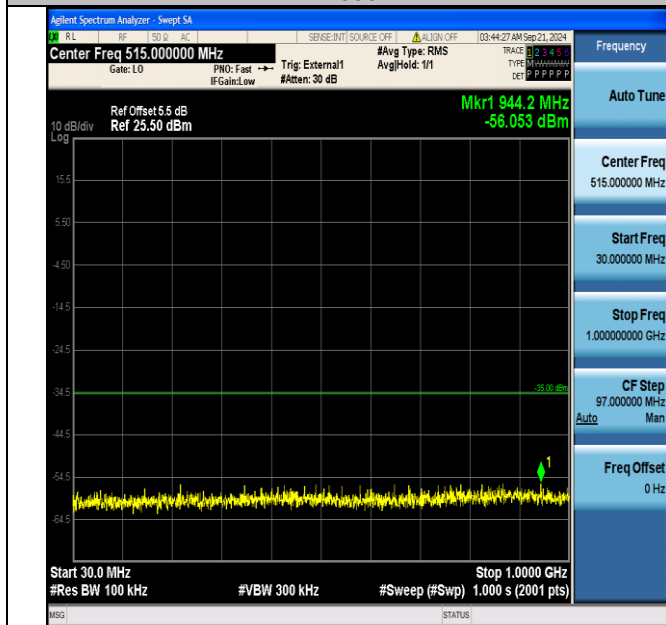
Band41_5MHz_QPSK_40690_25RB#0_30~1000_30~1000
