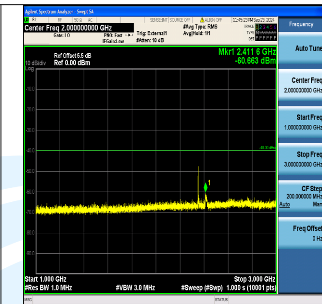
Band40_10MHz_QPSK_39200_1RB#0_1000~3000_1000~3000
