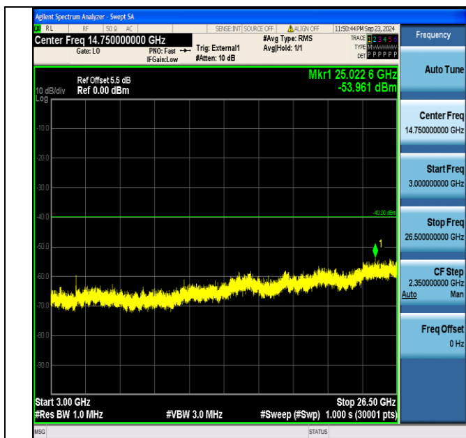
Band40_10MHz_QPSK_39200_50RB#0_3000~26500_3000~26500
