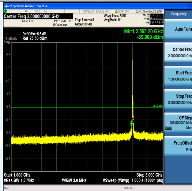
Band41_5MHz_QPSK_40690_1RB#24_1000~3000_1000~3000
