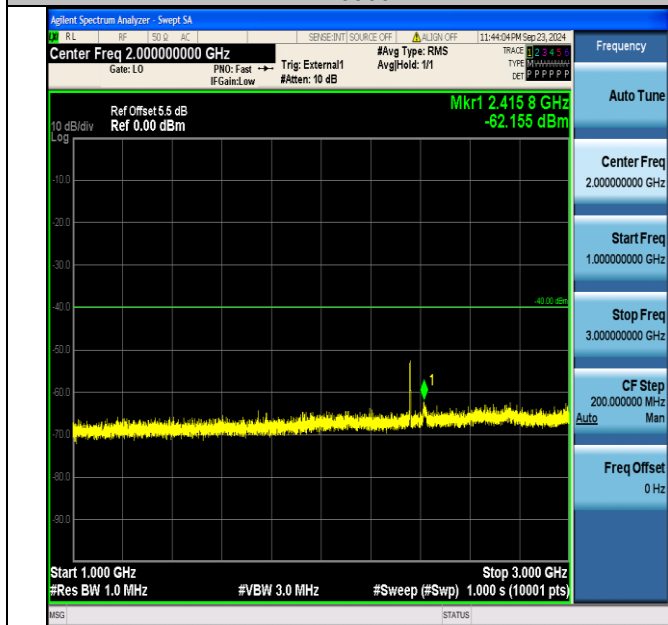
Band40_5MHz_16QAM_39225_25RB#0_1000~3000_1000~3000
