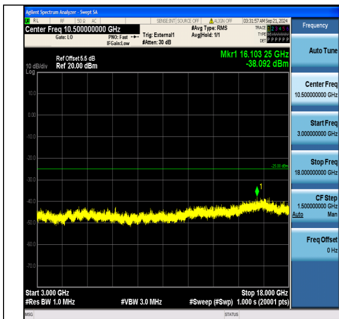
Band41_5MHz_QPSK_40265_1RB#24_3000~18000_3000~18000
