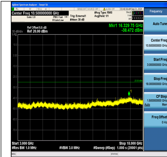
Band41_5MHz_QPSK_41215_1RB#0_3000~18000_3000~18000
