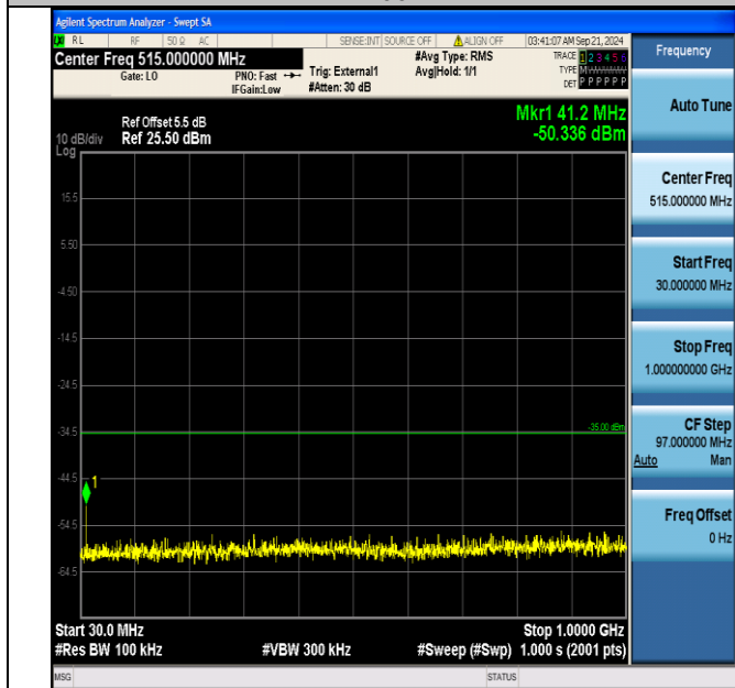
Band41_5MHz_QPSK_40690_1RB#24_30~1000_30~1000
