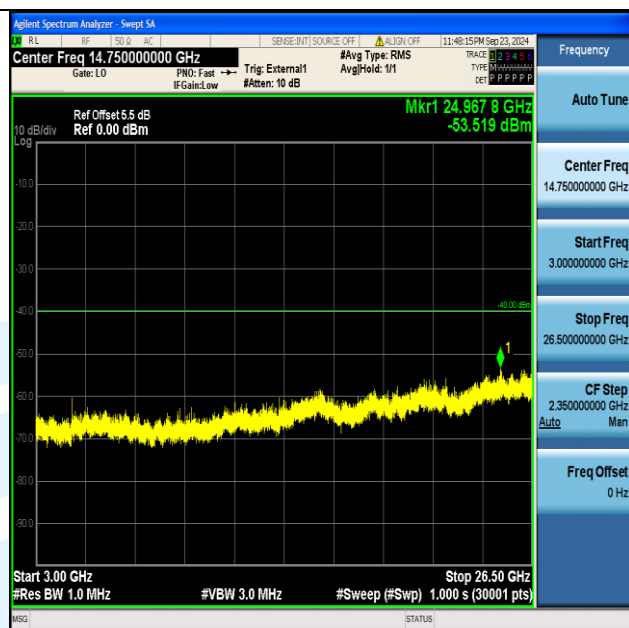
Band40_10MHz_QPSK_39200_1RB#49_3000~26500_3000~26500
