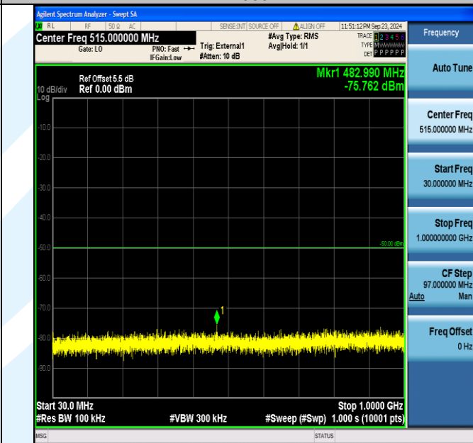
Band40_10MHz_16QAM_39200_50RB#0_30~1000_30~1000
