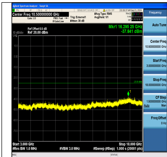
Band41_5MHz_QPSK_40690_1RB#0_3000~18000_3000~18000
