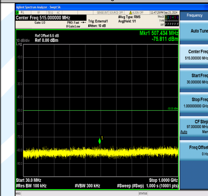
Band40_10MHz_QPSK_39200_1RB#49_30~1000_30~1000
