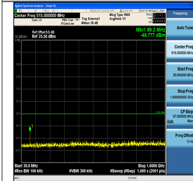
Band41_5MHz_QPSK_41215_1RB#0_30~1000_30~1000
