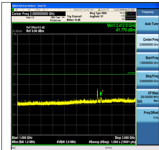
Band40_10MHz_16QAM_39200_50RB#0_1000~3000_1000~3000
