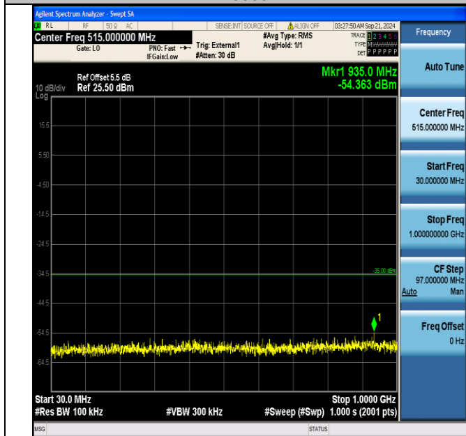
Band41_5MHz_QPSK_40265_1RB#0_30~1000_30~1000
