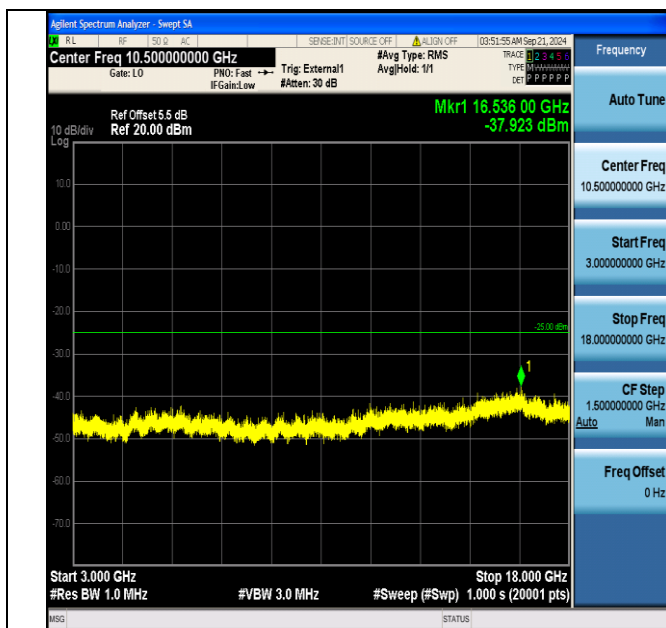
Band41_5MHz_QPSK_41215_1RB#24_3000~18000_3000~18000
