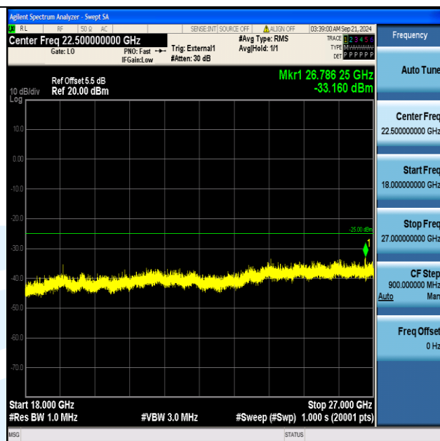
Band41_5MHz_QPSK_40690_1RB#0_18000~27000_18000~27000
