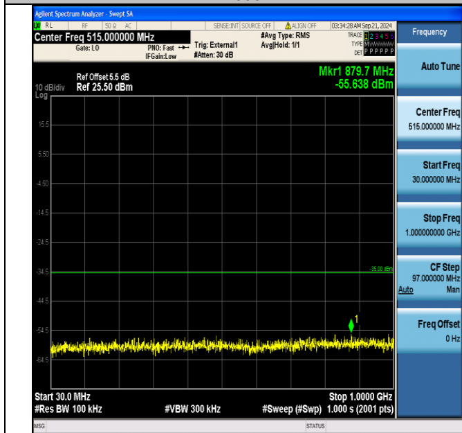
Band41_5MHz_QPSK_40265_25RB#0_30~1000_30~1000
