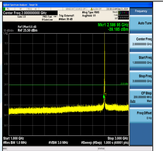
Band41_5MHz_QPSK_40690_1RB#0_1000~3000_1000~3000
