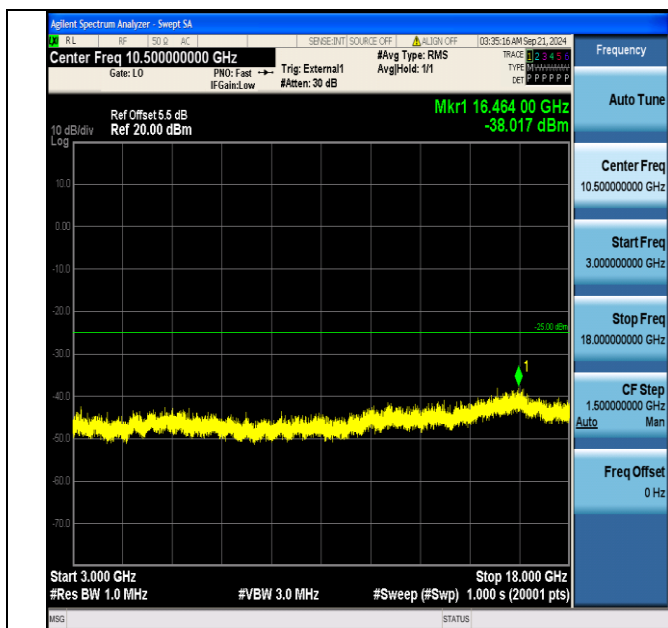
Band41_5MHz_QPSK_40265_25RB#0_3000~18000_3000~18000
