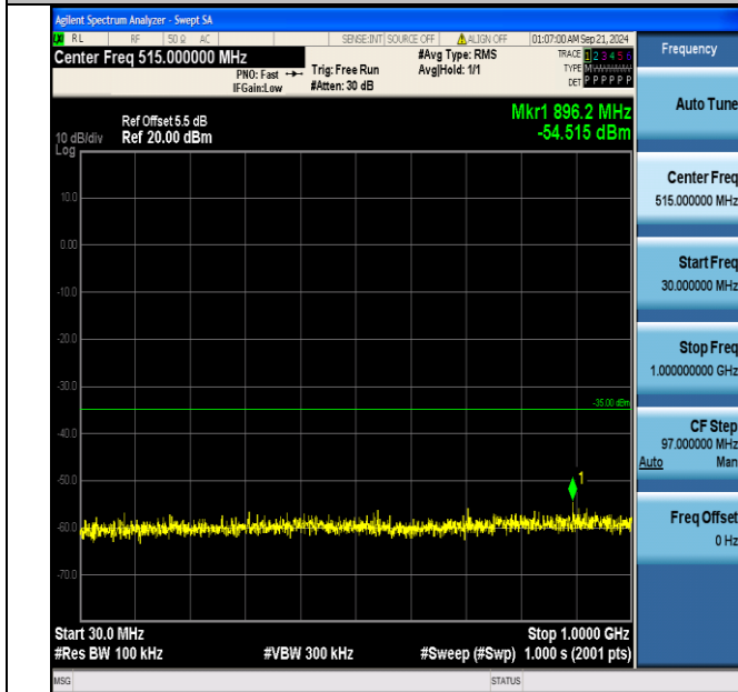
Band7_15MHz_QPSK_21375_1RB#74_30~1000_30~1000
