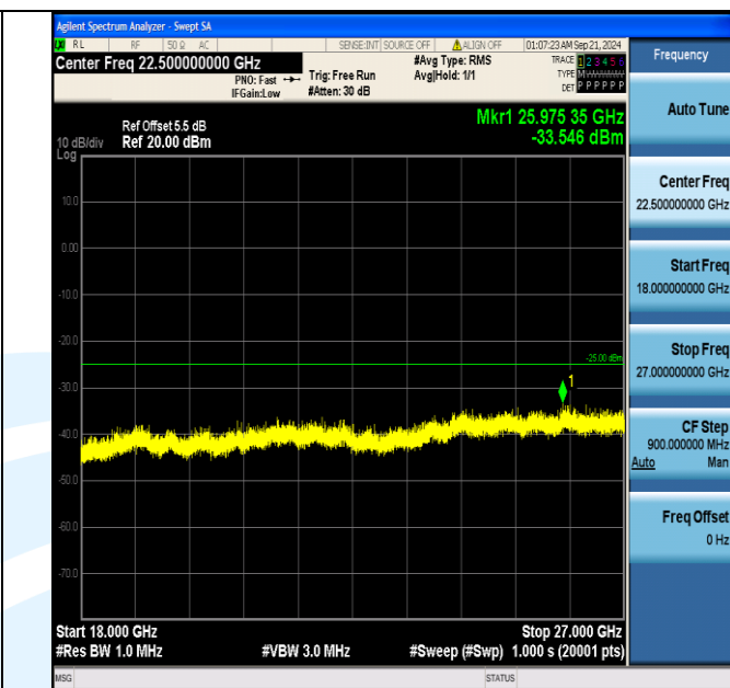
Band7_15MHz_QPSK_21375_1RB#74_18000~27000_18000~27000
