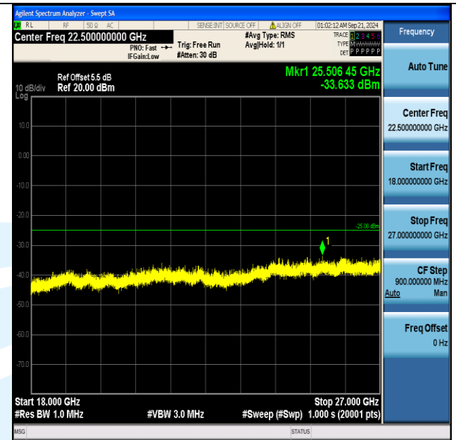
Band7_15MHz_16QAM_20825_75RB#0_18000~27000_18000~27000
