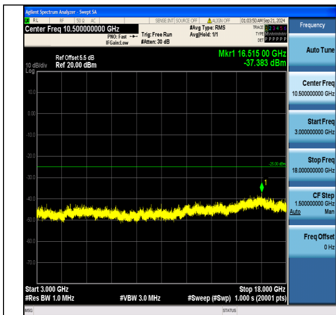
Band7_15MHz_QPSK_21100_1RB#74_3000~18000_3000~18000
