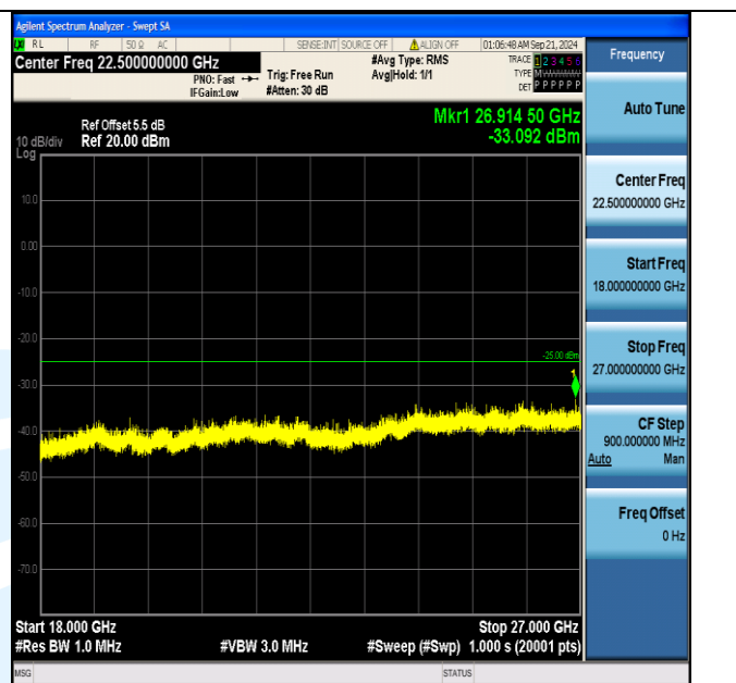
Band7_15MHz_16QAM_21375_1RB#0_18000~27000_18000~27000
