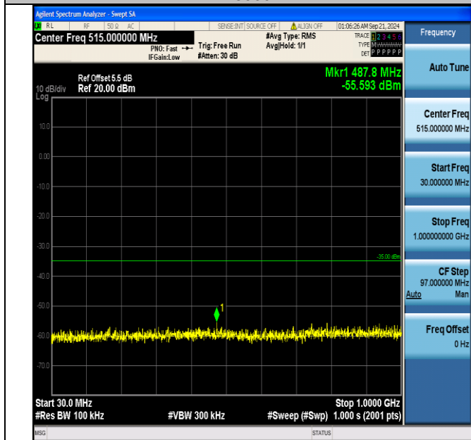
Band7_15MHz_16QAM_21375_1RB#0_30~1000_30~1000
