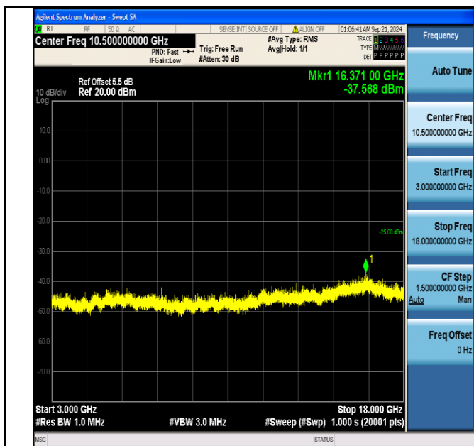
Band7_15MHz_16QAM_21375_1RB#0_3000~18000_3000~18000
