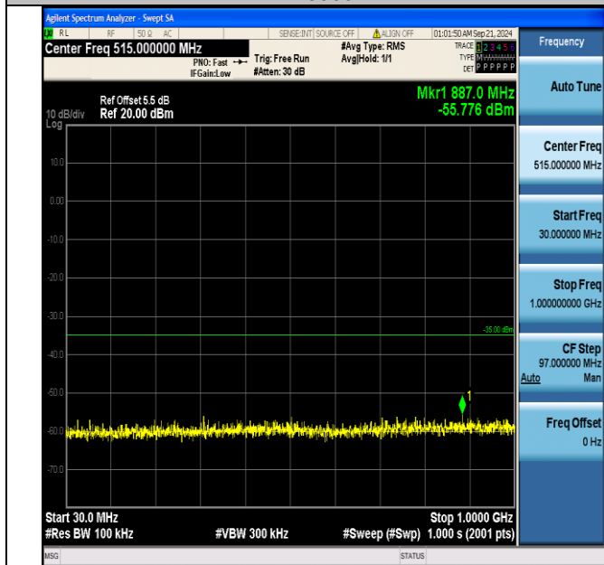
Band7_15MHz_16QAM_20825_75RB#0_30~1000_30~1000
