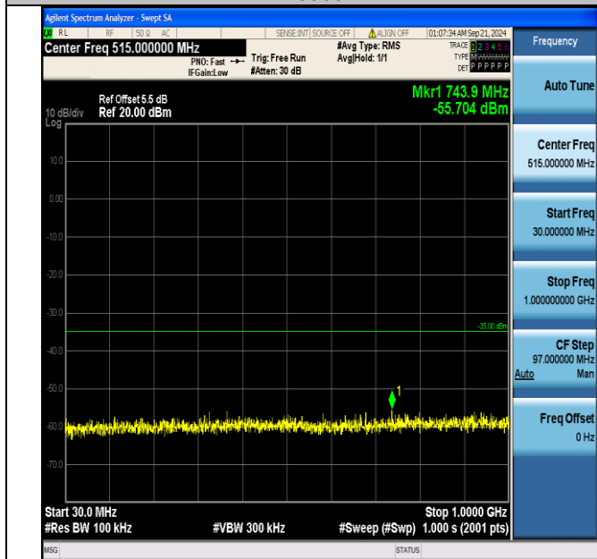
Band7_15MHz_16QAM_21375_1RB#74_30~1000_30~1000
