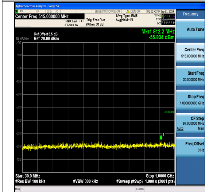
Band7_15MHz_16QAM_20825_1RB#74_30~1000_30~1000
