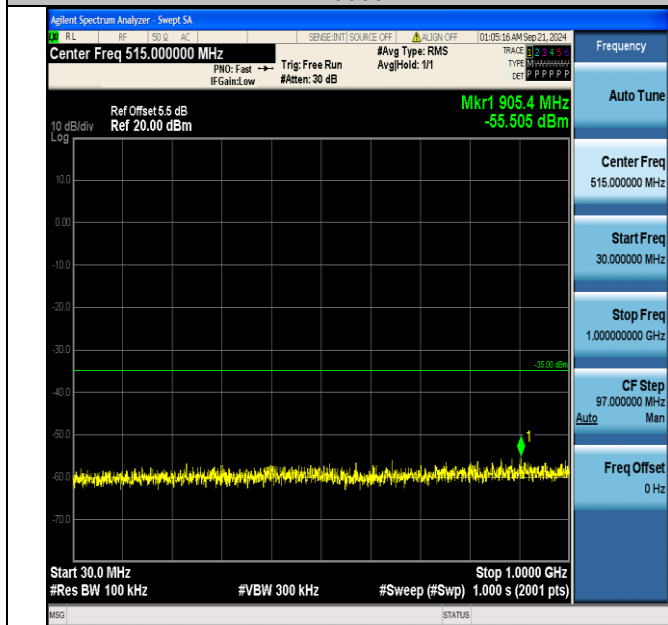
Band7_15MHz_16QAM_21100_75RB#0_30~1000_30~1000
