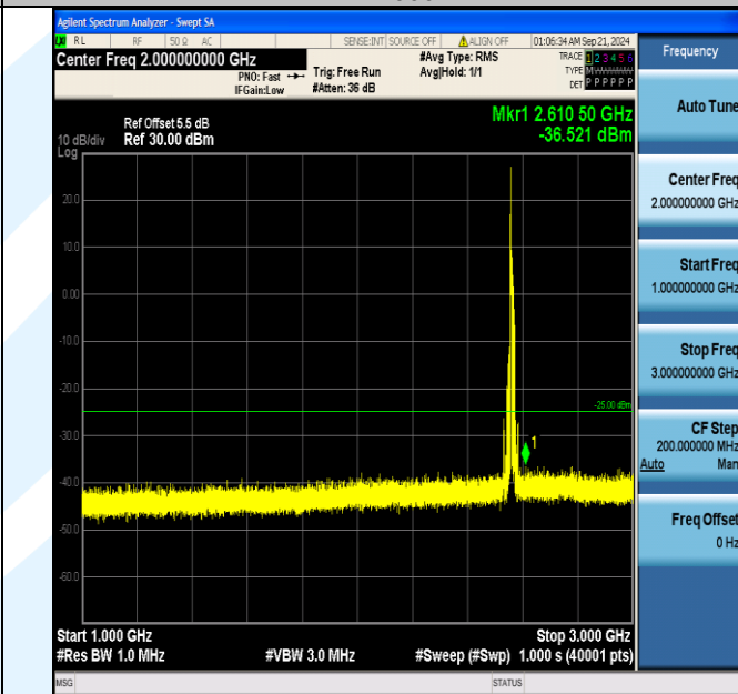
Band7_15MHz_16QAM_21375_1RB#0_1000~3000_1000~3000
