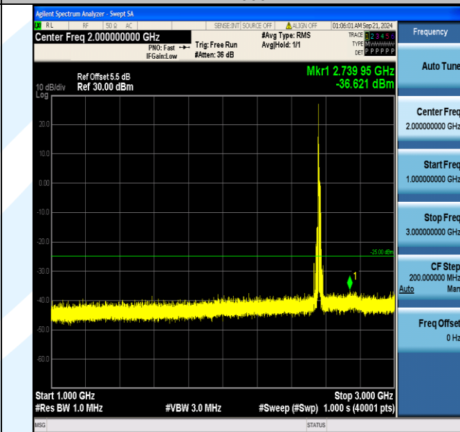
Band7_15MHz_QPSK_21375_1RB#0_1000~3000_1000~3000
