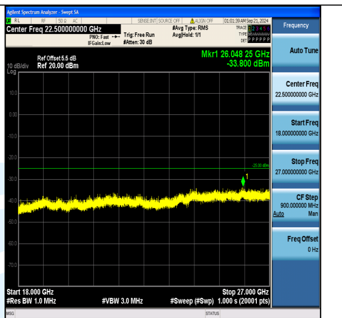
Band7_15MHz_QPSK_20825_75RB#0_18000~27000_18000~27000
