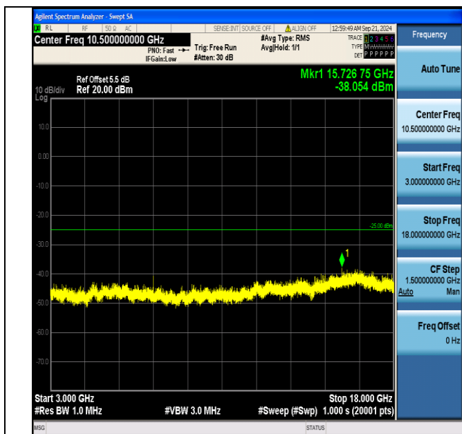
Band7_15MHz_16QAM_20825_1RB#0_3000~18000_3000~18000
