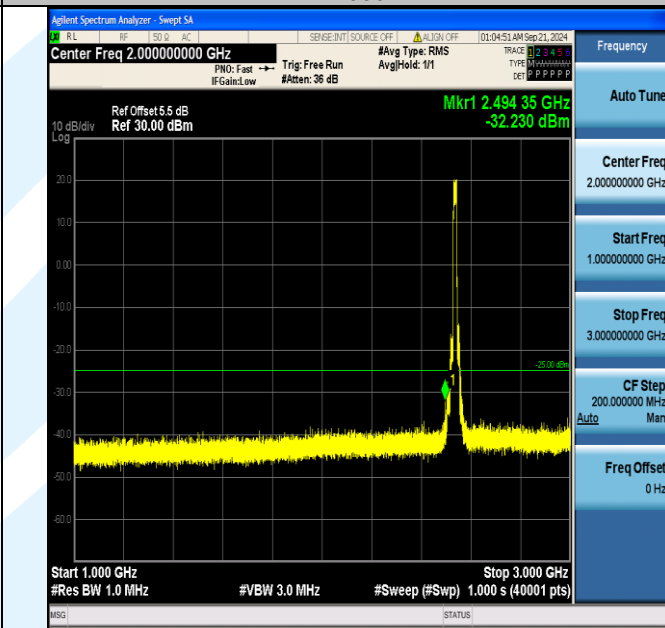
Band7_15MHz_QPSK_21100_75RB#0_1000~3000_1000~3000
