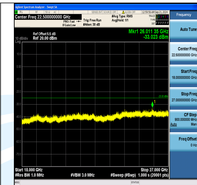
Band7_15MHz_16QAM_20825_1RB#0_18000~27000_18000~27000
