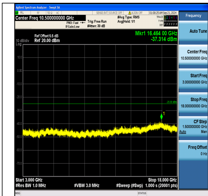
Band7_15MHz_QPSK_21375_75RB#0_3000~18000_3000~18000
