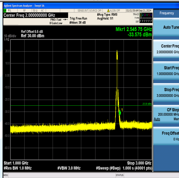
Band7_15MHz_16QAM_20825_75RB#0_1000~3000_1000~3000
