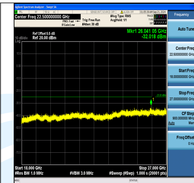
Band7_15MHz_16QAM_21100_75RB#0_18000~27000_18000~27000
