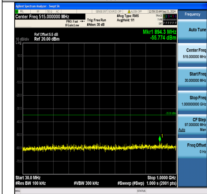
Band7_15MHz_16QAM_20825_1RB#0_30~1000_30~1000
