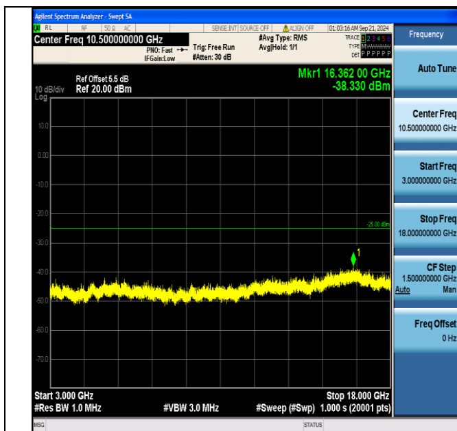
Band7_15MHz_16QAM_21100_1RB#0_3000~18000_3000~18000
