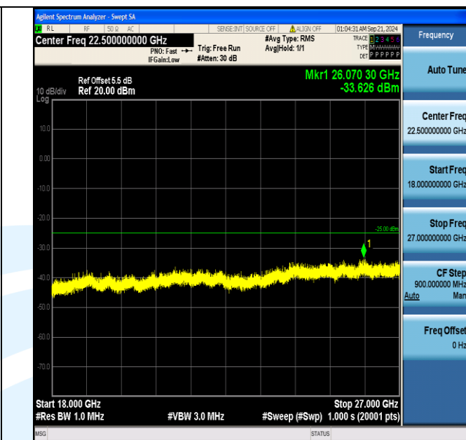
Band7_15MHz_16QAM_21100_1RB#74_18000~27000_18000~27000
