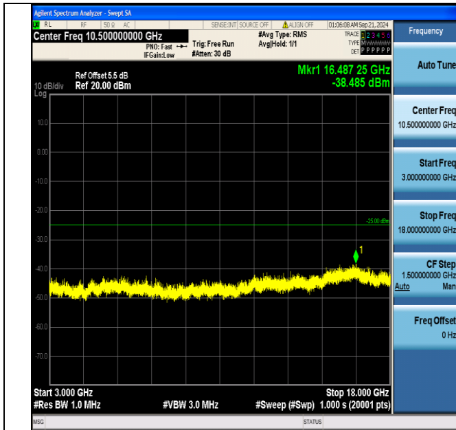
Band7_15MHz_QPSK_21375_1RB#0_3000~18000_3000~18000
