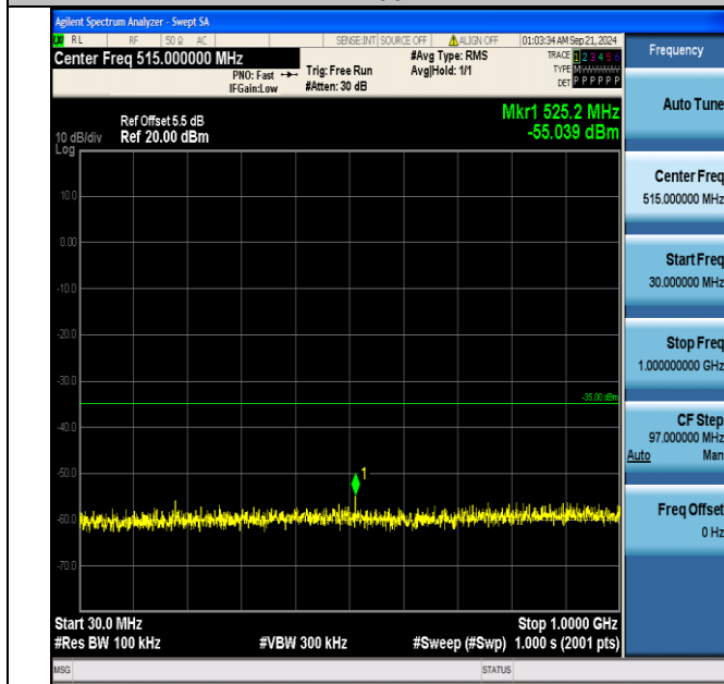
Band7_15MHz_QPSK_21100_1RB#74_30~1000_30~1000
