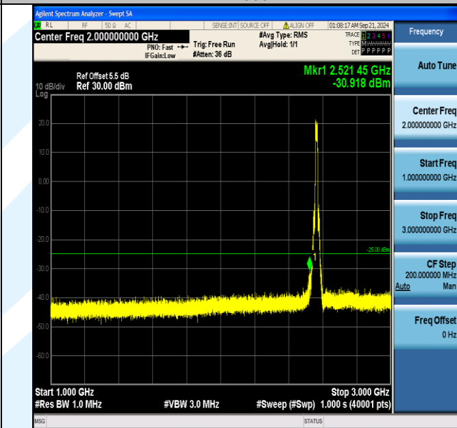
Band7_15MHz_QPSK_21375_75RB#0_1000~3000_1000~3000
