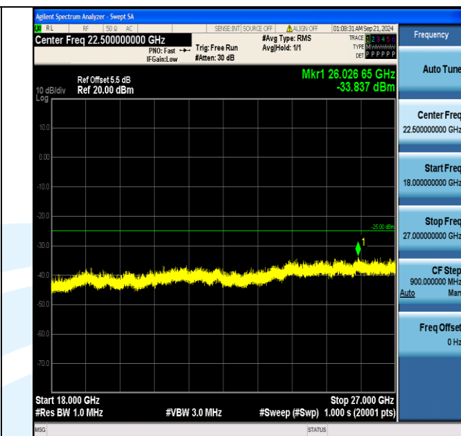
Band7_15MHz_QPSK_21375_75RB#0_18000~27000_18000~27000
