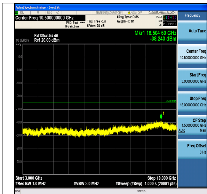
Band7_15MHz_16QAM_20825_1RB#74_3000~18000_3000~18000
