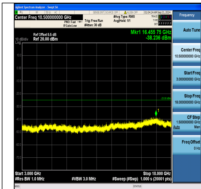
Band7_15MHz_16QAM_21100_1RB#74_3000~18000_3000~18000
