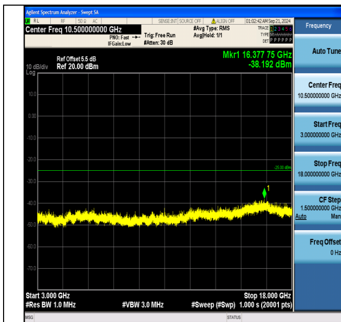
Band7_15MHz_QPSK_21100_1RB#0_3000~18000_3000~18000
