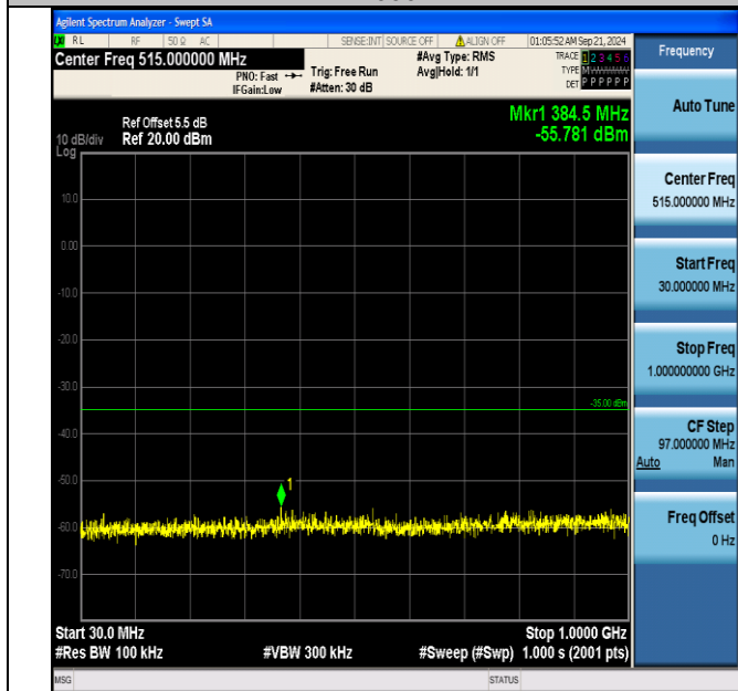
Band7_15MHz_QPSK_21375_1RB#0_30~1000_30~1000
