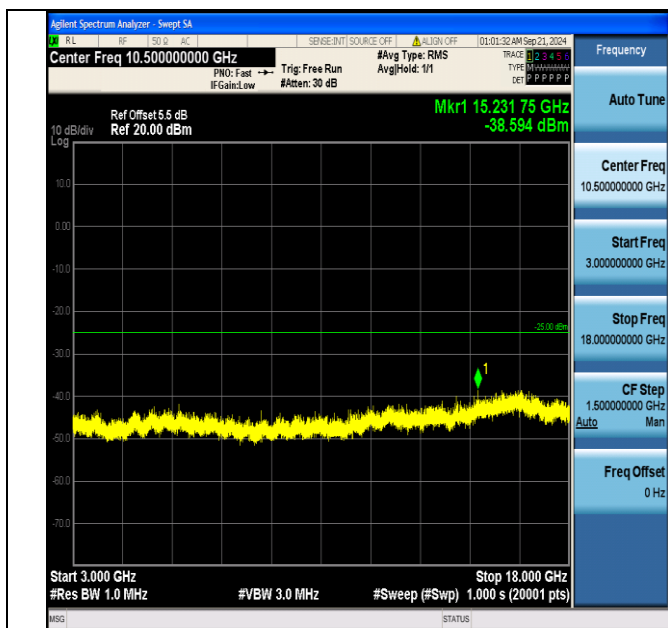
Band7_15MHz_QPSK_20825_75RB#0_3000~18000_3000~18000
