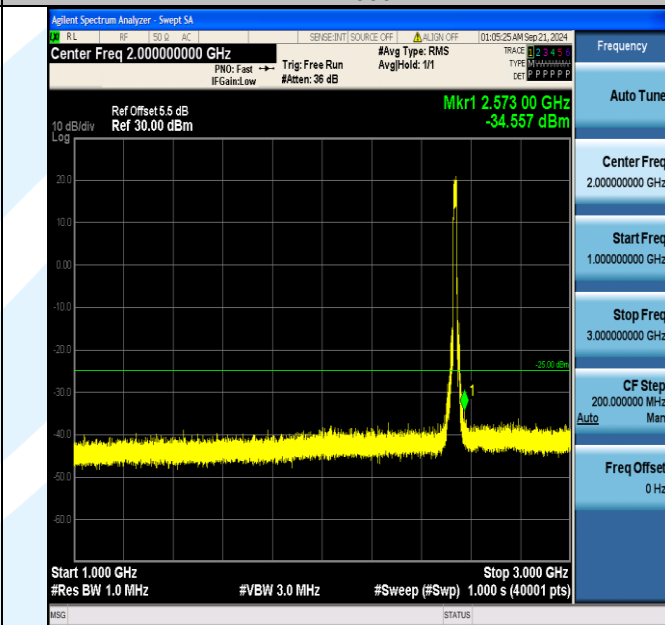
Band7_15MHz_16QAM_21100_75RB#0_1000~3000_1000~3000
