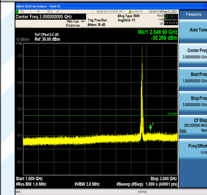
Band7_15MHz_16QAM_21100_1RB#74_1000~3000_1000~3000
