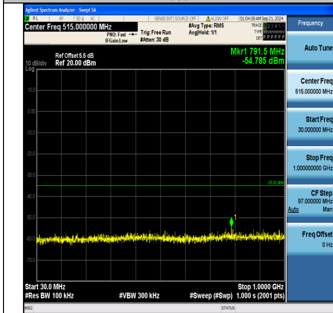
Band7_15MHz_16QAM_21100_1RB#74_30~1000_30~1000
