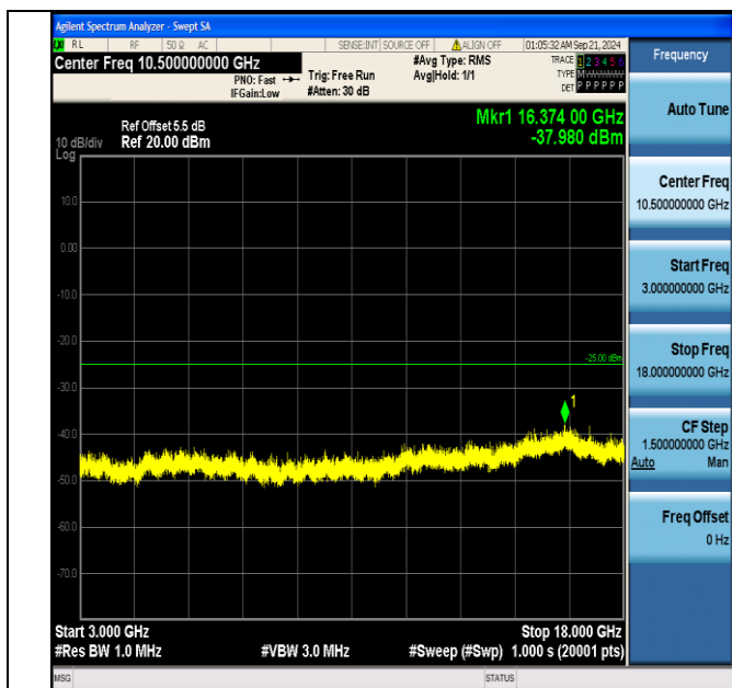
Band7_15MHz_16QAM_21100_75RB#0_3000~18000_3000~18000
