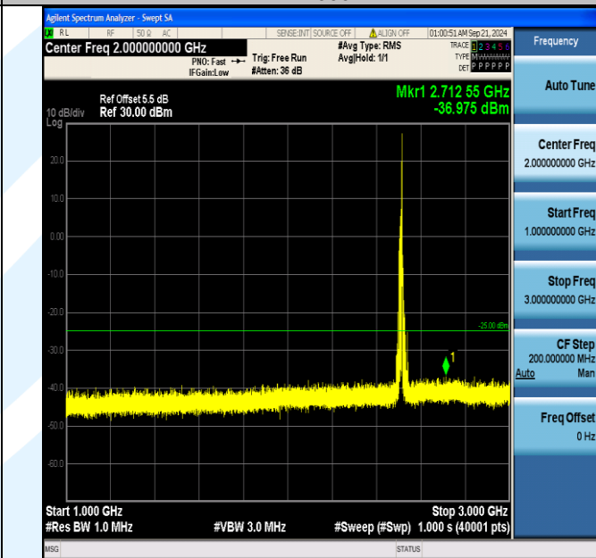
Band7_15MHz_16QAM_20825_1RB#74_1000~3000_1000~3000
