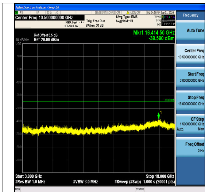
Band7_15MHz_QPSK_21100_75RB#0_3000~18000_3000~18000
