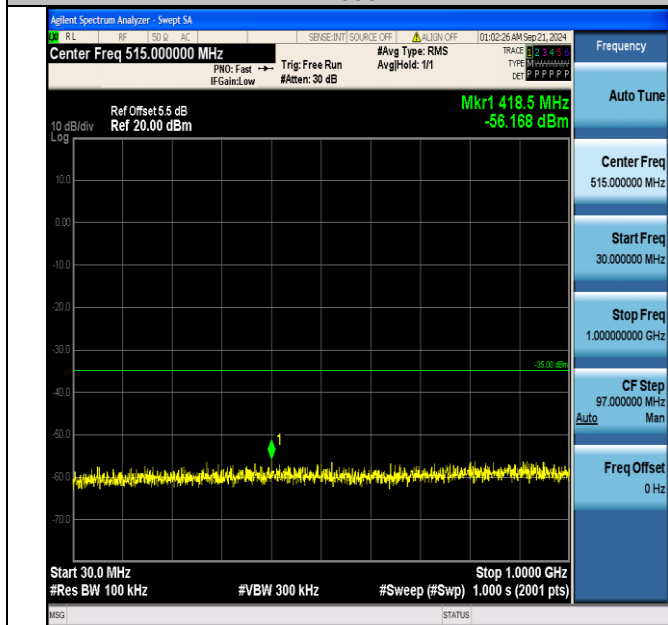
Band7_15MHz_QPSK_21100_1RB#0_30~1000_30~1000
