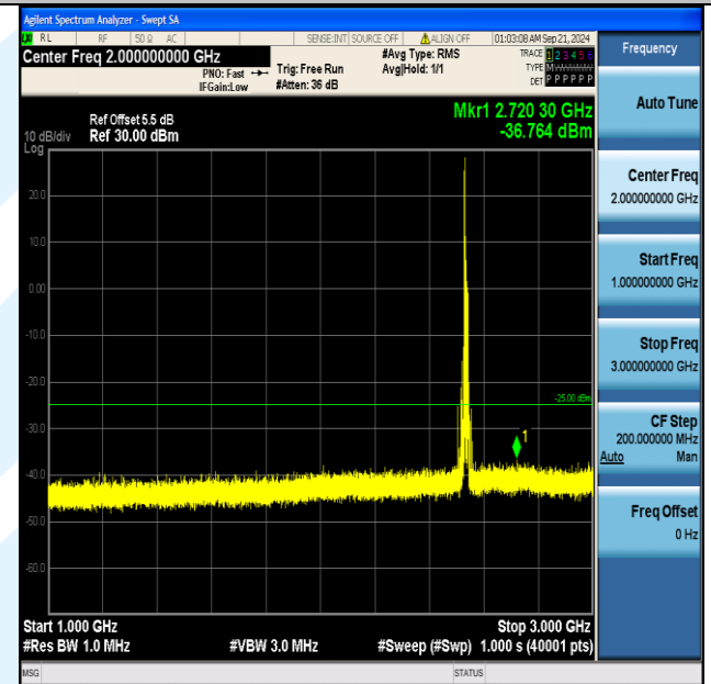
Band7_15MHz_16QAM_21100_1RB#0_1000~3000_1000~3000
