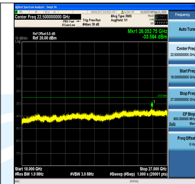
Band7_15MHz_QPSK_21100_1RB#74_18000~27000_18000~27000
