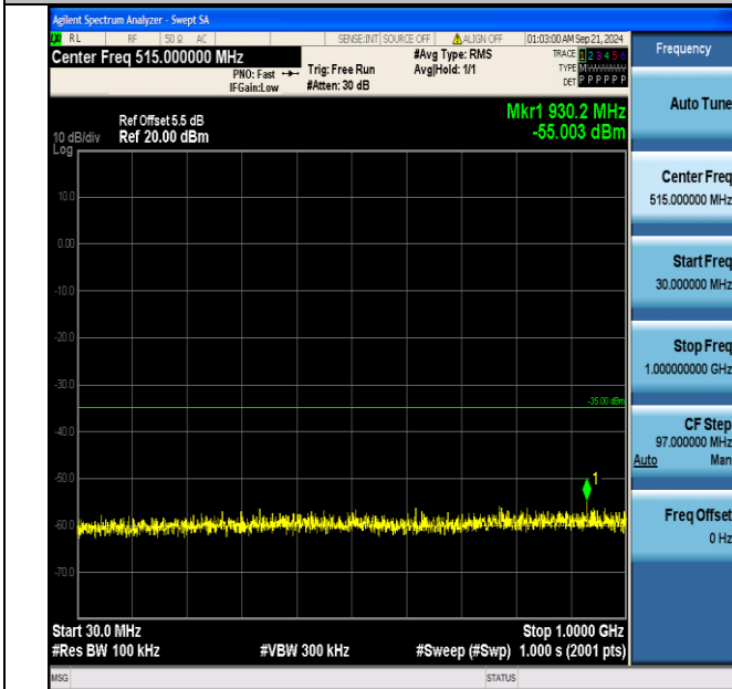
Band7_15MHz_16QAM_21100_1RB#0_30~1000_30~1000
