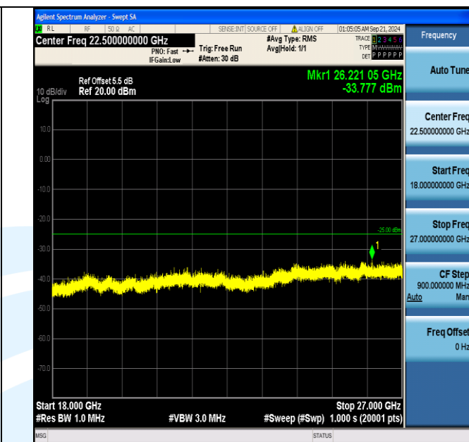
Band7_15MHz_QPSK_21100_75RB#0_18000~27000_18000~27000
