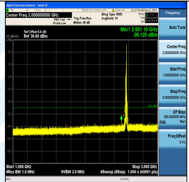
Band7_15MHz_QPSK_21375_1RB#74_1000~3000_1000~3000
