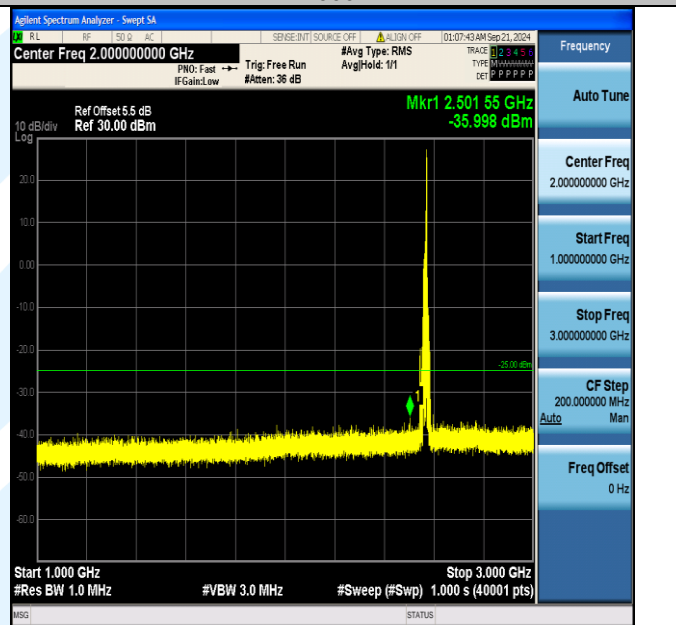
Band7_15MHz_16QAM_21375_1RB#74_1000~3000_1000~3000
