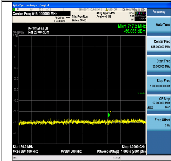
Band7_15MHz_QPSK_21100_75RB#0_30~1000_30~1000
