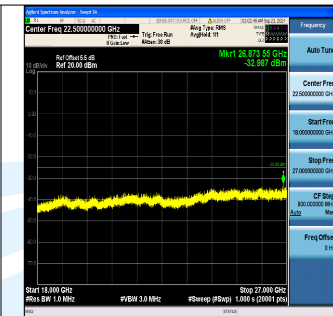
Band7_15MHz_QPSK_21100_1RB#0_18000~27000_18000~27000
