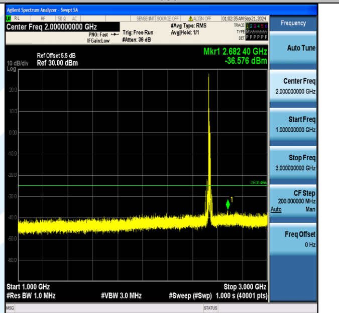
Band7_15MHz_QPSK_21100_1RB#0_1000~3000_1000~3000
