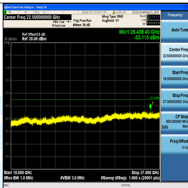
Band7_15MHz_16QAM_20825_1RB#74_18000~27000_18000~27000
