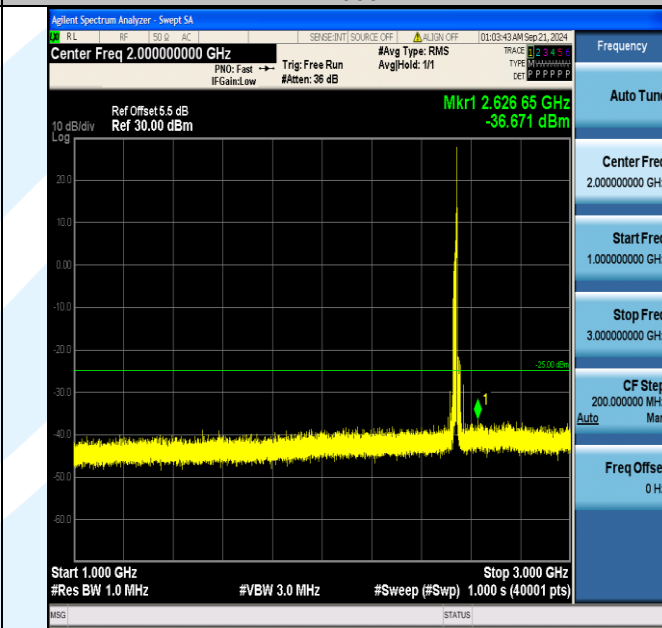
Band7_15MHz_QPSK_21100_1RB#74_1000~3000_1000~3000
