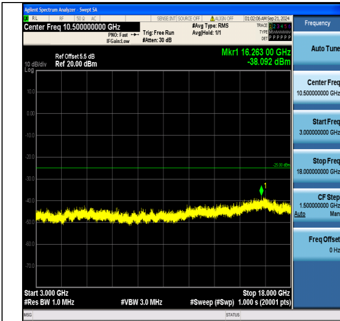
Band7_15MHz_16QAM_20825_75RB#0_3000~18000_3000~18000
