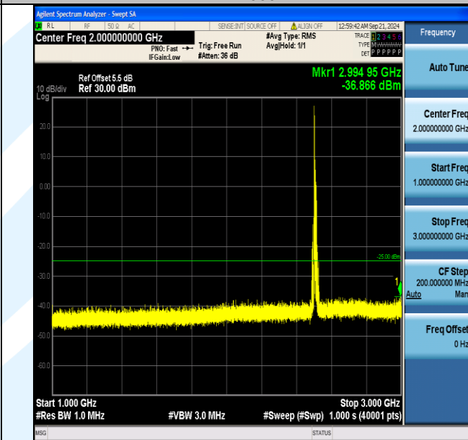
Band7_15MHz_16QAM_20825_1RB#0_1000~3000_1000~3000
