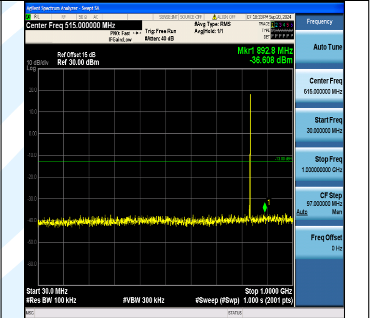
Band5_3MHz_16QAM_20525_1RB#14_30~1000_30~1000
