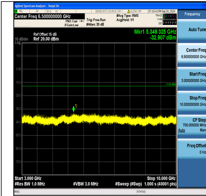
Band5_3MHz_16QAM_20525_15RB#0_3000~10000_3000~10000
