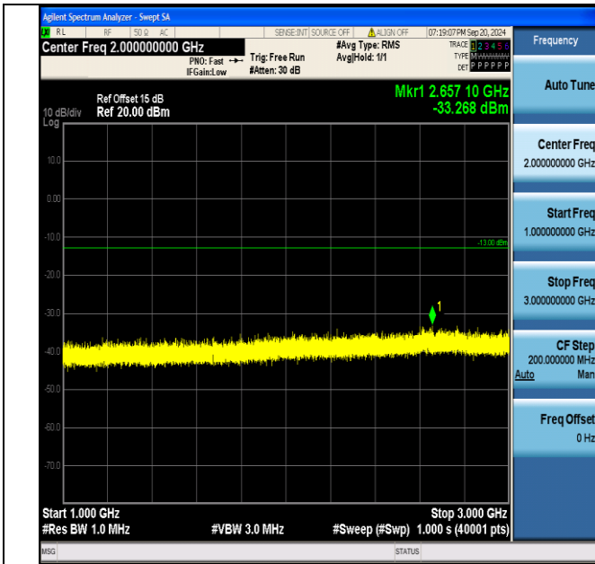
Band5_3MHz_QPSK_20525_15RB#0_1000~3000_1000~3000
