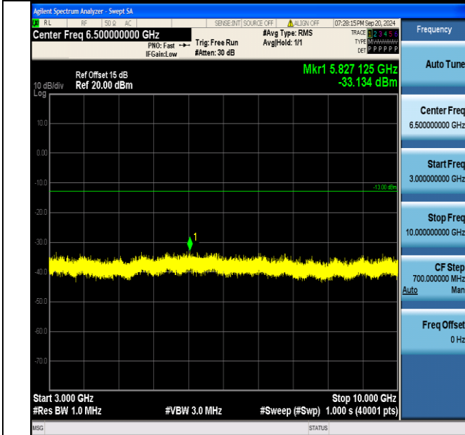
Band5_5MHz_QPSK_20625_1RB#0_3000~10000_3000~1000 0
