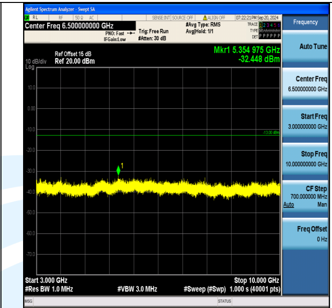
Band5_3MHz_16QAM_20635_15RB#0_3000~10000_3000~10000
