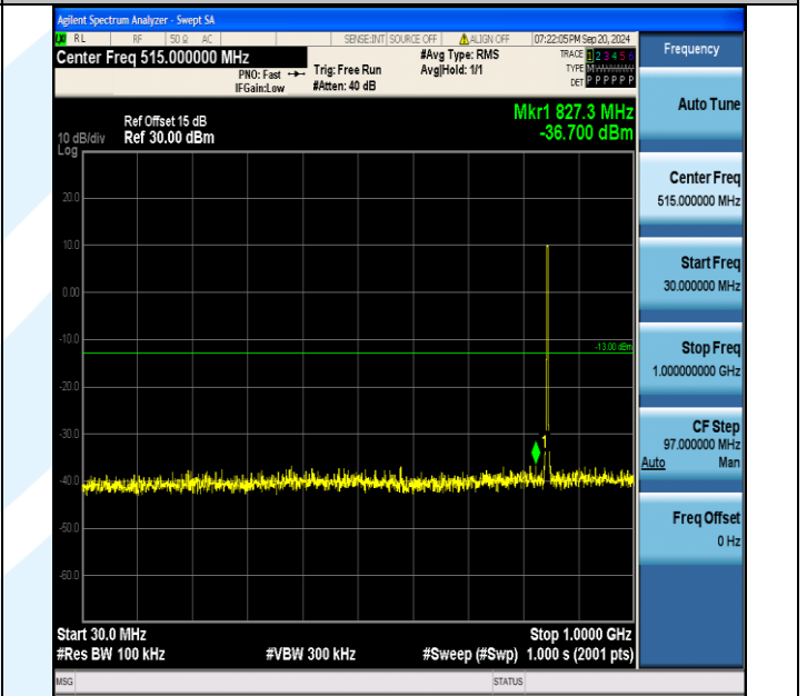
Band5_3MHz_16QAM_20635_15RB#0_30~1000_30~1000
