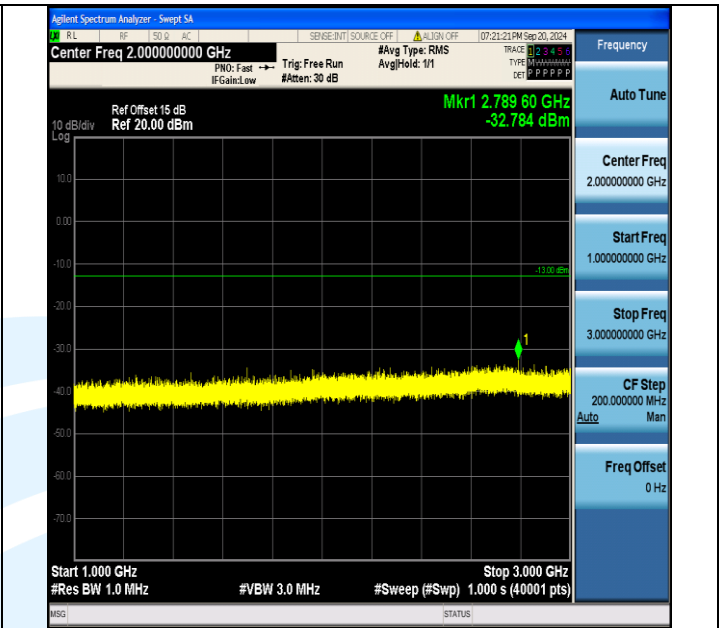
Band5_3MHz_16QAM_20635_1RB#14_1000~3000_1000~3000
