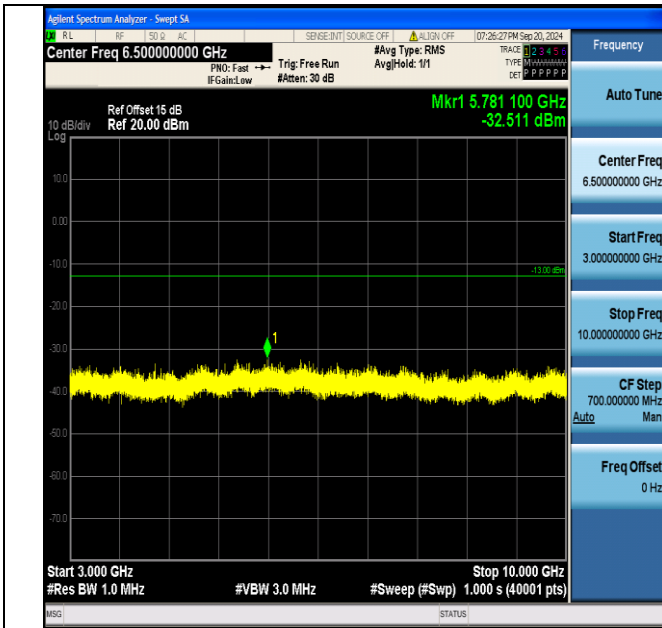
Band5_5MHz_QPSK_20525_1RB#24_3000~10000_3000~10000
