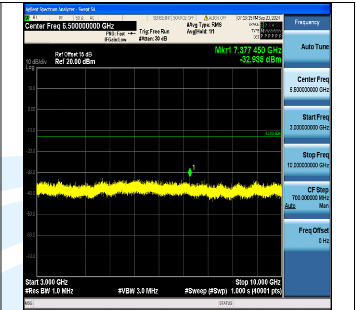
Band5_3MHz_QPSK_20525_15RB#0_3000~10000_3000~10000
