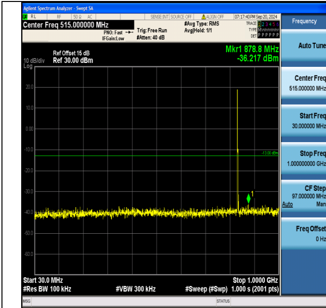
Band5 3MHz 16QAM 20525 1RB#0 30~1000 30~1000
