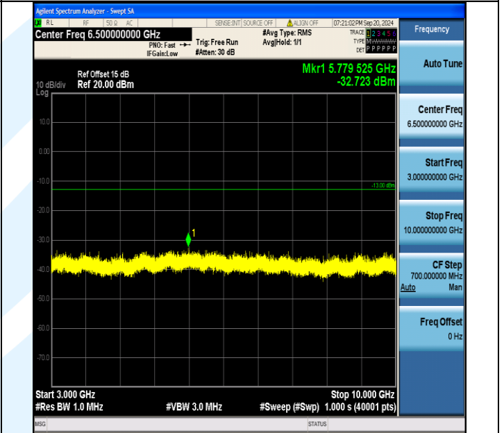
Band5_3MHz_QPSK_20635_1RB#14_3000~10000_3000~1000 00
