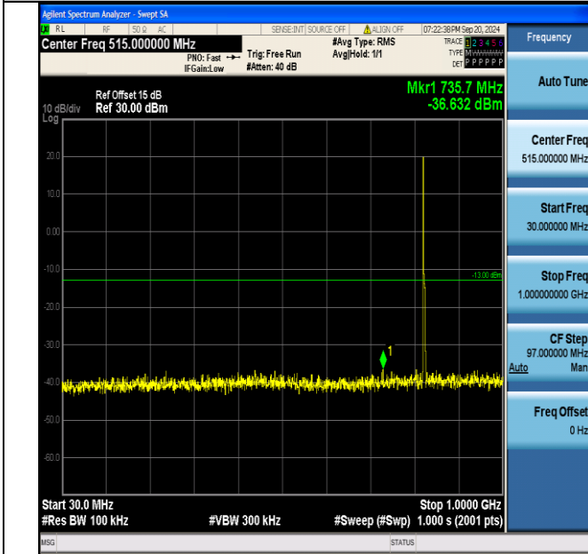
Band5_5MHz_QPSK_20425_1RB#0_30~1000_30~1000
