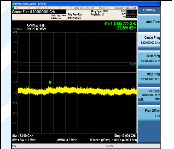
Band5_3MHz_16QAM_20635_1RB#0_3000~10000_3000~10000
