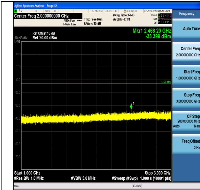
Band5_3MHz_16QAM_20635_15RB#0_1000~3000_1000~3000
