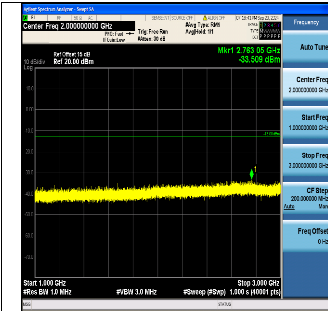
Band5_3MHz_16QAM_20525_1RB#14_1000~3000_1000~3000
