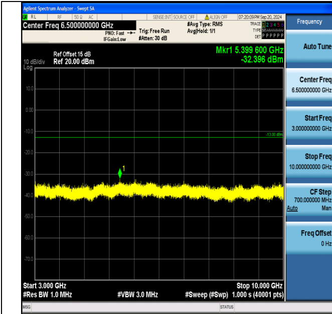
Band5_3MHz_QPSK_20635_1RB#0_3000~10000_3000~1000 0
