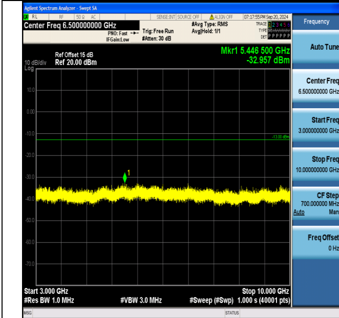
Band5_3MHz_16QAM_20525_1RB#0_3000~10000_3000~1000
