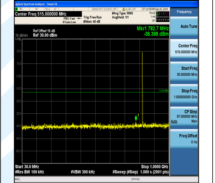
Band5_3MHz_16QAM_20415_1RB#0_30~1000_30~1000
