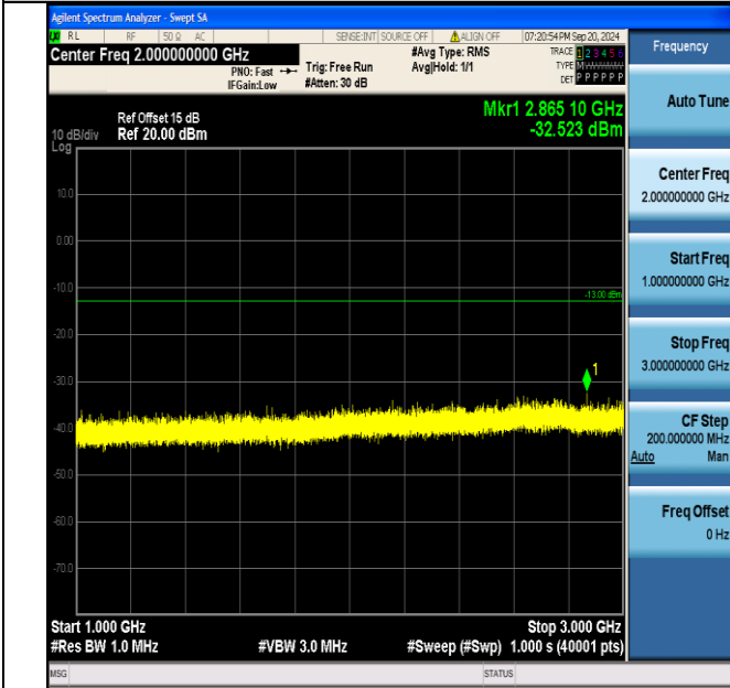
Band5_3MHz_QPSK_20635_1RB#14_1000~3000_1000~3000
