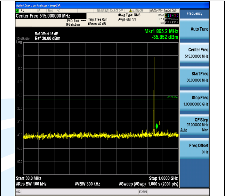
Band5_3MHz_QPSK_20635_1RB#14_30~1000_30~1000
