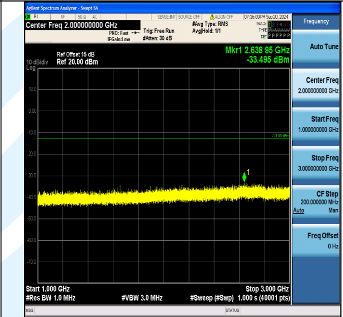
Band5_3MHz_16QAM_20415_1RB#14_1000~3000_1000~3000
