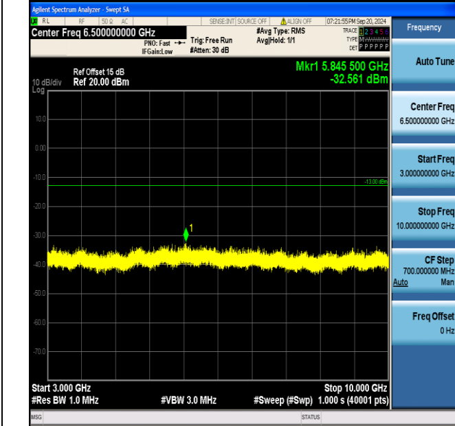
Band5_3MHz_QPSK_20635_15RB#0_3000~10000_3000~1000
