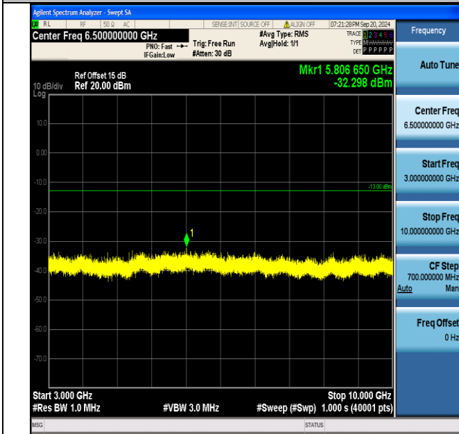
Band5_3MHz_16QAM_20635_1RB#14_3000~10000_3000~10000
