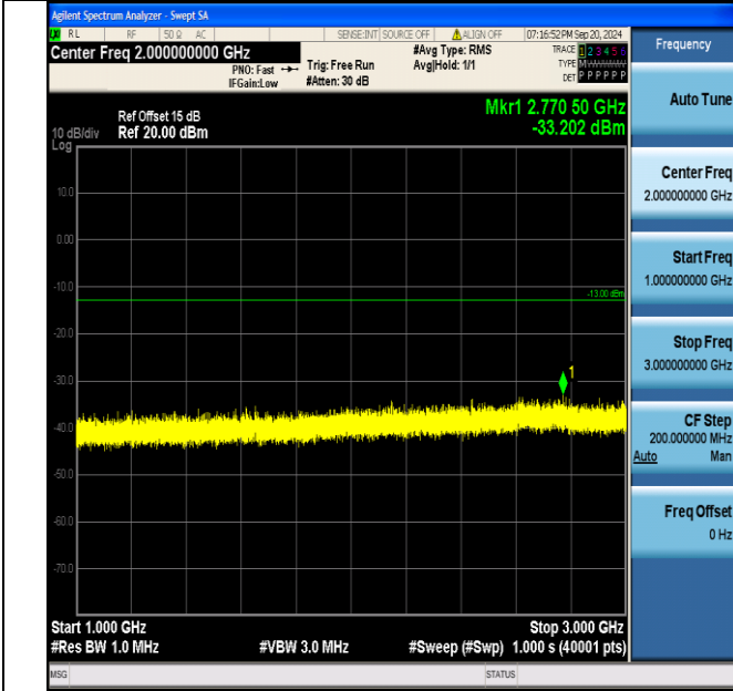
Band5_3MHz_16QAM_20415_15RB#0_1000~3000_1000~3000
