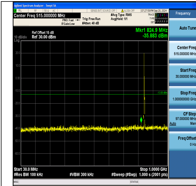
Band5 5MHz QPSK 20625 1RB#0 30~1000 30~1000
