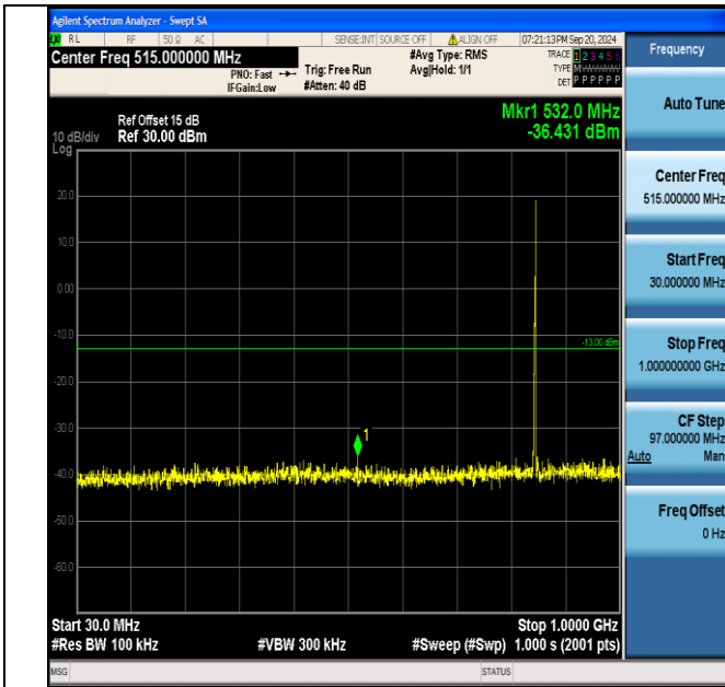
Band5_3MHz_16QAM_20635_1RB#14_30~1000_30~1000
