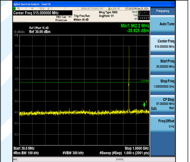
Band5_5MHz_QPSK_20625_1RB#24_30~1000_30~1000
