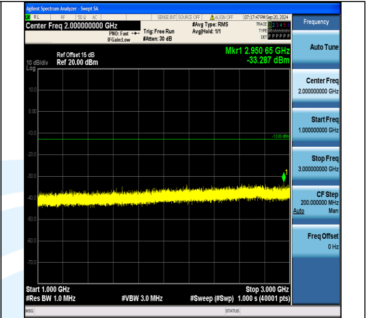
Band5 3MHz 16QAM 20525 1RB#0 1000~3000 1000~3000
