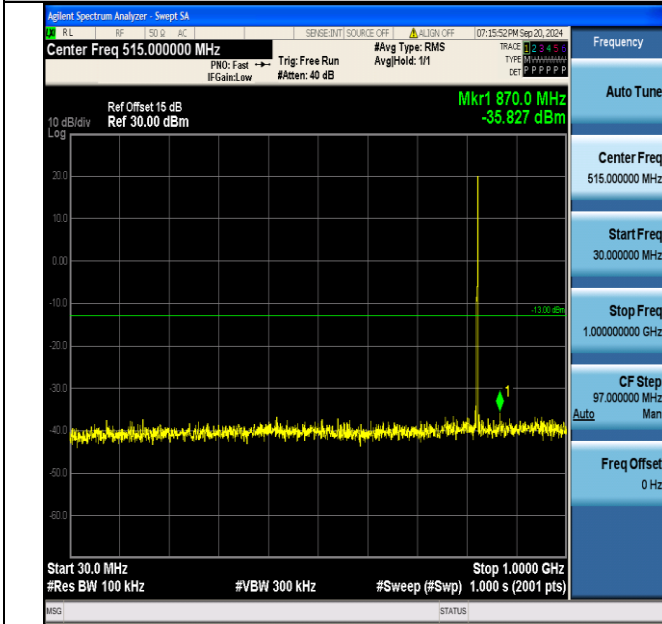
Band5_3MHz_16QAM_20415_1RB#14_30~1000_30~1000
