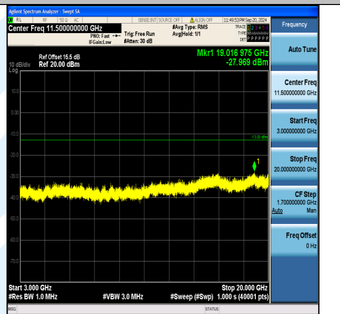
Band4_3MHz_16QAM_19965_15RB#0_3000~20000_3000~20000
