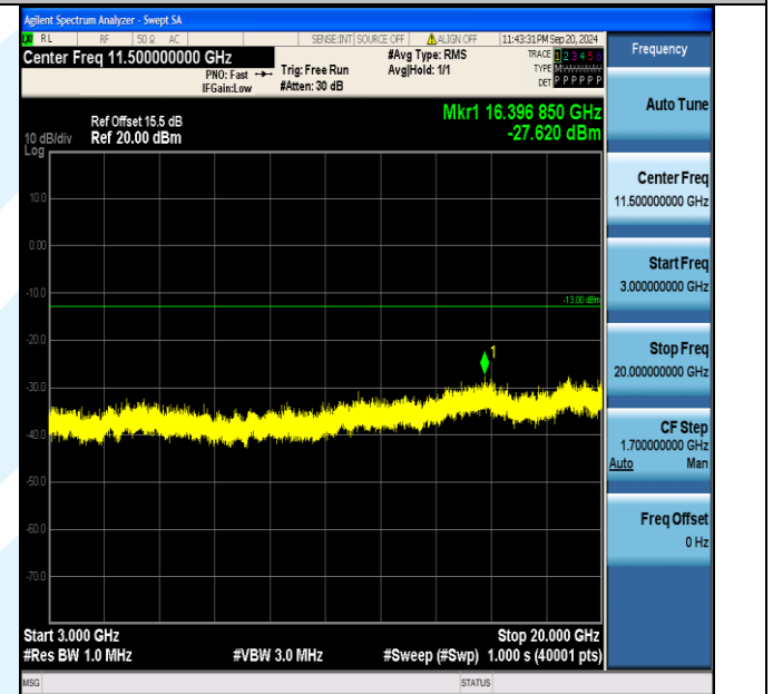
Band4_1.4MHz_16QAM_20175_1RB#5_3000~20000_3000~20000
