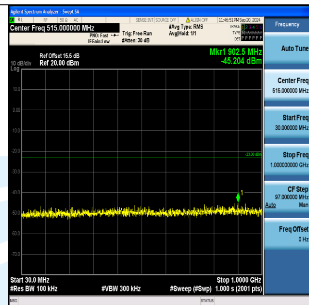
Band4_1.4MHz_16QAM_20393_6RB#0_30~1000_30~1000
