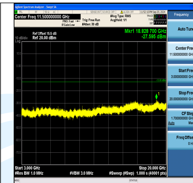
Band4_3MHz_QPSK_20175_15RB#0_3000~20000_3000~20000
