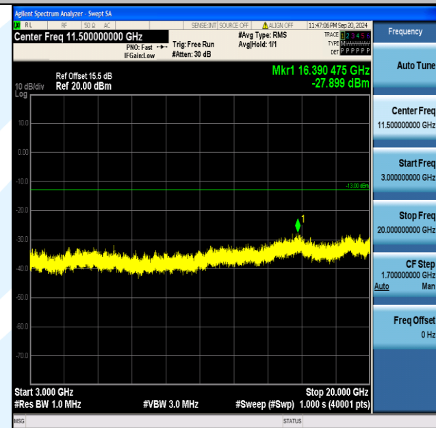
Band4_1.4MHz_16QAM_20393_6RB#0_3000~20000_3000~20000
