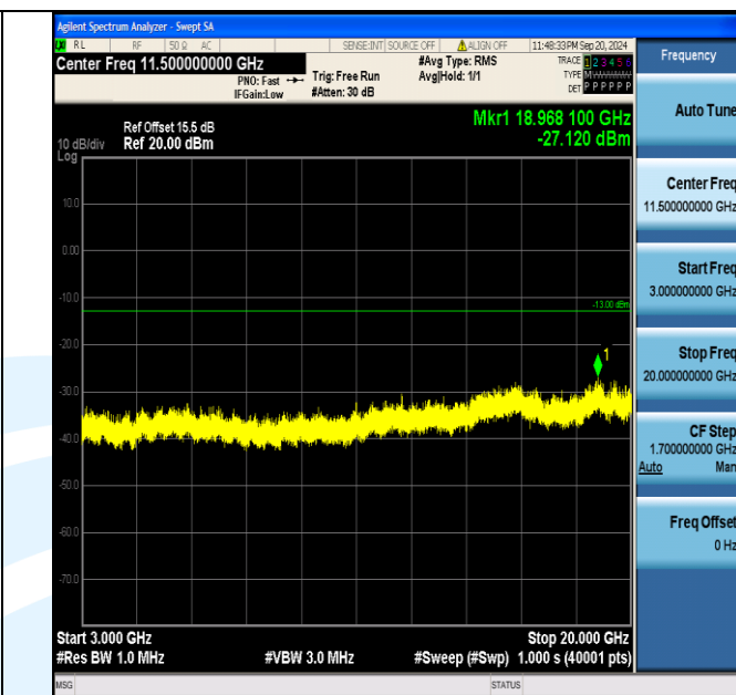
Band4_3MHz_QPSK_19965_1RB#14_3000~20000_3000~20000
