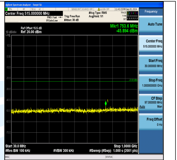
Band4_1.4MHz_16QAM_20175_1RB#5_30~1000_30~1000
