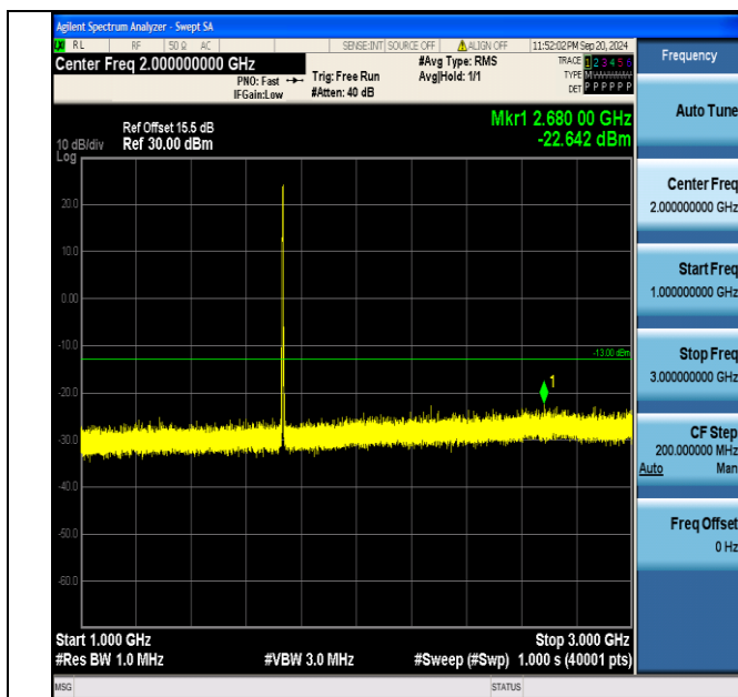
Band4_3MHz_QPSK_20175_15RB#0_1000~3000_1000~3000
