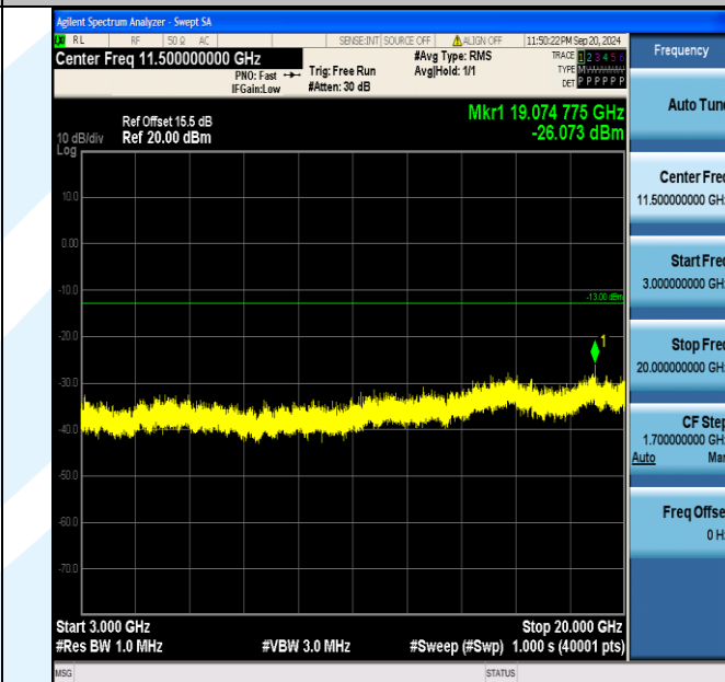
Band4_3MHz_QPSK_20175_1RB#0_3000~20000_3000~20000
