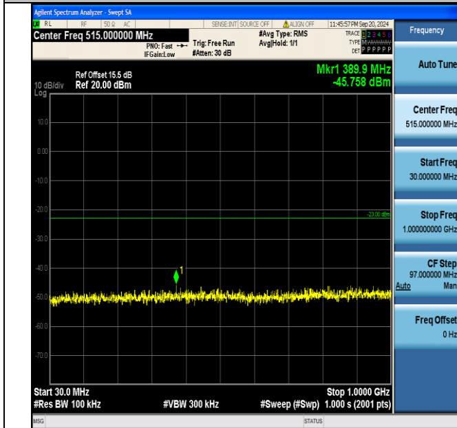
Band4_1.4MHz_16QAM_20393_1RB#5_30~1000_30~1000
