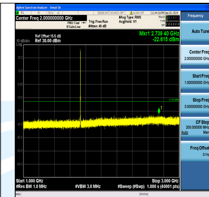
Band4_1.4MHz_16QAM_20175_6RB#0_1000~3000_1000~3000
