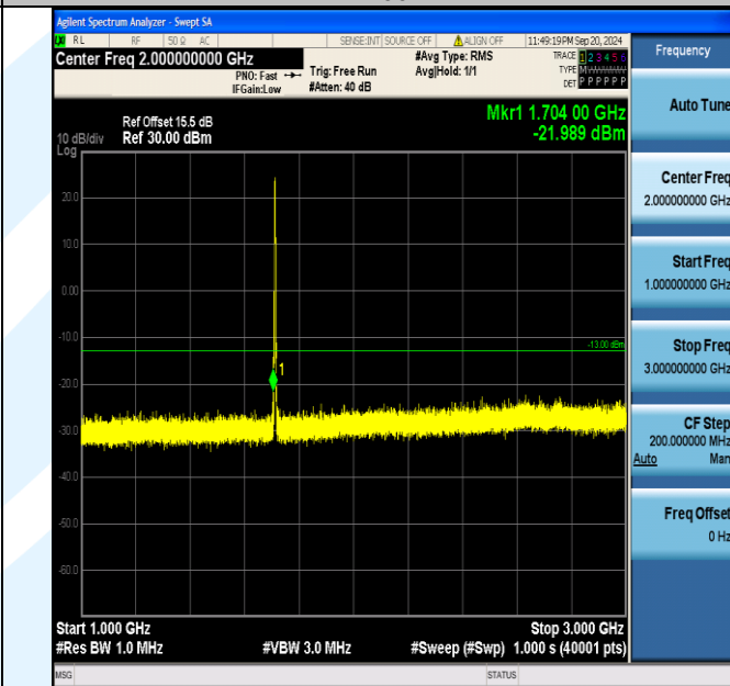
Band4_3MHz_QPSK_19965_15RB#0_1000~3000_1000~3000
