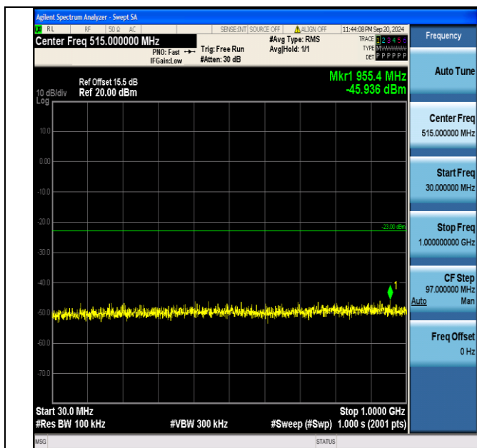
Band4_1.4MHz_16QAM_20175_6RB#0_30~1000_30~1000
