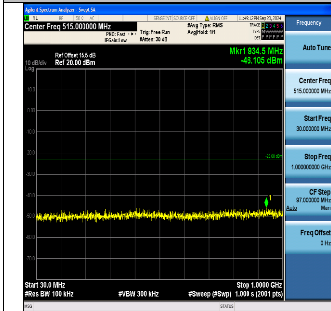
Band4_3MHz_QPSK_19965_15RB#0_30~1000_30~1000
