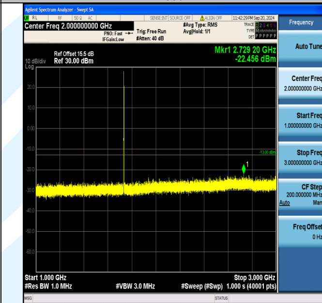
Band4_1.4MHz_16QAM_20175_1RB#0_1000~3000_1000~3000
