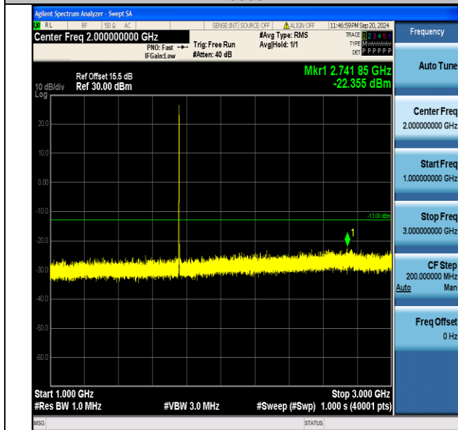
Band4_1.4MHz_16QAM_20393_6RB#0_1000~3000_1000~3000
