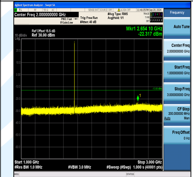
Band4_1.4MHz_16QAM_20393_1RB#5_1000~3000_1000~3000
