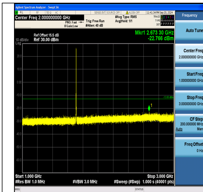
Band4_1.4MHz_16QAM_19957_6RB#0_1000~3000_1000~3000
