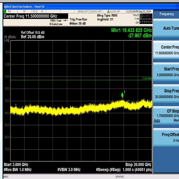
Band4_3MHz_QPSK_20385_1RB#14_3000~20000_3000~20000
