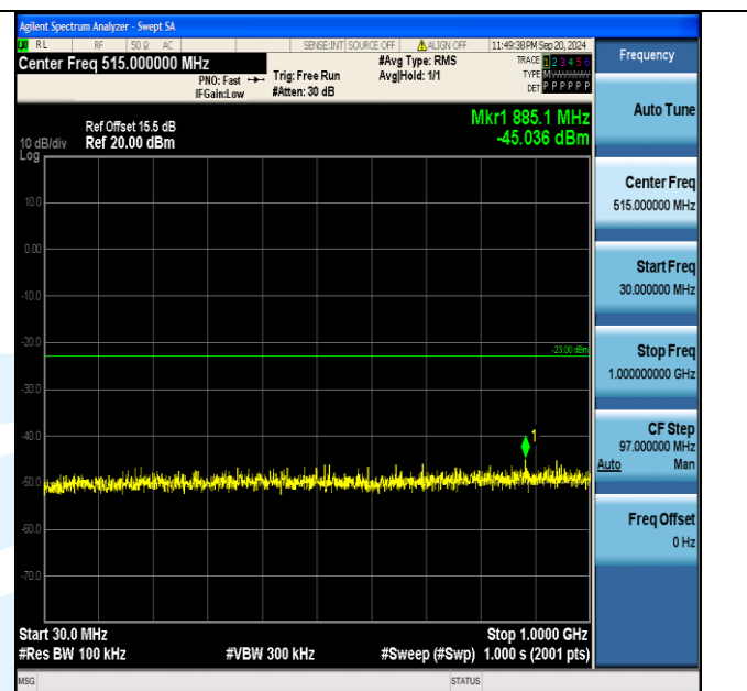
Band4_3MHz_16QAM_19965_15RB#0_30~1000_30~1000
