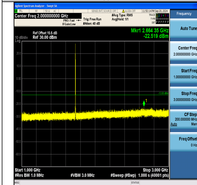
Band4_3MHz_QPSK_20175_1RB#0_1000~3000_1000~3000
