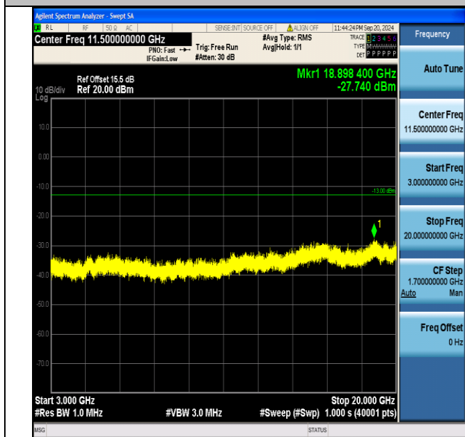
Band4_1.4MHz_16QAM_20175_6RB#0_3000~20000_3000~20000
