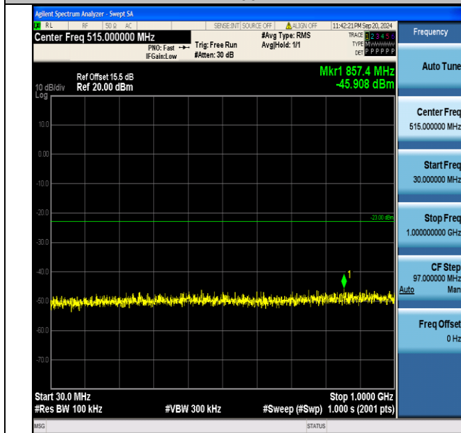
Band4_1.4MHz_16QAM_20175_1RB#0_30~1000_30~1000
