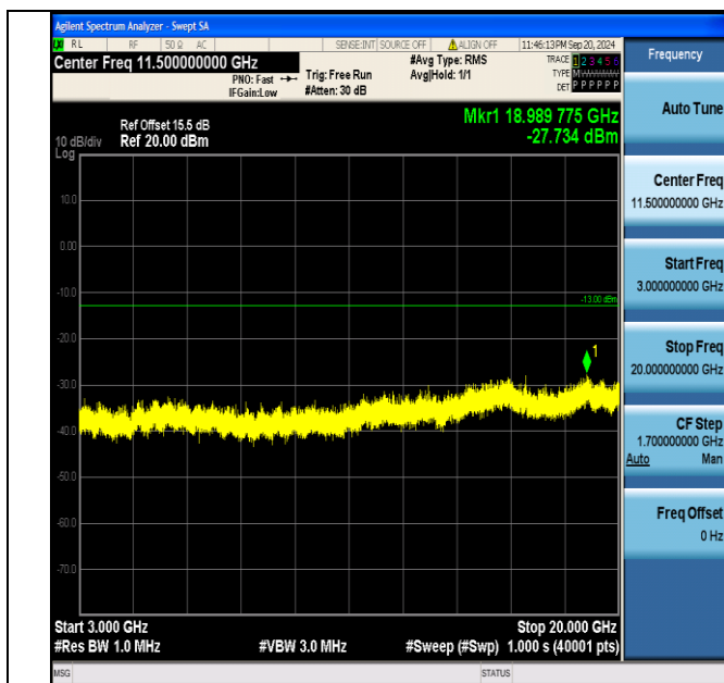
Band4_1.4MHz_16QAM_20393_1RB#5_3000~20000_3000~20000
