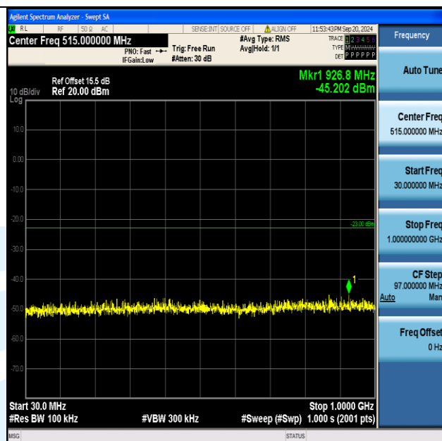
Band4_3MHz_QPSK_20385_1RB#14_30~1000_30~1000
