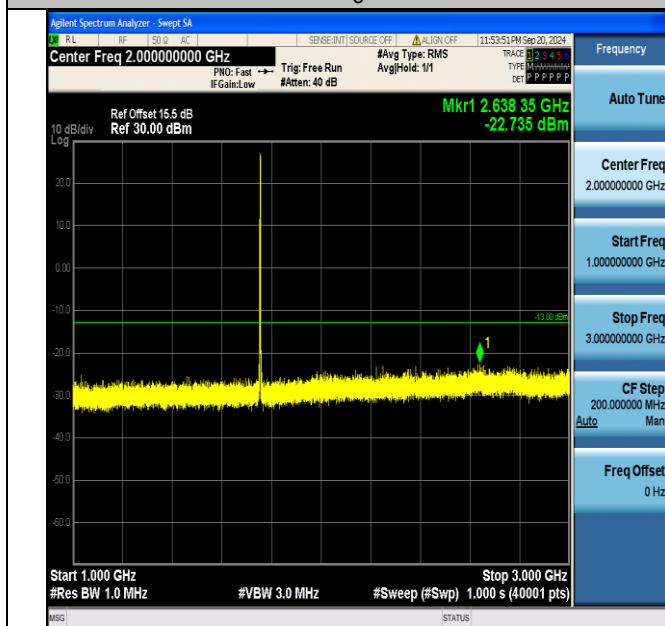
Band4_3MHz_QPSK_20385_1RB#14_1000~3000_1000~3000
