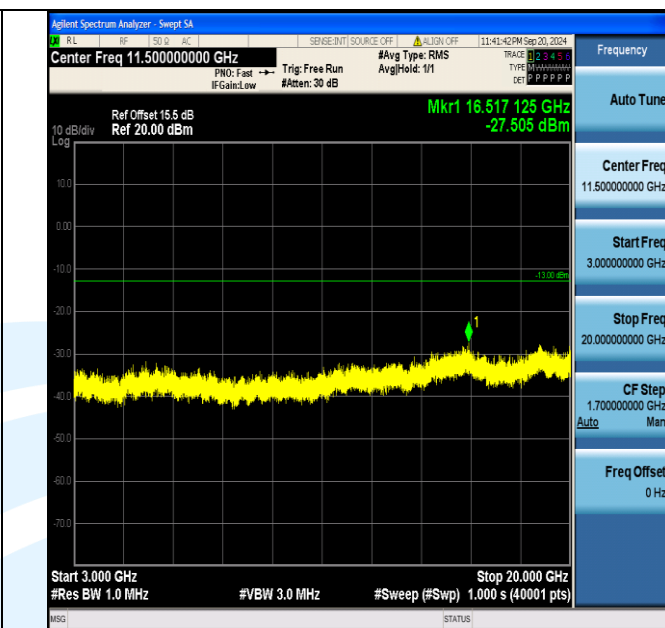
Band4_1.4MHz_16QAM_19957_6RB#0_3000~20000_3000~20000
