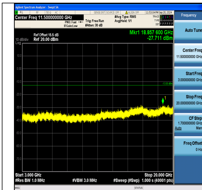
Band4_3MHz_QPSK_20385_1RB#0_3000~20000_3000~20000
