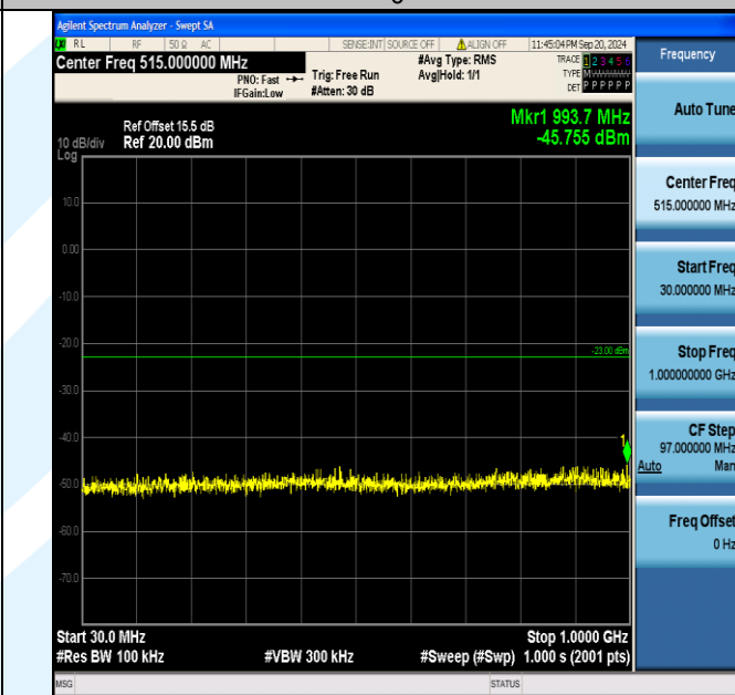
Band4_1.4MHz_16QAM_20393_1RB#0_30~1000_30~1000
