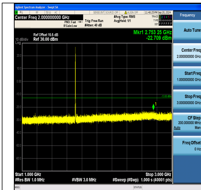
Band4_3MHz_QPSK_19965_1RB#14_1000~3000_1000~3000
