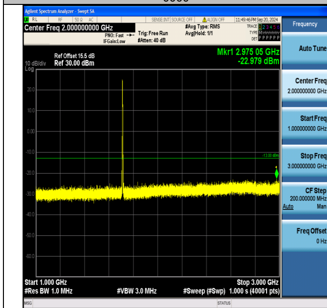
Band4_3MHz_16QAM_19965_15RB#0_1000~3000_1000~3000
