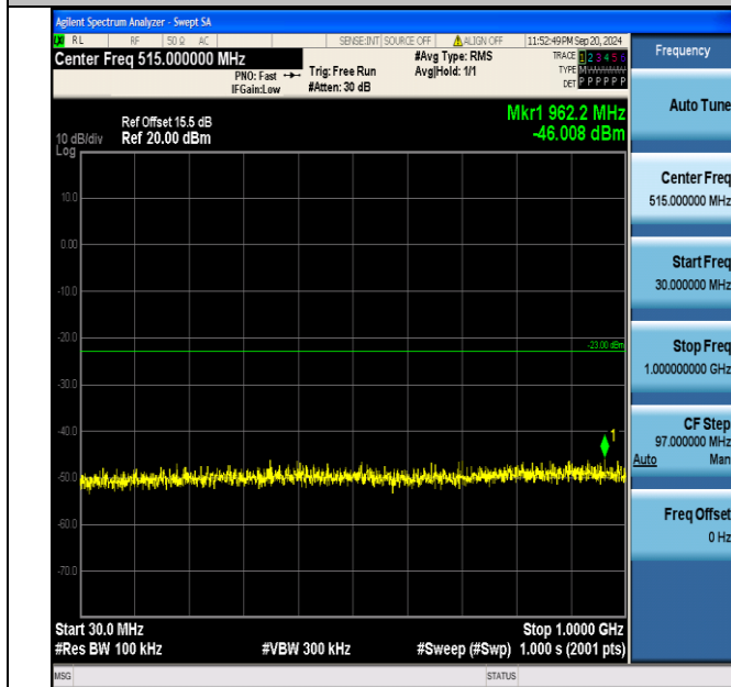
Band4_3MHz_QPSK_20385_1RB#0_30~1000_30~1000
