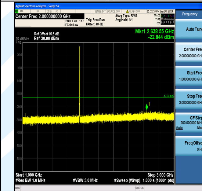
Band4_3MHz_QPSK_20385_1RB#0_1000~3000_1000~3000
