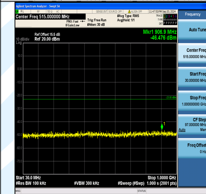
Band4_3MHz_16QAM_19965_1RB#0_30~1000_30~1000
