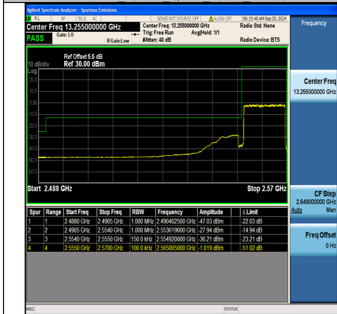
Band41 15MHz QPSK 40315 75RB#0
