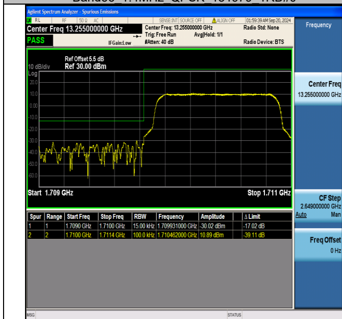
Band66 1.4MHz QPSK 131979 6RB#0
