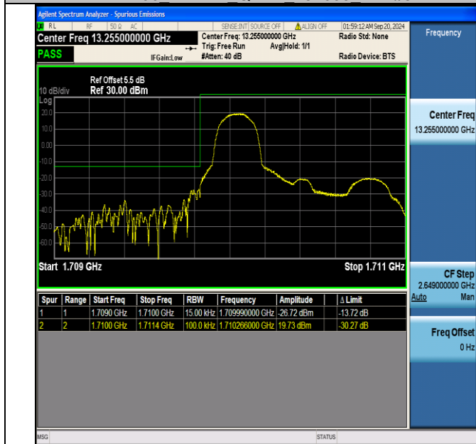
Band66 1.4MHz 16QAM 131979 1RB#0
