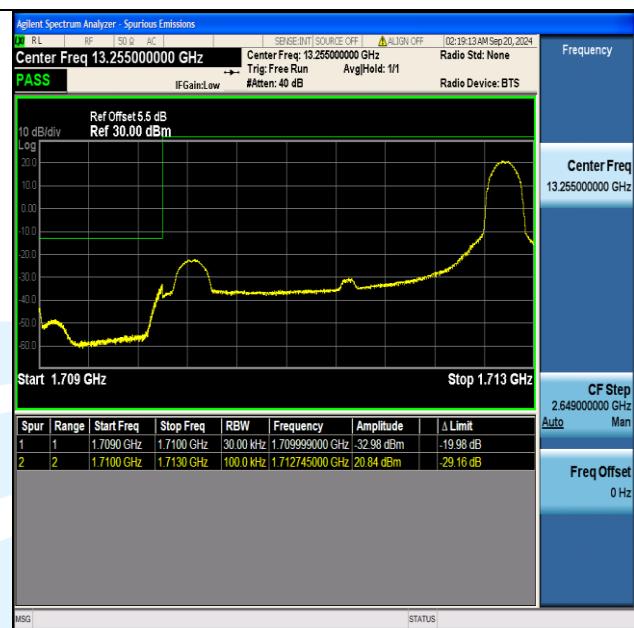
Band66 3MHz QPSK 131987 1RB#14
