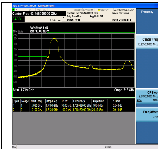
Band66 3MHz QPSK 131987 1RB#0
