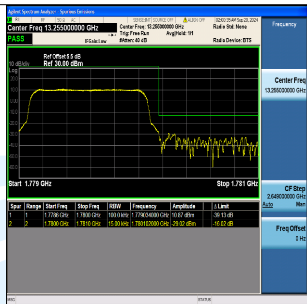
Band66 1.4MHz QPSK 132665 6RB#0
