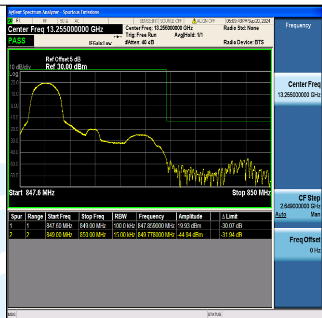
Band5 1.4MHz 16QAM 20643 1RB#0
