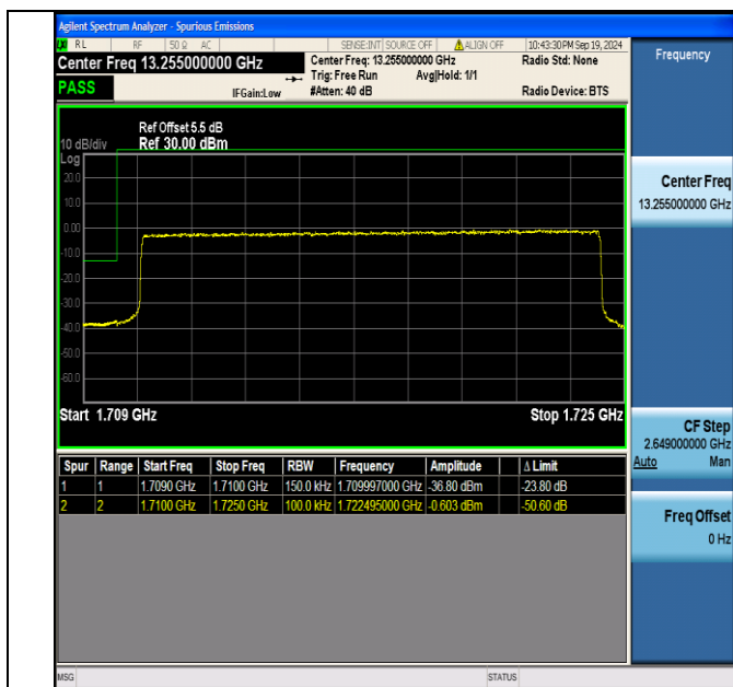
Band4 15MHz 16QAM 20025 75RB#0
