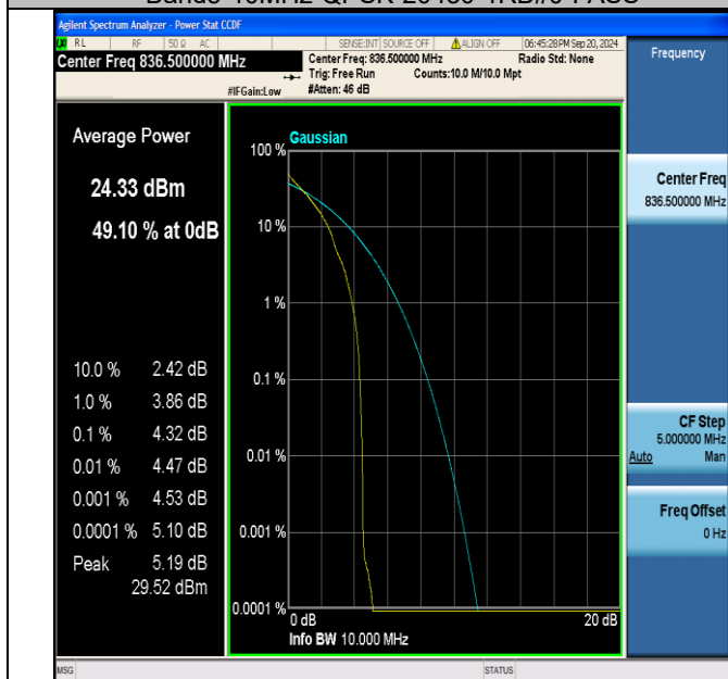
Band5-10MHz-QPSK-20525-1RB#0-PASS
