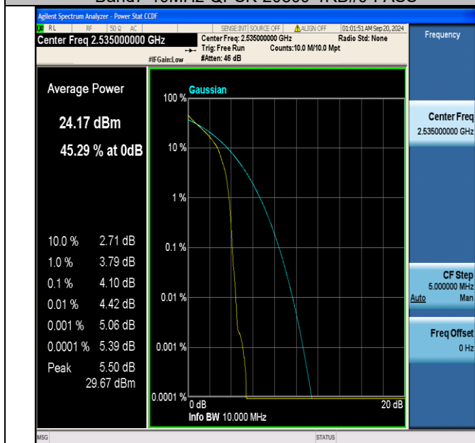
Band7-10MHz-QPSK-21100-1RB#0-PASS
