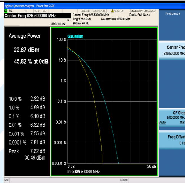
Band5-5MHz-16QAM-20425-25RB#0-PASS
