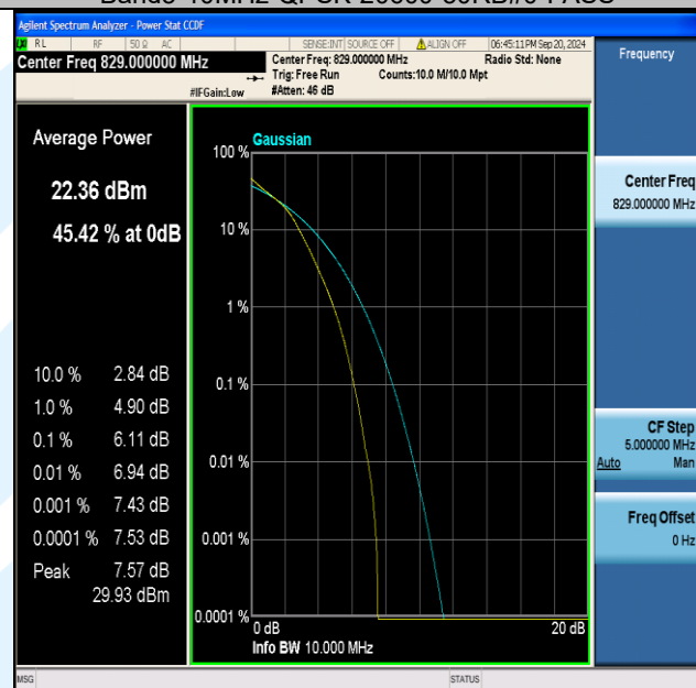
Band5-10MHz-16QAM-20450-50RB#0-PASS
