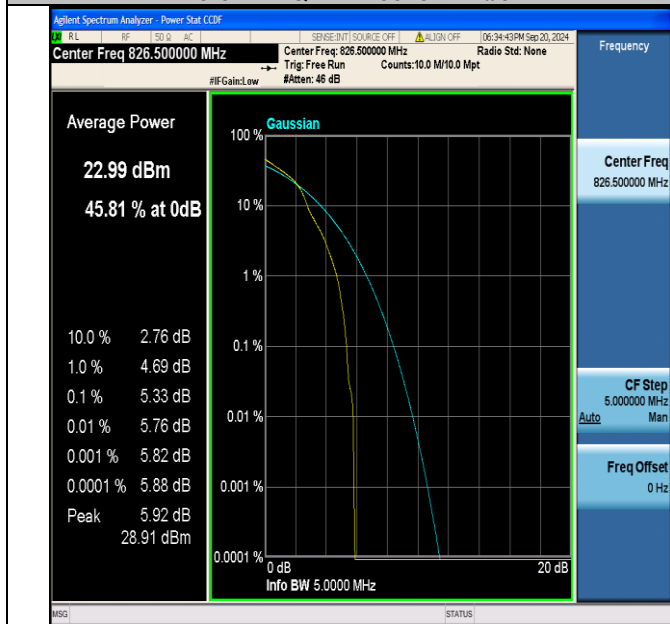
Band5-5MHz-16QAM-20425-1RB#0-PASS
