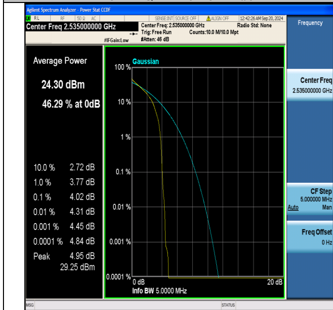
Band7-5MHz-QPSK-21100-1RB#0-PASS
