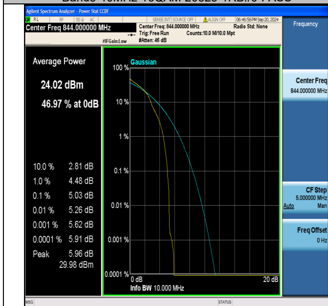
Band5-10MHz-16QAM-20600-1RB#0-PASS
