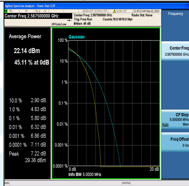
Band7-5MHz-16QAM-21425-25RB#0-PASS
