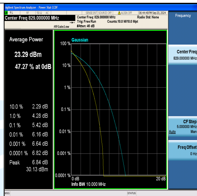
Band5-10MHz-QPSK-20450-50RB#0-PASS
