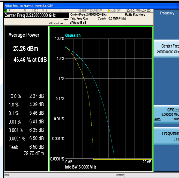
Band7-5MHz-QPSK-21100-25RB#0-PASS
