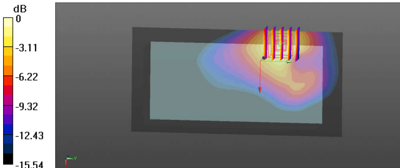
0 dB = 1.40 W/kg
