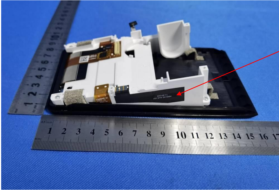
LTE Diversity antenna
