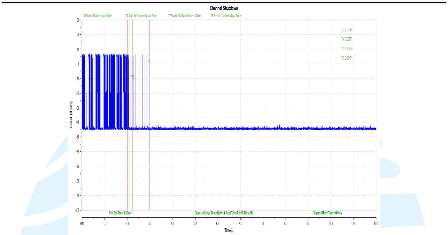
11AC20SISO-5300-Type0-PASS
