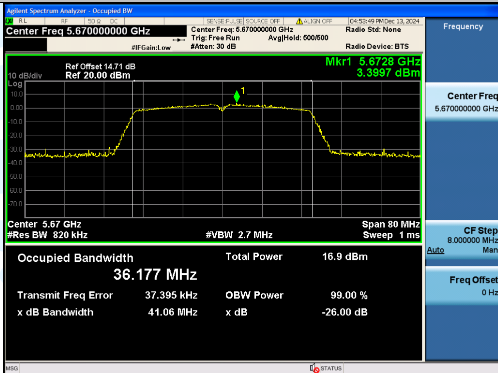
11AC40SISO-Ant1-5670
