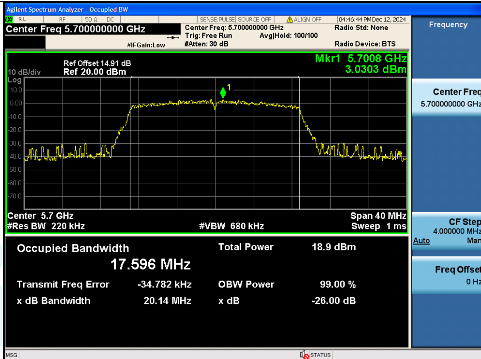
11N20SISO-Ant1-5700
