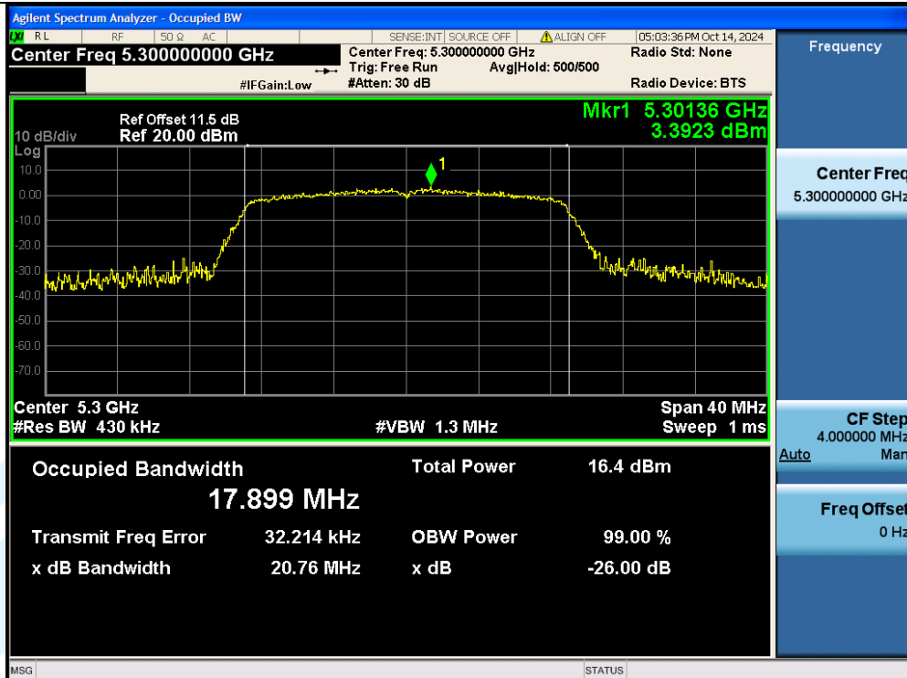
11AC20SISO-Ant1-5300
