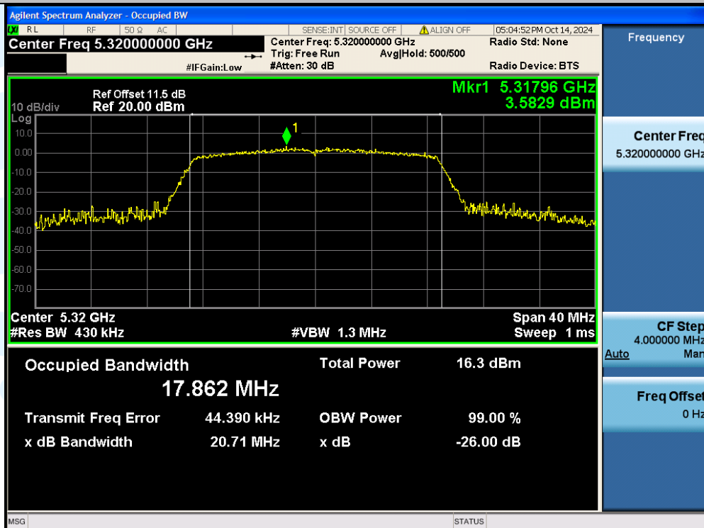
11AC20SISO-Ant1-5320
