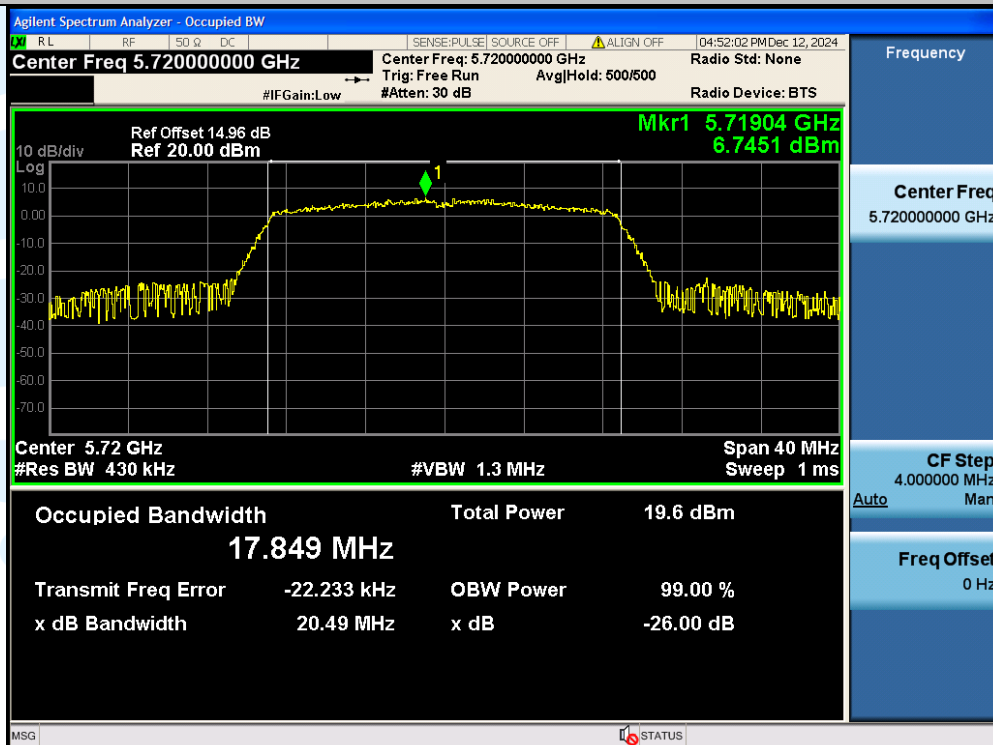
11N20SISO-Ant1-5720
