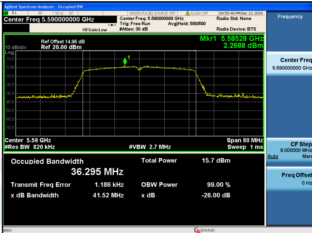
11AC40SISO-Ant1-5590
