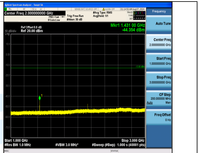
Band17_10MHz_16QAM_23800_1RB#49_1000~3000_1000~3000
