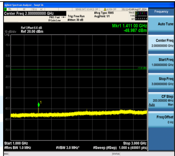
Band17_10MHz_16QAM_23790_1RB#0_1000~3000_1000~3000
