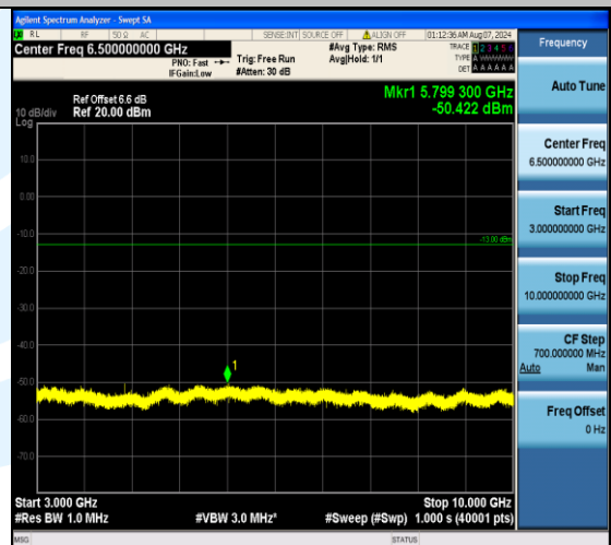
Band17_10MHz_16QAM_23790_1RB#49_3000~10000_3000~10000
