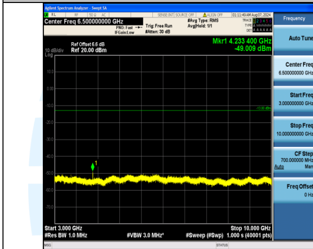
Band17_10MHz_16QAM_23790_1RB#0_3000~10000_3000~10000
