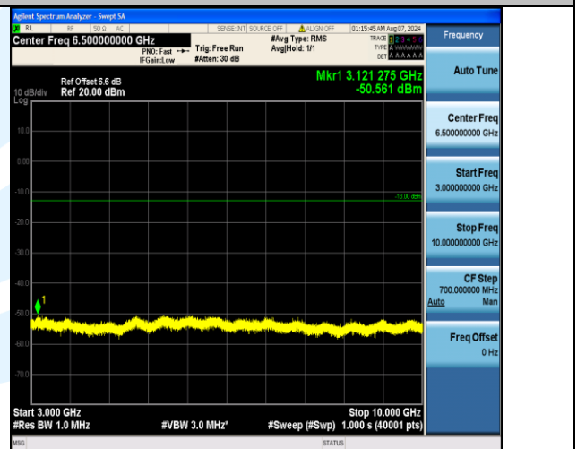
Band17_10MHz_16QAM_23800_50RB#0_3000~10000_3000~10000
