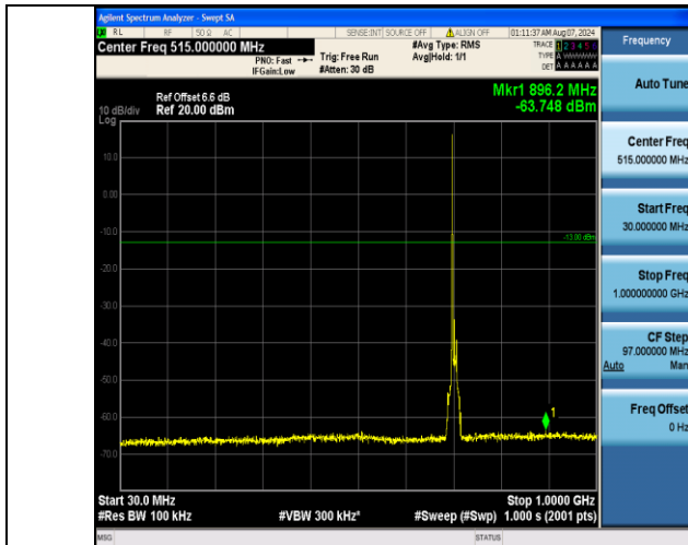
Band17_10MHz_16QAM_23790_1RB#0_30~1000_30~1000
