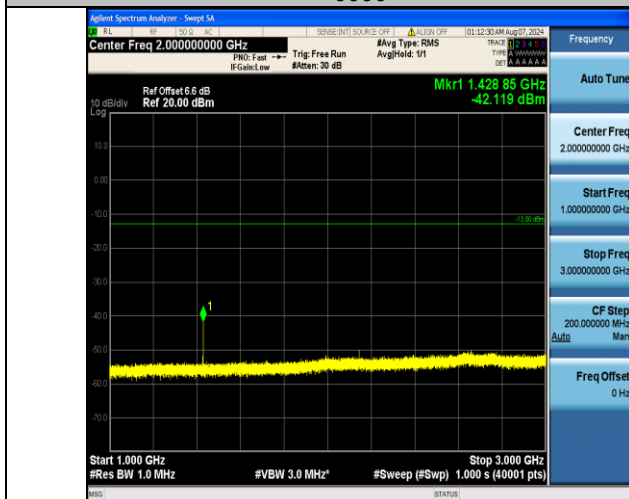
Band17_10MHz_16QAM_23790_1RB#49_1000~3000_1000~3000
