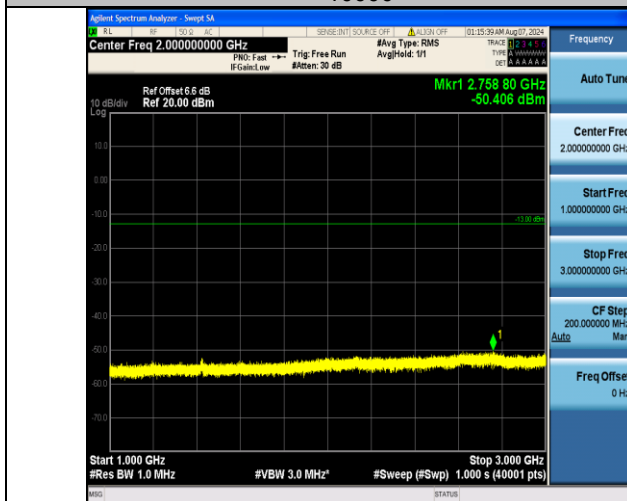
Band17_10MHz_16QAM_23800_50RB#0_1000~3000_1000~3000
