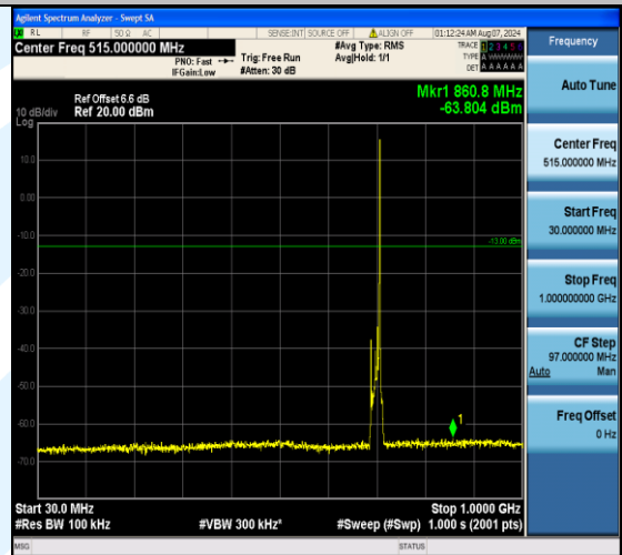
Band17_10MHz_16QAM_23790_1RB#49_30~1000_30~1000
