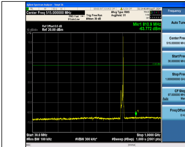
Band17_10MHz_16QAM_23800_1RB#49_30~1000_30~1000
