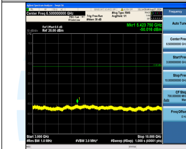
Band17_10MHz_16QAM_23800_1RB#49_3000~10000_3000~10000
