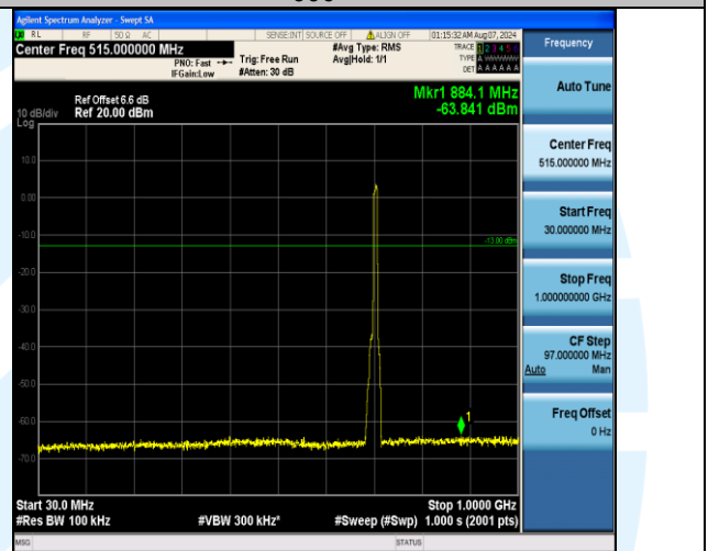
Band17_10MHz_16QAM_23800_50RB#0_30~1000_30~1000
