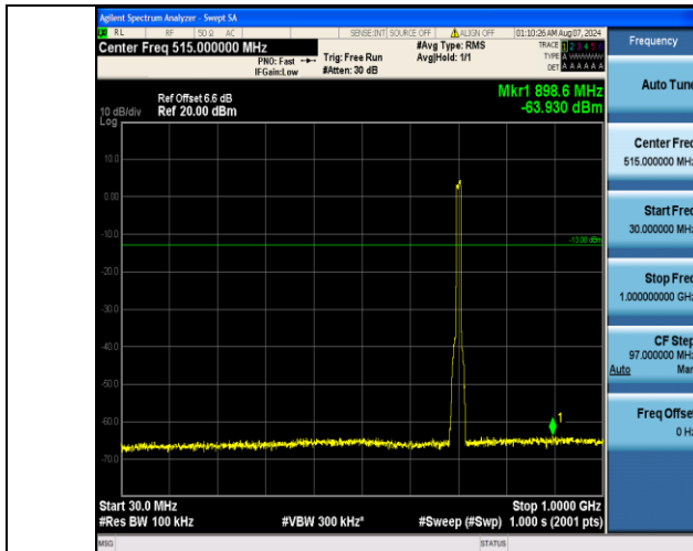
Band17_10MHz_QPSK_23780_50RB#0_30~1000_30~1000
