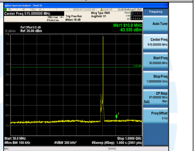
Band17_10MHz_QPSK_23780_1RB#49_30~1000_30~1000
