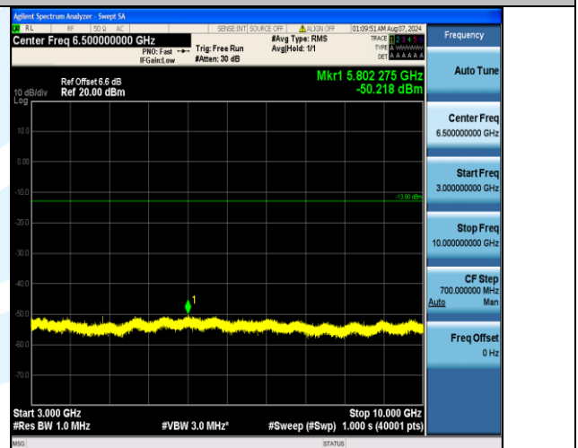
Band17_10MHz_QPSK_23780_1RB#49_3000~10000_3000~10000
