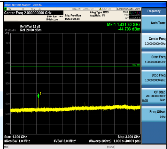
Band17_5MHz_16QAM_23825_1RB#24_1000~3000_1000~3000
