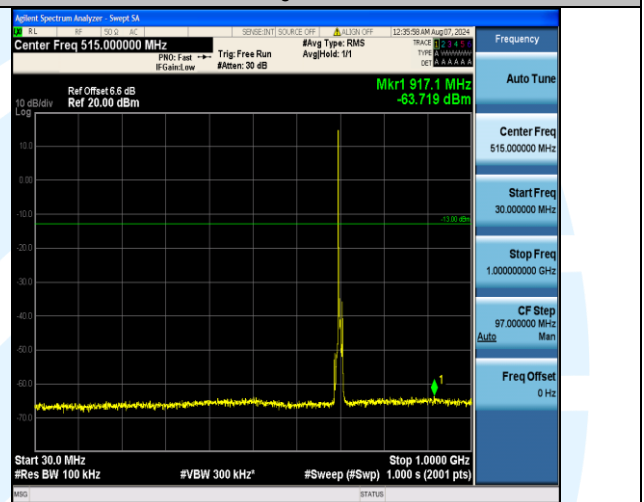
Band17_5MHz_16QAM_23755_1RB#0_30~1000_30~1000
