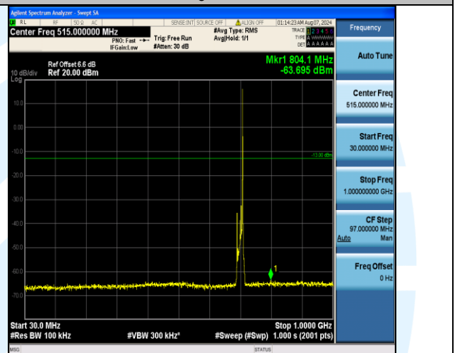
Band17_10MHz_QPSK_23800_1RB#49_30~1000_30~1000
