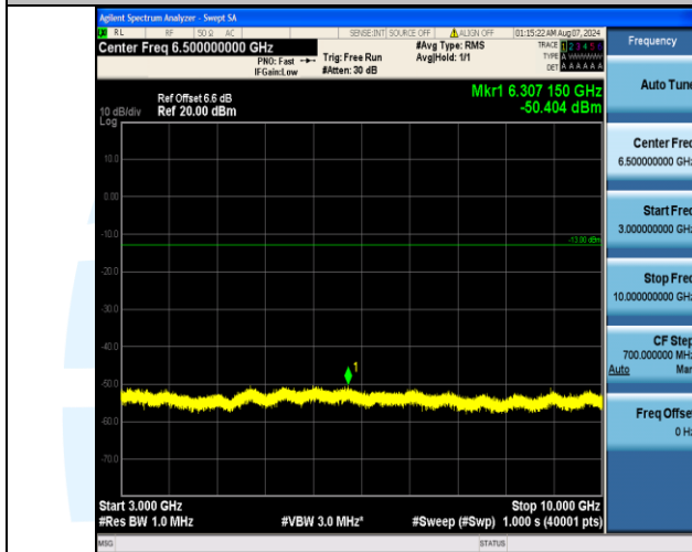
Band17_10MHz_QPSK_23800_50RB#0_3000~10000_3000~10000
