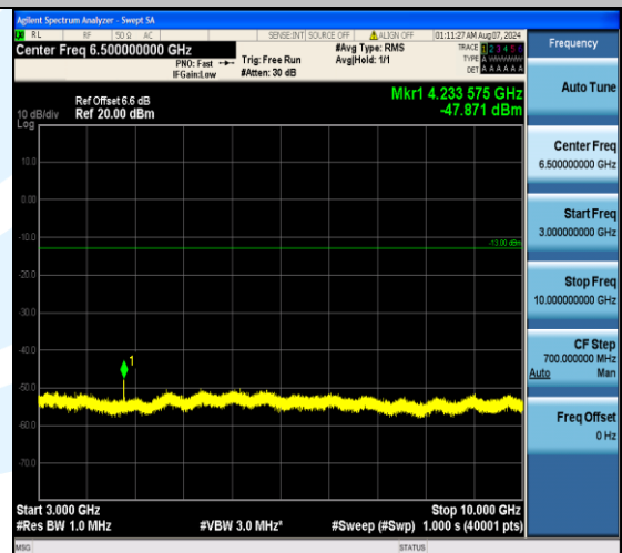
Band17_10MHz_QPSK_23790_1RB#0_3000~10000_3000~10000
