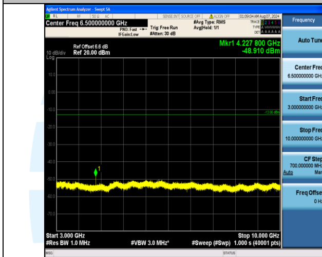
Band17_10MHz_QPSK_23780_1RB#0_3000~10000_3000~10000
