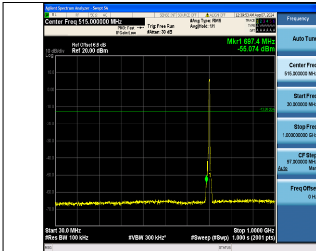
Band17_5MHz_16QAM_23790_25RB#0_30~1000_30~1000
