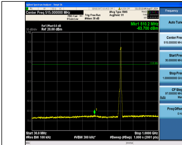
Band17_10MHz_QPSK_23800_50RB#0_30~1000_30~1000
