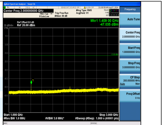
Band17_10MHz_QPSK_23780_1RB#0_1000~3000_1000~3000
