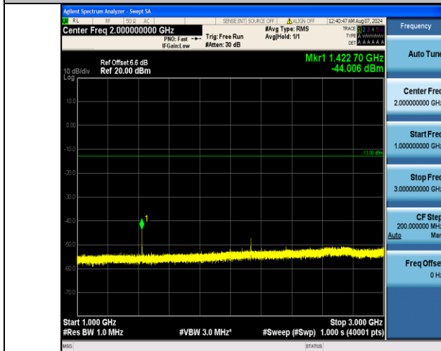
Band17_5MHz_16QAM_23825_1RB#0_1000~3000_1000~3000
