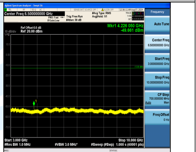
Band17_5MHz_16QAM_23755_1RB#0_3000~10000_3000~10000
