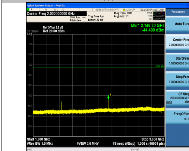
Band17_10MHz_QPSK_23800_1RB#49_1000~3000_1000~3000
