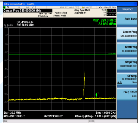
Band17_5MHz_16QAM_23825_1RB#0_30~1000_30~1000
