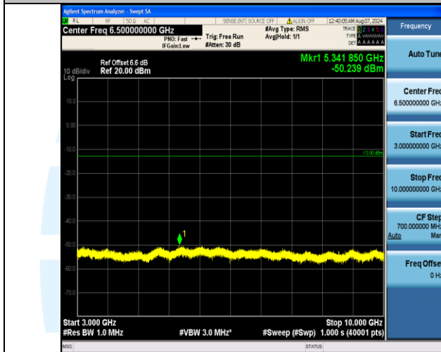
Band17_5MHz_16QAM_23790_25RB#0_3000~10000_3000~10000
