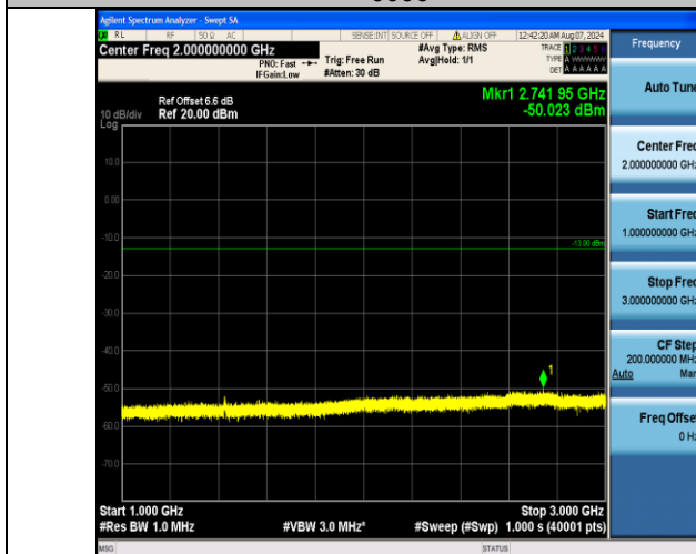
Band17_5MHz_16QAM_23825_25RB#0_1000~3000_1000~3000
