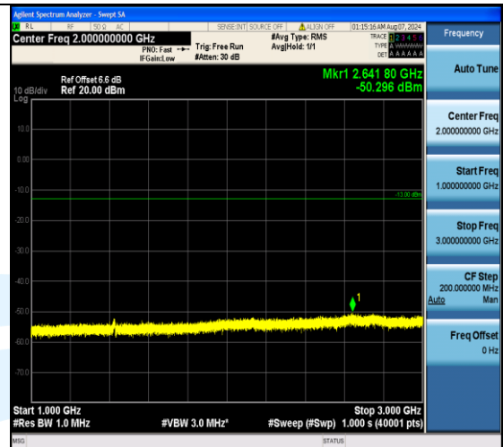
Band17_10MHz_QPSK_23800_50RB#0_1000~3000_1000~3000
