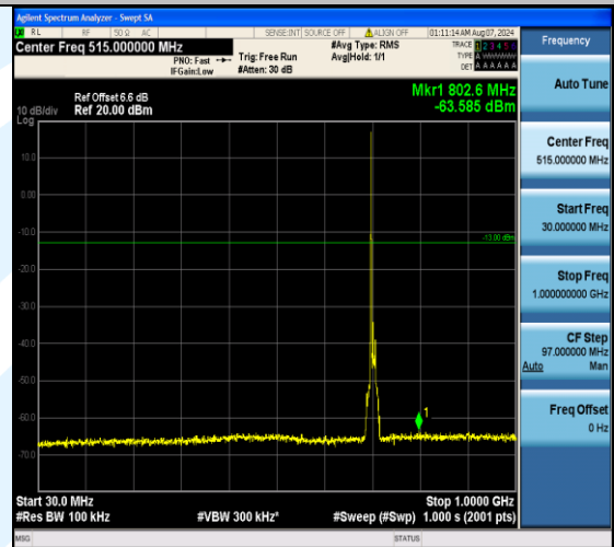
Band17_10MHz_QPSK_23790_1RB#0_30~1000_30~1000
