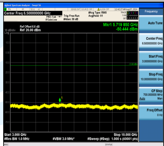
Band17_5MHz_16QAM_23825_25RB#0_3000~10000_3000~10000
