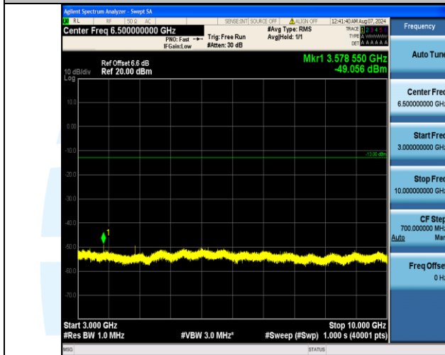
Band17_5MHz_16QAM_23825_1RB#24_3000~10000_3000~10000
