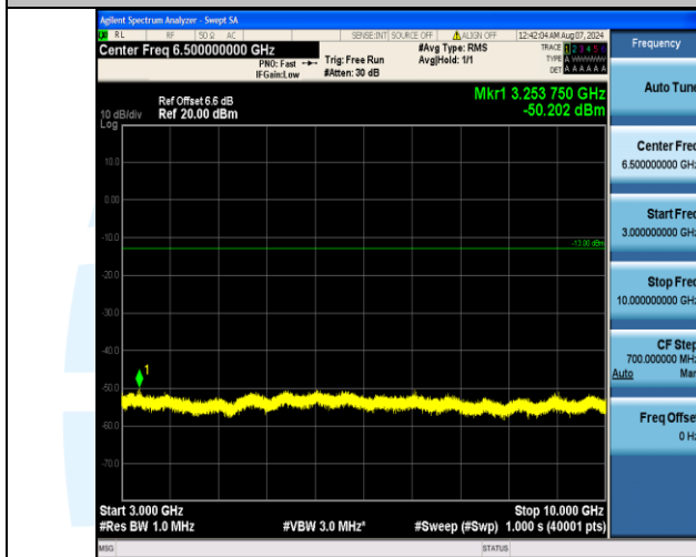
Band17_5MHz_QPSK_23825_25RB#0_3000~10000_3000~10000
