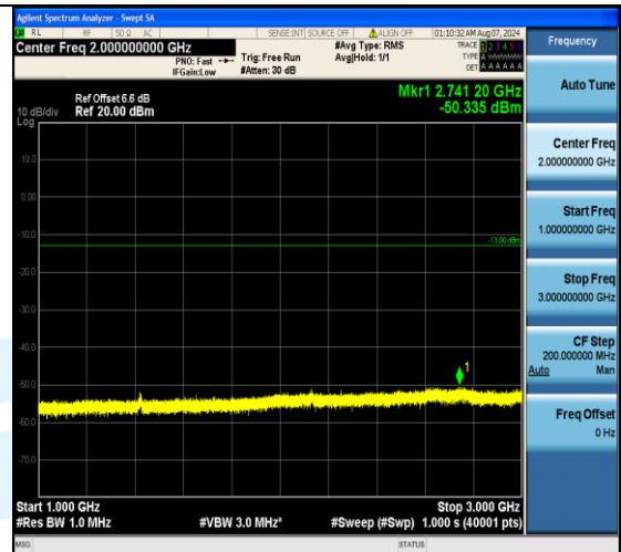
Band17_10MHz_QPSK_23780_50RB#0_1000~3000_1000~3000
