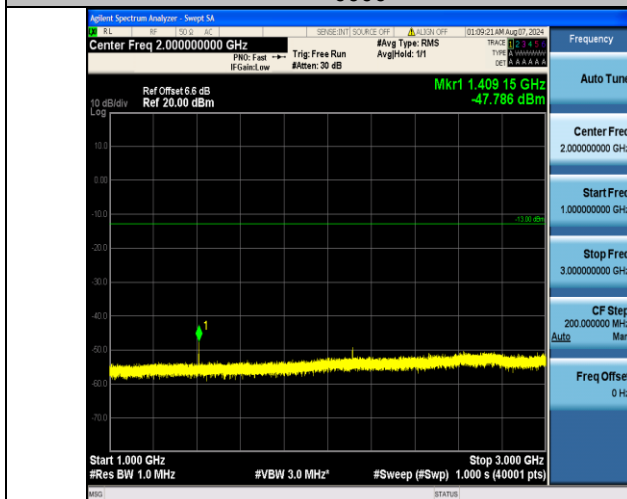
Band17_10MHz_16QAM_23780_1RB#0_1000~3000_1000~3000
