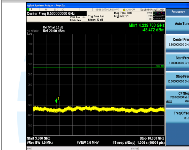
Band17_10MHz_QPSK_23800_1RB#0_3000~10000_3000~10000
