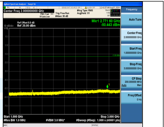
Band17_5MHz_QPSK_23825_25RB#0_1000~3000_1000~3000
