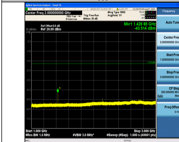
Band17_10MHz_QPSK_23780_1RB#49_1000~3000_1000~3000
