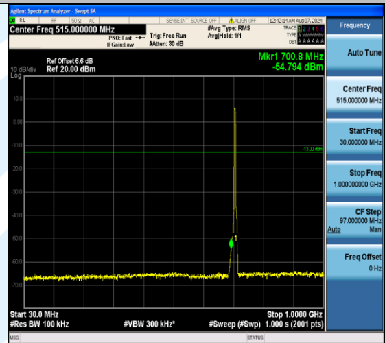
Band17_5MHz_16QAM_23825_25RB#0_30~1000_30~1000
