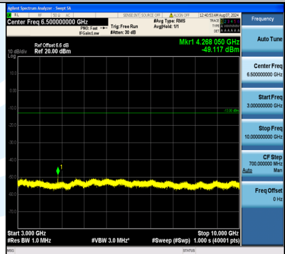
Band17_5MHz_16QAM_23825_1RB#0_3000~10000_3000~10000
