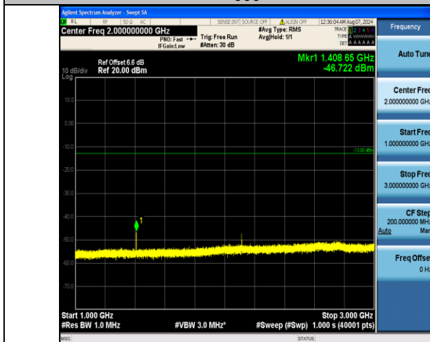
Band17_5MHz_16QAM_23755_1RB#0_1000~3000_1000~3000
