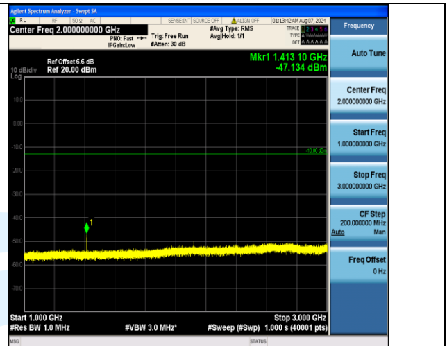
Band17_10MHz_QPSK_23800_1RB#0_1000~3000_1000~3000
