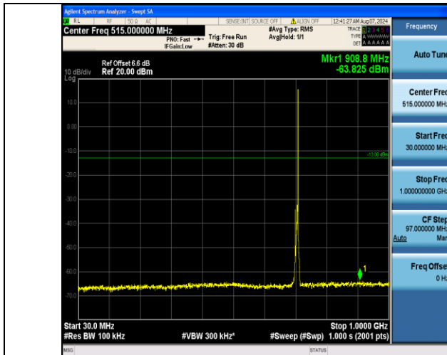
Band17_5MHz_16QAM_23825_1RB#24_30~1000_30~1000
