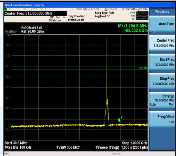
Band17_10MHz_16QAM_23780_1RB#0_30~1000_30~1000
