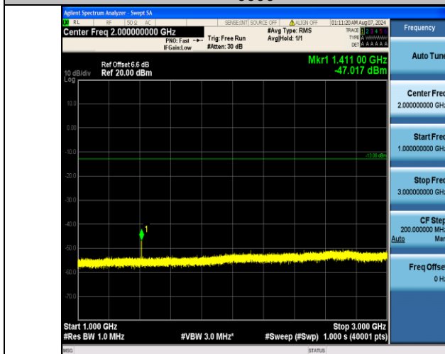
Band17_10MHz_QPSK_23790_1RB#0_1000~3000_1000~3000
