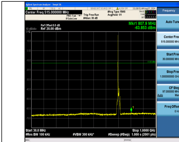
Band17_10MHz_QPSK_23780_1RB#0_30~1000_30~1000
