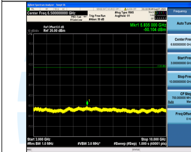
Band17_10MHz_QPSK_23780_50RB#0_3000~10000_3000~10000
