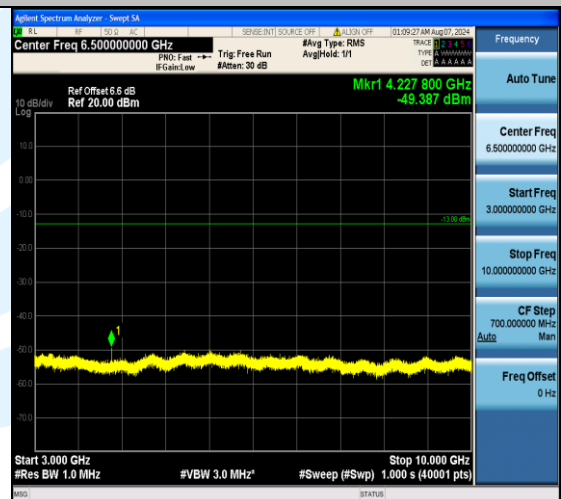
Band17_10MHz_16QAM_23780_1RB#0_3000~10000_3000~10000
