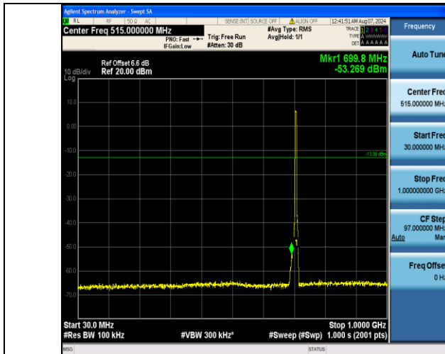
Band17_5MHz_QPSK_23825_25RB#0_30~1000_30~1000
