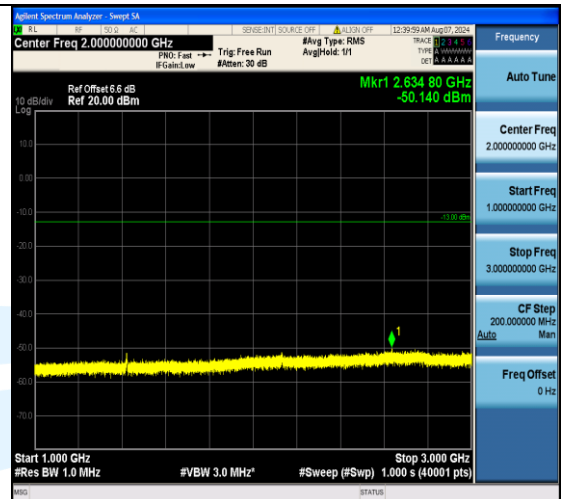
Band17_5MHz_16QAM_23790_25RB#0_1000~3000_1000~3000
