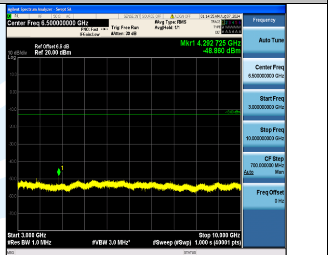
Band17_10MHz_QPSK_23800_1RB#49_3000~10000_3000~10000
