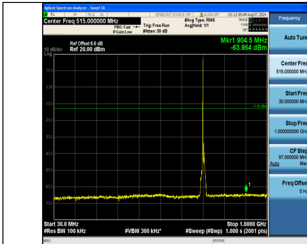
Band17_10MHz_QPSK_23800_1RB#0_30~1000_30~1000
