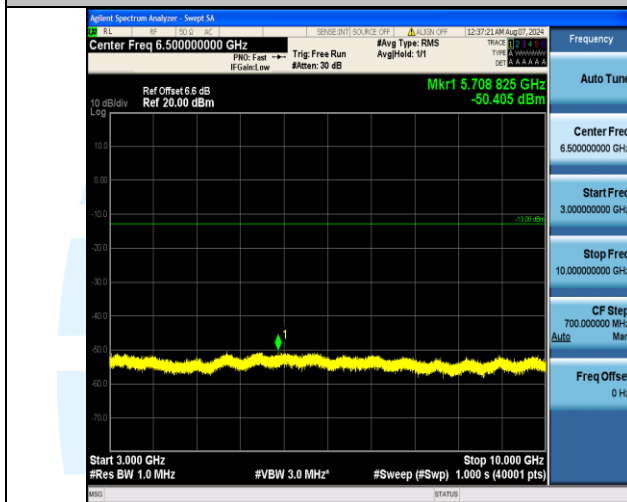
Band17_5MHz_QPSK_23755_25RB#0_3000~10000_3000~10000
