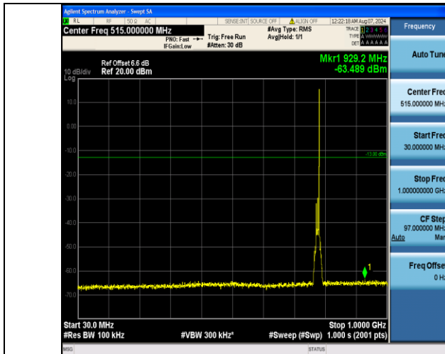
Band13_10MHz_16QAM_23230_1RB#49_30~1000_30~1000
