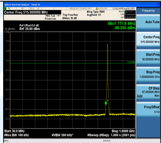
Band13_5MHz_16QAM_23255_25RB#0_30~1000_30~1000
