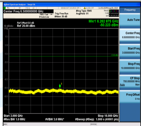
Band13_5MHz_16QAM_23230_1RB#24_3000~10000_3000~10000
