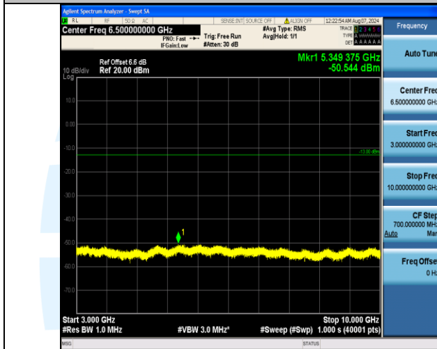
Band13_10MHz_QPSK_23230_50RB#0_3000~10000_3000~10000
