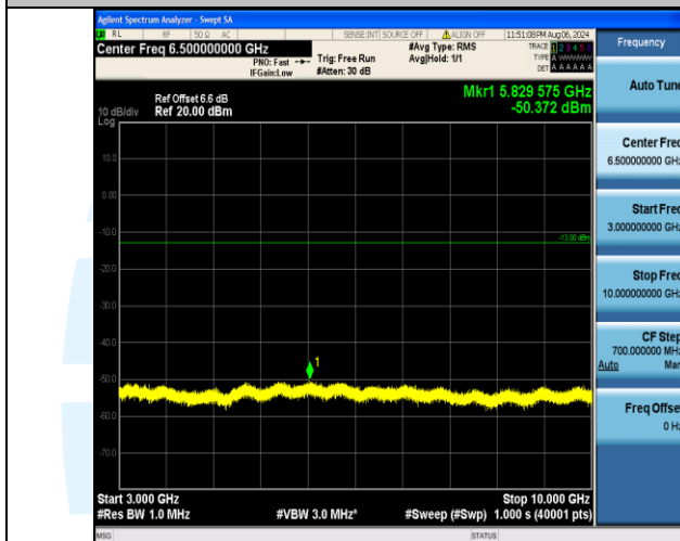
Band13_5MHz_16QAM_23205_1RB#24_3000~10000_3000~10000
