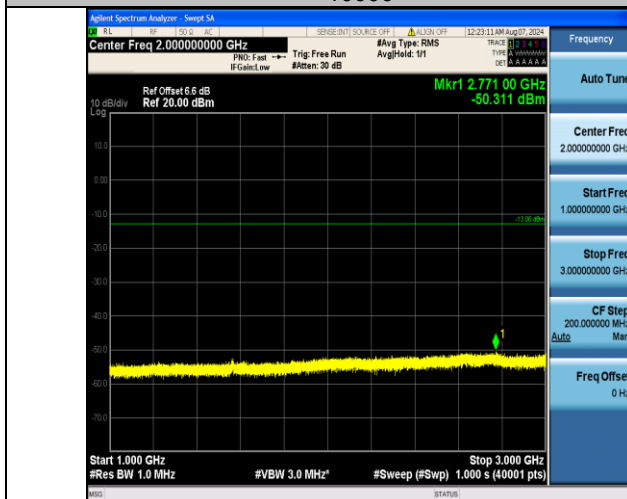
Band13_10MHz_16QAM_23230_50RB#0_1000~3000_1000~3000
