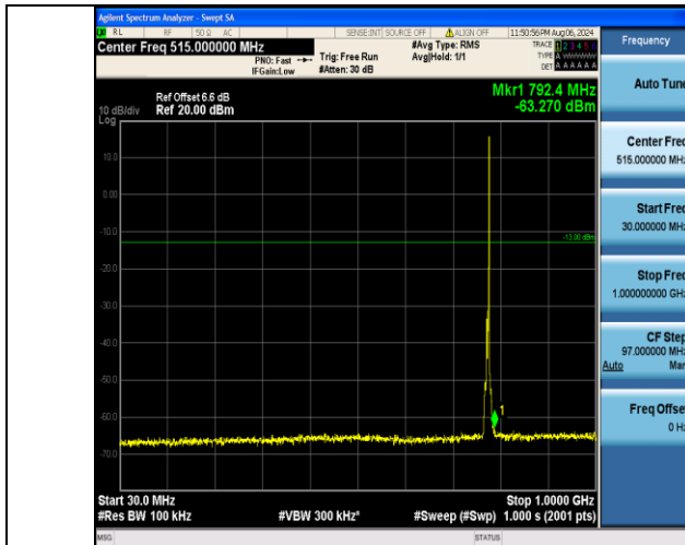
Band13_5MHz_16QAM_23205_1RB#24_30~1000_30~1000
