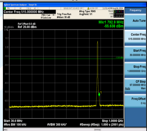
Band13_5MHz_16QAM_23205_25RB#0_30~1000_30~1000
