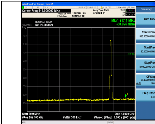
Band13_10MHz_QPSK_23230_50RB#0_30~1000_30~1000
