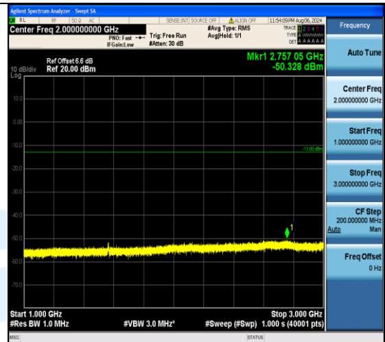
Band13_5MHz_16QAM_23230_25RB#0_1000~3000_1000~3000
