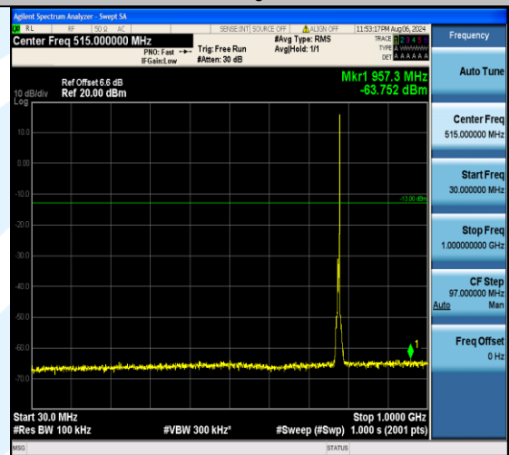
Band13_5MHz_16QAM_23230_1RB#24_30~1000_30~1000
