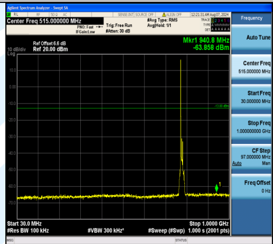
Band13_10MHz_16QAM_23230_1RB#0_30~1000_30~1000
