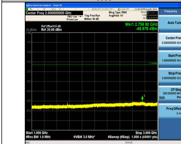
Band13_5MHz_16QAM_23255_25RB#0_1000~3000_1000~3000
