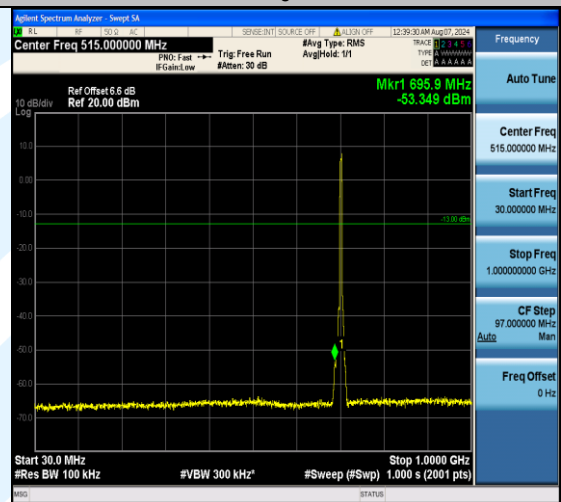
Band17_5MHz_QPSK_23790_25RB#0_30~1000_30~1000
