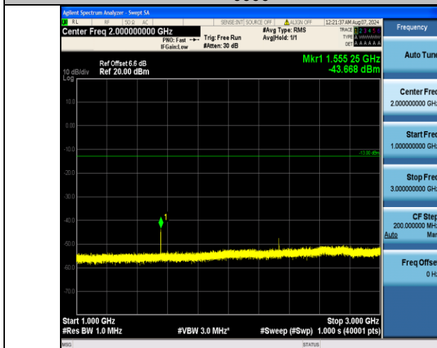
Band13_10MHz_16QAM_23230_1RB#0_1000~3000_1000~3000
