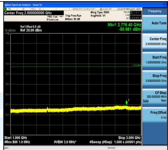
Band13_10MHz_QPSK_23230_50RB#0_1000~3000_1000~3000
