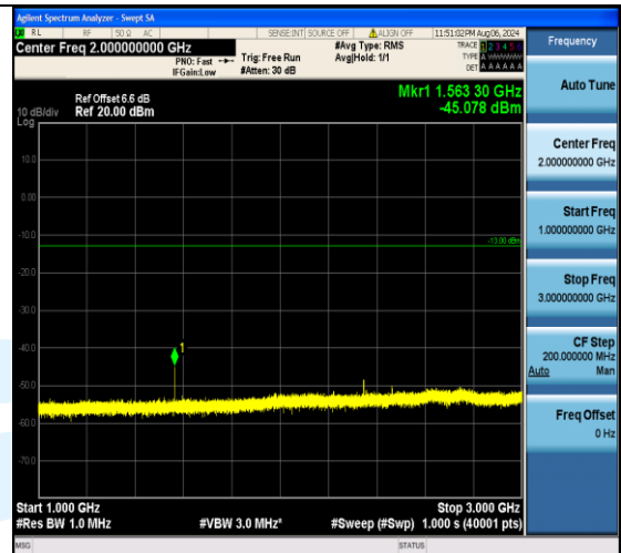
Band13_5MHz_16QAM_23205_1RB#24_1000~3000_1000~3000
