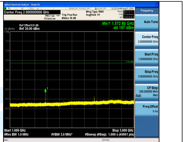
Band13_10MHz_16QAM_23230_1RB#49_1000~3000_1000~3000
