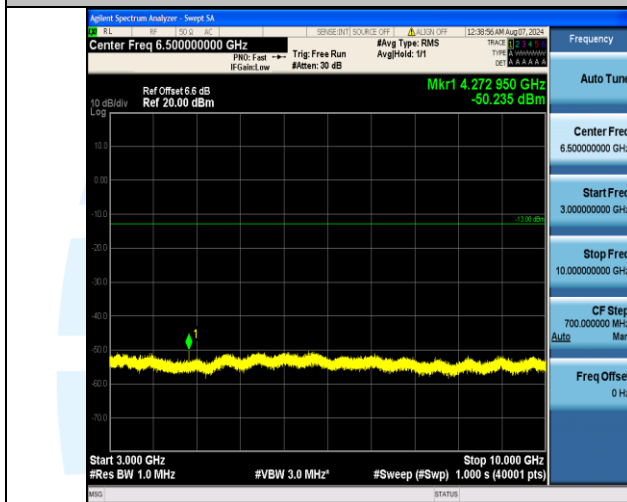
Band17_5MHz_QPSK_23790_1RB#24_3000~10000_3000~10000
