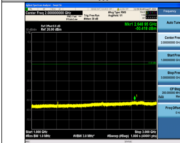
Band17_5MHz_QPSK_23790_25RB#0_1000~3000_1000~3000
