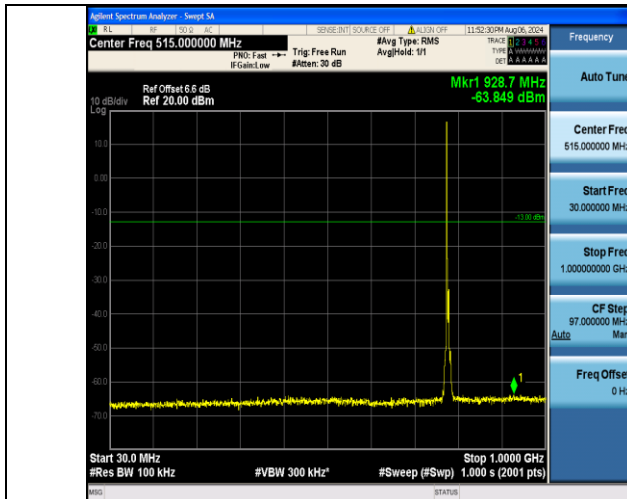
Band13_5MHz_16QAM_23230_1RB#0_30~1000_30~1000
