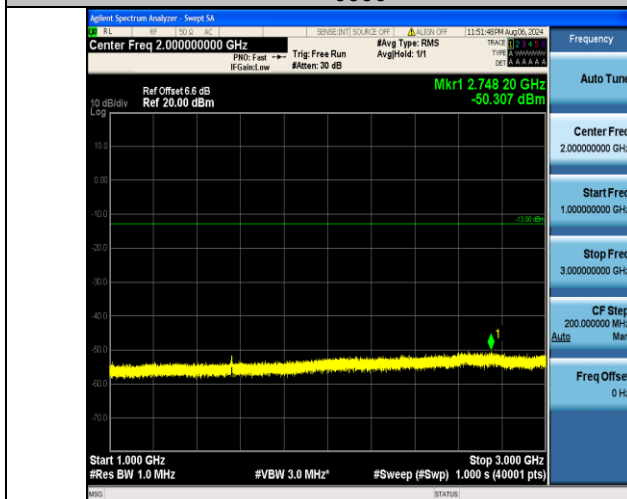
Band13_5MHz_16QAM_23205_25RB#0_1000~3000_1000~3000
