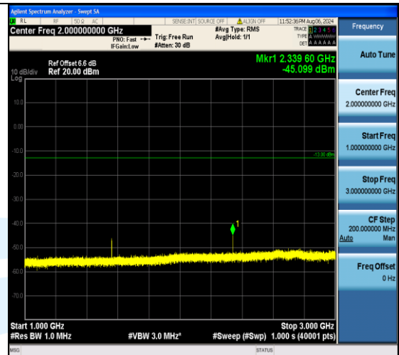
Band13_5MHz_16QAM_23230_1RB#0_1000~3000_1000~3000
