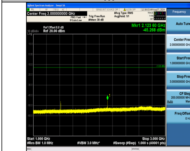
Band17_5MHz_QPSK_23790_1RB#0_1000~3000_1000~3000
