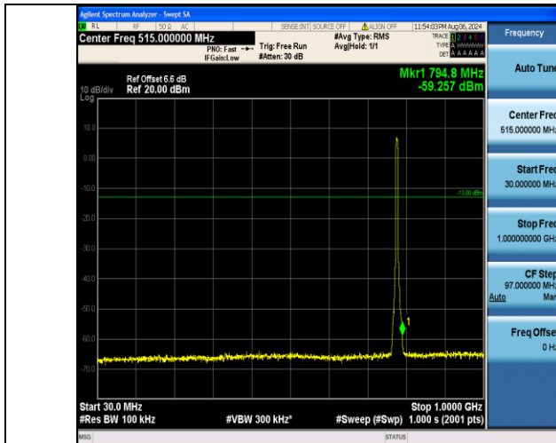
Band13_5MHz_16QAM_23230_25RB#0_30~1000_30~1000
