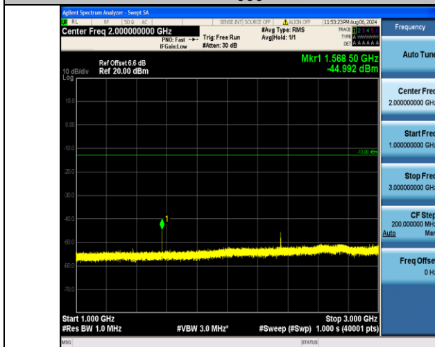
Band13_5MHz_16QAM_23230_1RB#24_1000~3000_1000~3000
