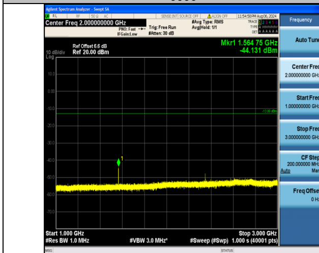
Band13_5MHz_16QAM_23255_1RB#0_1000~3000_1000~3000
