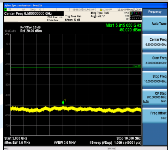
Band13_10MHz_16QAM_23230_1RB#0_3000~10000_3000~10000
