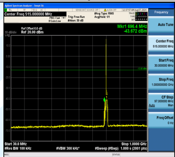
Band17_5MHz_QPSK_23790_1RB#0_30~1000_30~1000
