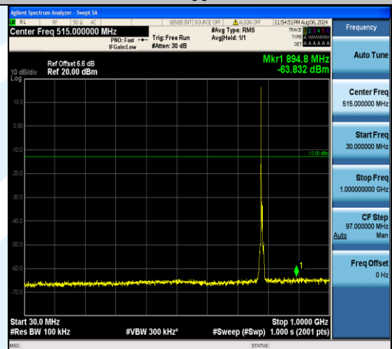
Band13_5MHz_16QAM_23255_1RB#0_30~1000_30~1000
