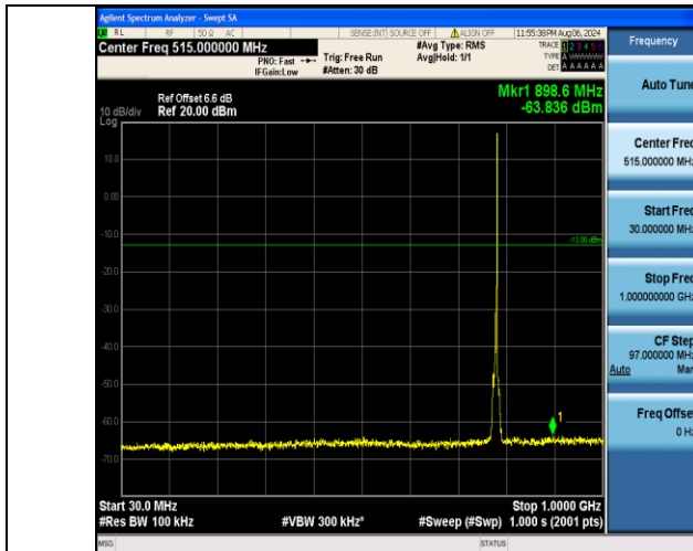
Band13_5MHz_16QAM_23255_1RB#24_30~1000_30~1000
