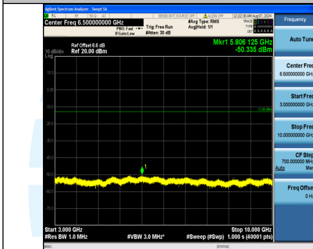
Band13_10MHz_16QAM_23230_1RB#49_3000~10000_3000~10000
