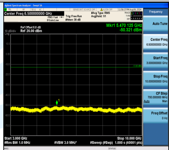
Band13_5MHz_16QAM_23255_25RB#0_3000~10000_3000~10000
