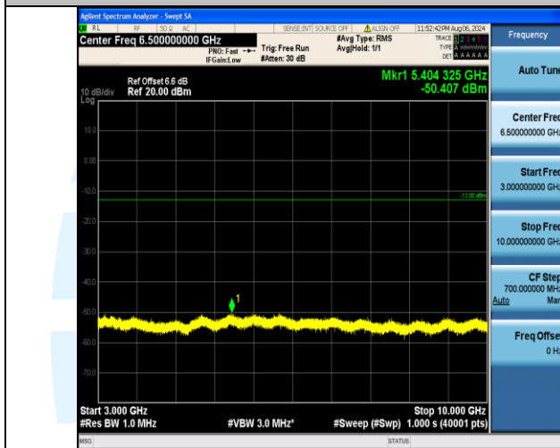
Band13_5MHz_16QAM_23230_1RB#0_3000~10000_3000~10000
