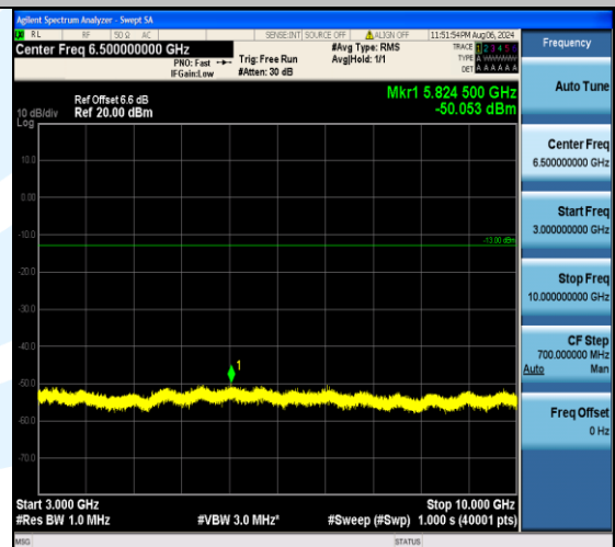
Band13_5MHz_16QAM_23205_25RB#0_3000~10000_3000~10000
