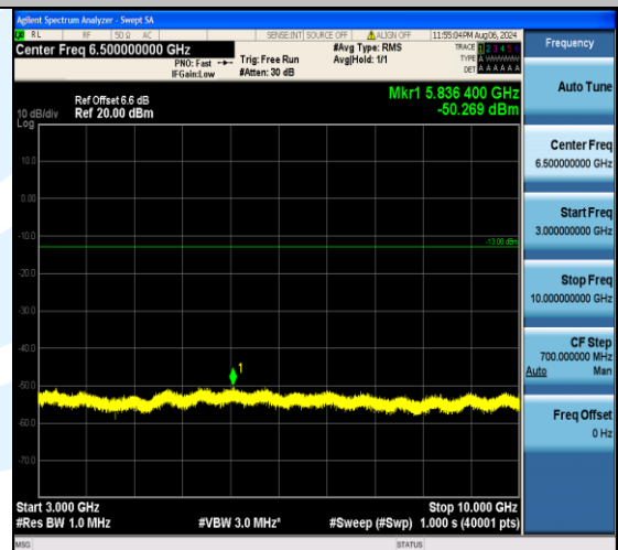
Band13_5MHz_16QAM_23255_1RB#0_3000~10000_3000~10000
