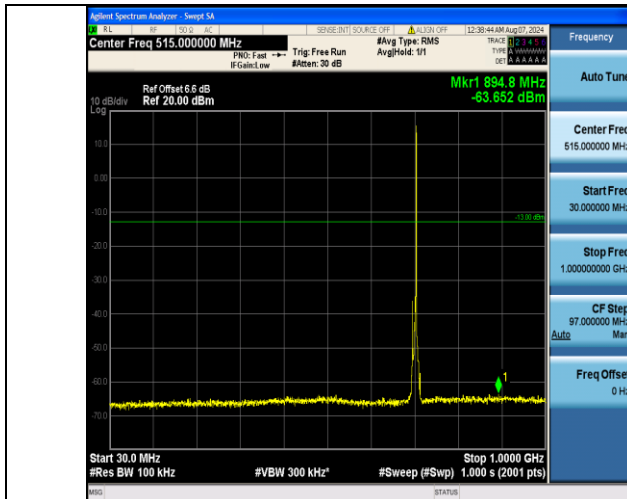
Band17_5MHz_QPSK_23790_1RB#24_30~1000_30~1000
