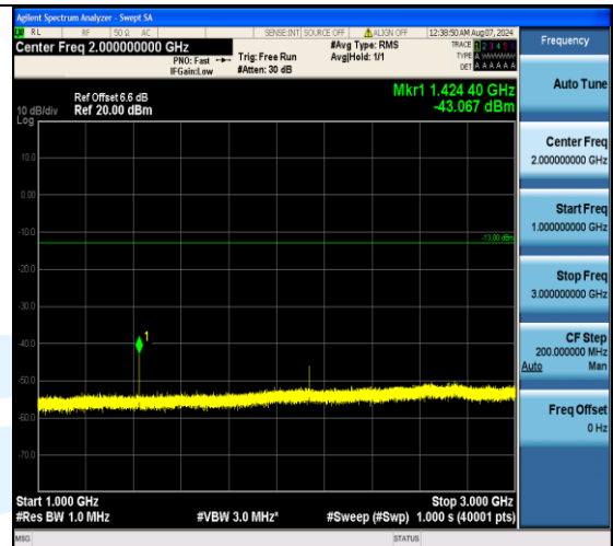
Band17_5MHz_QPSK_23790_1RB#24_1000~3000_1000~3000
