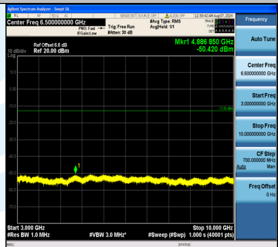
Band17_5MHz_QPSK_23790_25RB#0_3000~10000_3000~10000
