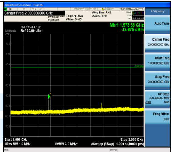
Band13_5MHz_16QAM_23255_1RB#24_1000~3000_1000~3000
