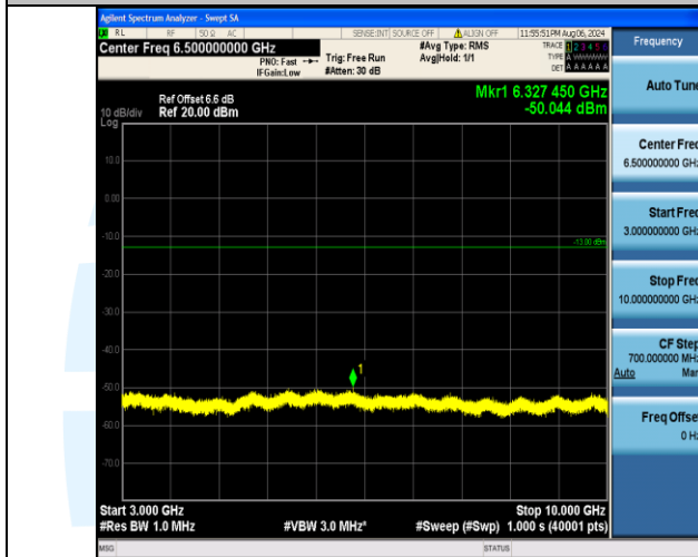
Band13_5MHz_16QAM_23255_1RB#24_3000~10000_3000~10000
