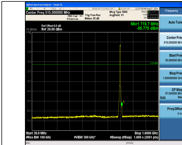
Band17_5MHz_QPSK_23755_25RB#0_30~1000_30~1000
