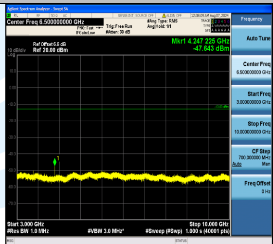
Band17_5MHz_QPSK_23790_1RB#0_3000~10000_3000~10000
