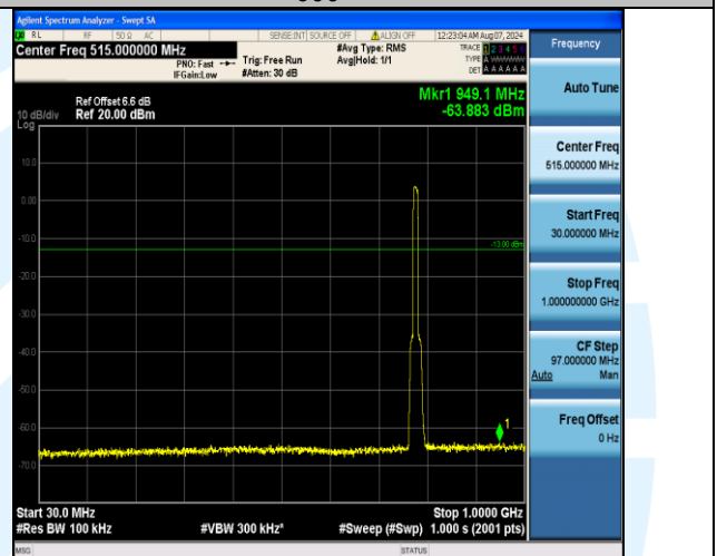
Band13_10MHz_16QAM_23230_50RB#0_30~1000_30~1000
