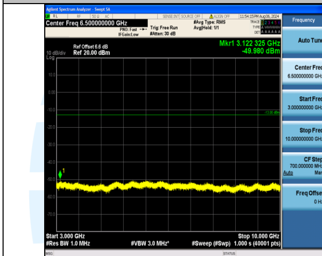
Band13_5MHz_16QAM_23230_25RB#0_3000~10000_3000~10000
