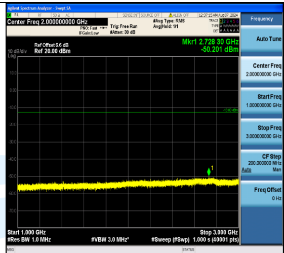
Band17_5MHz_QPSK_23755_25RB#0_1000~3000_1000~3000
