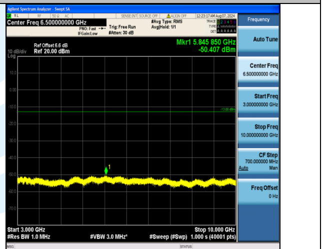
Band13_10MHz_16QAM_23230_50RB#0_3000~10000_3000~10000
