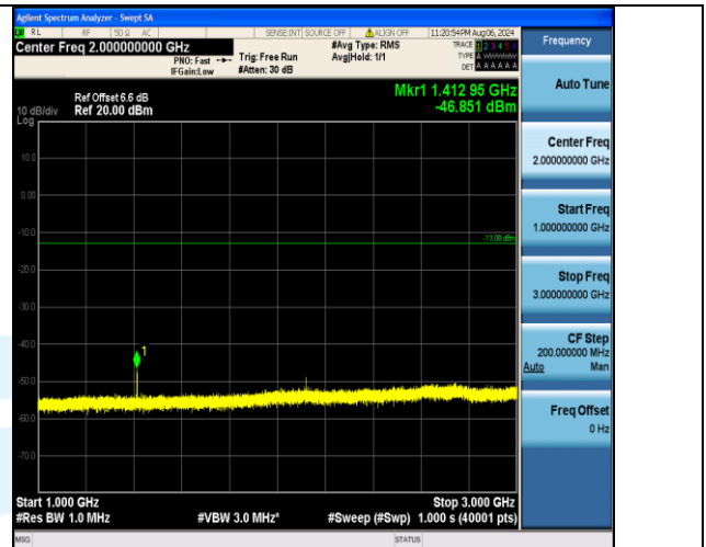
Band12_10MHz_QPSK_23130_1RB#0_1000~3000_1000~3000
