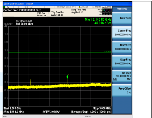
Band12_10MHz_16QAM_23130_1RB#49_1000~3000_1000~3000
