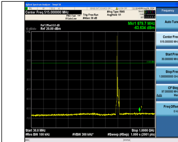
Band12_10MHz_16QAM_23095_1RB#0_30~1000_30~1000
