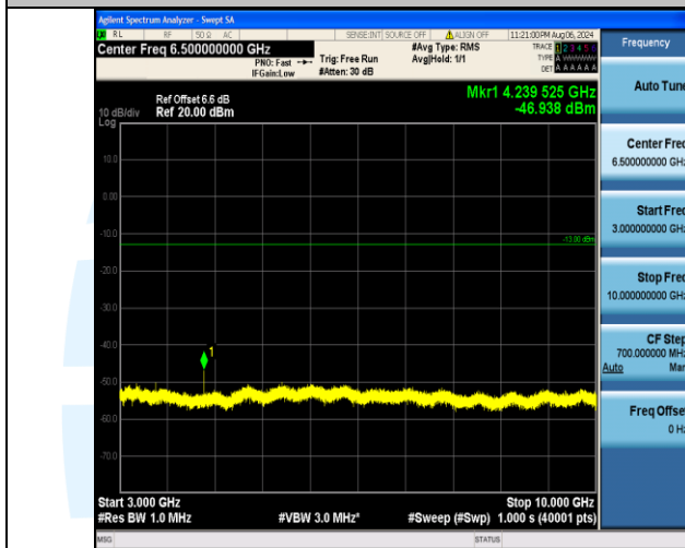
Band12_10MHz_QPSK_23130_1RB#0_3000~10000_3000~10000
