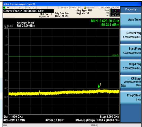
Band13_5MHz_QPSK_23205_25RB#0_1000~3000_1000~3000
