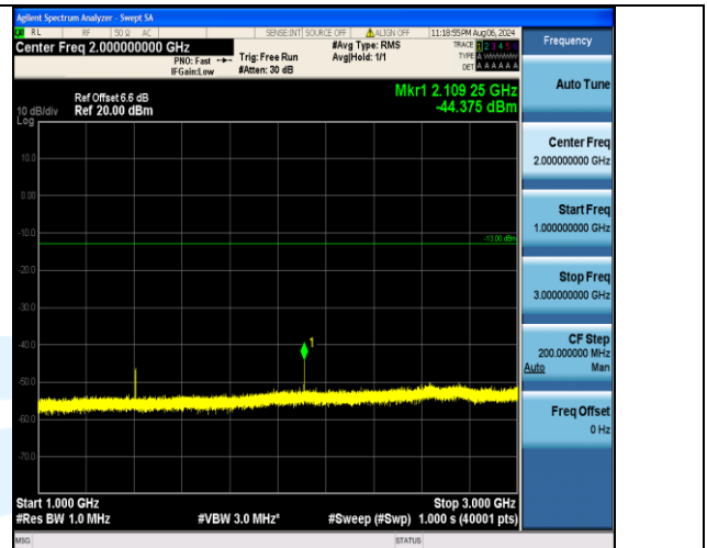
Band12_10MHz_16QAM_23095_1RB#0_1000~3000_1000~3000
