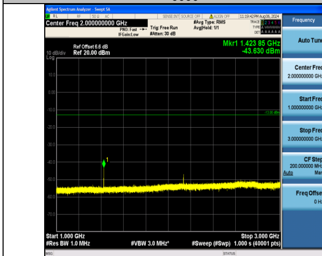
Band12_10MHz_16QAM_23095_1RB#49_1000~3000_1000~3000
