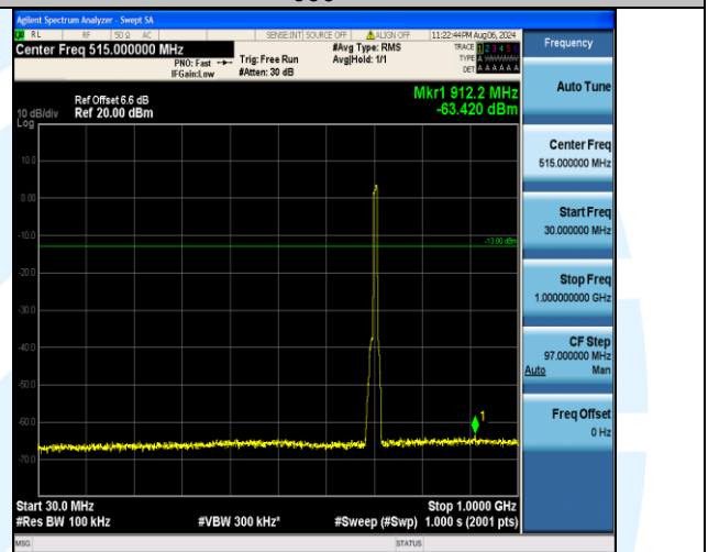
Band12_10MHz_16QAM_23130_50RB#0_30~1000_30~1000
