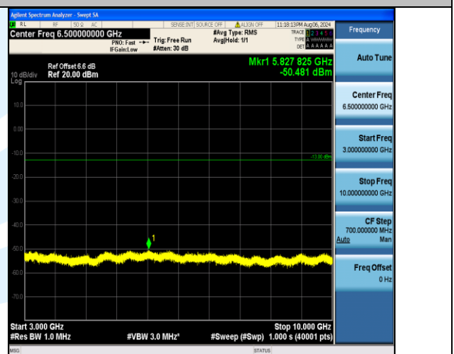
Band12_10MHz_16QAM_23060_50RB#0_3000~10000_3000~10000
