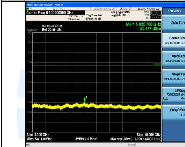
Band12_10MHz_16QAM_23095_1RB#0_3000~10000_3000~10000
