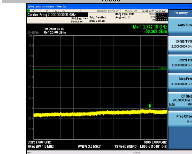
Band12_10MHz_16QAM_23060_50RB#0_1000~3000_1000~3000
