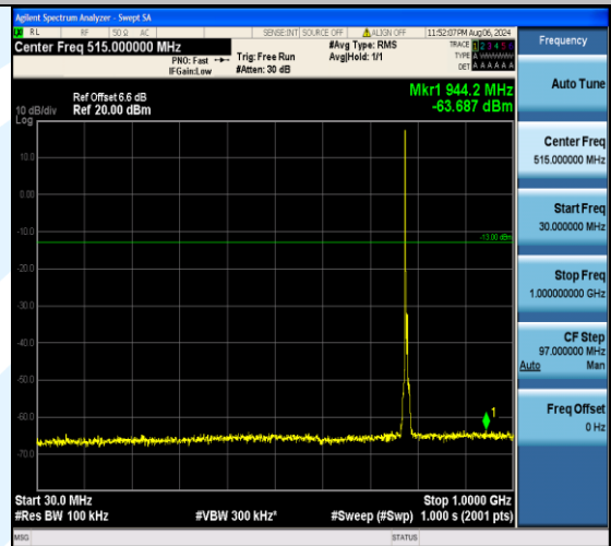
Band13_5MHz_QPSK_23230_1RB#0_30~1000_30~1000
