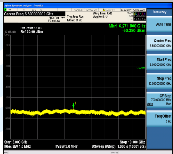
Band13_5MHz_QPSK_23230_1RB#0_3000~10000_3000~10000
