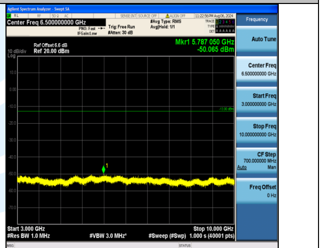
Band12_10MHz_16QAM_23130_50RB#0_3000~10000_3000~10000
