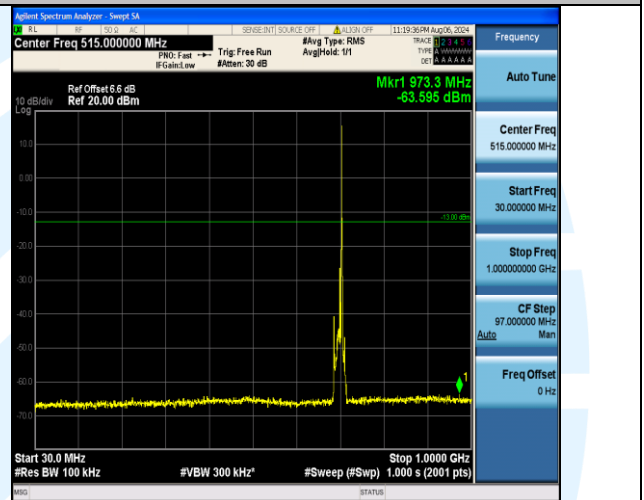
Band12_10MHz_16QAM_23095_1RB#49_30~1000_30~1000
