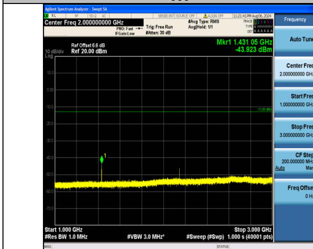
Band12_10MHz_QPSK_23130_1RB#49_1000~3000_1000~3000
