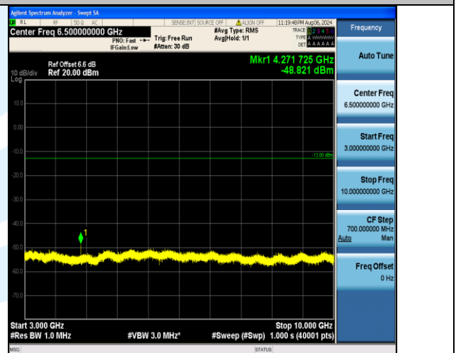
Band12_10MHz_16QAM_23095_1RB#49_3000~10000_3000~10000
