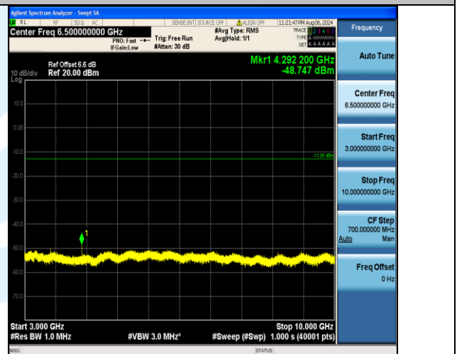
Band12_10MHz_QPSK_23130_1RB#49_3000~10000_3000~10000
