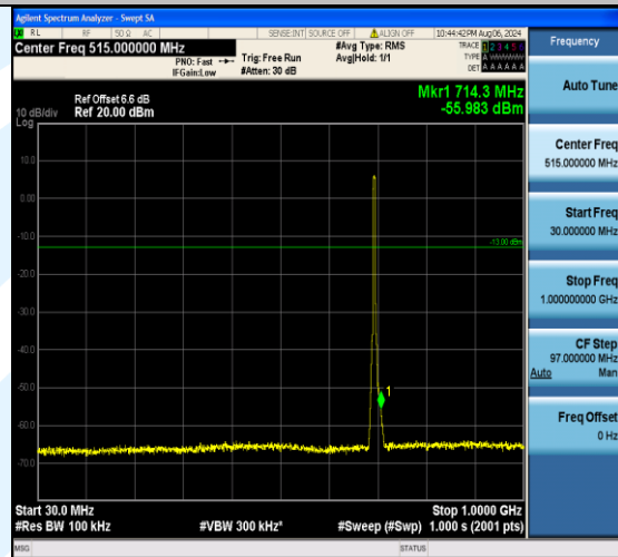
Band12_5MHz_16QAM_23035_25RB#0_30~1000_30~1000
