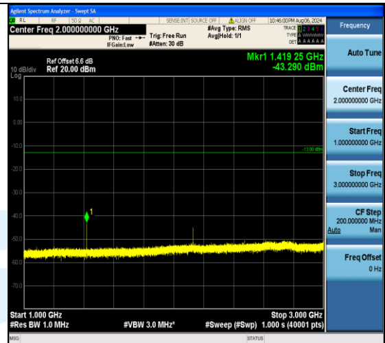
Band12_5MHz_QPSK_23095_1RB#24_1000~3000_1000~3000
