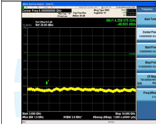
Band12_5MHz_QPSK_23095_1RB#24_3000~10000_3000~10000
