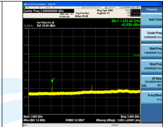
Band12_10MHz_QPSK_23095_1RB#49_1000~3000_1000~3000
