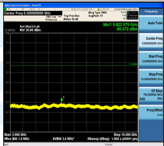
Band12_5MHz_QPSK_23095_25RB#0_3000~10000_3000~10000
