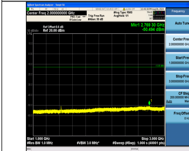
Band12_5MHz_16QAM_23155_25RB#0_1000~3000_1000~3000
