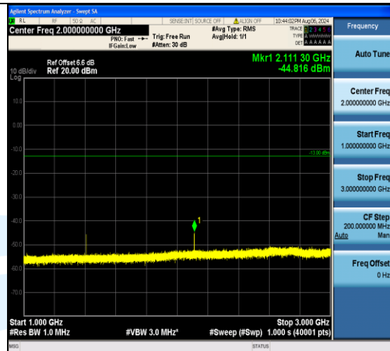
Band12_5MHz_16QAM_23035_1RB#24_1000~3000_1000~3000
