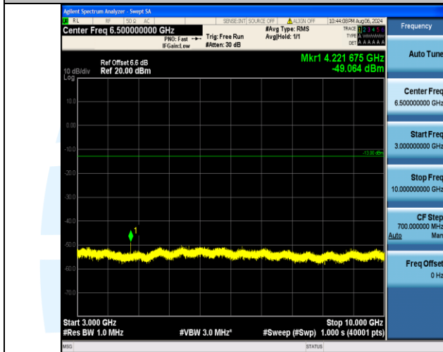
Band12_5MHz_16QAM_23035_1RB#24_3000~10000_3000~10000
