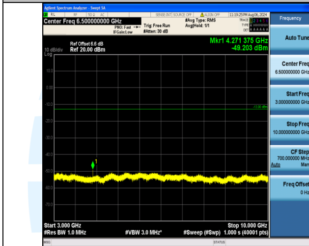
Band12_10MHz_QPSK_23095_1RB#49_3000~10000_3000~10000
