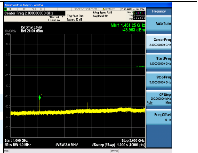
Band12_5MHz_16QAM_23155_1RB#24_1000~3000_1000~3000
