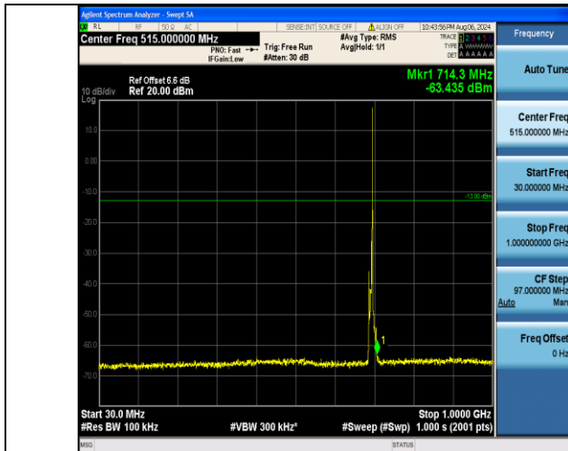
Band12_5MHz_16QAM_23035_1RB#24_30~1000_30~1000
