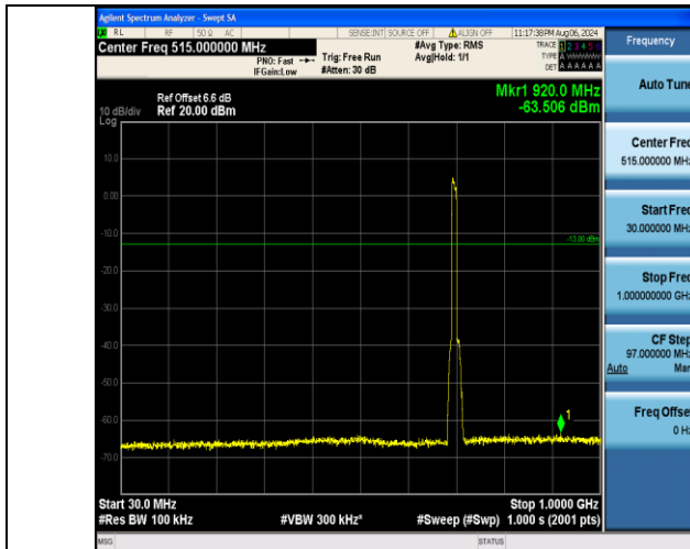
Band12_10MHz_QPSK_23060_50RB#0_30~1000_30~1000
