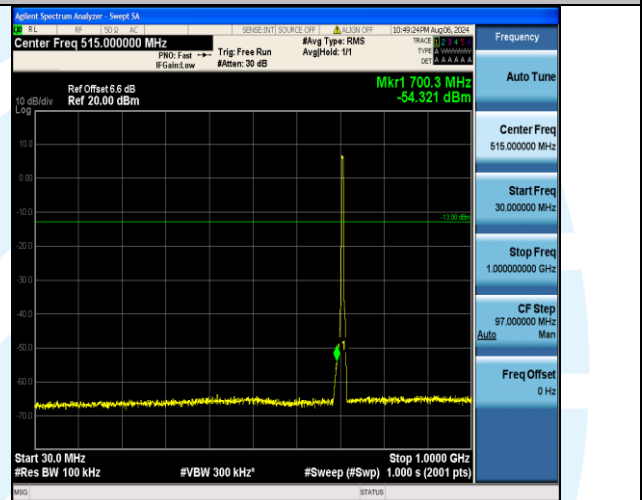
Band12_5MHz_16QAM_23155_25RB#0_30~1000_30~1000
