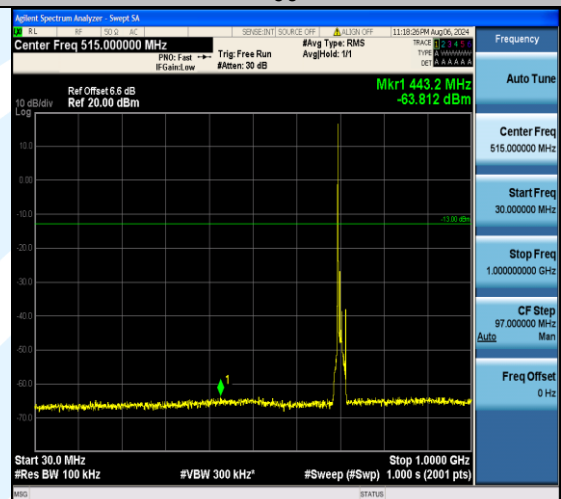
Band12_10MHz_QPSK_23095_1RB#0_30~1000_30~1000
