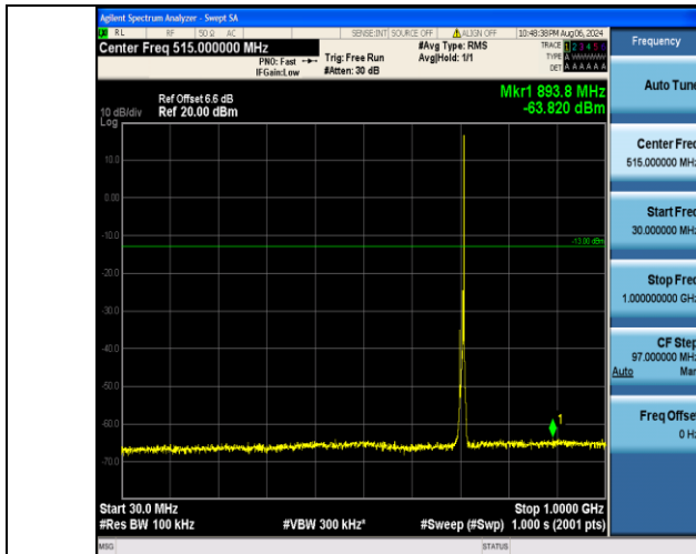
Band12_5MHz_16QAM_23155_1RB#24_30~1000_30~1000
