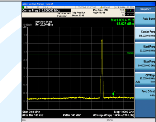
Band12_10MHz_QPSK_23095_50RB#0_30~1000_30~1000
