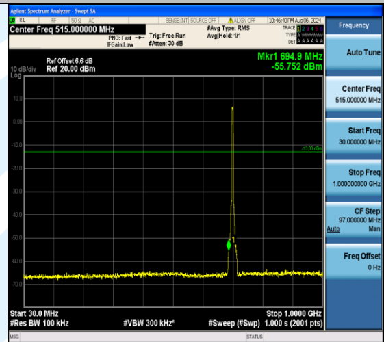
Band12_5MHz_QPSK_23095_25RB#0_30~1000_30~1000
