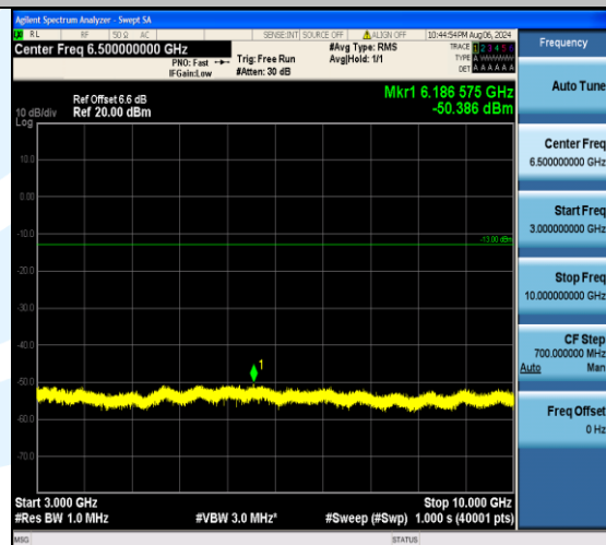
Band12_5MHz_16QAM_23035_25RB#0_3000~10000_3000~10000
