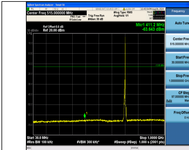
Band12_5MHz_QPSK_23095_1RB#24_30~1000_30~1000
