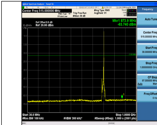
Band12_10MHz_QPSK_23095_1RB#49_30~1000_30~1000
