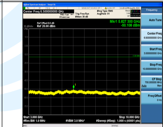
Band12_10MHz_QPSK_23095_50RB#0_3000~10000_3000~10000
