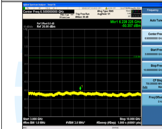
Band12_10MHz_QPSK_23060_50RB#0_3000~10000_3000~10000
