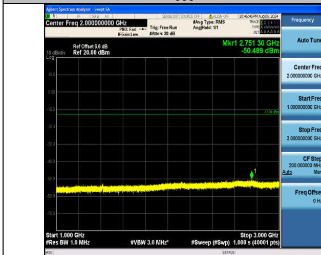
Band12_5MHz_QPSK_23095_25RB#0_1000~3000_1000~3000
