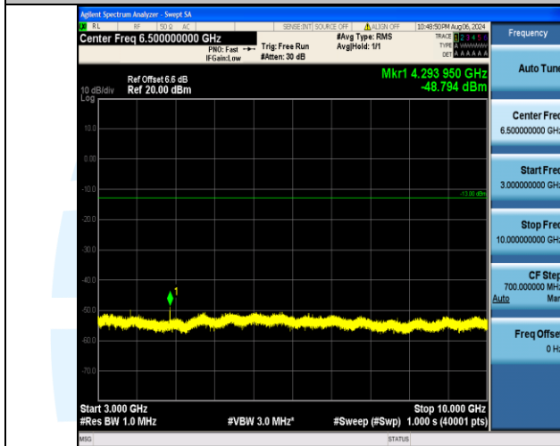
Band12_5MHz_16QAM_23155_1RB#24_3000~10000_3000~10000
