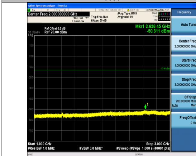
Band12_10MHz_QPSK_23095_50RB#0_1000~3000_1000~3000
