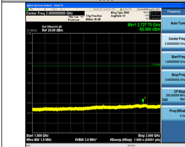
Band12_5MHz_16QAM_23035_25RB#0_1000~3000_1000~3000
