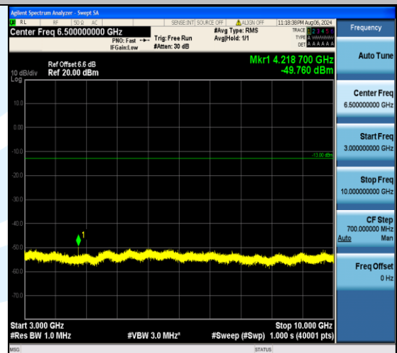
Band12_10MHz_QPSK_23095_1RB#0_3000~10000_3000~10000
