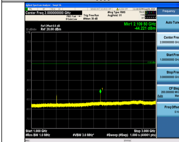
Band12_10MHz_QPSK_23095_1RB#0_1000~3000_1000~3000
