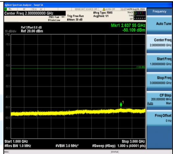
Band12_10MHz_QPSK_23060_50RB#0_1000~3000_1000~3000
