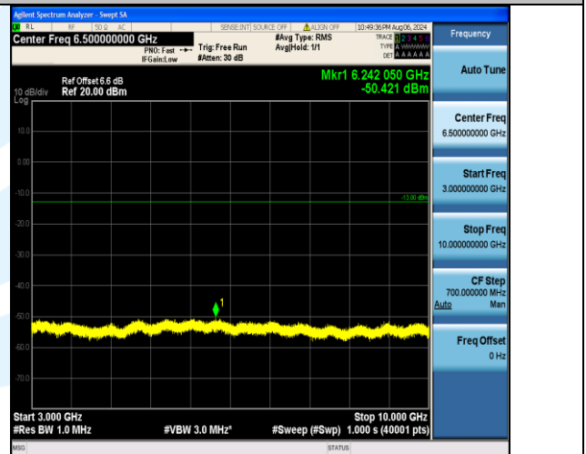
Band12_5MHz_16QAM_23155_25RB#0_3000~10000_3000~10000
