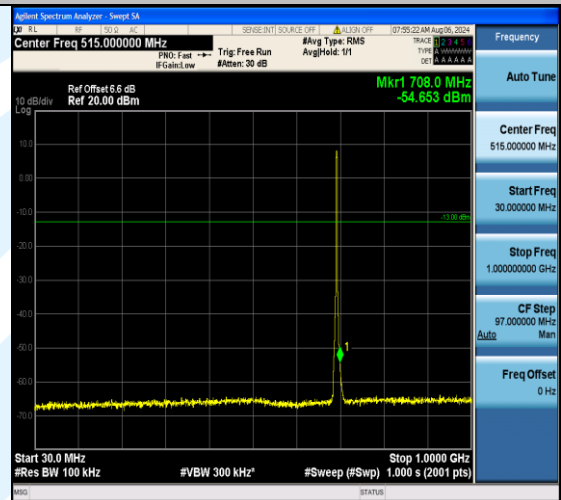
Band12_3MHz_16QAM_23025_15RB#0_30~1000_30~1000
