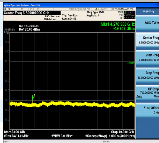
Band12_3MHz_16QAM_23165_1RB#0_3000~10000_3000~10000
