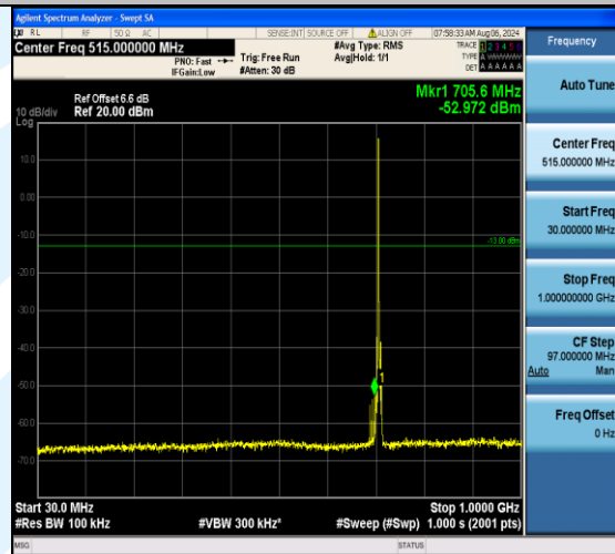
Band12_3MHz_16QAM_23165_1RB#0_30~1000_30~1000
