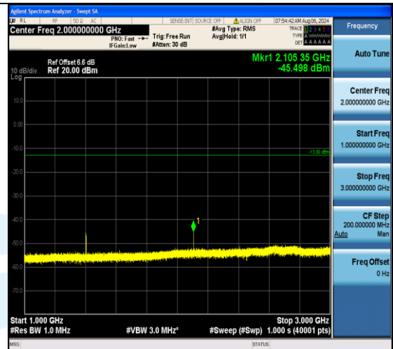
Band12_3MHz_16QAM_23025_1RB#14_1000~3000_1000~3000
