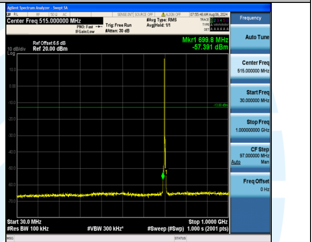
Band12_3MHz_QPSK_23095_1RB#0_30~1000_30~1000
