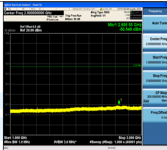
Band12_3MHz_16QAM_23095_15RB#0_1000~3000_1000~3000
