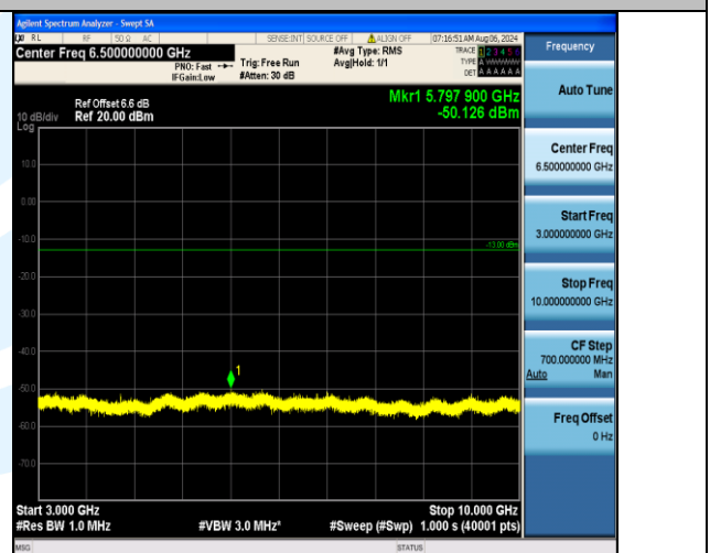
Band12_1.4MHz_16QAM_23017_6RB#0_3000~10000_3000~10000
