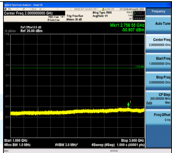
Band12_1.4MHz_16QAM_23095_6RB#0_1000~3000_1000~3000
