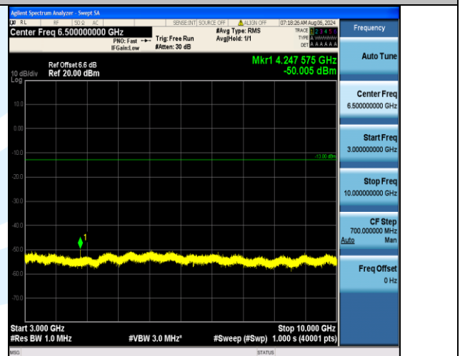
Band12_1.4MHz_16QAM_23095_1RB#5_3000~10000_3000~10000
