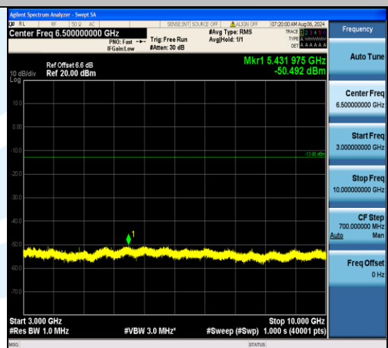
Band12_1.4MHz_16QAM_23173_1RB#0_3000~10000_3000~10000
