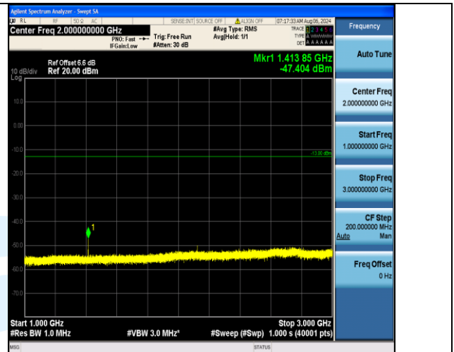
Band12_1.4MHz_16QAM_23095_1RB#0_1000~3000_1000~3000
