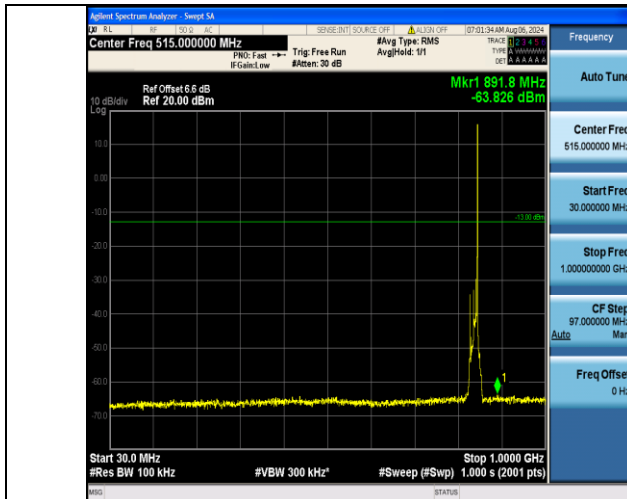
Band5_10MHz_16QAM_20600_1RB#49_30~1000_30~1000
