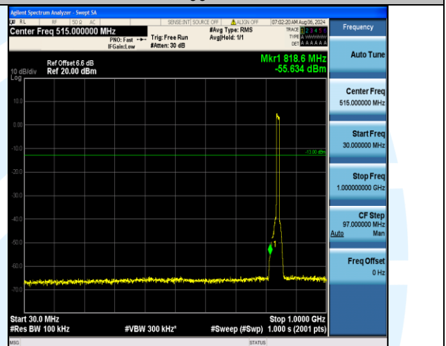
Band5_10MHz_16QAM_20600_50RB#0_30~1000_30~1000
