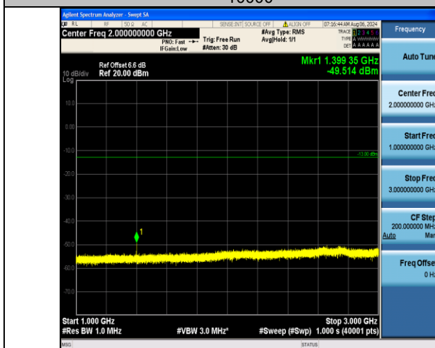
Band12_1.4MHz_16QAM_23017_6RB#0_1000~3000_1000~3000
