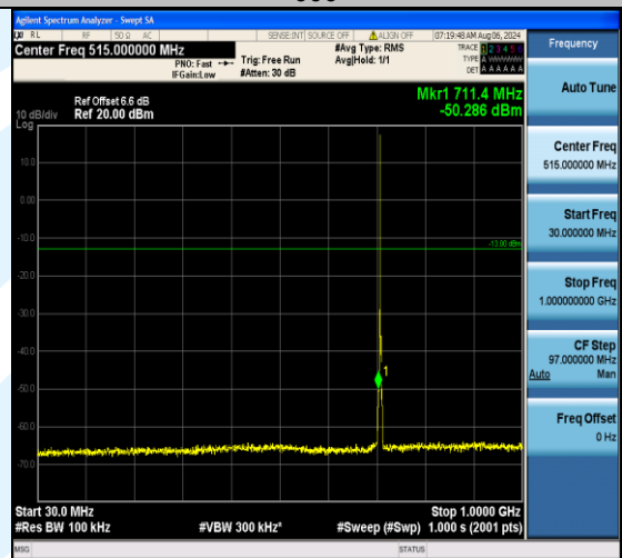
Band12_1.4MHz_16QAM_23173_1RB#0_30~1000_30~1000
