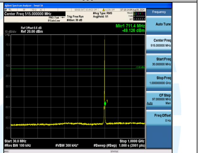
Band12_1.4MHz_16QAM_23095_1RB#5_30~1000_30~1000
