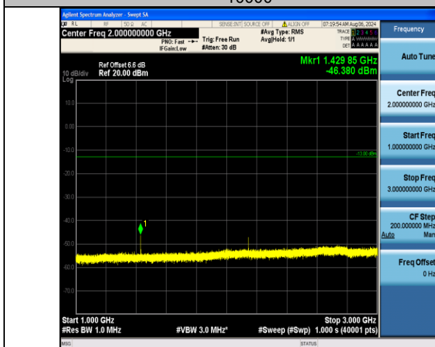
Band12_1.4MHz_16QAM_23173_1RB#0_1000~3000_1000~3000
