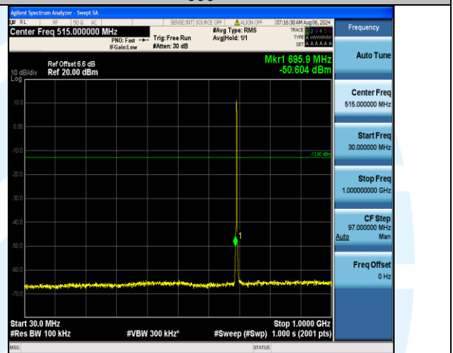
Band12_1.4MHz_16QAM_23017_6RB#0_30~1000_30~1000
