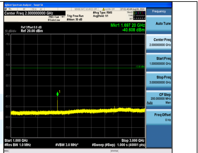
Band5_10MHz_16QAM_20600_1RB#49_1000~3000_1000~3000
