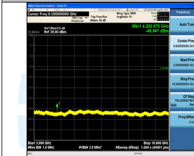
Band12_1.4MHz_16QAM_23017_1RB#5_3000~10000_3000~10000
