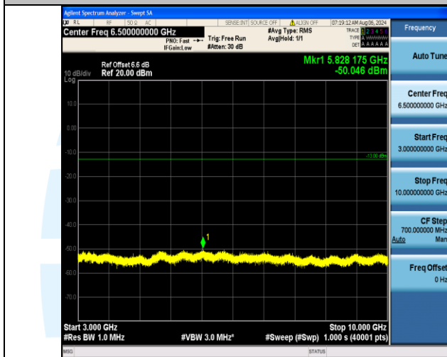
Band12_1.4MHz_16QAM_23095_6RB#0_3000~10000_3000~10000
