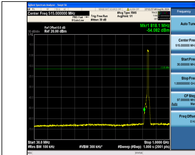
Band5_10MHz_QPSK_20600_50RB#0_30~1000_30~1000
