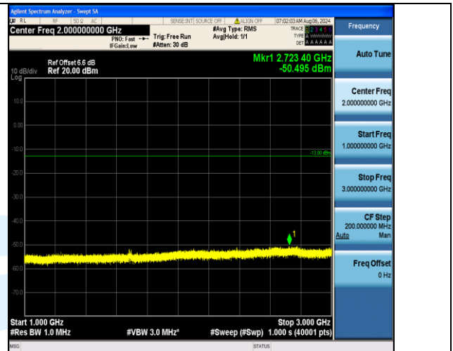
Band5_10MHz_QPSK_20600_50RB#0_1000~3000_1000~3000
