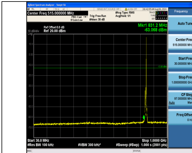
Band5_5MHz_16QAM_20625_1RB#24_30~1000_30~1000
