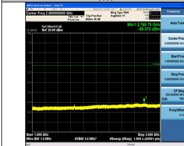
Band5_10MHz_16QAM_20450_50RB#0_1000~3000_1000~3000
