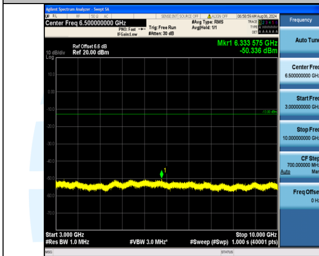
Band5_10MHz_QPSK_20525_1RB#49_3000~10000_3000~10000 000
