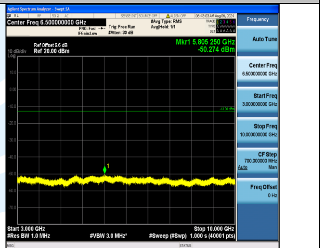
Band5_5MHz_16QAM_20625_25RB#0_3000~10000_3000~10000
