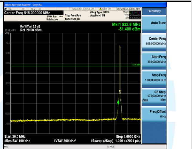
Band5_5MHz_16QAM_20625_25RB#0_30~1000_30~1000
