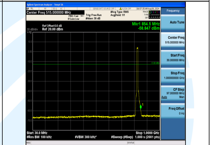
Band5_10MHz_16QAM_20450_50RB#0_30~1000_30~1000
