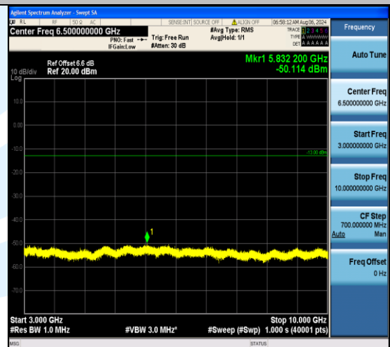
Band5_10MHz_QPSK_20525_1RB#0_3000~10000_3000~10000
