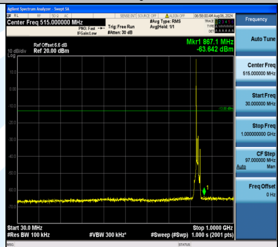
Band5_10MHz_QPSK_20525_1RB#0_30~1000_30~1000
