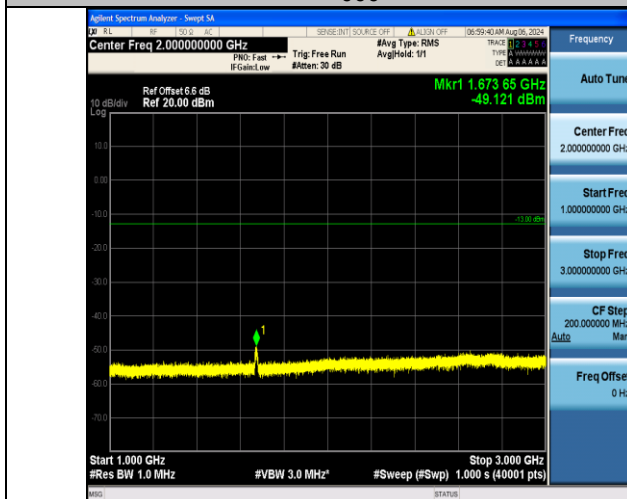
Band5_10MHz_QPSK_20525_50RB#0_1000~3000_1000~3000 0
