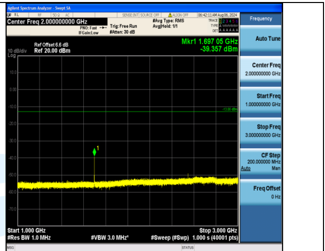
Band5_5MHz_16QAM_20625_1RB#24_1000~3000_1000~3000
