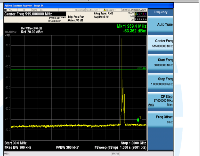
Band5_10MHz_16QAM_20450_1RB#0_30~1000_30~1000
