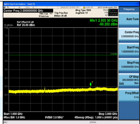
Band5_10MHz_QPSK_20450_50RB#0_1000~3000_1000~3000
