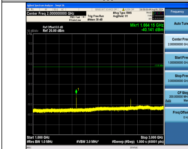
Band5_10MHz_QPSK_20525_1RB#0_1000~3000_1000~3000
