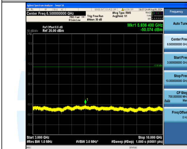
Band5_10MHz_QPSK_20450_50RB#0_3000~10000_3000~10000
