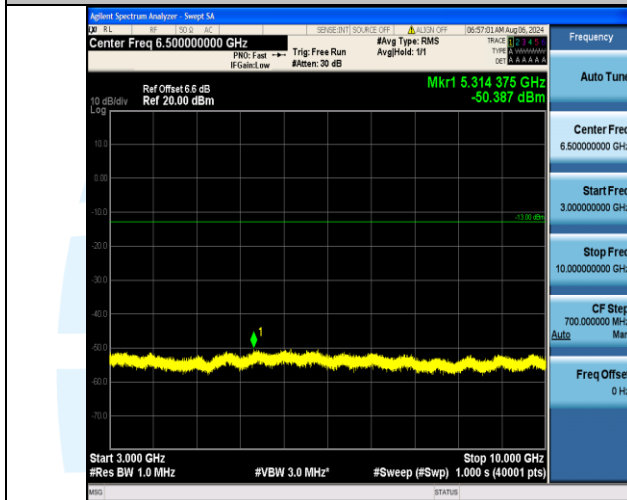
Band5_10MHz_16QAM_20450_1RB#49_3000~10000_3000~10000
