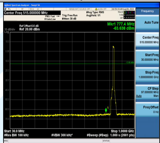
Band5_10MHz_QPSK_20525_50RB#0_30~1000_30~1000
