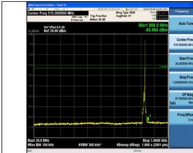
Band5_10MHz_16QAM_20450_1RB#49_30~1000_30~1000
