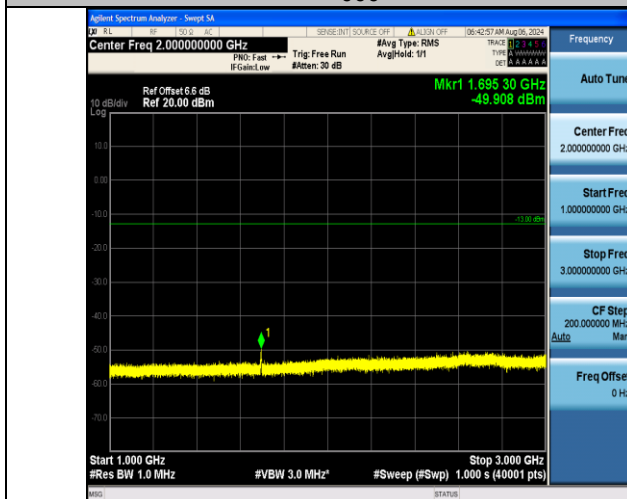
Band5_5MHz_16QAM_20625_25RB#0_1000~3000_1000~3000
