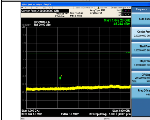
Band5_10MHz_16QAM_20450_1RB#0_1000~3000_1000~3000
