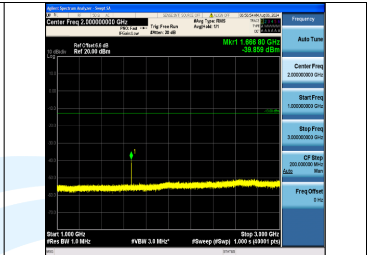
Band5_10MHz_16QAM_20450_1RB#49_1000~3000_1000~3000
