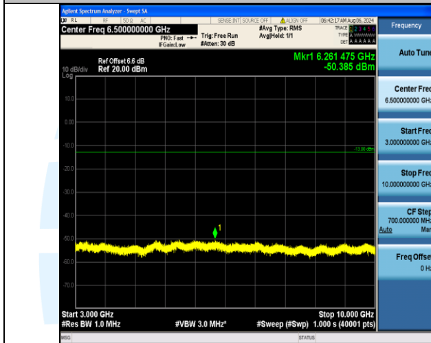
Band5_5MHz_16QAM_20625_1RB#24_3000~10000_3000~10000
