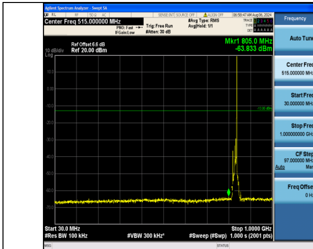
Band5_10MHz_QPSK_20525_1RB#49_30~1000_30~1000
