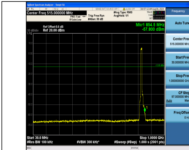
Band5_10MHz_QPSK_20450_50RB#0_30~1000_30~1000
