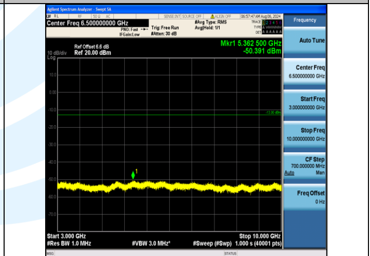
Band5_10MHz_16QAM_20450_50RB#0_3000~10000_3000~10000
