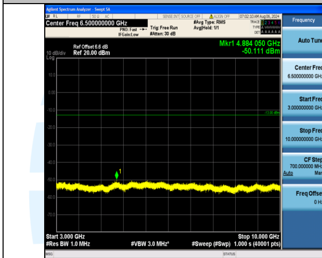
Band5_10MHz_QPSK_20600_50RB#0_3000~10000_3000~10000
