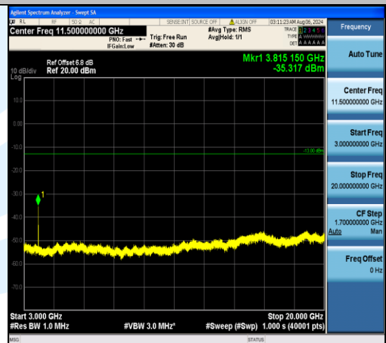
Band2_5MHz_16QAM_19175_25RB#0_3000~20000_3000~20000
