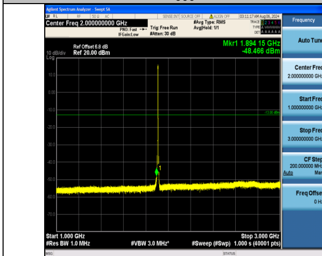
Band2_5MHz_16QAM_19175_25RB#0_1000~3000_1000~3000
