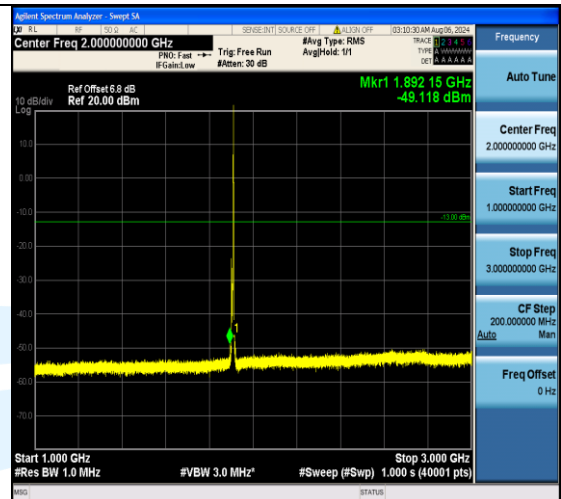
Band2_5MHz_16QAM_19175_1RB#24_1000~3000_1000~3000
