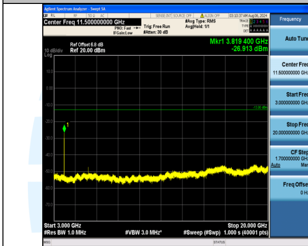
Band2_5MHz_16QAM_19175_1RB#24_3000~20000_3000~20000
