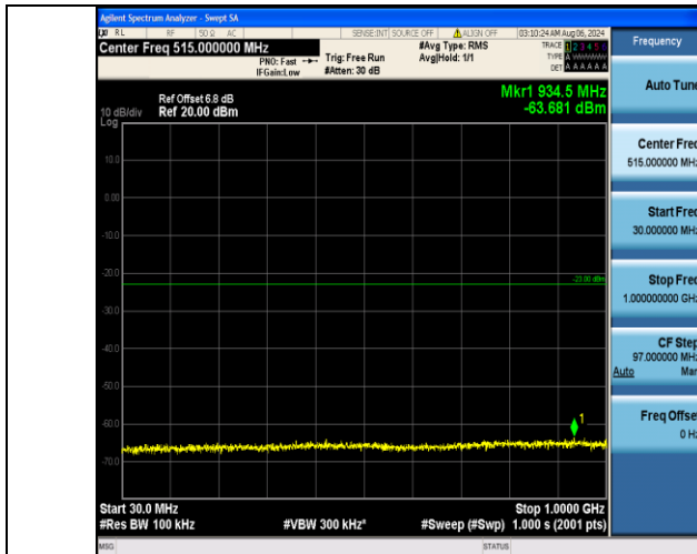
Band2_5MHz_16QAM_19175_1RB#24_30~1000_30~1000
