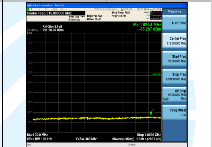
Band4_15MHz_16QAM_20175_1RB#74_30~1000_30~1000
