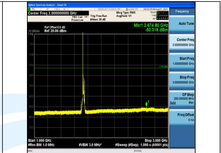
Band4_15MHz_16QAM_20175_1RB#0_1000~3000_1000~3000
