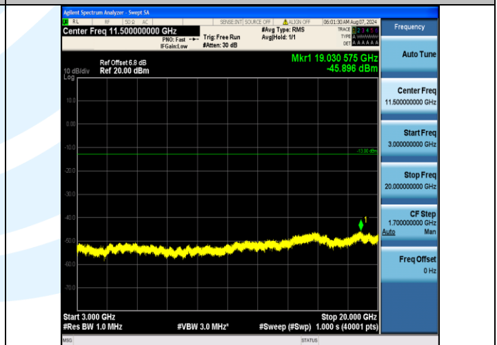
Band4_15MHz_16QAM_20175_1RB#74_3000~20000_3000~20000
