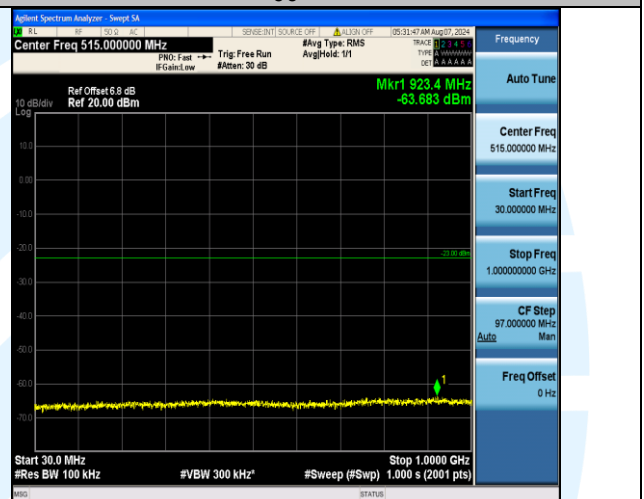
Band4_10MHz_16QAM_20350_50RB#0_30~1000_30~1000
