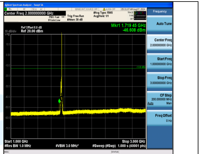
Band4_10MHz_16QAM_20350_1RB#49_1000~3000_1000~3000
