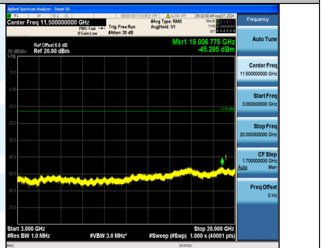
Band4_10MHz_16QAM_20350_50RB#0_3000~20000_3000~20000
