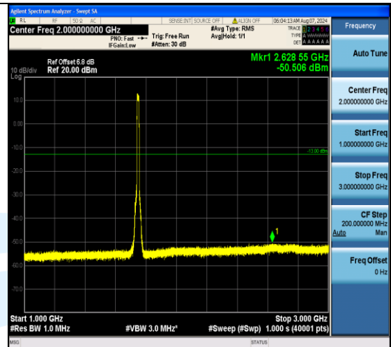
Band4_15MHz_QPSK_20325_75RB#0_1000~3000_1000~3000
