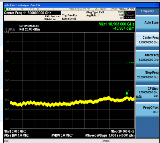
Band4_15MHz_16QAM_20025_1RB#0_3000~20000_3000~20000
