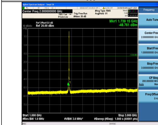
Band4_5MHz_16QAM_20375_25RB#0_1000~3000_1000~3000
