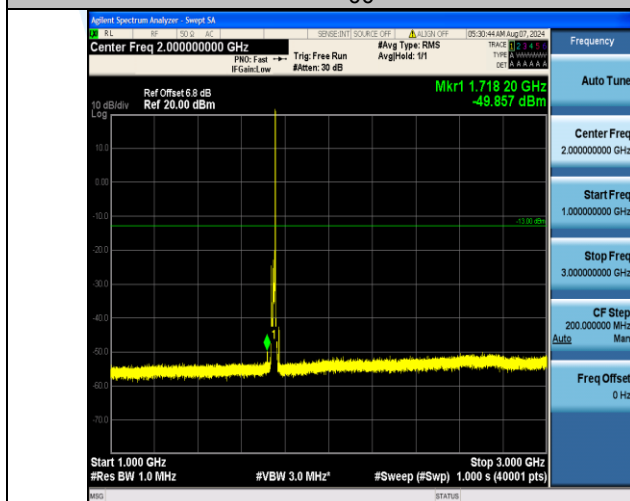
Band4_10MHz_QPSK_20350_1RB#49_1000~3000_1000~3000
