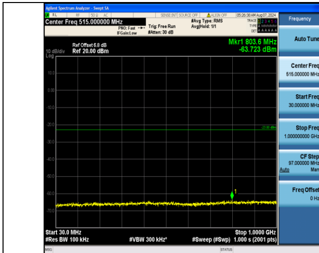
Band4_10MHz_QPSK_20000_50RB#0_30~1000_30~1000
