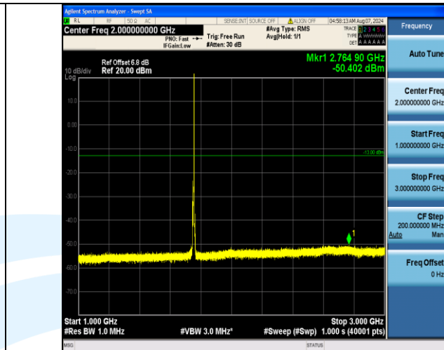
Band4_5MHz_16QAM_20375_1RB#24_1000~3000_1000~3000
