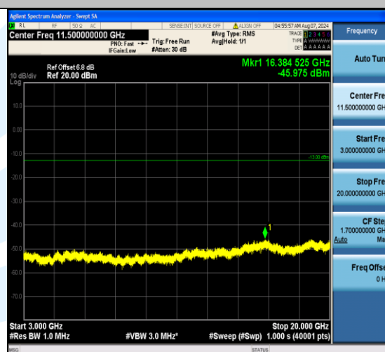
Band4_5MHz_16QAM_20175_1RB#24_3000~20000_3000~20000
