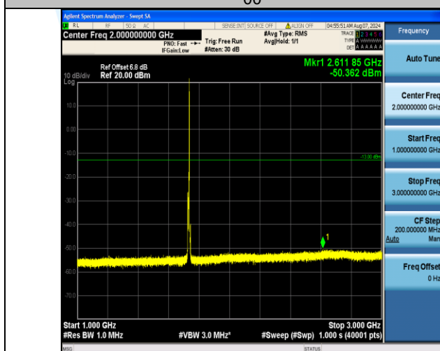
Band4_5MHz_16QAM_20175_1RB#24_1000~3000_1000~3000
