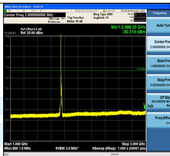
Band4_10MHz_QPSK_20350_1RB#0_1000~3000_1000~3000
