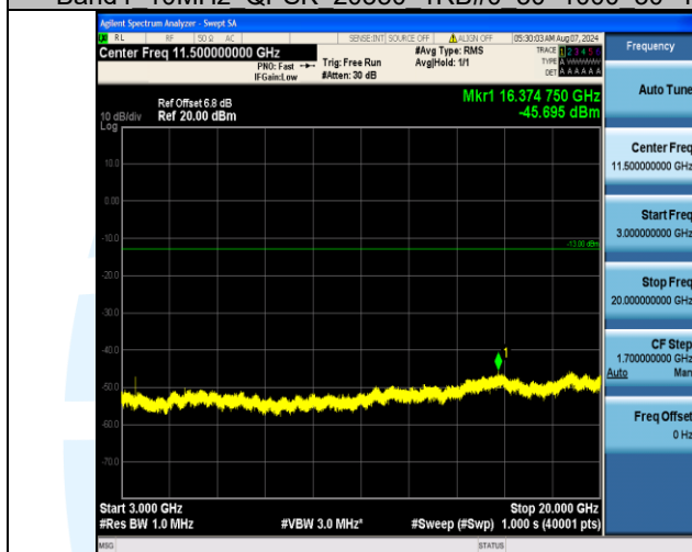
Band4_10MHz_QPSK_20350_1RB#0_3000~20000_3000~20000
