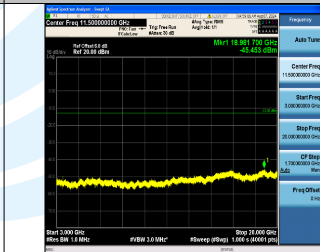
Band4_5MHz_16QAM_20375_25RB#0_3000~20000_3000~20000
