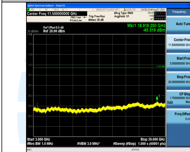
Band4_5MHz_16QAM_20375_1RB#24_3000~20000_3000~20000
