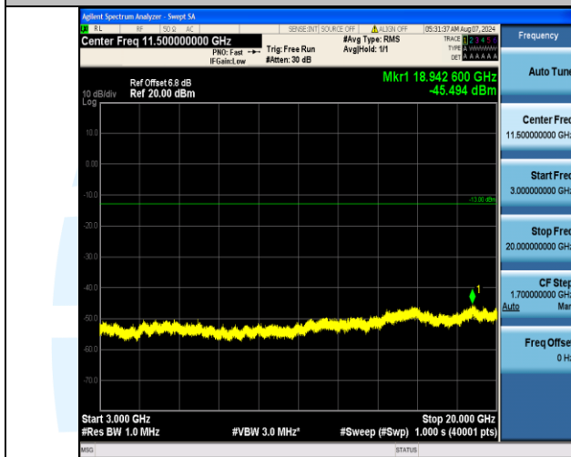
Band4_10MHz_QPSK_20350_50RB#0_3000~20000_3000~20000
