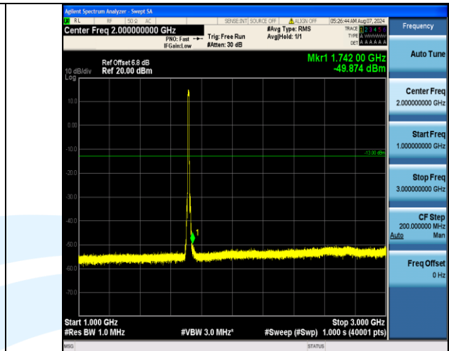
Band4_10MHz_QPSK_20000_50RB#0_1000~3000_1000~3000
