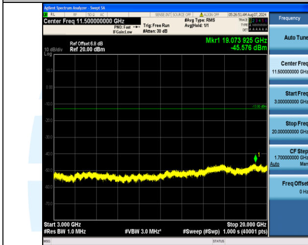
Band4_10MHz_QPSK_20000_50RB#0_3000~20000_3000~20000
