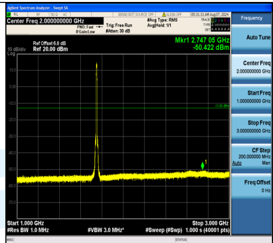
Band4_10MHz_QPSK_20350_50RB#0_1000~3000_1000~3000
