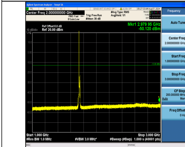
Band4_10MHz_QPSK_20175_1RB#0_1000~3000_1000~3000
