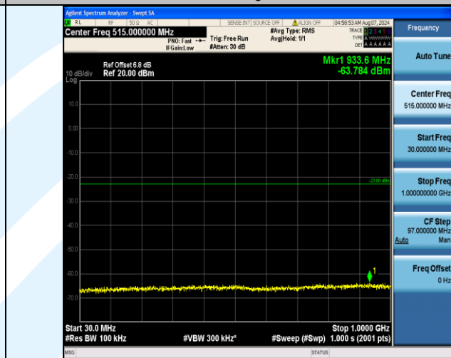
Band4_5MHz_16QAM_20375_25RB#0_30~1000_30~1000
