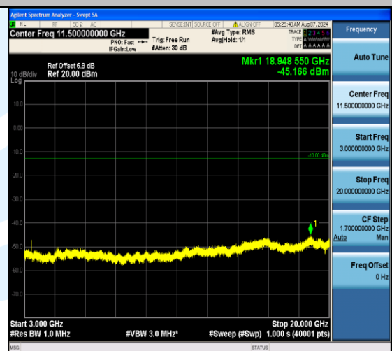
Band4_10MHz_16QAM_20000_1RB#0_3000~20000_3000~20000
