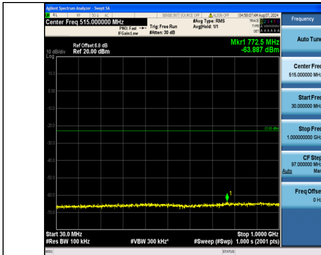
Band4_5MHz_16QAM_20375_1RB#24_30~1000_30~1000
