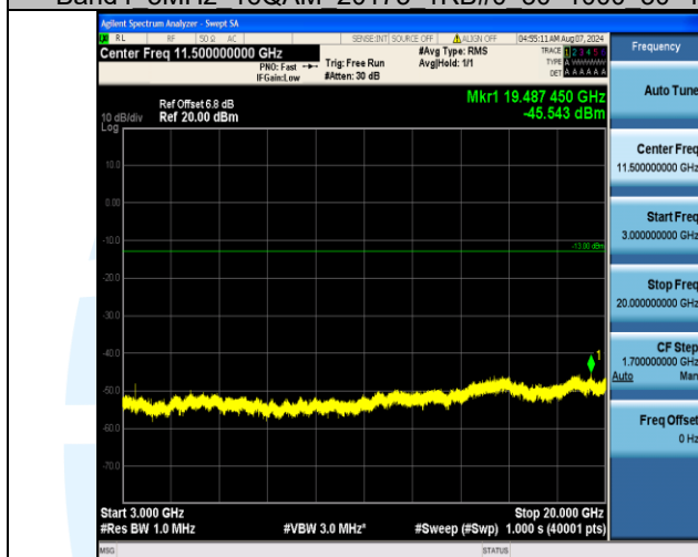
Band4_5MHz_16QAM_20175_1RB#0_3000~20000_3000~20000
