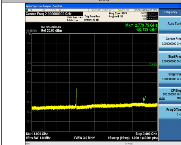
Band4_10MHz_16QAM_20000_1RB#0_1000~3000_1000~3000
