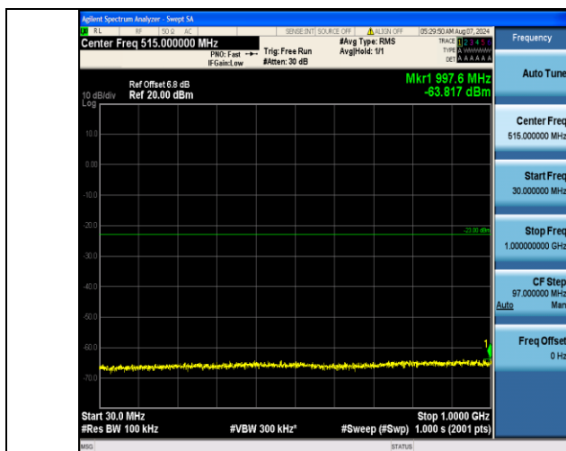
Band4_10MHz_QPSK_20350_1RB#0_30~1000_30~1000
