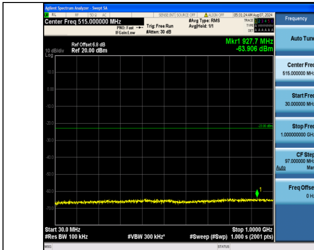
Band4_10MHz_QPSK_20350_50RB#0_30~1000_30~1000
