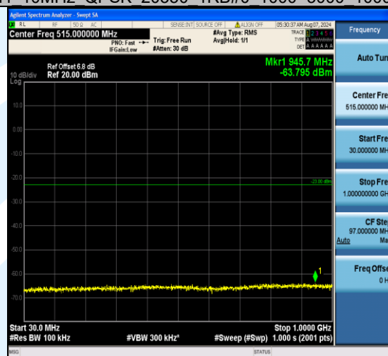
Band4_10MHz_QPSK_20350_1RB#49_30~1000_30~1000
