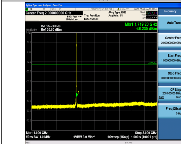
Band4_3MHz_16QAM_19965_15RB#0_1000~3000_1000~3000
