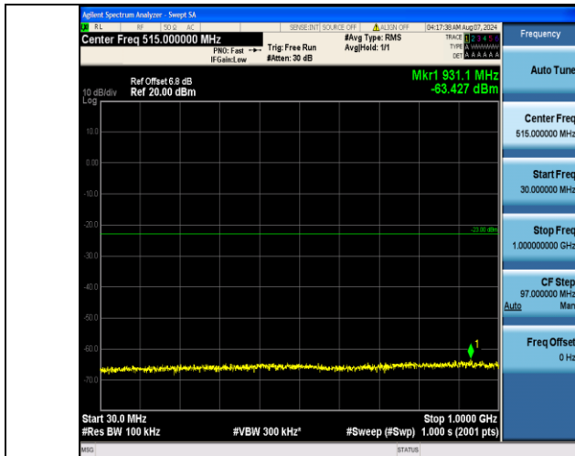
Band4_3MHz_16QAM_19965_1RB#14_30~1000_30~1000
