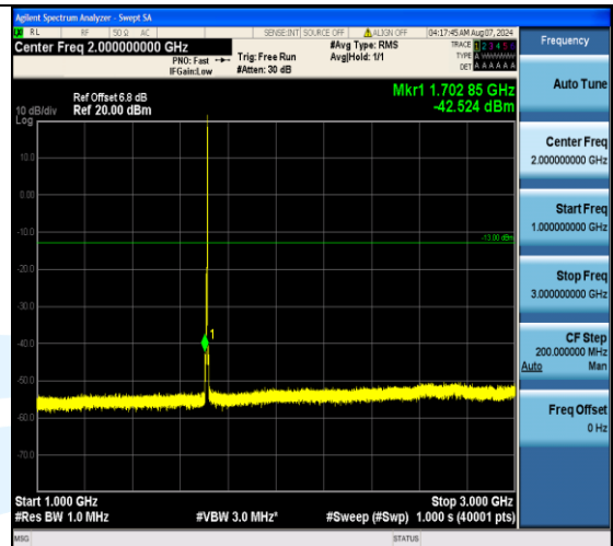
Band4_3MHz_16QAM_19965_1RB#14_1000~3000_1000~3000
