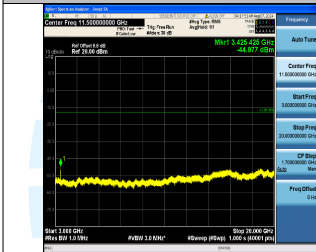
Band4_3MHz_16QAM_19965_1RB#14_3000~20000_3000~20000
