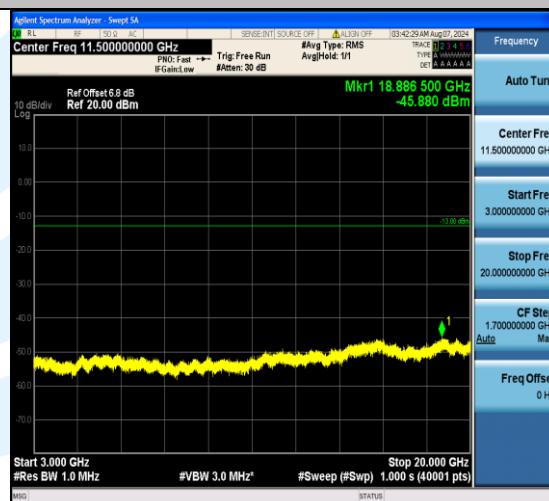
Band4_1.4MHz_QPSK_20175_6RB#0_3000~20000_3000~20000
