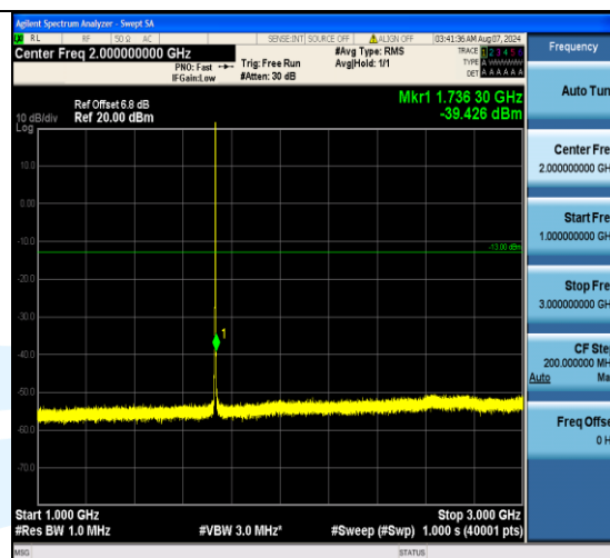
Band4_1.4MHz_QPSK_20175_1RB#5_1000~3000_1000~3000
