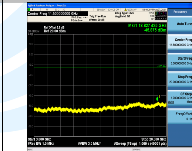
Band4_1.4MHz_16QAM_19957_6RB#0_3000~20000_3000~20000
