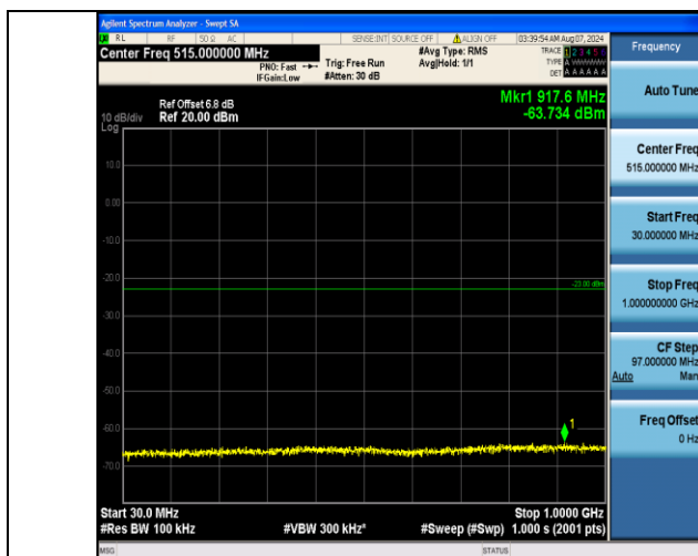
Band4_1.4MHz_QPSK_19957_6RB#0_30~1000_30~1000
