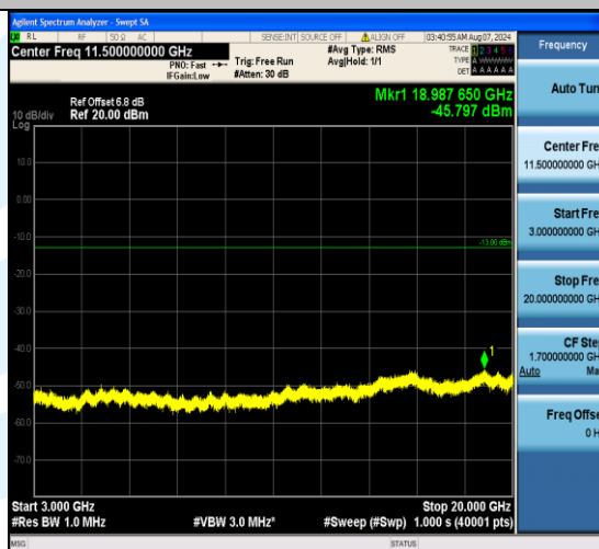
Band4_1.4MHz_QPSK_19957_6RB#0_3000~20000_3000~20000
