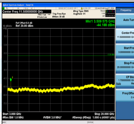
Band4_1.4MHz_QPSK_20393_1RB#5_3000~20000_3000~20000
