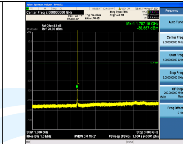
Band4_1.4MHz_16QAM_19957_1RB#5_1000~3000_1000~3000
