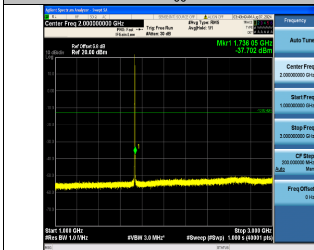
Band4_1.4MHz_QPSK_19957_6RB#0_1000~3000_1000~3000
