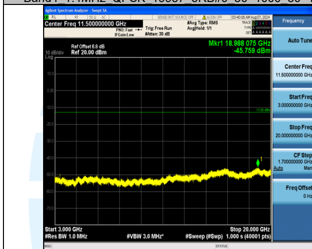
Band4_1.4MHz_QPSK_19957_6RB#0_3000~20000_3000~20000
