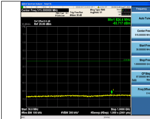
Band4_1.4MHz_16QAM_19957_1RB#5_30~1000_30~1000
