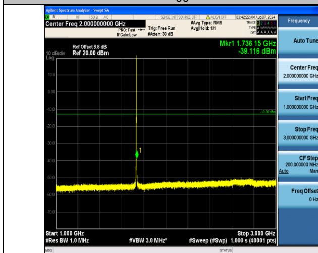
Band4_1.4MHz_QPSK_20175_6RB#0_1000~3000_1000~3000
