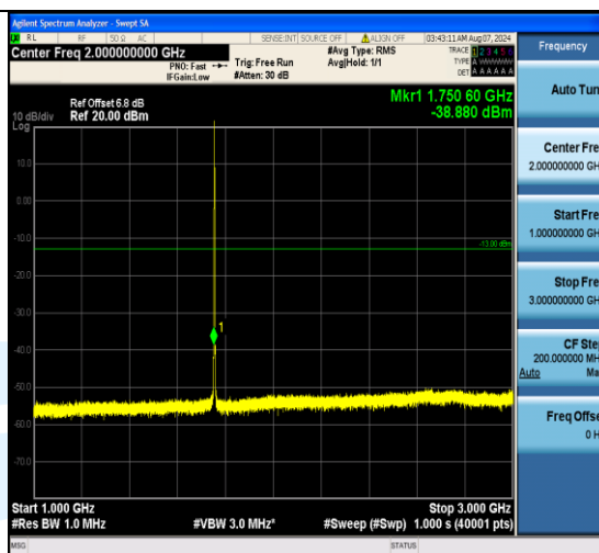
Band4_1.4MHz_QPSK_20393_1RB#0_1000~3000_1000~3000
