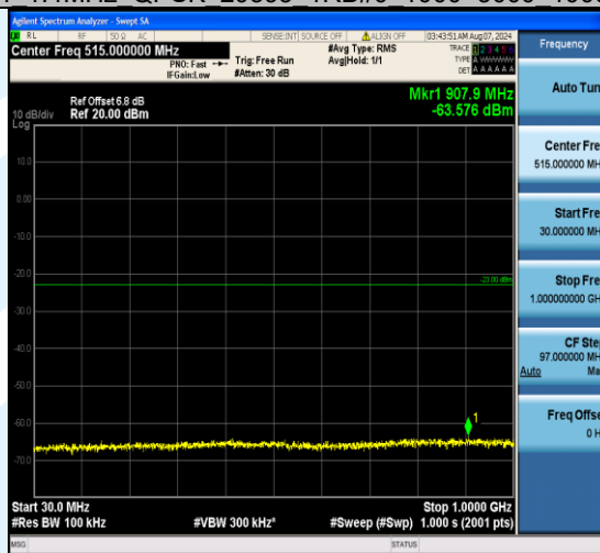
Band4_1.4MHz_QPSK_20393_1RB#5_30~1000_30~1000
