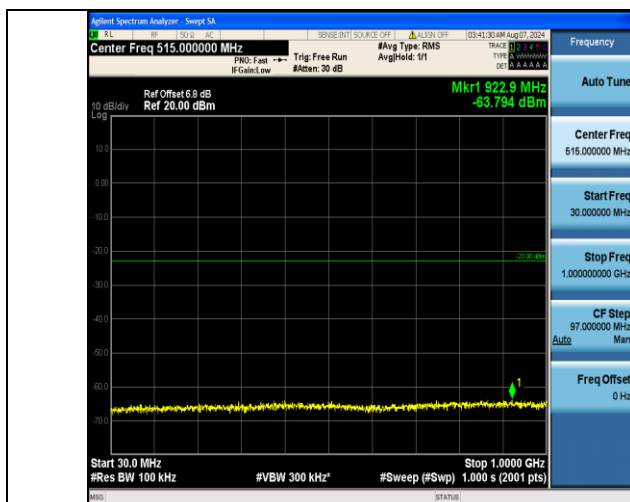
Band4_1.4MHz_QPSK_20175_1RB#5_30~1000_30~1000
