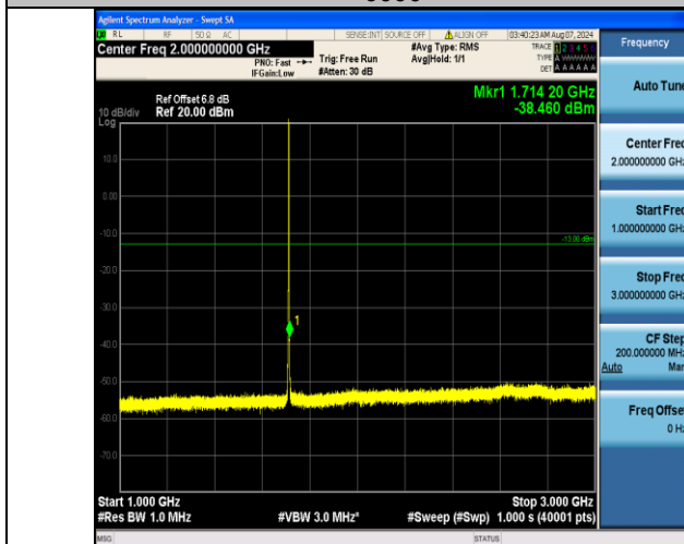
Band4_1.4MHz_16QAM_19957_6RB#0_1000~3000_1000~3000
