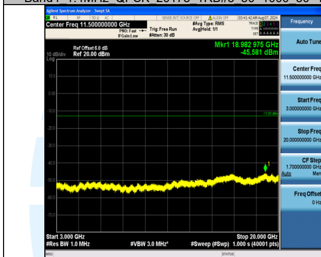
Band4_1.4MHz_QPSK_20175_1RB#5_3000~20000_3000~20000
