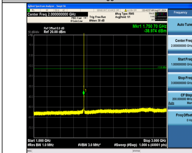
Band4_1.4MHz_QPSK_20393_1RB#5_1000~3000_1000~3000
