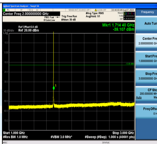
Band4_1.4MHz_QPSK_19957_6RB#0_1000~3000_1000~3000
