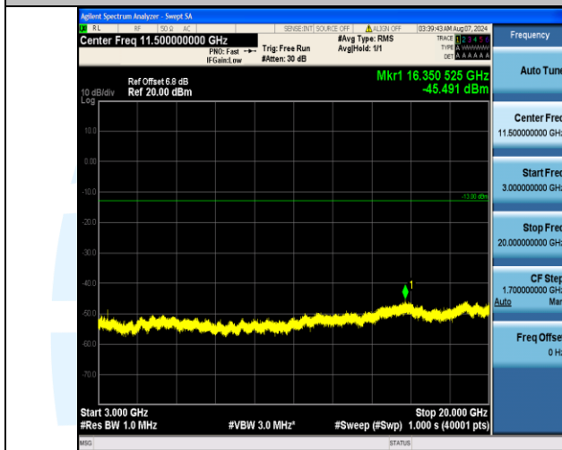
Band4_1.4MHz_16QAM_19957_1RB#5_3000~20000_3000~20000
