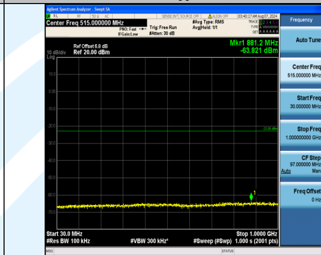
Band4_1.4MHz_16QAM_19957_6RB#0_30~1000_30~1000
