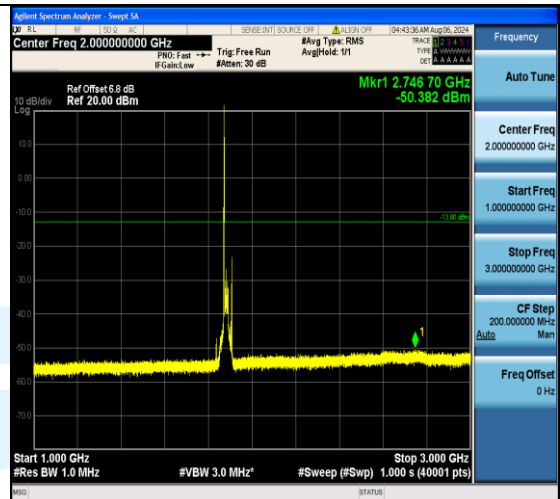
Band2_20MHz_16QAM_18900_1RB#0_1000~3000_1000~3000
