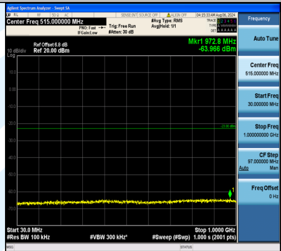
Band2_15MHz_16QAM_19125_1RB#0_30~1000_30~1000
