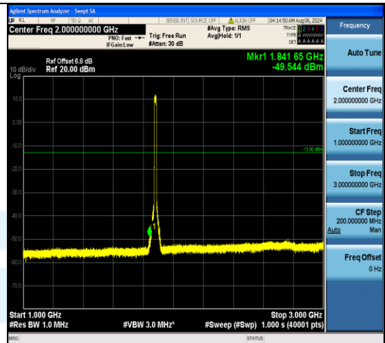
Band2_15MHz_16QAM_18900_75RB#0_1000~3000_1000~3000
