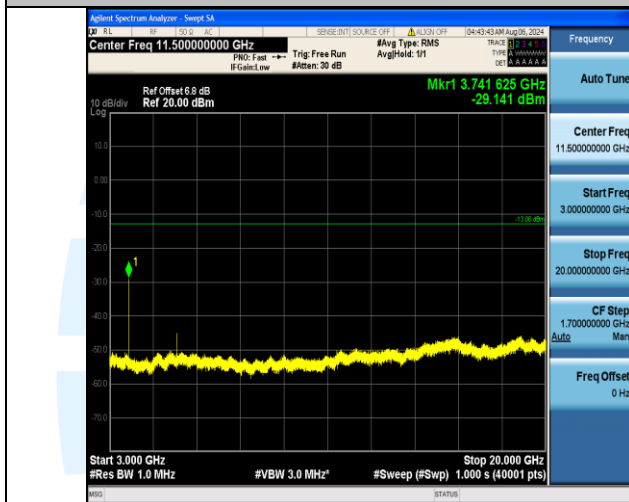
Band2_20MHz_16QAM_18900_1RB#0_3000~20000_3000~20000
