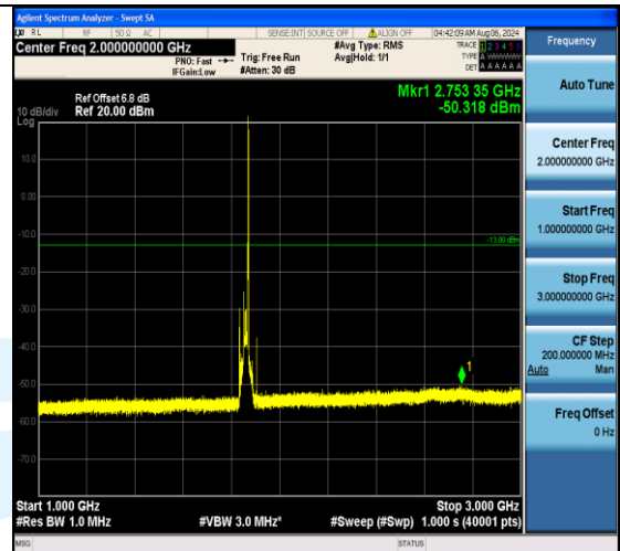
Band2_20MHz_16QAM_18700_1RB#99_1000~3000_1000~3000
