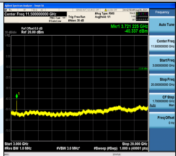
Band2_20MHz_16QAM_18700_100RB#0_3000~20000_3000~20000
