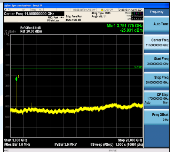
Band2_15MHz_16QAM_19125_1RB#0_3000~20000_3000~20000
