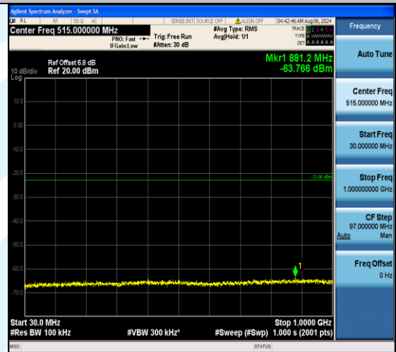
Band2_20MHz_16QAM_18700_100RB#0_30~1000_30~1000
