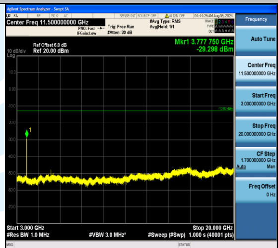
Band2_20MHz_16QAM_18900_1RB#99_3000~20000_3000~20000
