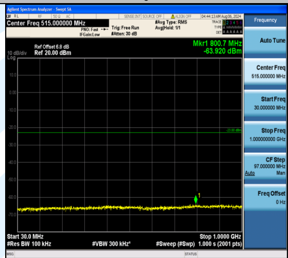
Band2_20MHz_16QAM_18900_1RB#99_30~1000_30~1000
