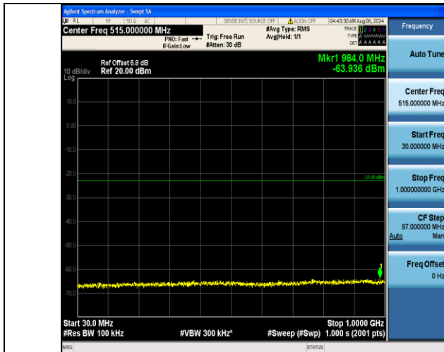
Band2_20MHz_16QAM_18900_1RB#0_30~1000_30~1000
