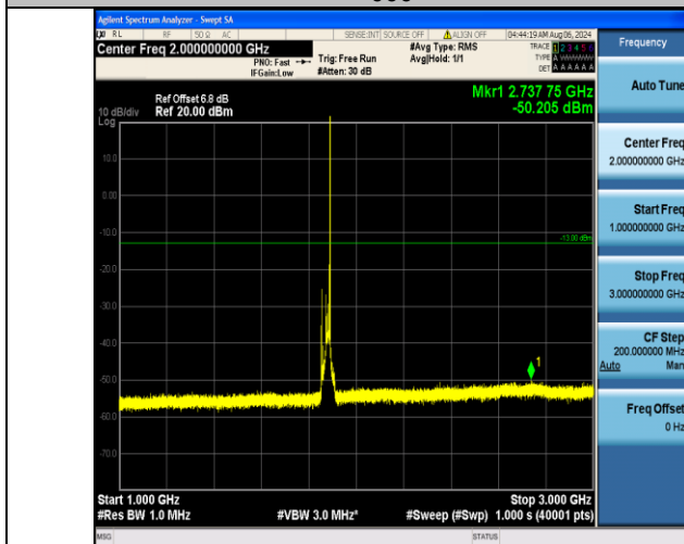
Band2_20MHz_16QAM_18900_1RB#99_1000~3000_1000~3000
