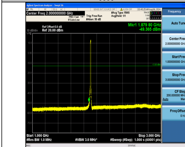
Band2_10MHz_16QAM_19150_50RB#0_1000~3000_1000~3000
