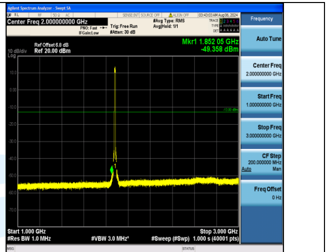
Band2_10MHz_16QAM_18900_50RB#0_1000~3000_1000~3000
