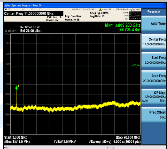
Band2_10MHz_16QAM_19150_50RB#0_3000~20000_3000~20000
