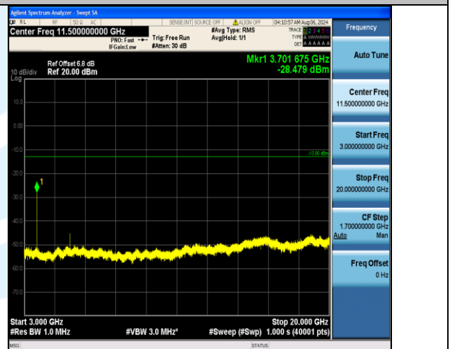
Band2_15MHz_16QAM_18675_1RB#0_3000~20000_3000~20000
