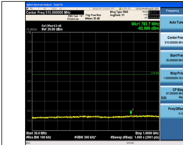
Band2_15MHz_QPSK_19125_75RB#0_30~1000_30~1000
