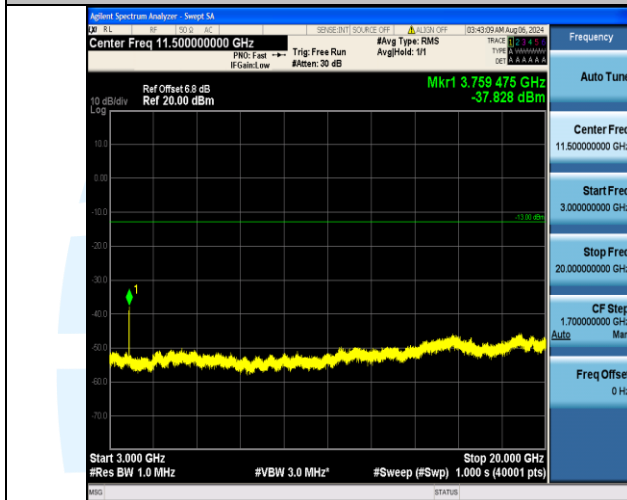
Band2_10MHz_16QAM_18900_50RB#0_3000~20000_3000~20000
