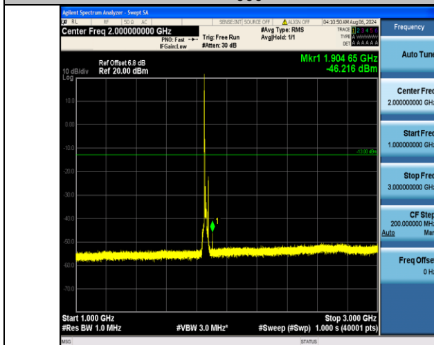
Band2_15MHz_16QAM_18675_1RB#0_1000~3000_1000~3000
