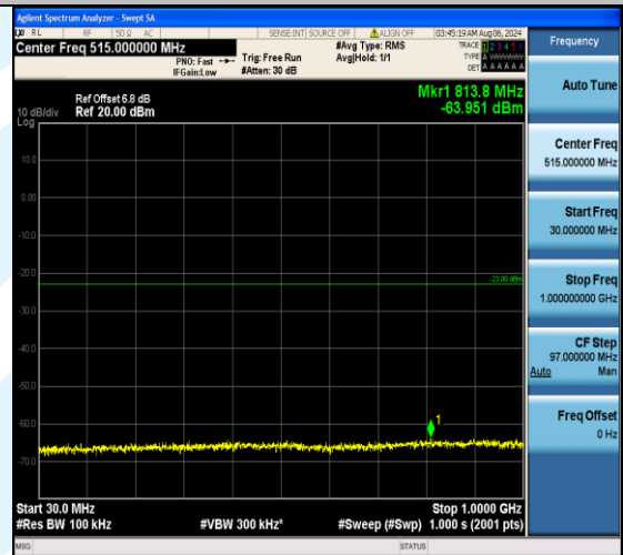
Band2_10MHz_16QAM_19150_50RB#0_30~1000_30~1000
