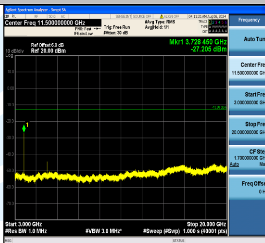
Band2_15MHz_QPSK_18675_1RB#74_3000~20000_3000~20000
