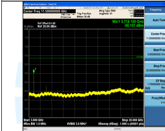
Band2_10MHz_16QAM_18650_1RB#49_3000~20000_3000~20000
