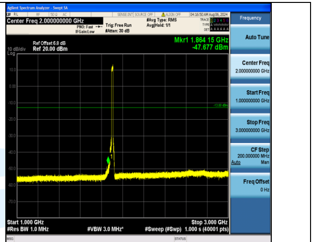
Band2_15MHz_QPSK_19125_75RB#0_1000~3000_1000~3000
