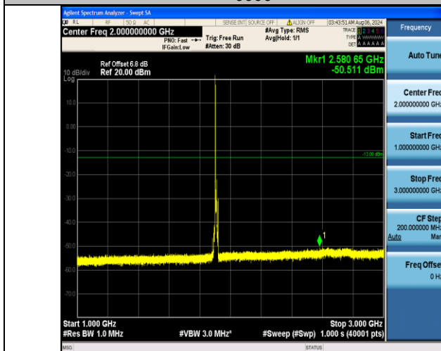
Band2_10MHz_16QAM_19150_1RB#0_1000~3000_1000~3000
