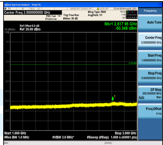
Band2_10MHz_16QAM_19150_1RB#49_1000~3000_1000~3000
