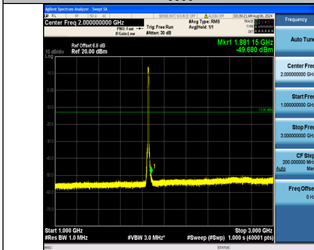
Band2_10MHz_16QAM_18650_50RB#0_1000~3000_1000~3000
