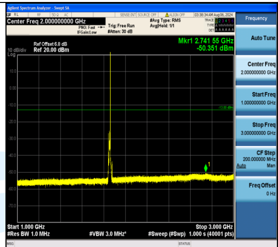
Band2_10MHz_16QAM_18650_1RB#49_1000~3000_1000~3000
