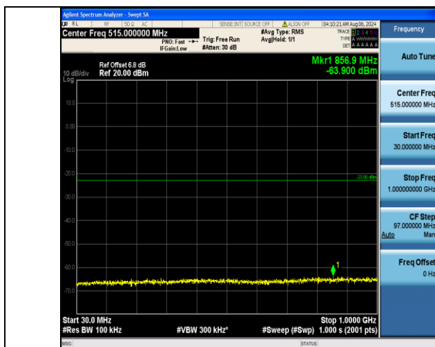
Band2_15MHz_QPSK_18675_1RB#0_30~1000_30~1000
