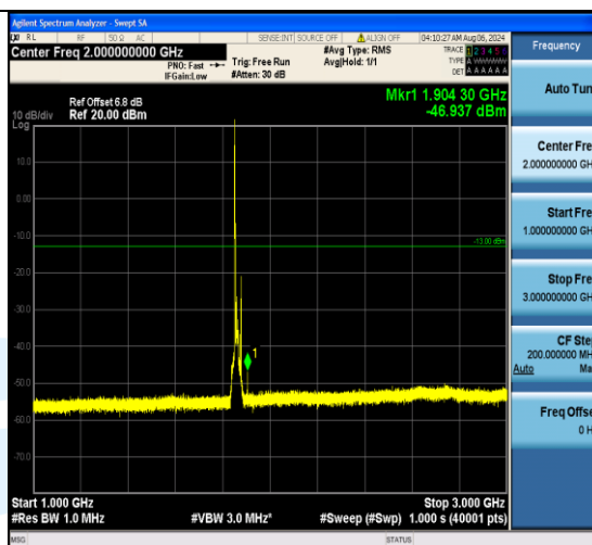
Band2_15MHz_QPSK_18675_1RB#0_1000~3000_1000~3000
