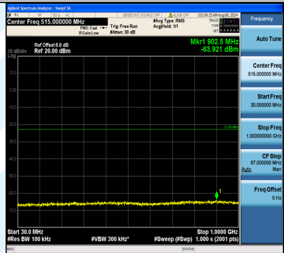
Band2_10MHz_16QAM_18650_50RB#0_30~1000_30~1000
