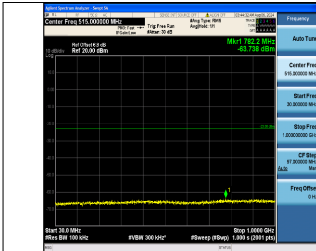
Band2_10MHz_16QAM_19150_1RB#49_30~1000_30~1000
