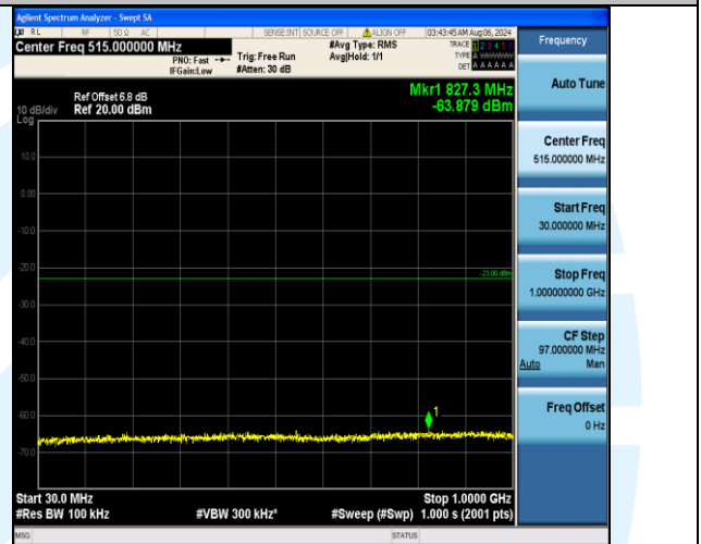
Band2_10MHz_16QAM_19150_1RB#0_30~1000_30~1000
