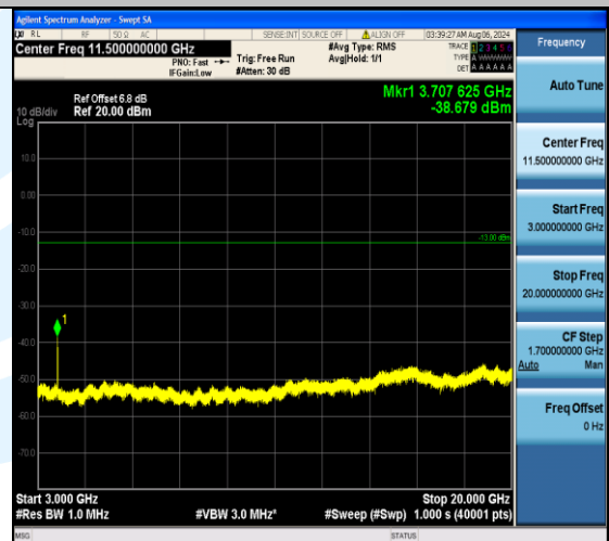
Band2_10MHz_16QAM_18650_50RB#0_3000~20000_3000~20000
