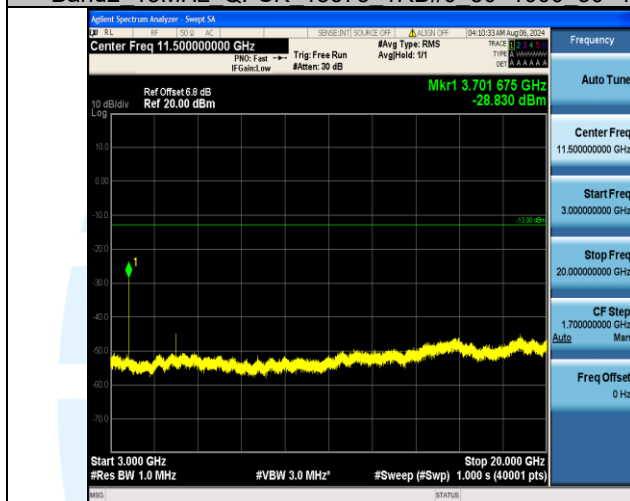
Band2_15MHz_QPSK_18675_1RB#0_3000~20000_3000~20000
