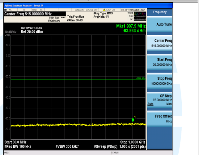
Band2_15MHz_16QAM_18675_1RB#0_30~1000_30~1000
