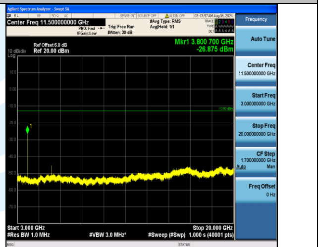
Band2_10MHz_16QAM_19150_1RB#0_3000~20000_3000~20000
