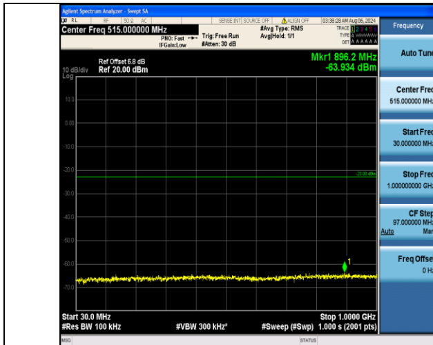
Band2_10MHz_16QAM_18650_1RB#49_30~1000_30~1000
