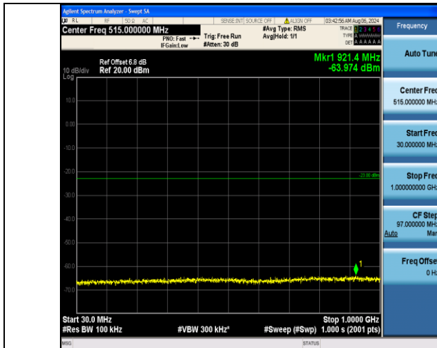
Band2_10MHz_16QAM_18900_50RB#0_30~1000_30~1000
