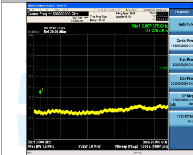
Band2_15MHz_QPSK_19125_75RB#0_3000~20000_3000~20000
