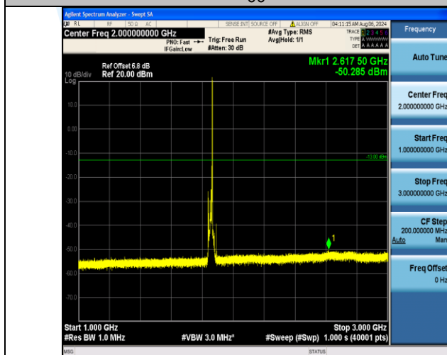
Band2_15MHz_QPSK_18675_1RB#74_1000~3000_1000~3000
