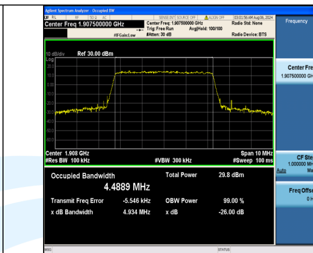
Band2-5MHz-16QAM-19175-25RB#0-PASS
