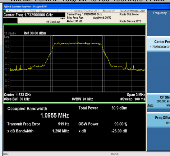
Band4-1.4MHz-QPSK-20175-6RB#0-PASS
