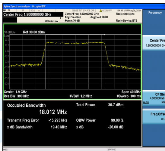
Band2-20MHz-16QAM-19100-100RB#0-PASS
