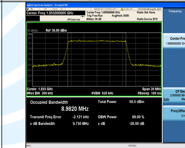
Band2-10MHz-16QAM-18650-50RB#0-PASS
