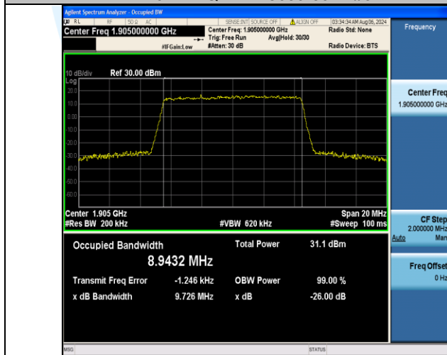
Band2-10MHz-QPSK-19150-50RB#0-PASS
