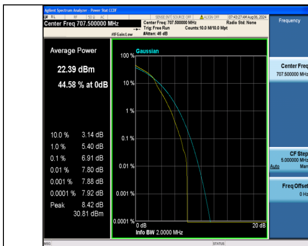
Band12-1.4MHz-16QAM-23095-1RB#0-PASS
