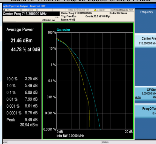
Band12-1.4MHz-16QAM-23173-6RB#0-PASS
