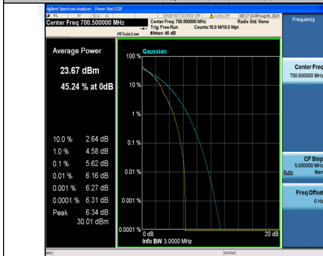
Band12-3MHz-QPSK-23025-1RB#0-PASS
