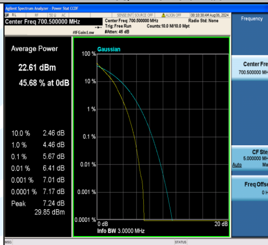
Band12-3MHz-QPSK-23025-15RB#0-PASS
