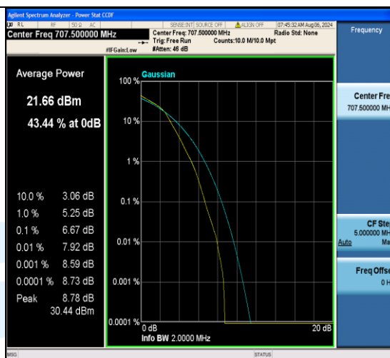
Band12-1.4MHz-16QAM-23095-6RB#0-PASS
