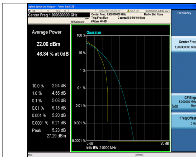
Band2-1.4MHz-16QAM-19193-1RB#0-PASS
