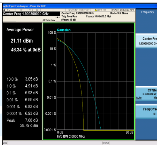
Band2-1.4MHz-16QAM-19193-6RB#0-PASS
