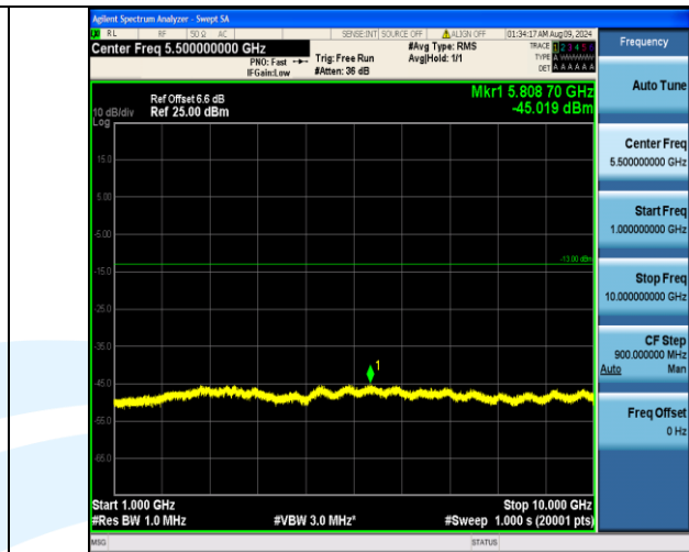
Band5-4132-1000~10000MHz-PASS
