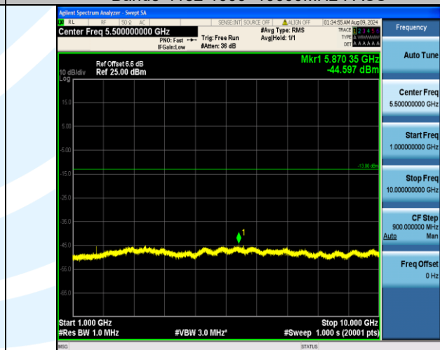
Band5-4233-1000~10000MHz-PASS
