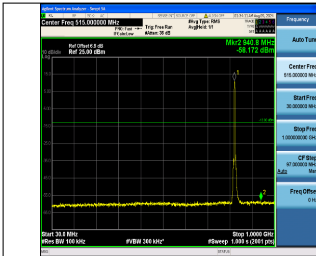
Band5-4132-30~1000MHz-PASS
