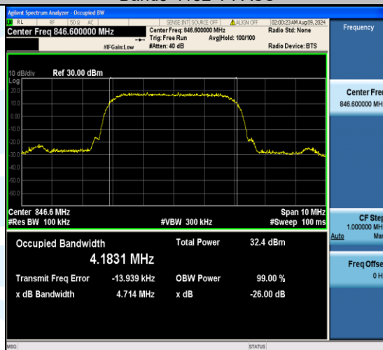
Band5-4233-1-PASS
