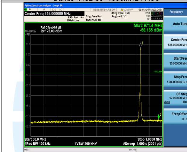
Band5-4182-30~1000MHz-PASS
