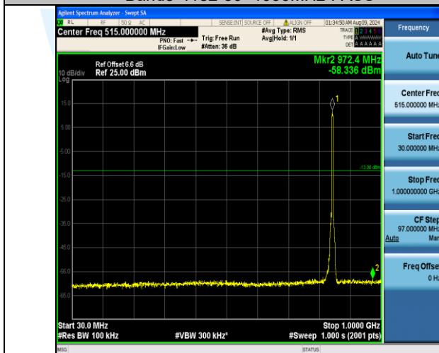
Band5-4233-30~1000MHz-PASS
