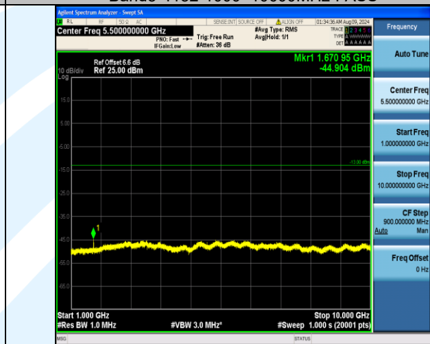
Band5-4182-1000~10000MHz-PASS
