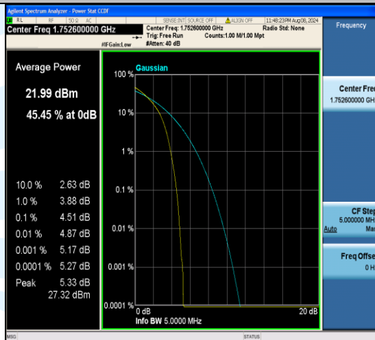
Band4-1513-1-PASS
