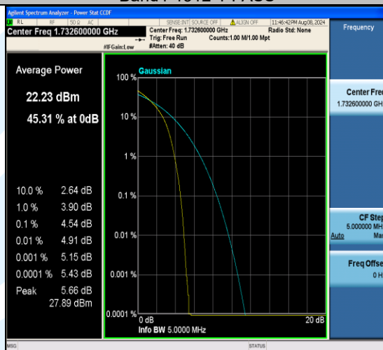
Band4-1413-1-PASS
