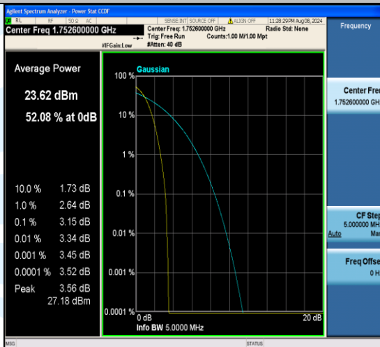
Band4-1513-1-PASS
