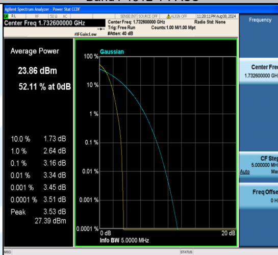
Band4-1413-1-PASS
