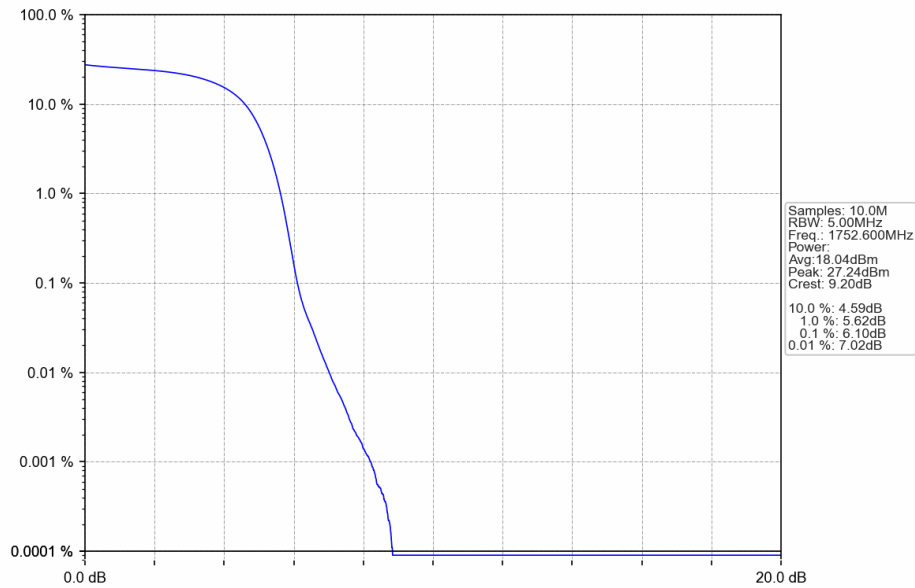
Band4_HSDPA_HCH_1752.6MHz_Subtest 1_NTNV
