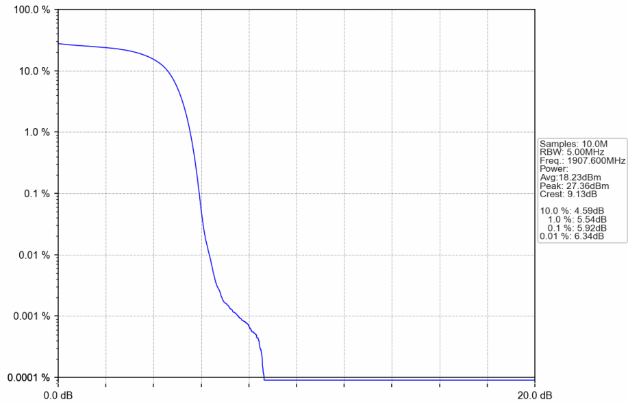
Band2_HSUPA_HCH_1907.6MHz_Subtest 1_NTNV
