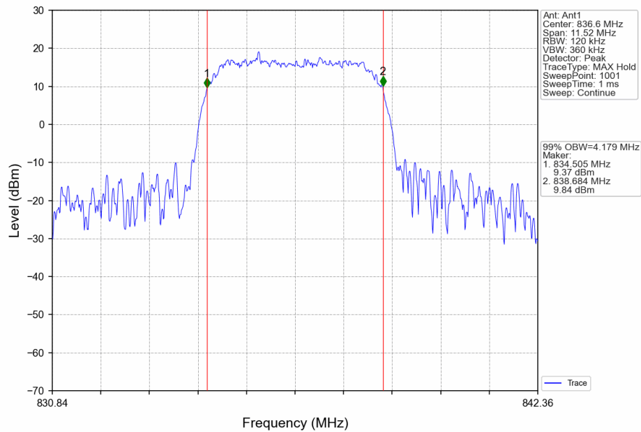
Band5_RMC_MCH_836.6MHz_12.2kbps RMC_NTNV
