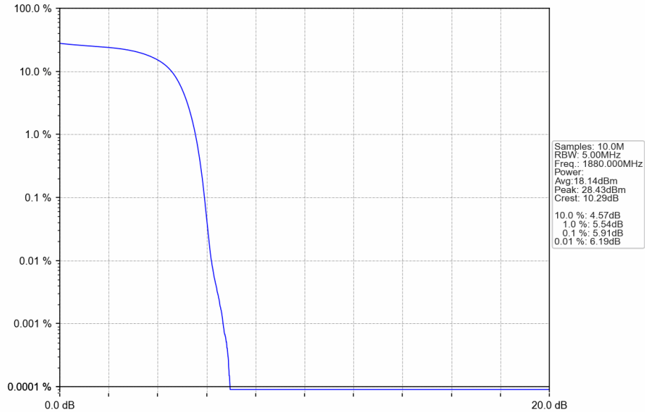
Band2_HSDPA_MCH_1880MHz_Subtest 1_NTNV
