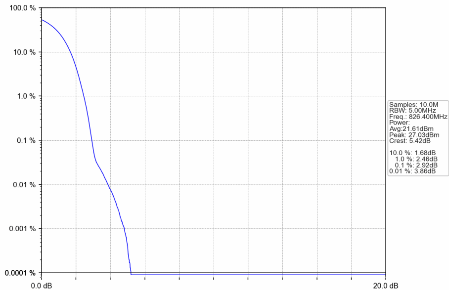
Band5_RMC_LCH_826.4MHz_12.2kbps RMC_NTNV
