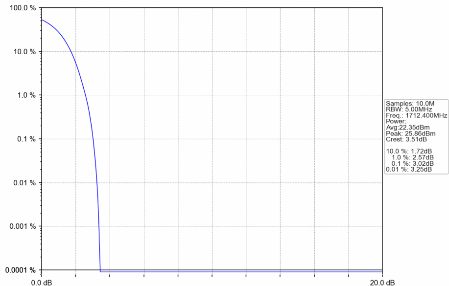
Band4_RMC_LCH_1712.4MHz_12.2kbps RMC_NTNV
