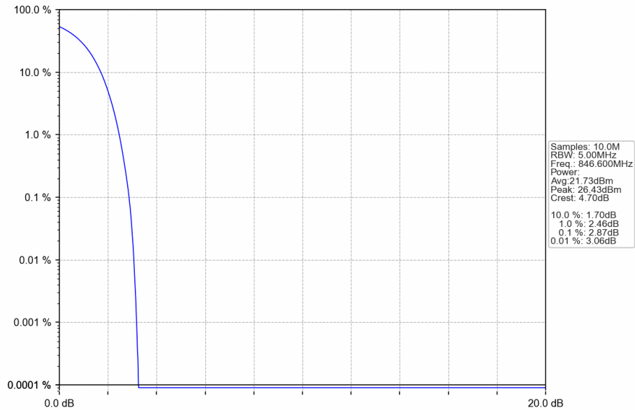
Band5_RMC_HCH_846.6MHz_12.2kbps RMC_NTNV
