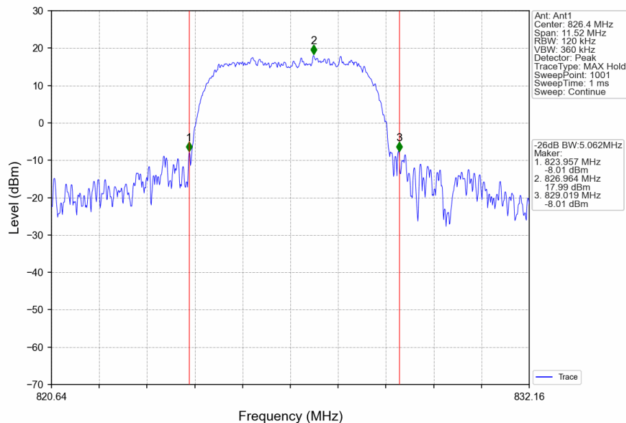
Band5_RMC_LCH_826.4MHz_12.2kbps RMC_NTNV
