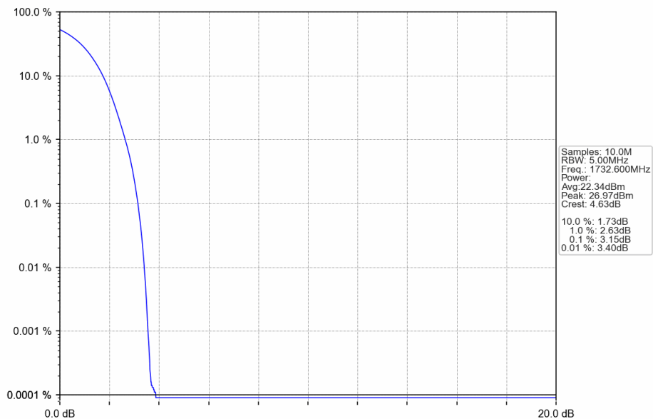
Band4_RMC_MCH_1732.6MHz_12.2kbps RMC_NTNV
