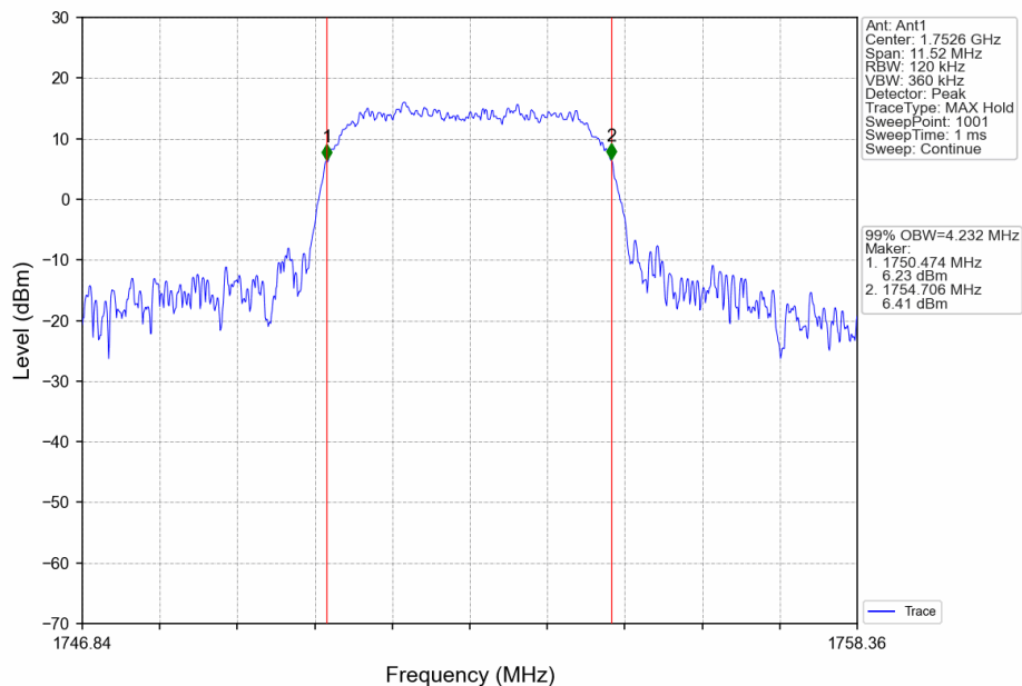
Band4_HSDPA_HCH_1752.6MHz_Subtest 1_NTNV
