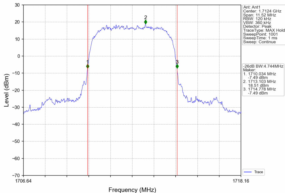
Band4_RMC_LCH_1712.4MHz_12.2kbps RMC_NTNV
