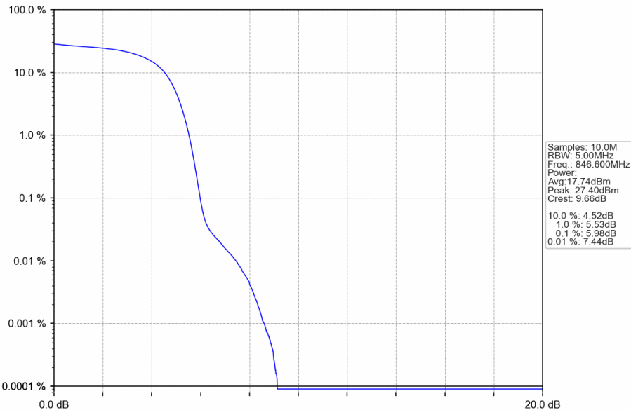
Band5_HSUPA_HCH_846.6MHz_Subtest 1_NTNV
