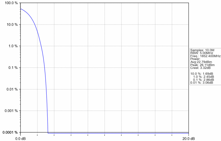
Band2_RMC_LCH_1852.4MHz_12.2kbps RMC_NTNV
