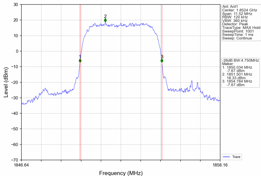
Band2_RMC_LCH_1852.4MHz_12.2kbps RMC_NTNV
