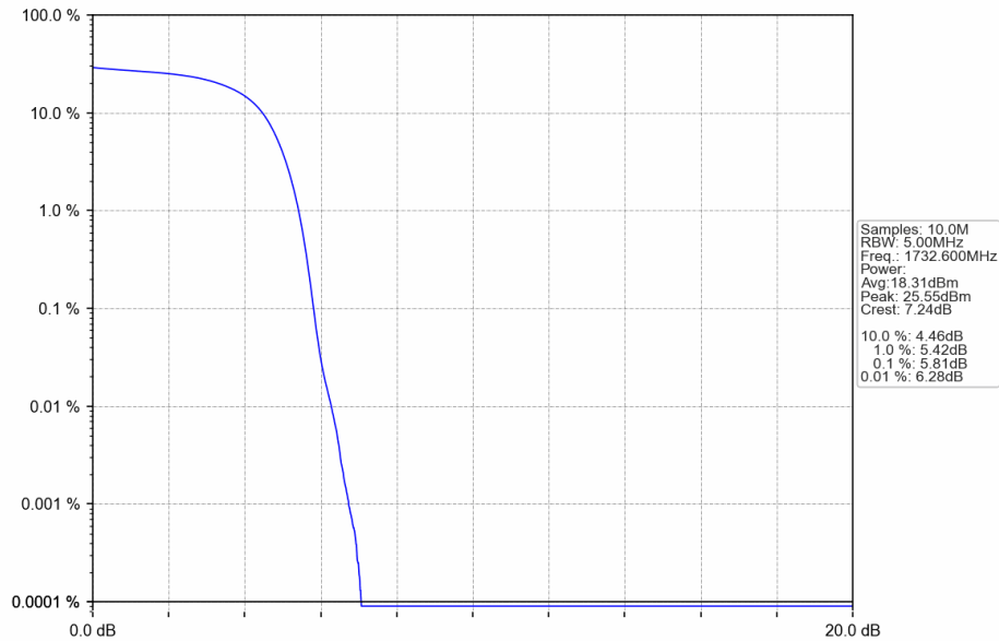
Band4_HSUPA_MCH_1732.6MHz_Subtest 1_NTNV
