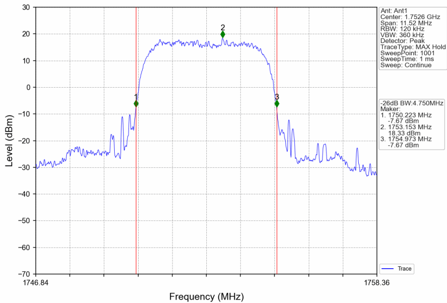
Band4_RMC_HCH_1752.6MHz_12.2kbps RMC_NTNV
