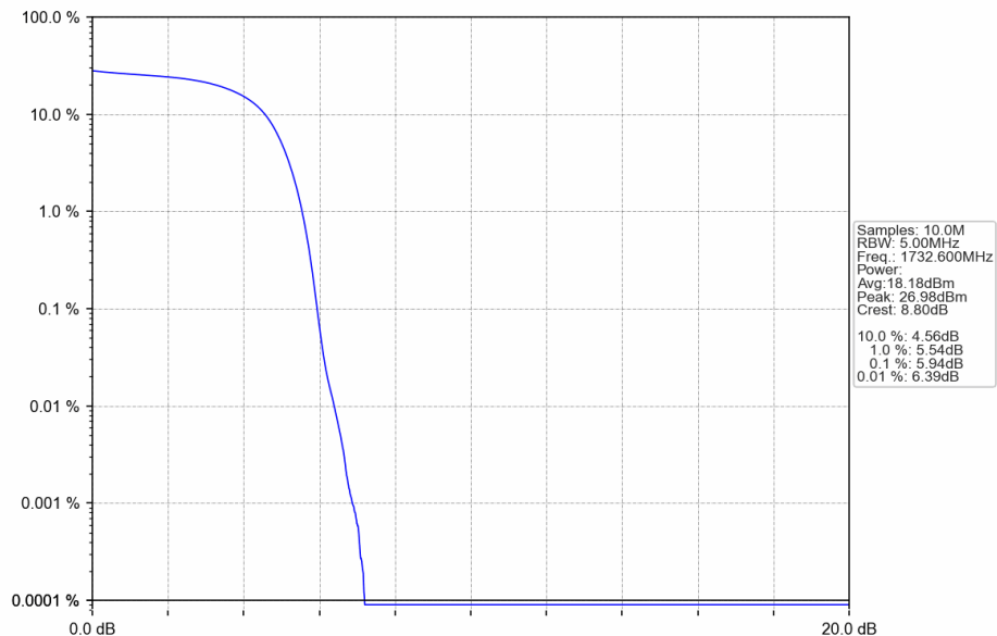
Band4_HSDPA_MCH_1732.6MHz_Subtest 1_NTNV
