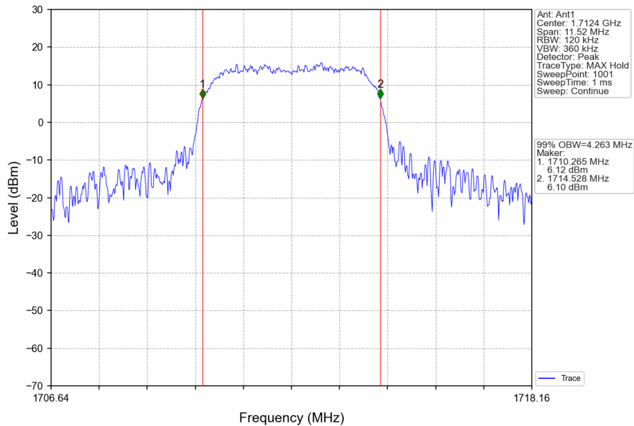
Band4_HSDPA_LCH_1712.4MHz_Subtest 1_NTNV
