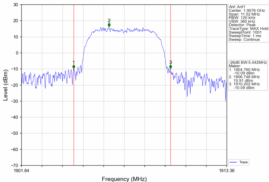
Band2_HSUPA_HCH_1907.6MHz_Subtest 1_NTNV
