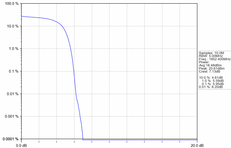
Band2_HSUPA_LCH_1852.4MHz_Subtest 1_NTNV
