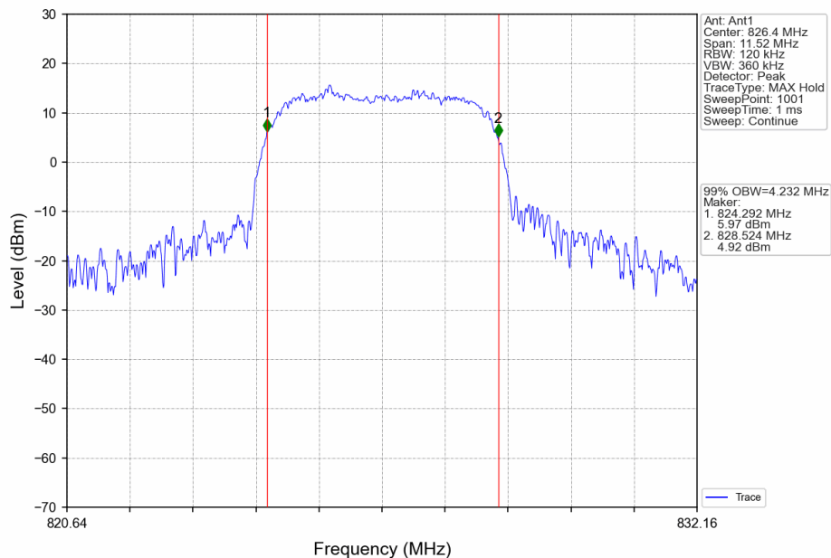
Band5_HSDPA_LCH_826.4MHz_Subtest 1_NTNV
