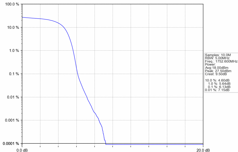
Band4_HSUPA_HCH_1752.6MHz_Subtest 1_NTNV
