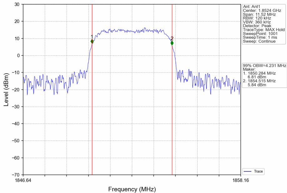
Band2_HSDPA_LCH_1852.4MHz_Subtest 1_NTNV
