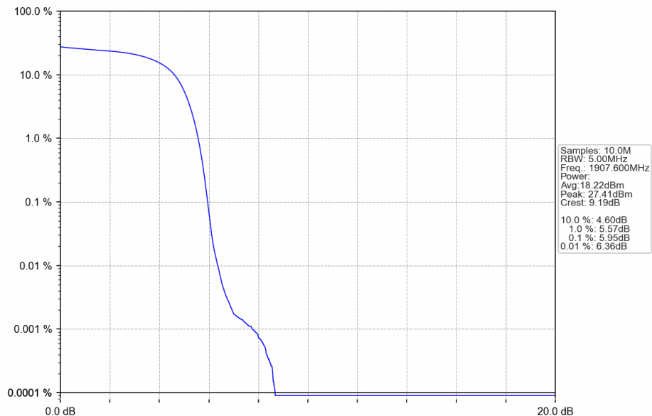
Band2_HSDPA_HCH_1907.6MHz_Subtest 1_NTNV
