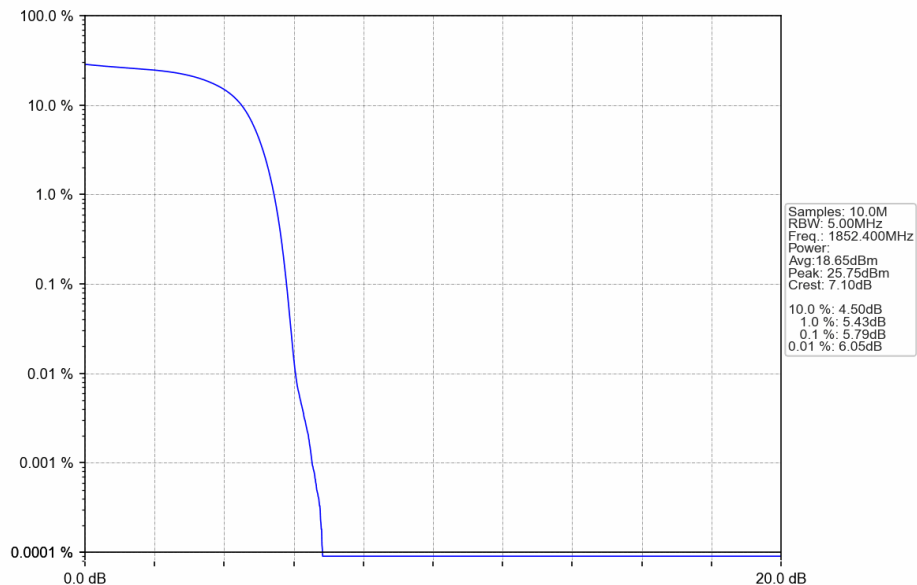
Band2_HSDPA_LCH_1852.4MHz_Subtest 1_NTNV
