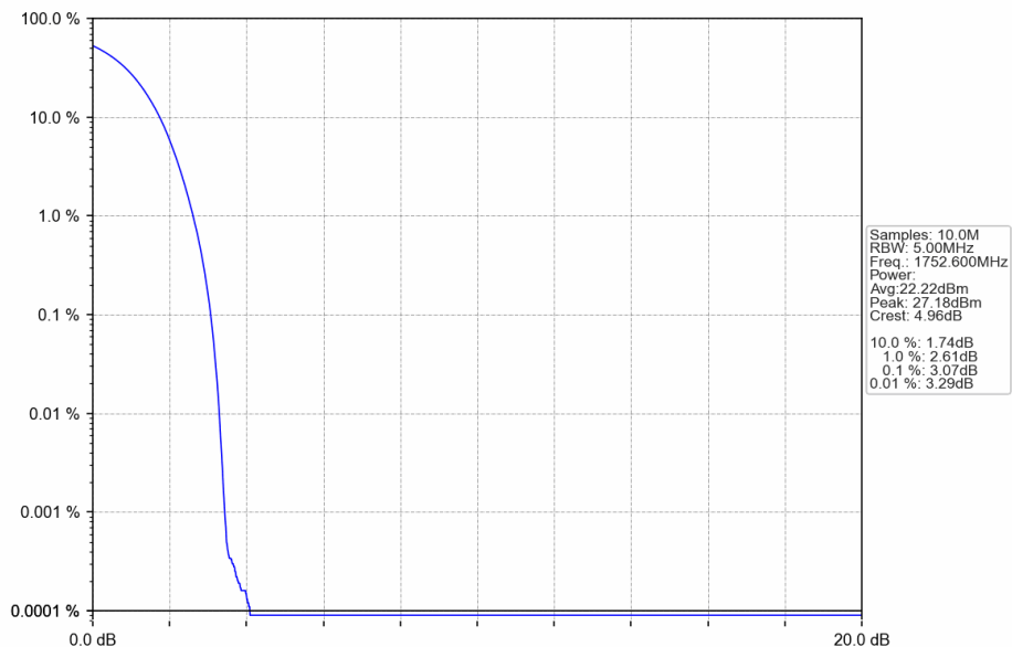
Band4_RMC_HCH_1752.6MHz_12.2kbps RMC_NTNV
