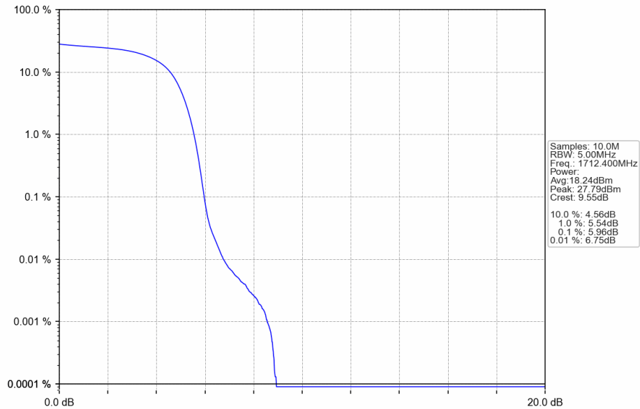
Band4_HSDPA_LCH_1712.4MHz_Subtest 1_NTNV
