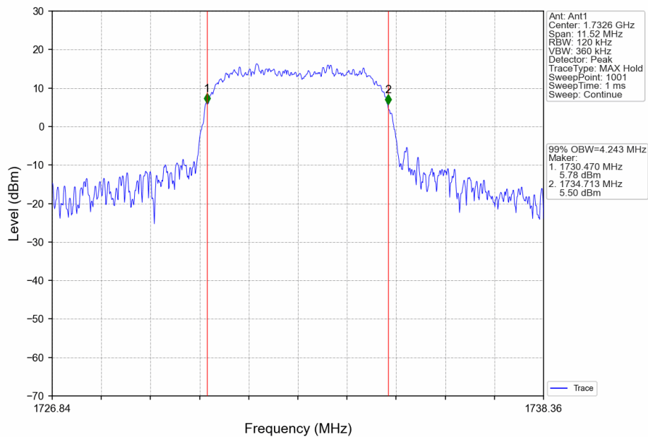
Band4_HSUPA_MCH_1732.6MHz_Subtest 1_NTNV
