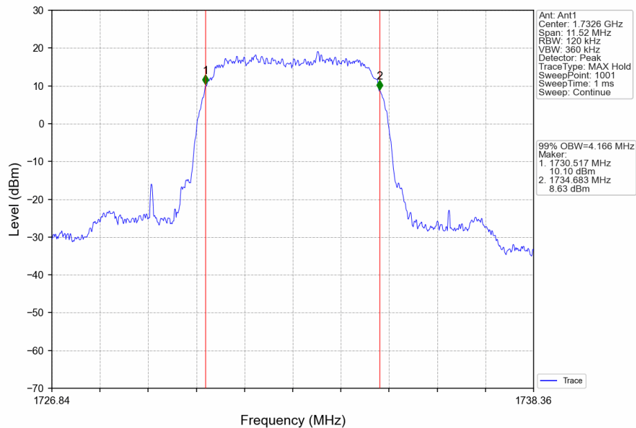
Band4_RMC_MCH_1732.6MHz_12.2kbps RMC_NTNV
