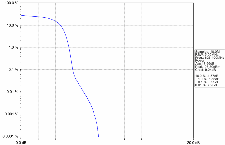
Band5_HSUPA_LCH_826.4MHz_Subtest 1_NTNV
