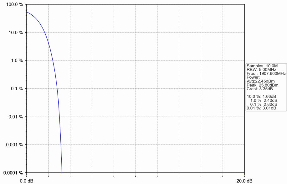
Band2_RMC_HCH_1907.6MHz_12.2kbps RMC_NTNV
