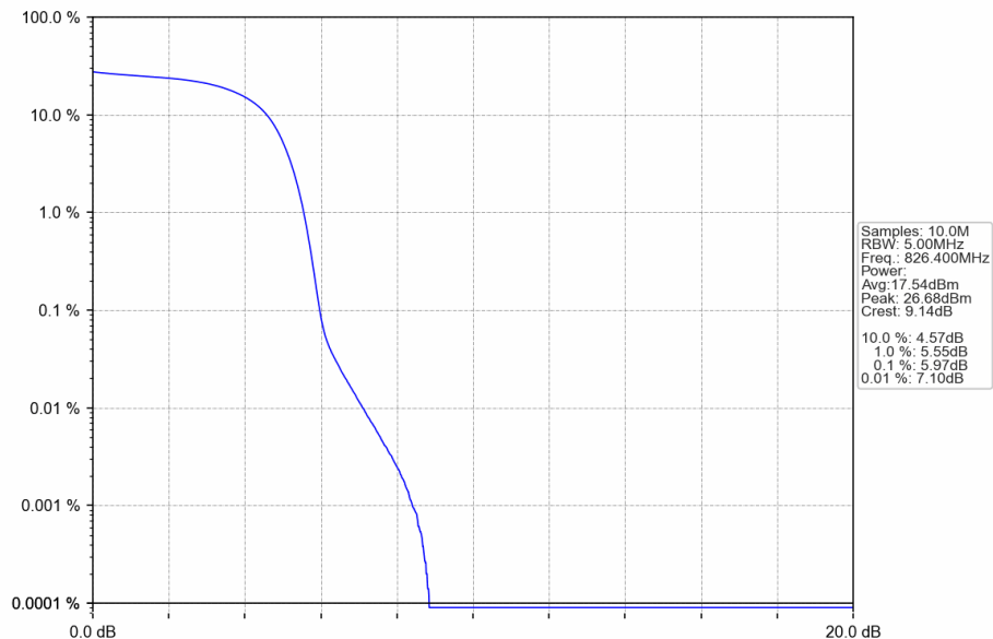
Band5_HSDPA_LCH_826.4MHz_Subtest 1_NTNV
