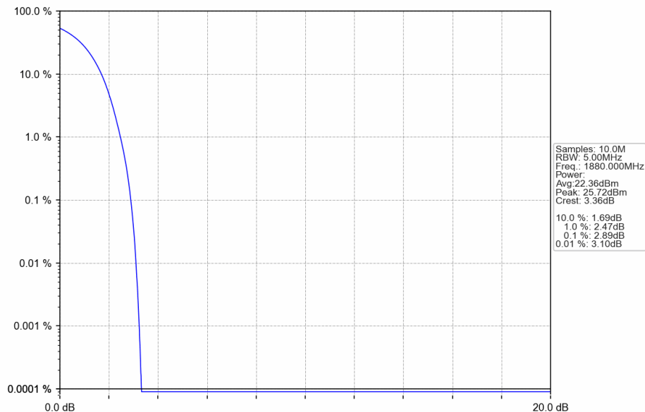
Band2_RMC_MCH_1880MHz_12.2kbps RMC_NTNV
