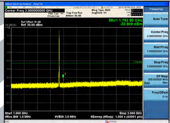
Band4_3MHz_64QAM_20175_1RB#0_1000~3000_1000~3000
