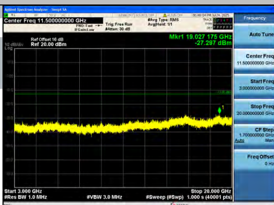
Band4_3MHz_64QAM_20175_1RB#0_3000~20000_3000~20000
