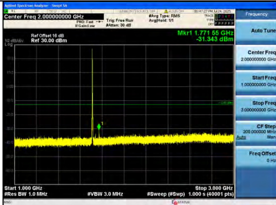
Band4_3MHz_64QAM_19965_1RB#0_1000~3000_1000~3000
