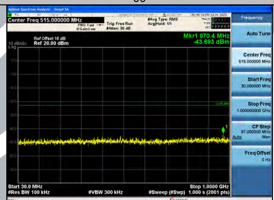
Band4_3MHz_64QAM_20385_1RB#0_30~1000_30~1000
