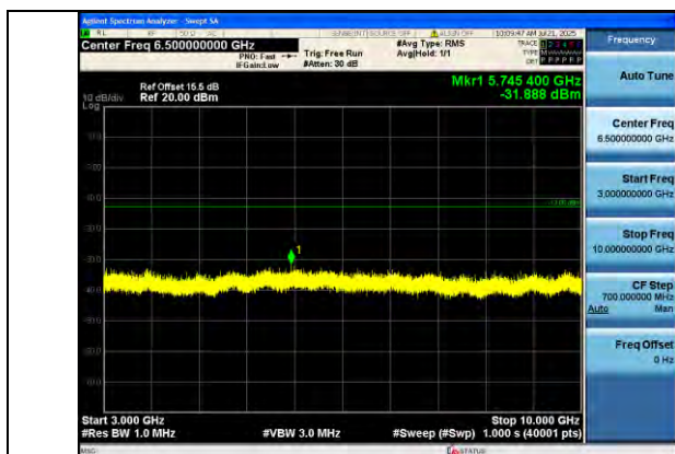
Band5_10MHz_QPSK_20450_1RB#0_3000~10000_3000~10000
