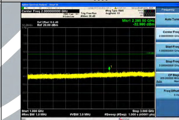
Band5_10MHz_QPSK_20600_1RB#0_1000~3000_1000~3000
