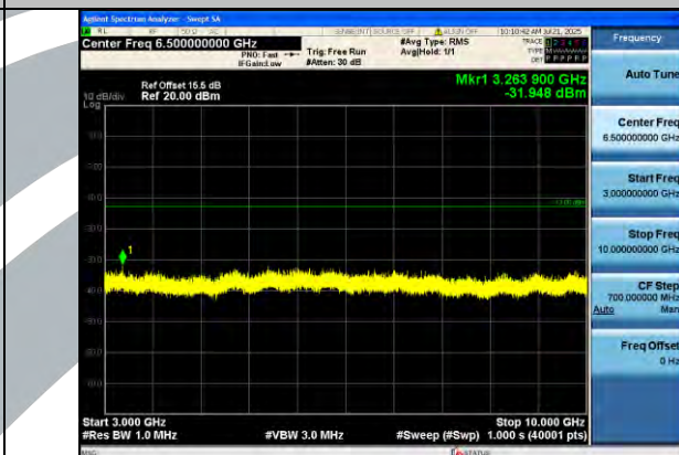
Band5_10MHz_QPSK_20525_1RB#0_3000~10000_3000~10000
