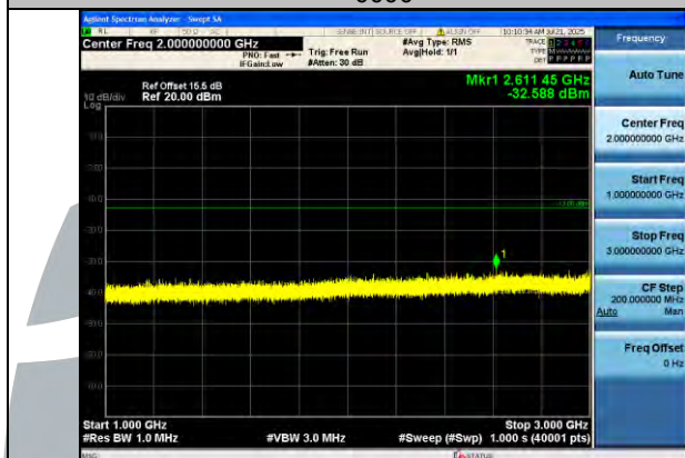
Band5_10MHz_QPSK_20525_1RB#0_1000~3000_1000~3000
