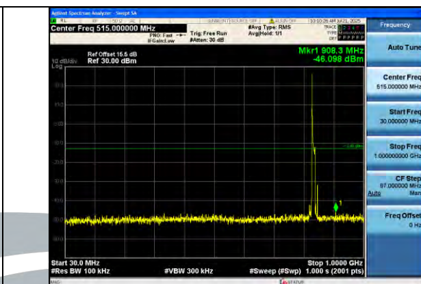
Band5_10MHz_QPSK_20525_1RB#0_30~1000_30~1000
