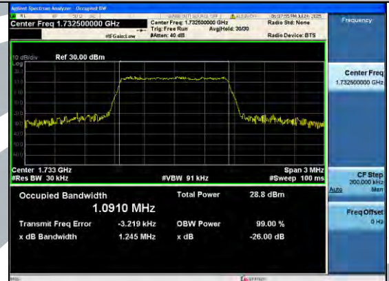
Band4-1.4MHz-64QAM-20175-6RB#0-PASS
