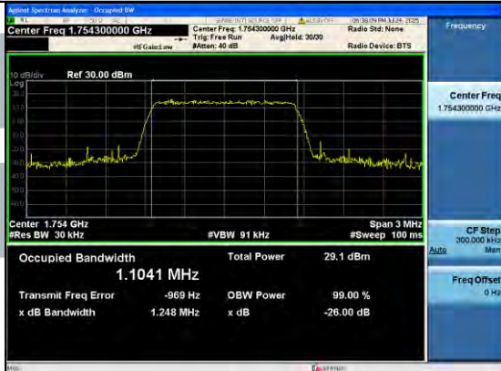
Band4-1.4MHz-64QAM-20393-6RB#0-PASS
