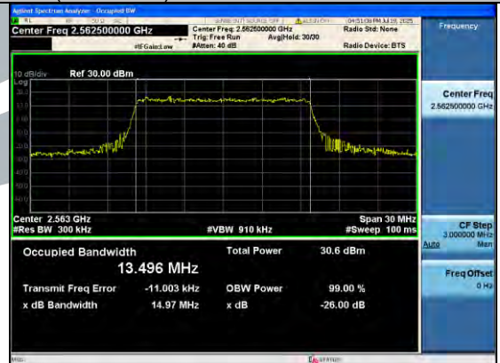
Band41(2555-2655)-15MHz-16QAM-40315-75RB#0-PASS
