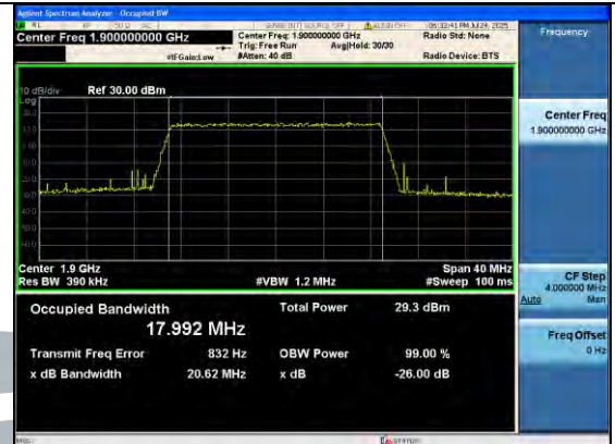
Band2-20MHz-64QAM-19100-100RB#0-PASS
