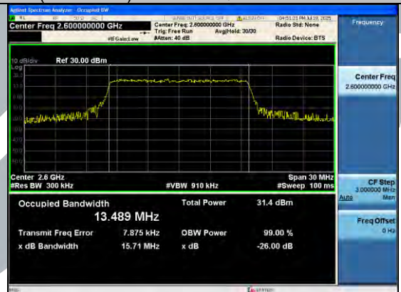
Band41(2555-2655)-15MHz-QPSK-40690-75RB#0-PASS
