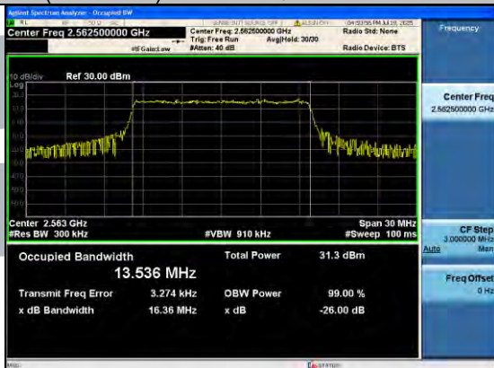
Band41(2555-2655)-15MHz-QPSK-40315-75RB#0-PASS
