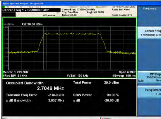
Band4-3MHz-64QAM-20175-15RB#0-PASS
