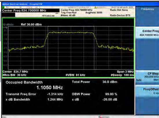
Band5-1.4MHz-64QAM-20407-6RB#0-PASS
