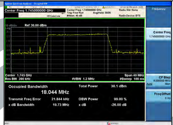
Band4-20MHz-64QAM-20300-100RB#0-PASS
