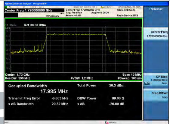
Band4-20MHz-64QAM-20050-100RB#0-PASS
