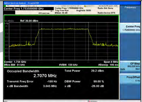
Band4-3MHz-64QAM-20385-15RB#0-PASS
