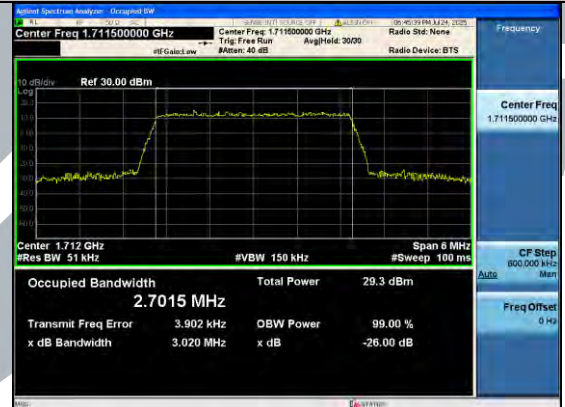
Band4-3MHz-64QAM-19965-15RB#0-PASS
