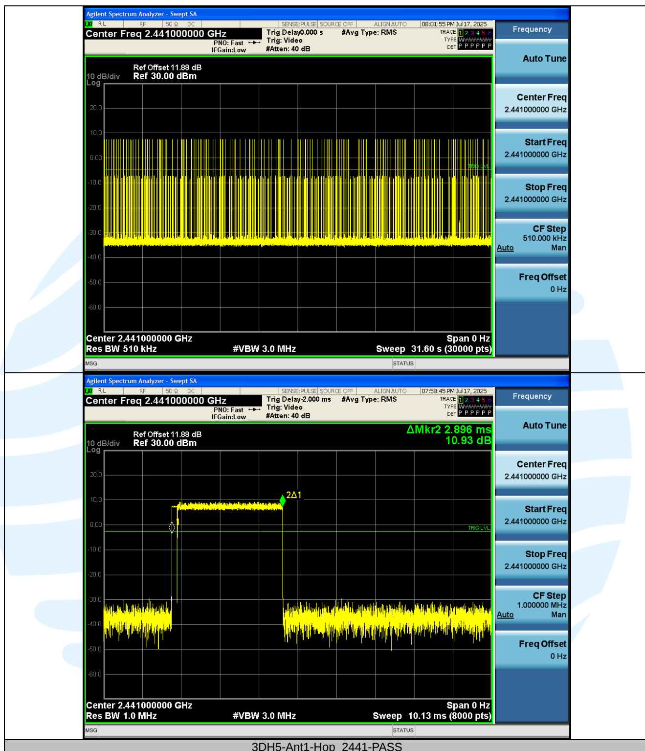
3DH5-Ant1-Hop_2441-PASS
